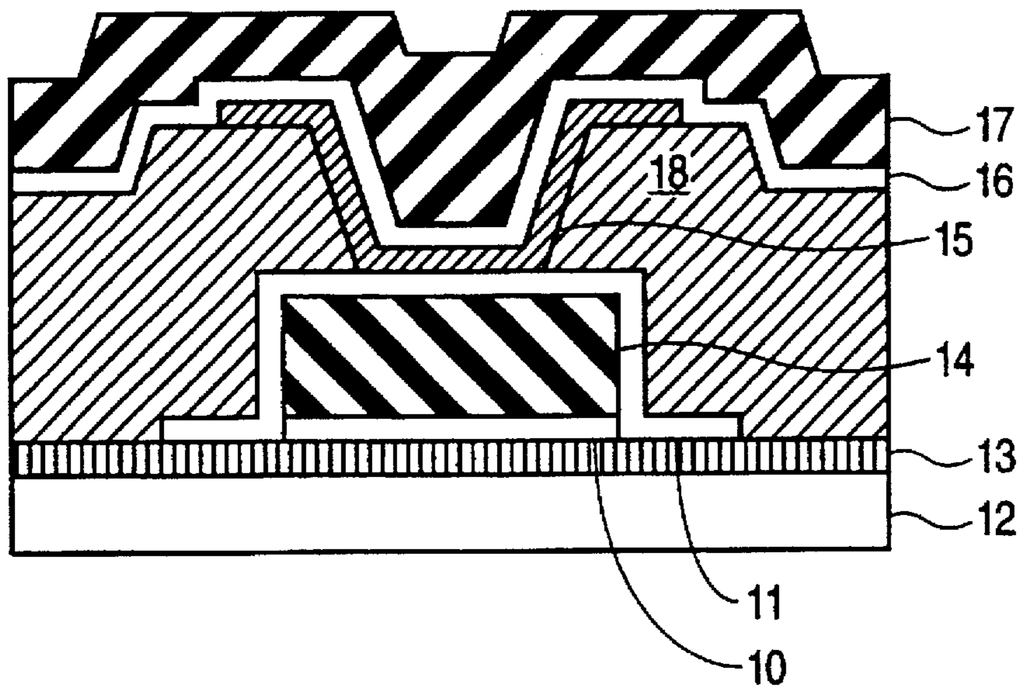
FIG. 1 (PRIOR ART)
