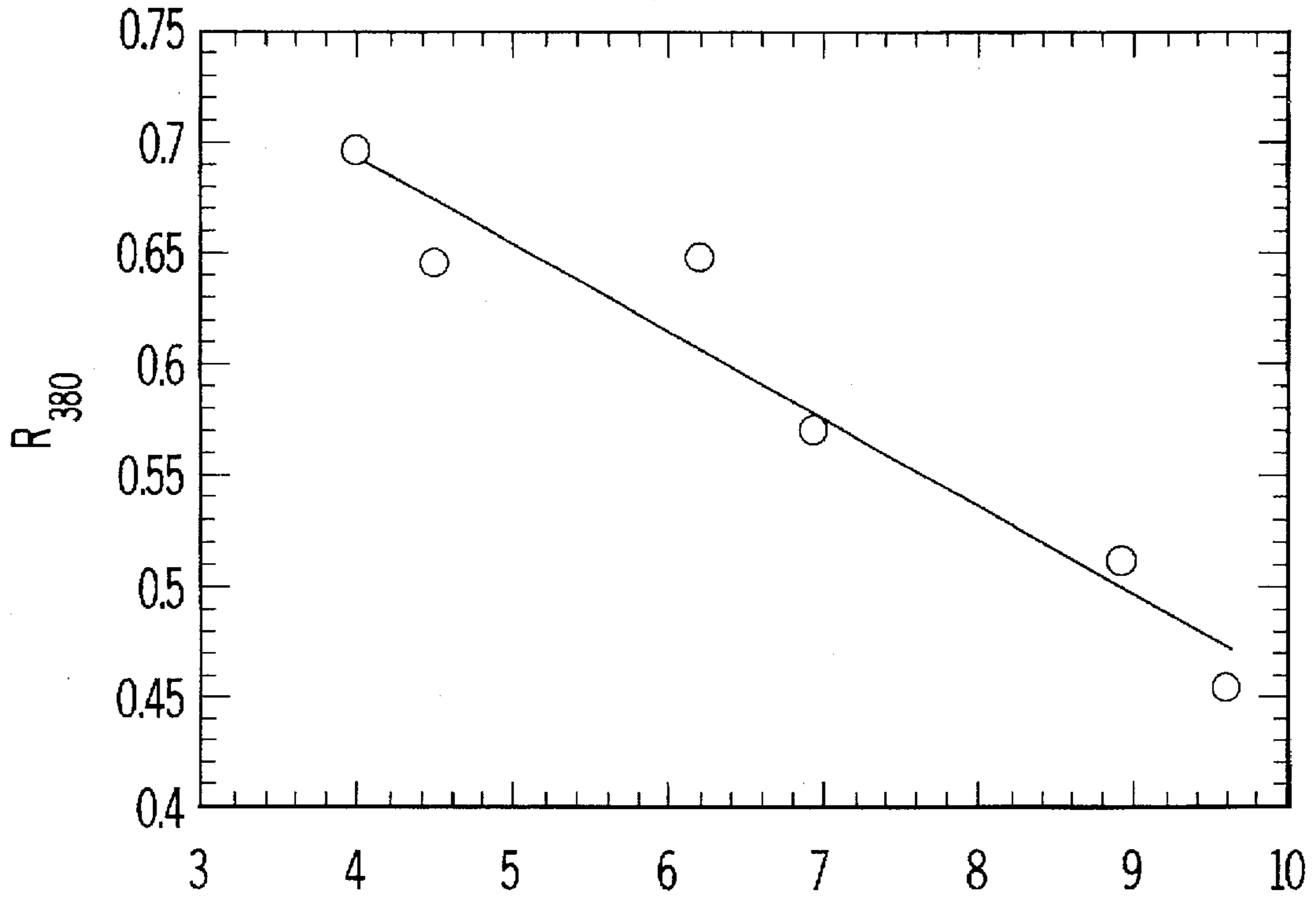
FIG. 4 THICKNESS (micrometer)
