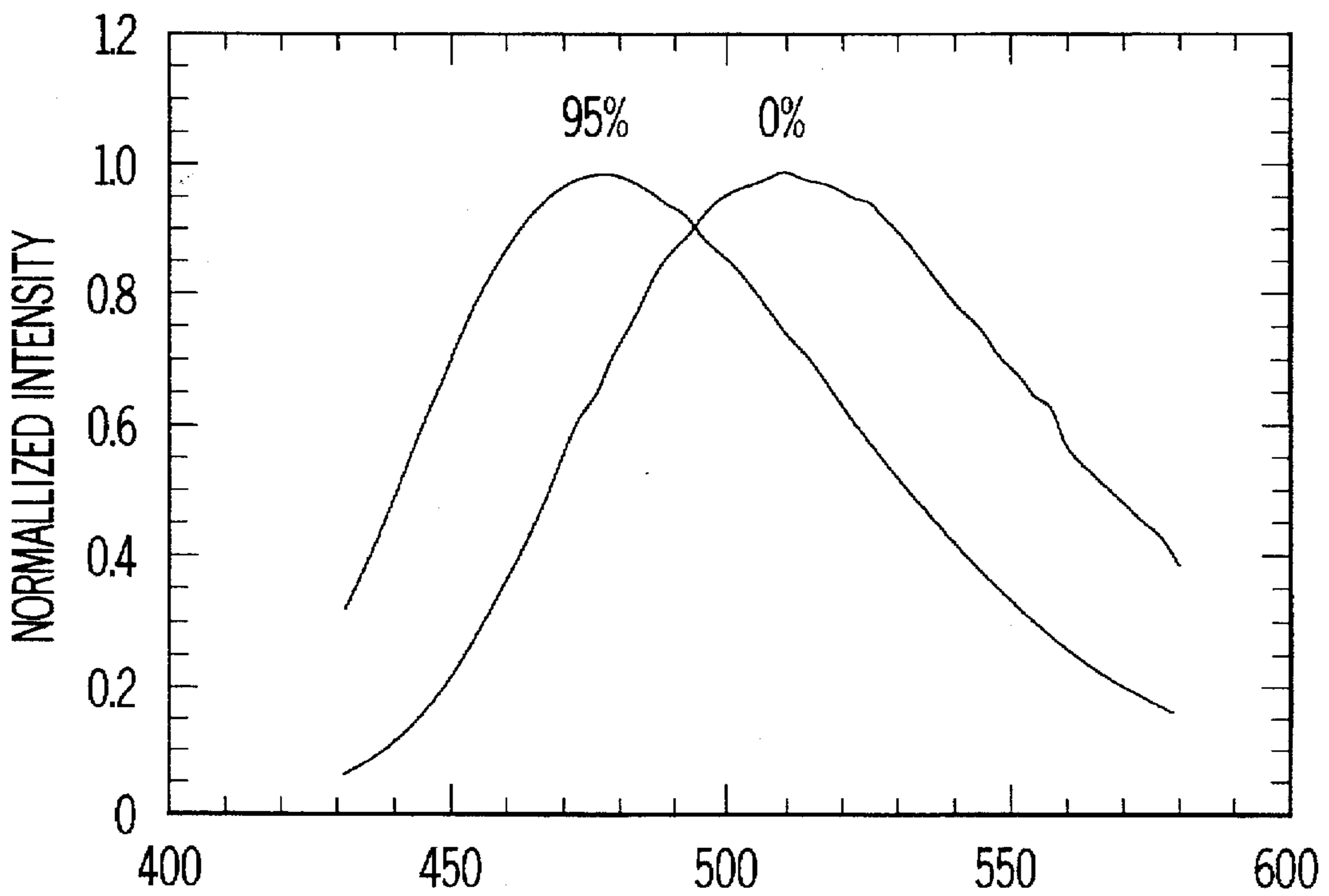
FIG. 5 WAVELENGTH (nm)
