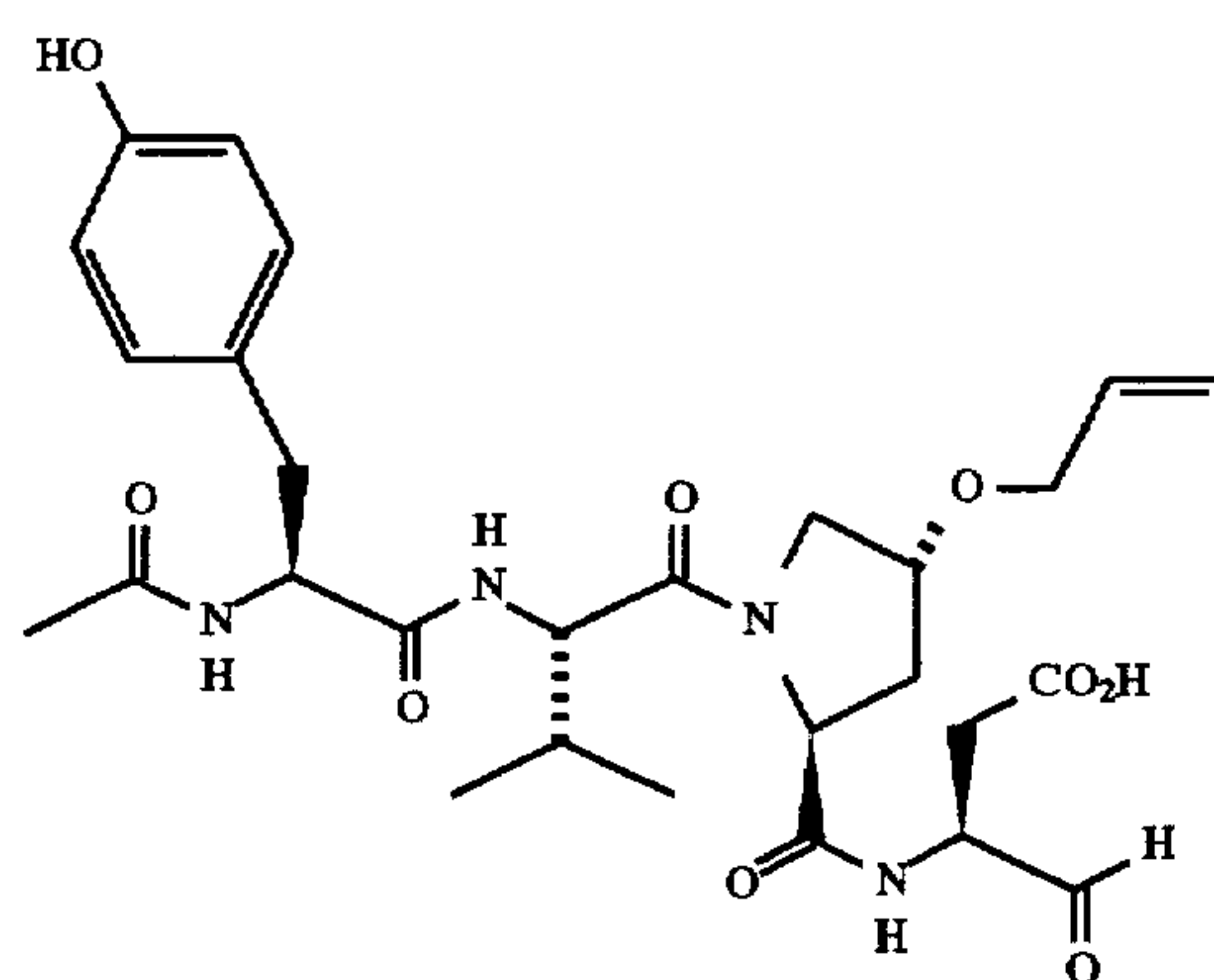
N-(N-Acetyl-tyrosinyl-valinyl-(4(R)-allyloxyprolinyl))-3(S)-amino-4-oxobutanoic acid (85)
