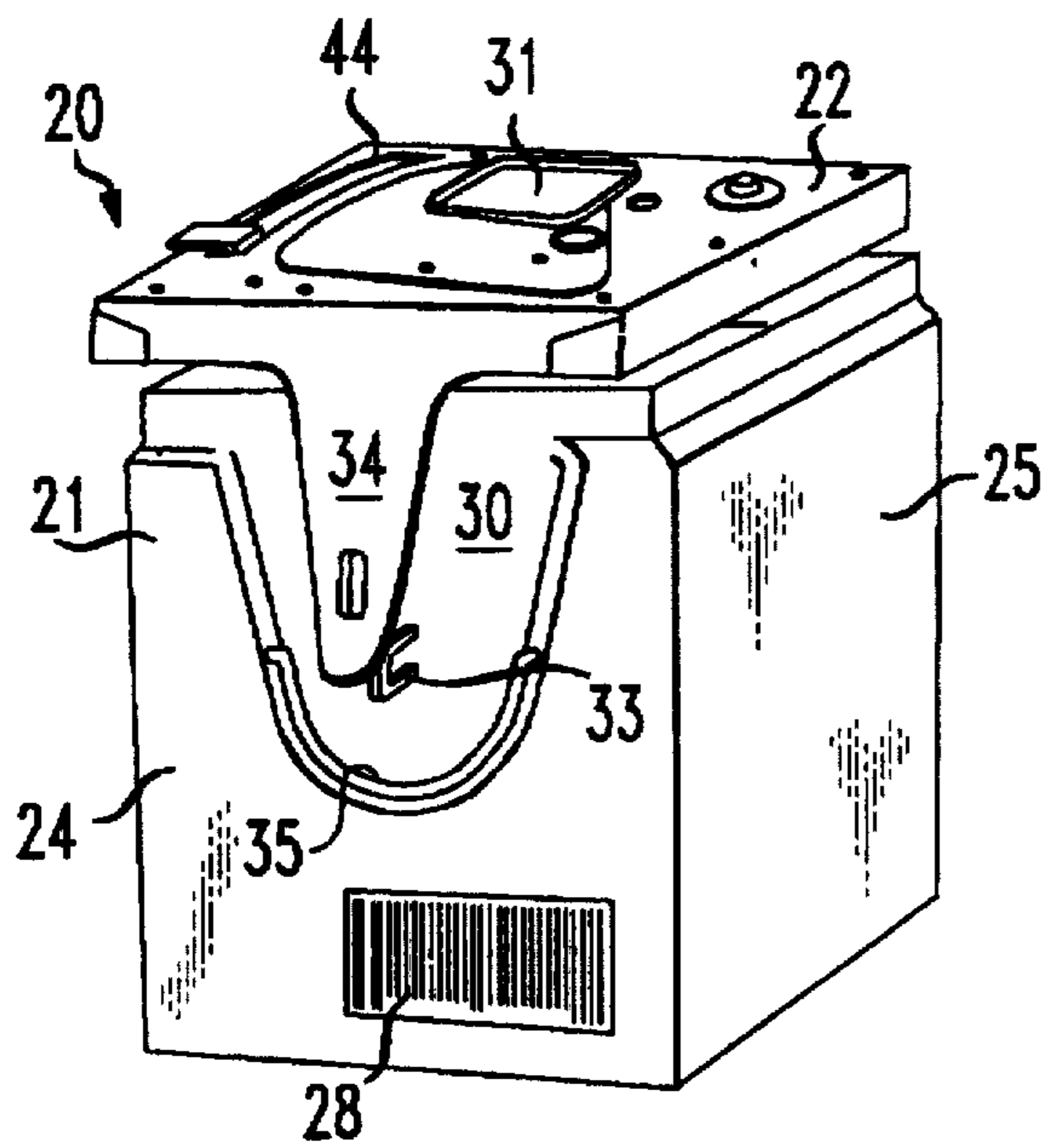
FIG. 3 (PRIOR ART)
