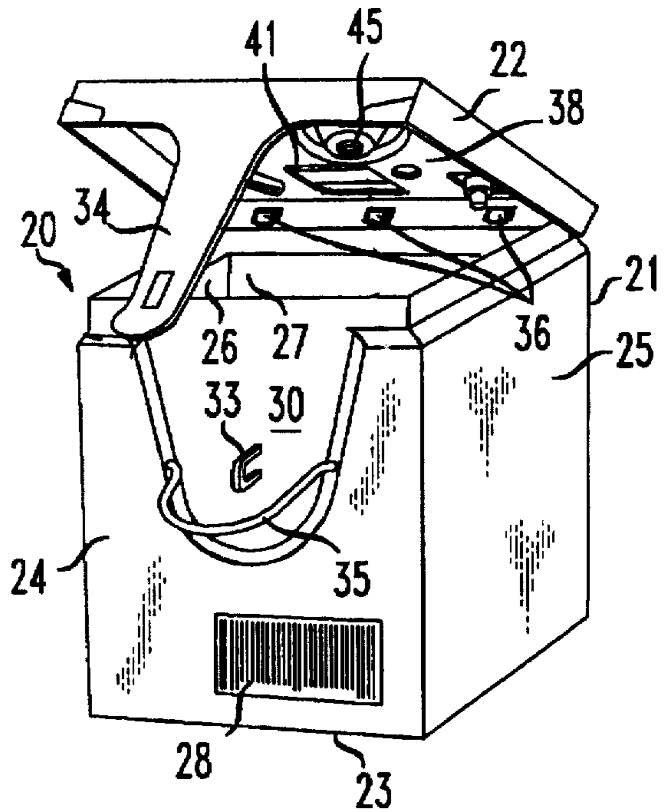
FIG. 2 (PRIOR ART)
