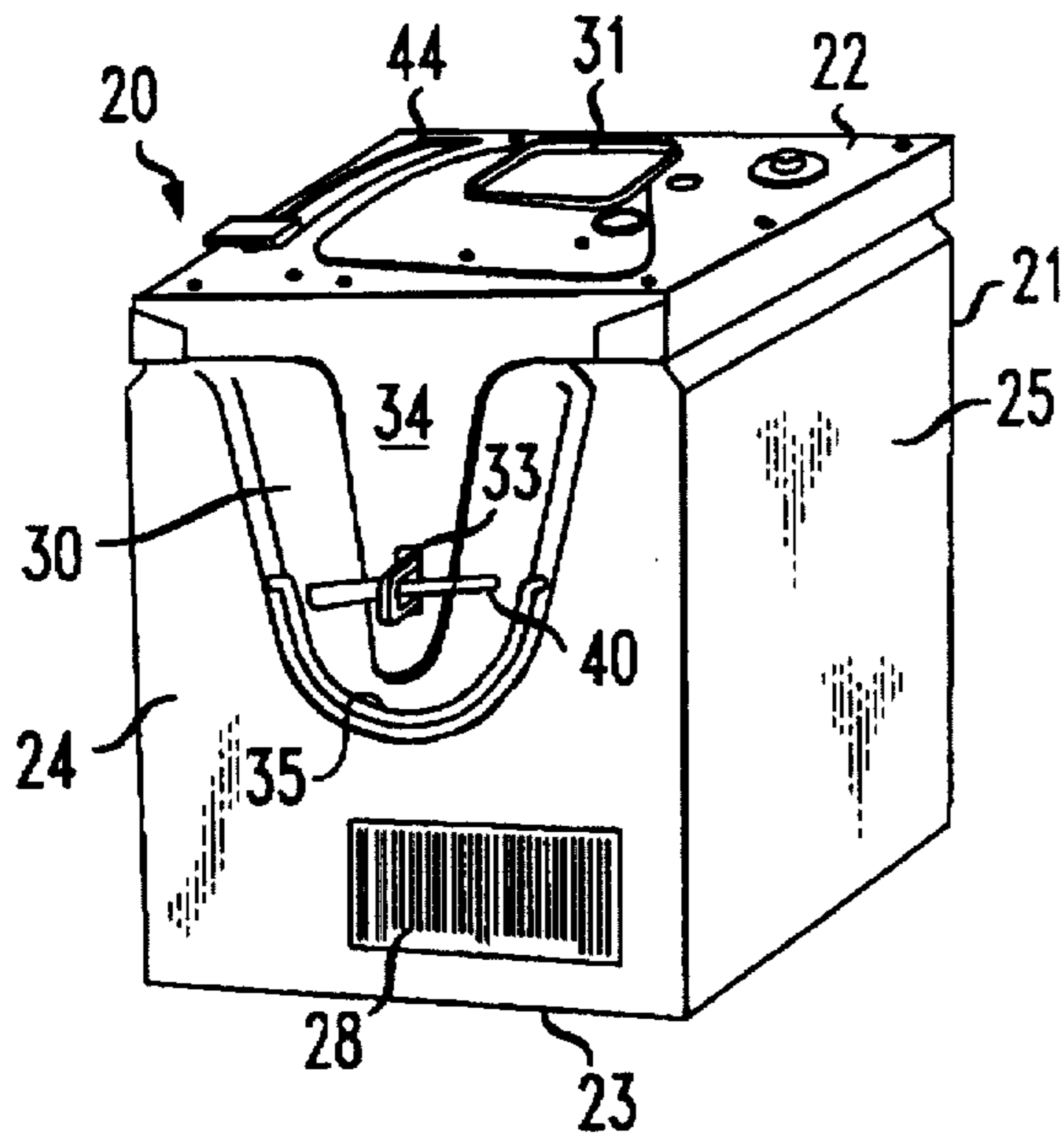
FIG. 1 (PRIOR ART)
