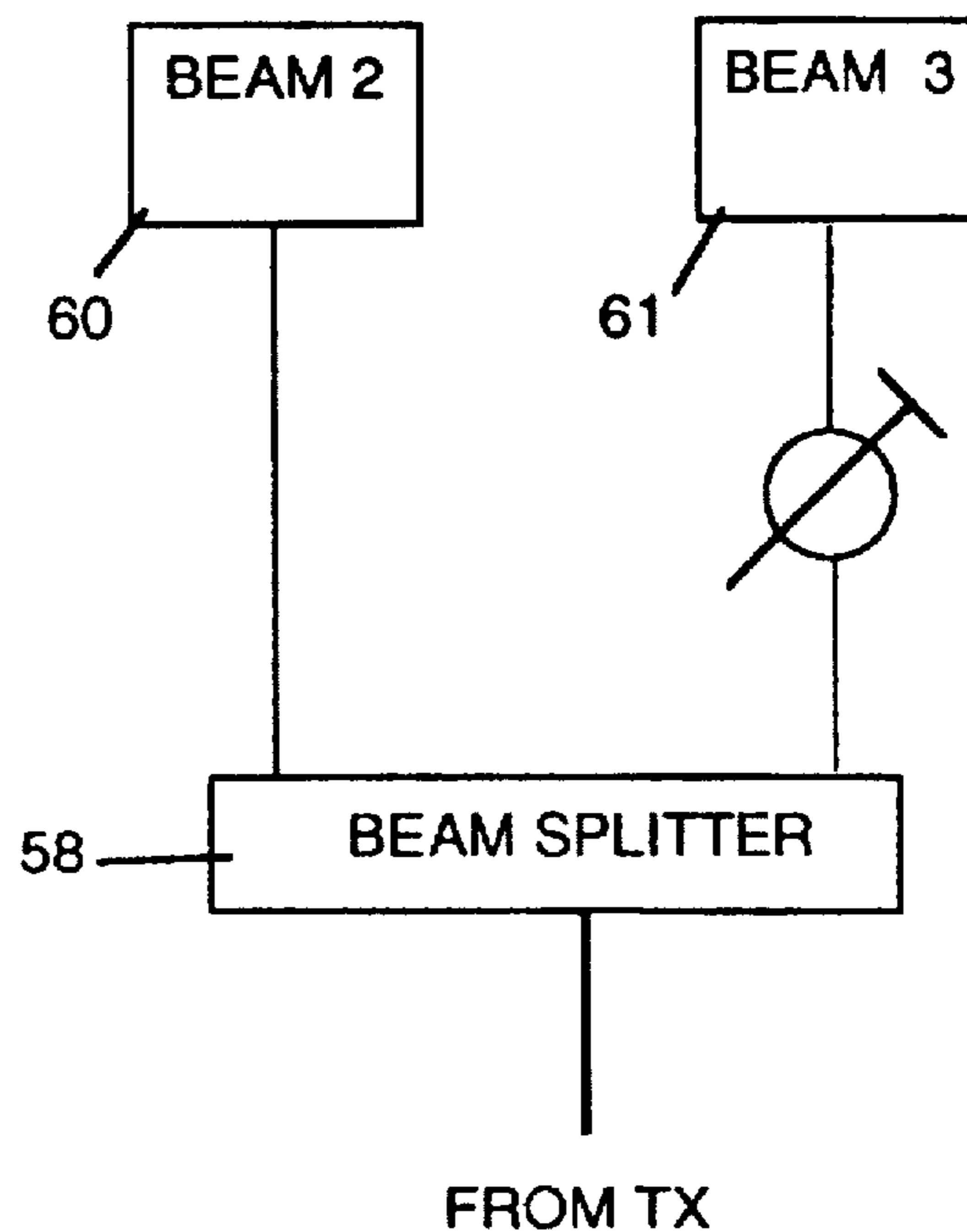
Fig. 14 (b) QUADRATURE
