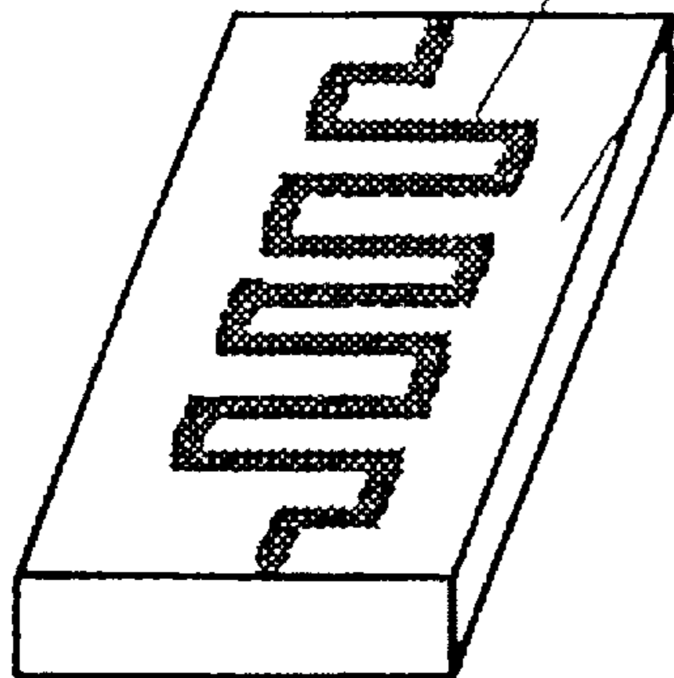
FIG. 11 COUPLING ADJUSTING LINE PATTERN SUBSTRATE
