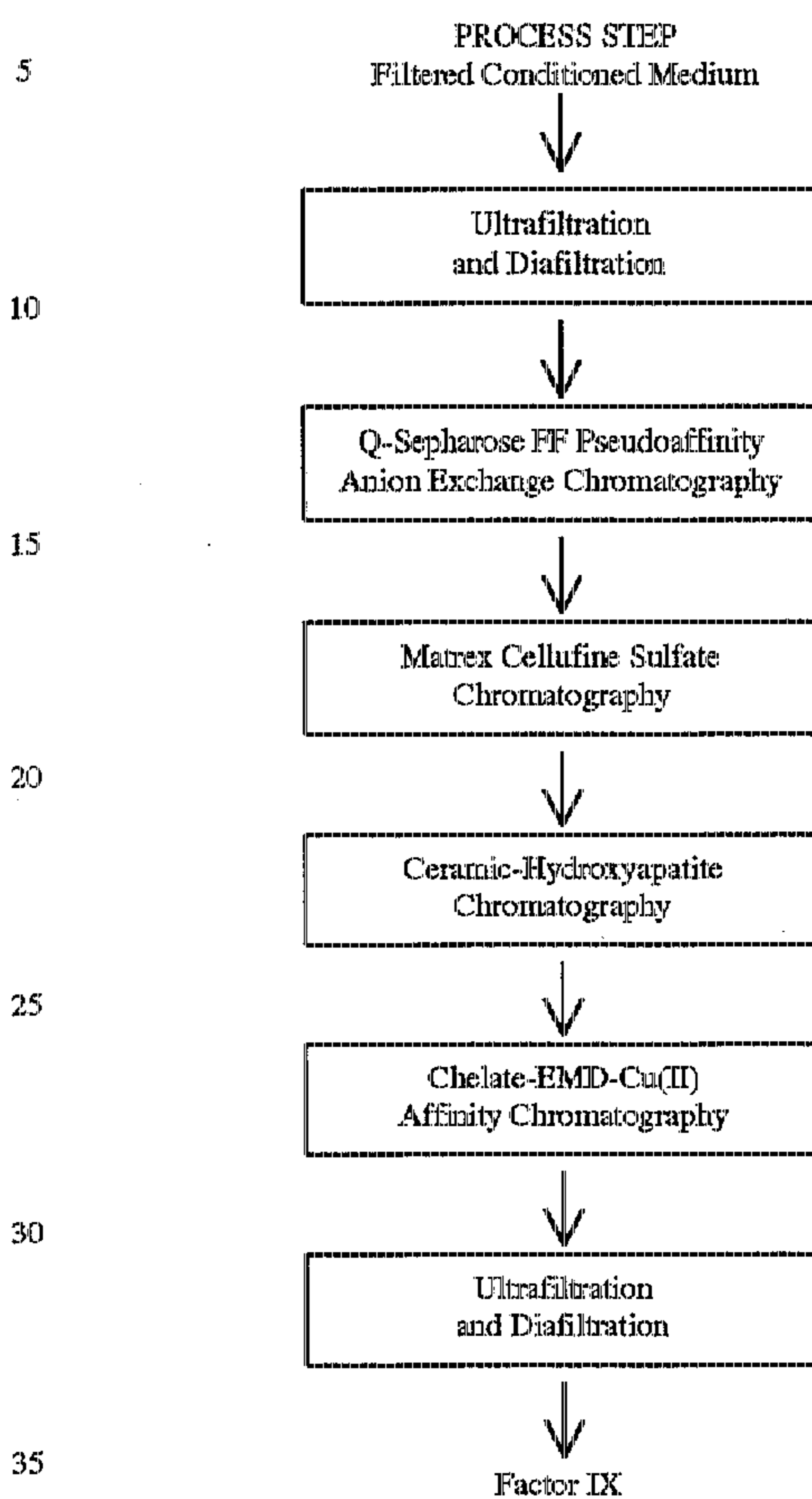
FIG. 1 Overview of factor IX Purification Process
