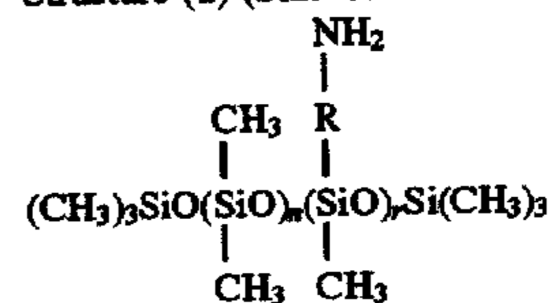
Structure (2) (Side-Chain amino silicone)
