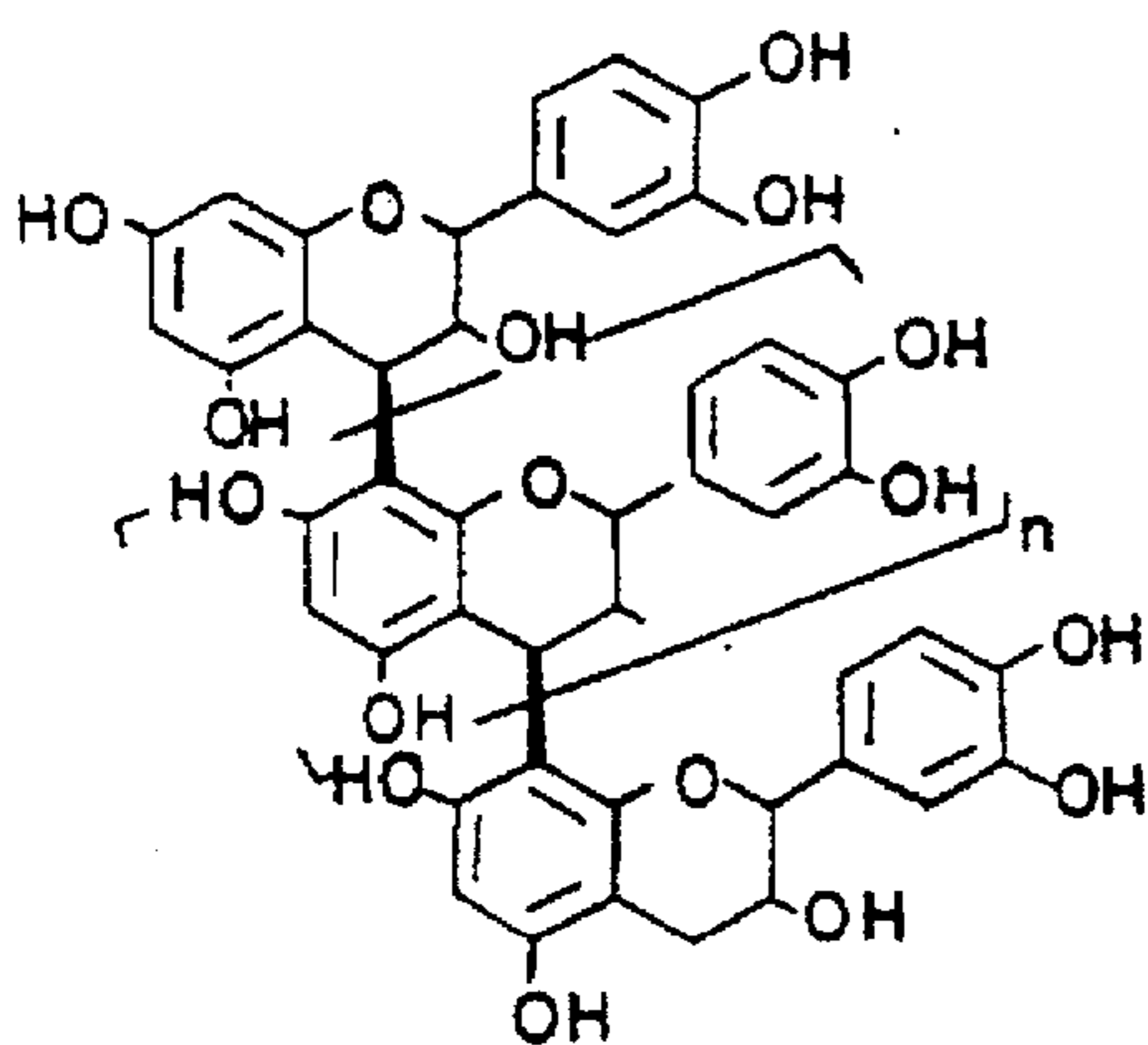
PROCYANIDIN OLIGOMERS n=2 THROUGH 5
