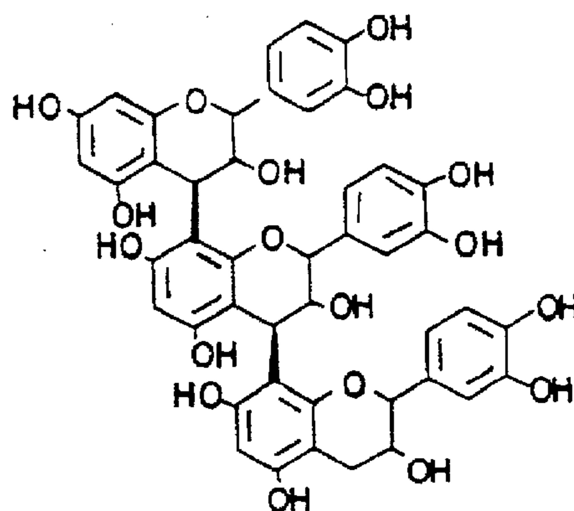
PROCYANIDIN C-1
