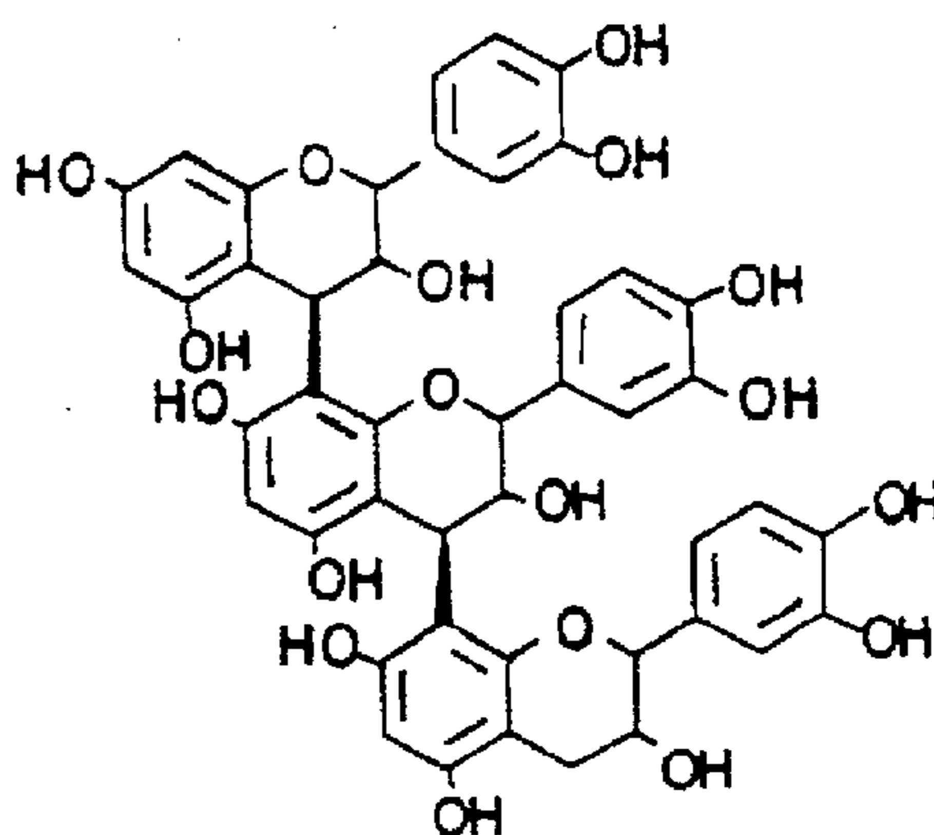
PROCYANIDIN C-1
