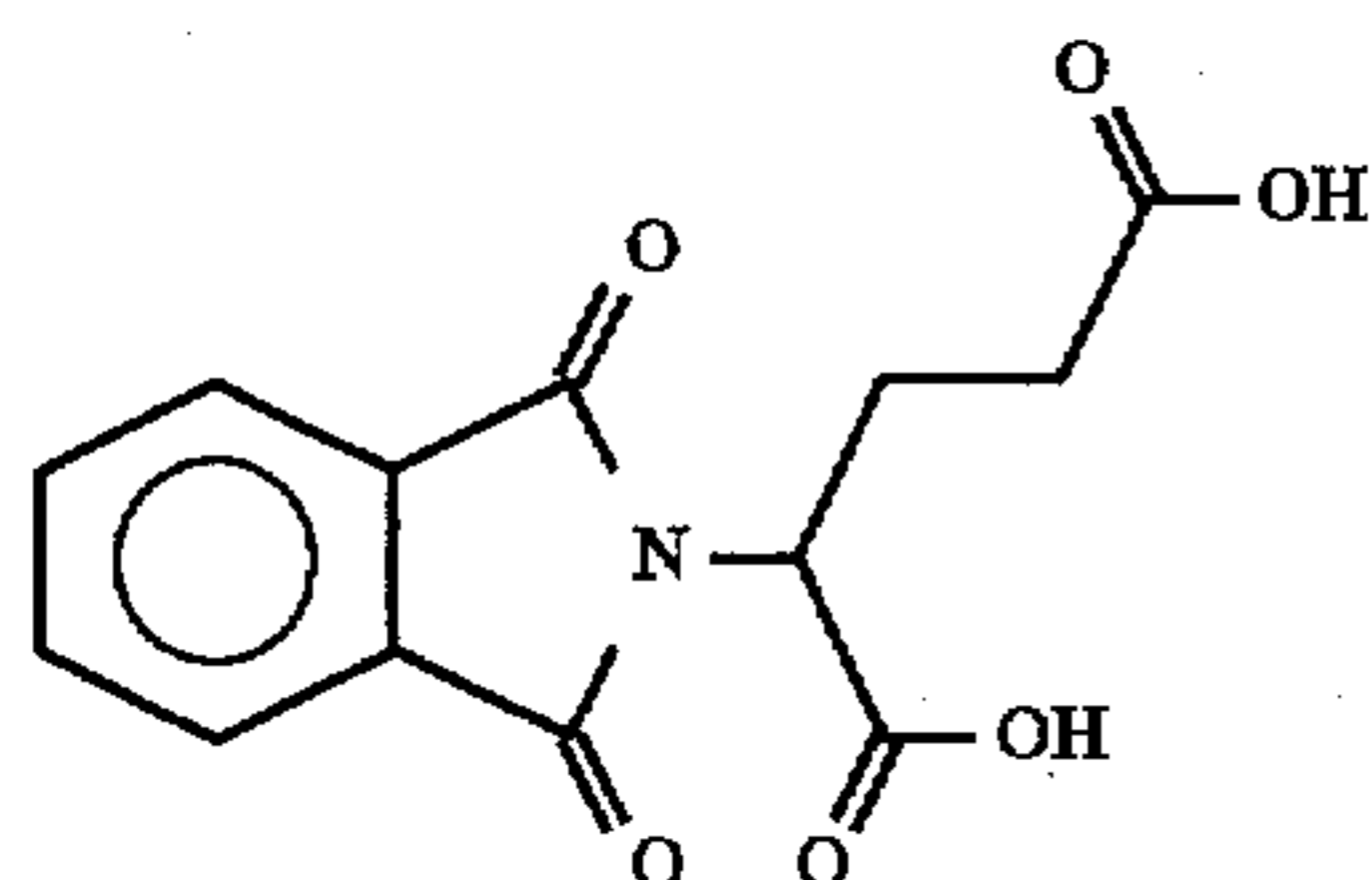
phthaloyl glutamic acid (PG Acid)
