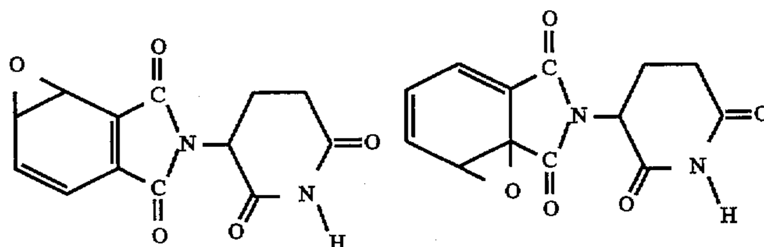
Epoxides of thalidomide
