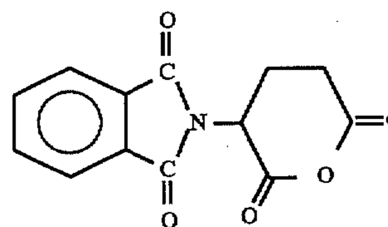
phthaloyl glutamic anhydride (PGA)
