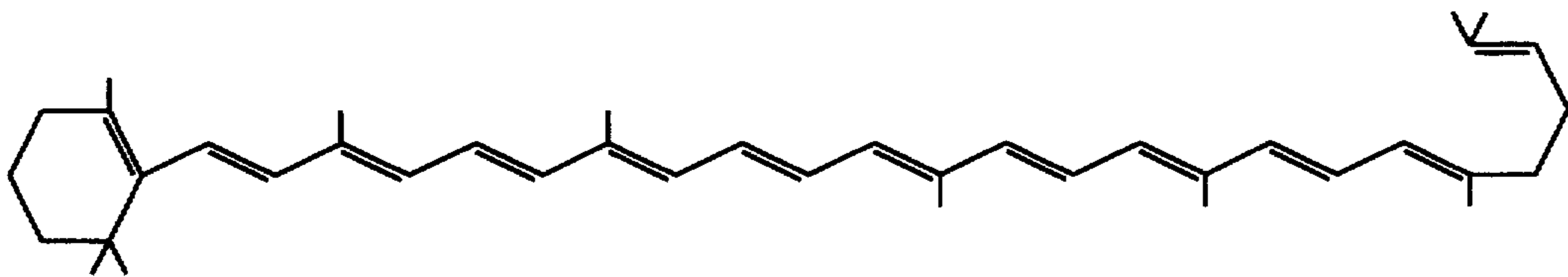
\gamma -CAROTENE
