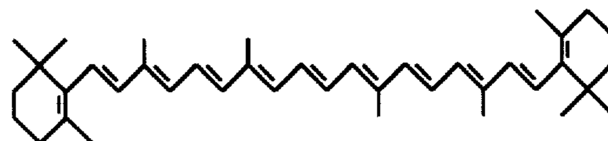
β-CAROTENE
