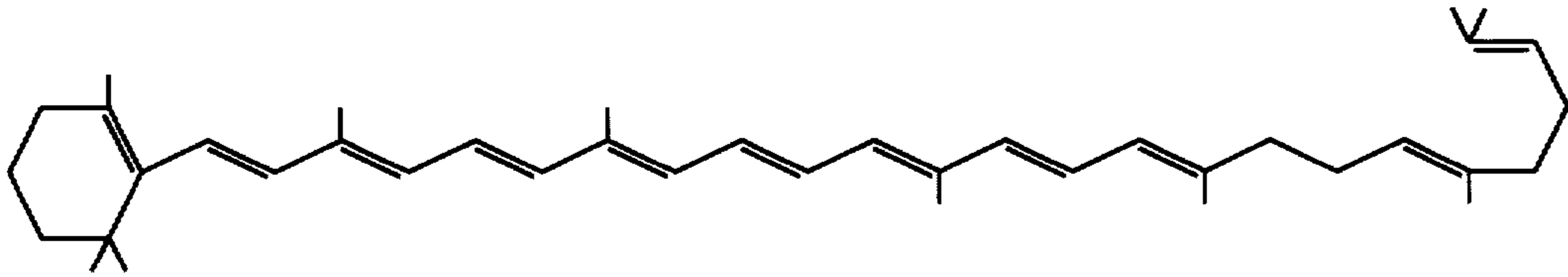
\beta -ZEACAROTENE
