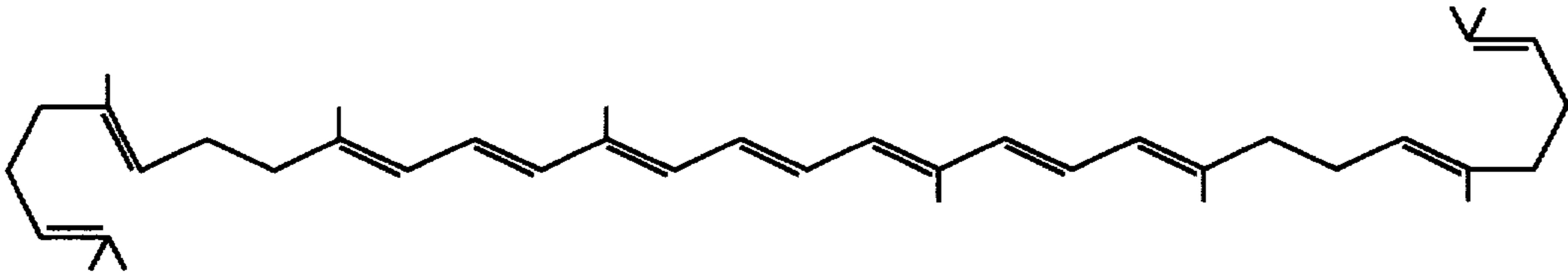
\beta -CAROTENE
