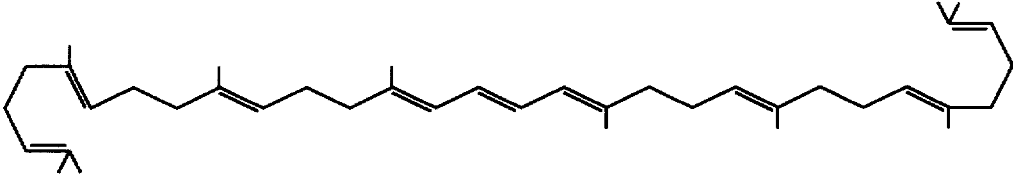
PHYTOENE
