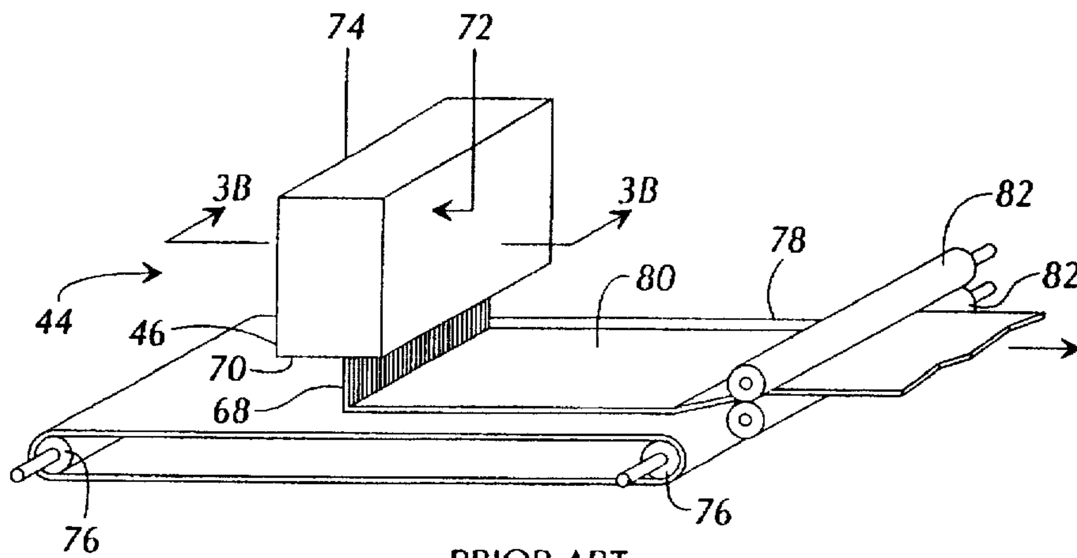
PRIOR ART FIG. 3A
