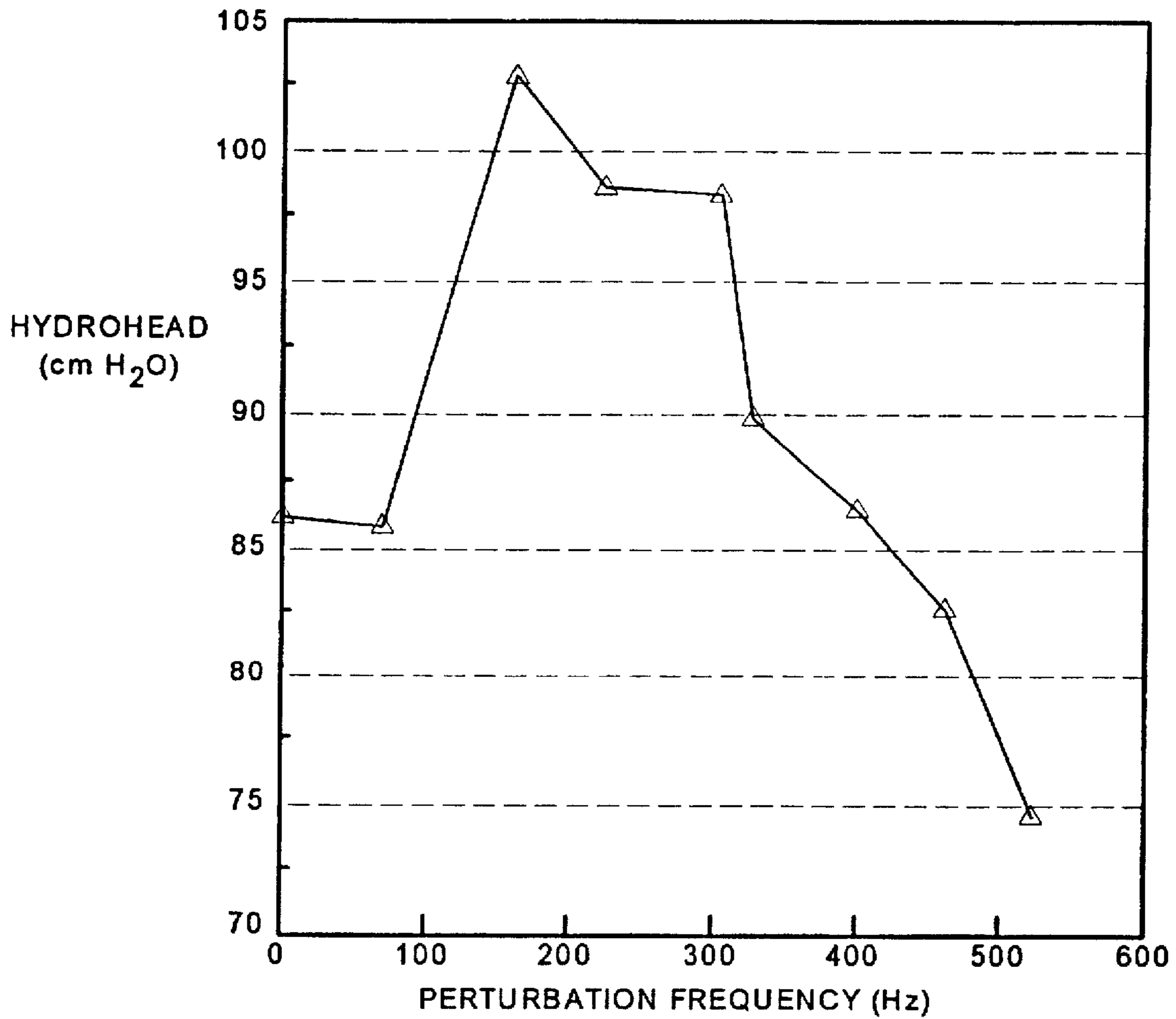
EFFECT OF PERTURBATION FREQUENCY ON HYDROHEAD.
