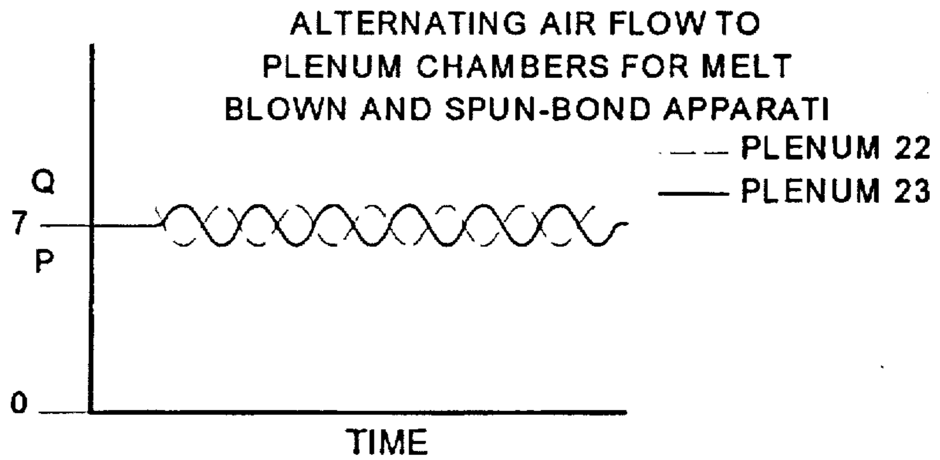
PRIOR ART FIG. 8B
