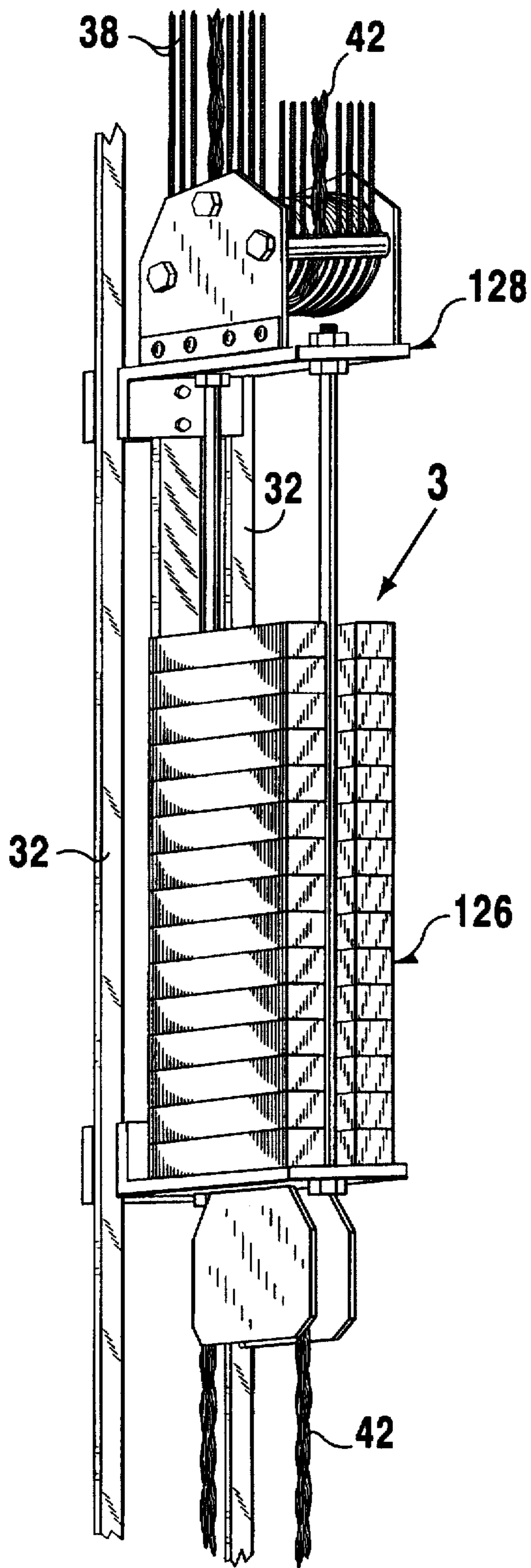
FIG 2 (PRIOR ART)
