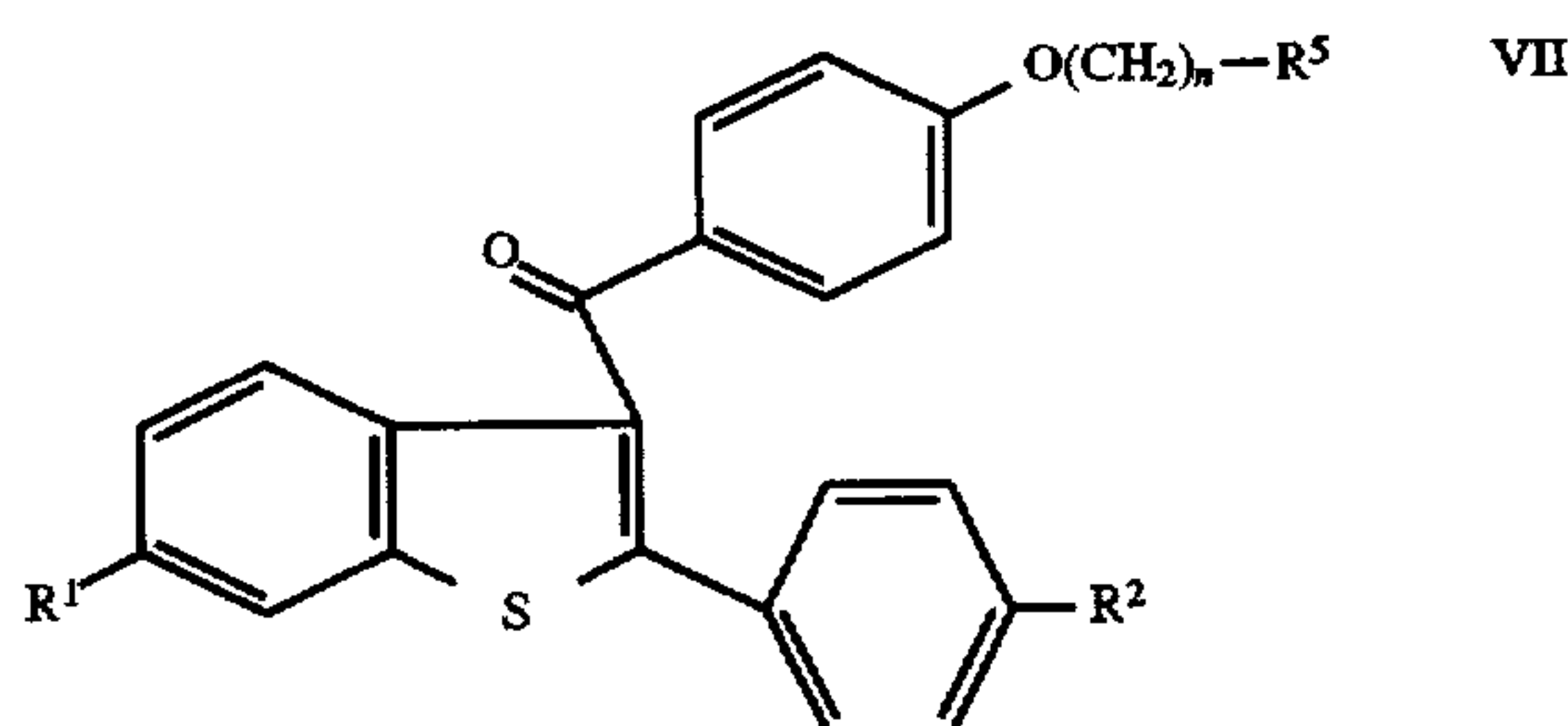
Compounds of Formula VII
