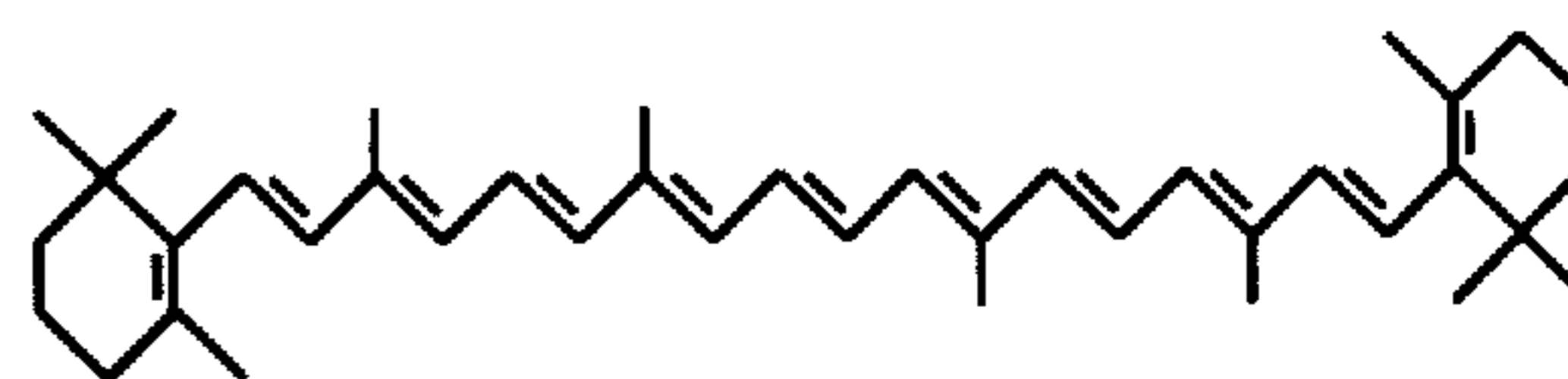
β-CAROTENE
