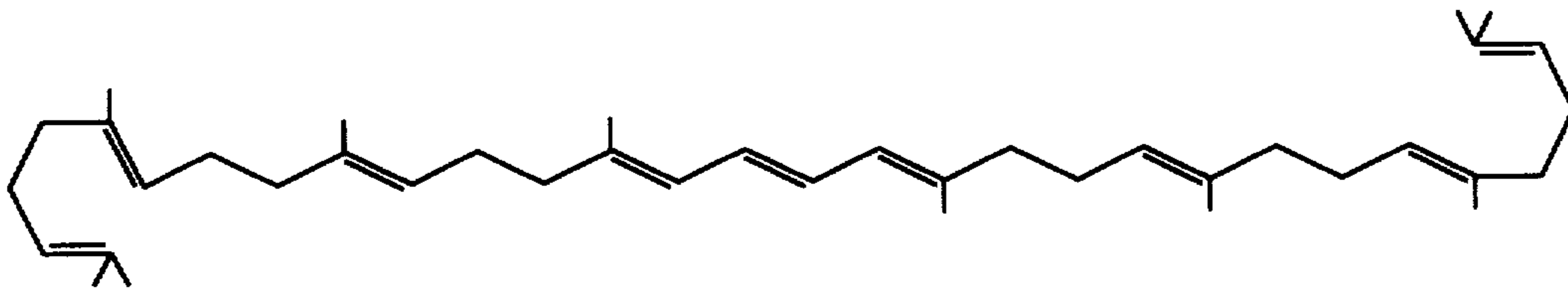
PHYTOENE
