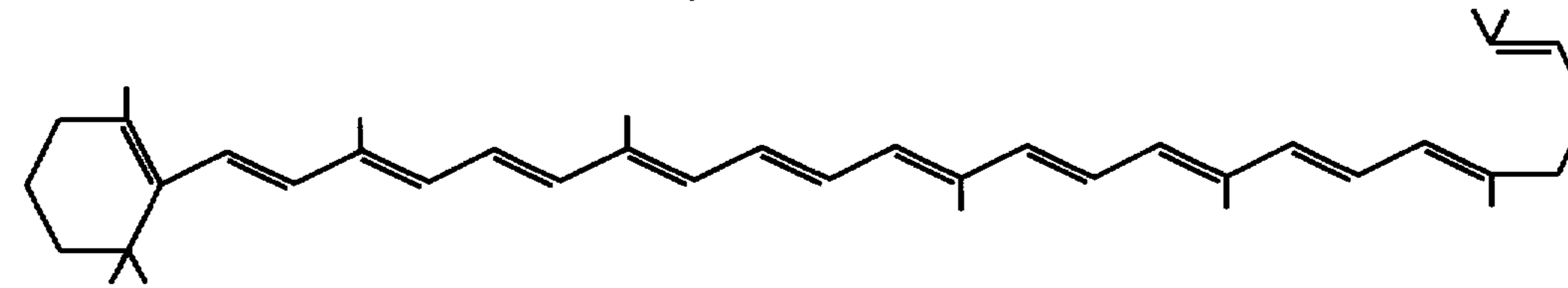
\gamma -CAROTENE
