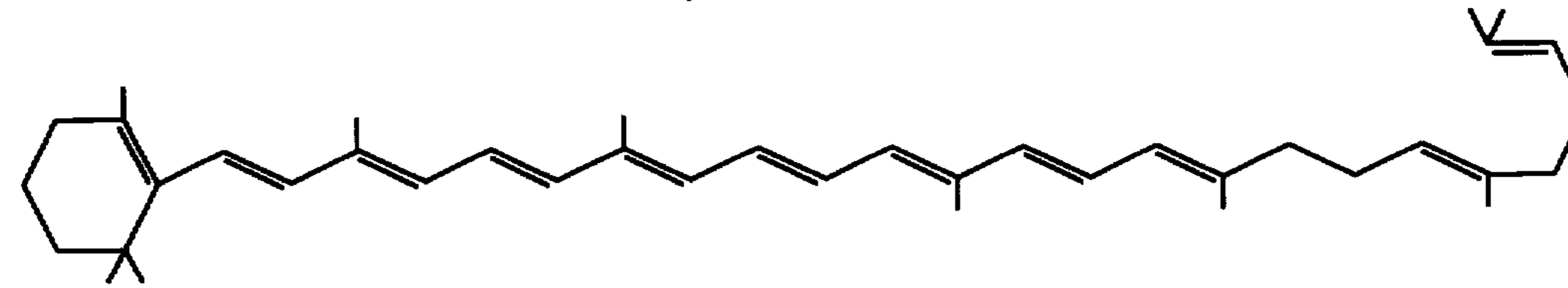
\beta -ZEACAROTENE
