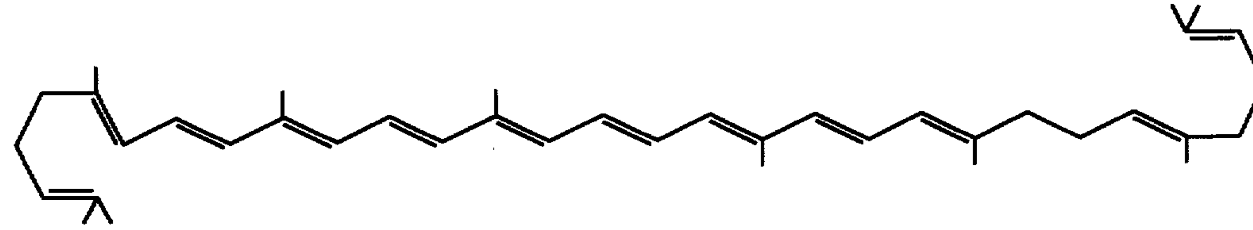
NEUROSPORENE
