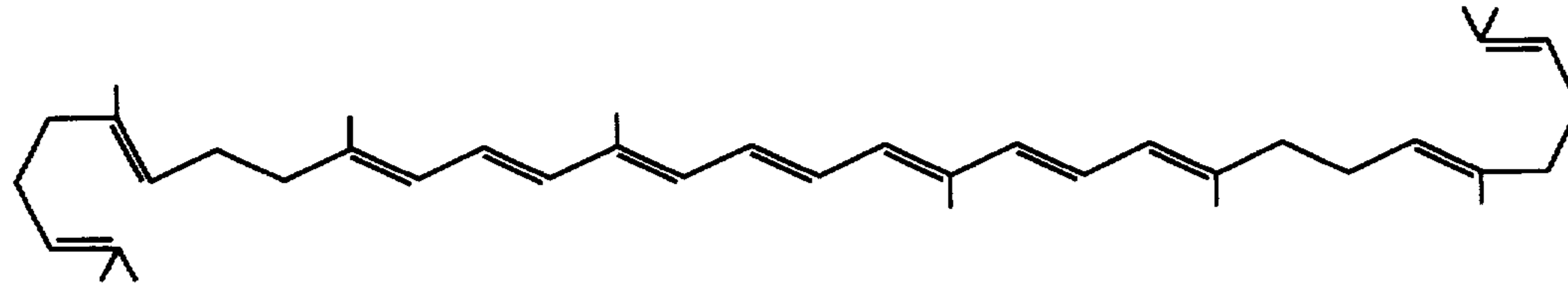
\beta -CAROTENE
