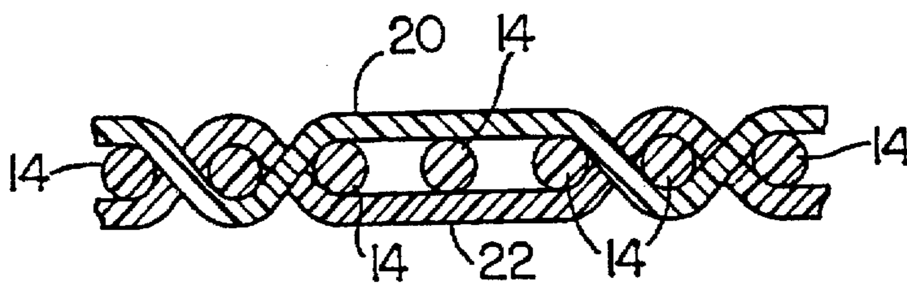
FIG. 3 PRIOR ART
