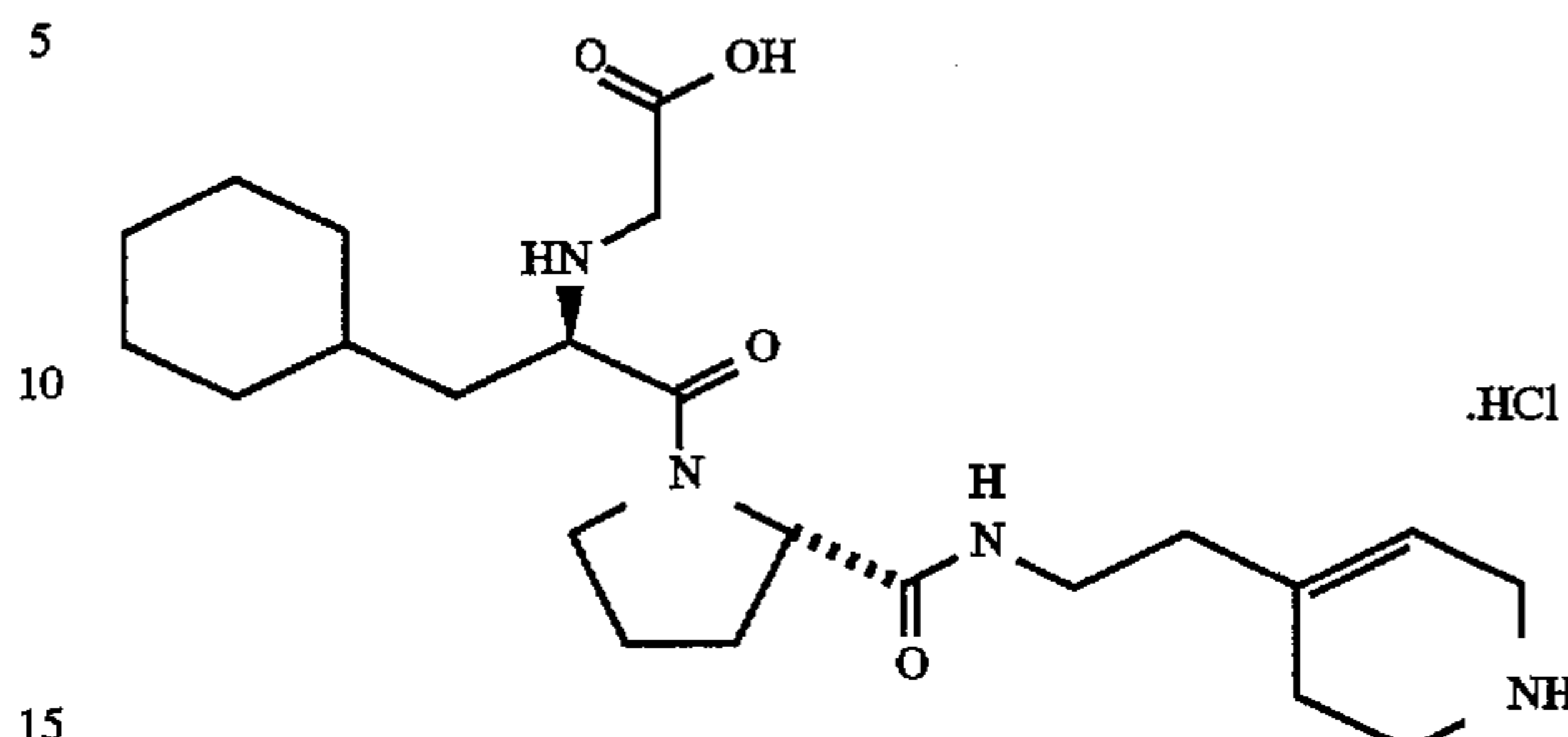
HO 2 CCH 2 -D-Cha-Pro-4-NHCH 2 CH 2 -3,4-dehydro-piperidine.HCl
