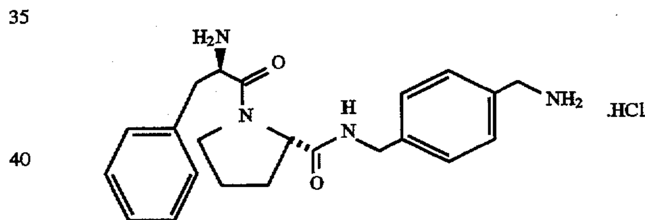
D-Phe-Pro-p-NHCH 2 C 6 H 4 CH 2 NH 2 ·HCl
