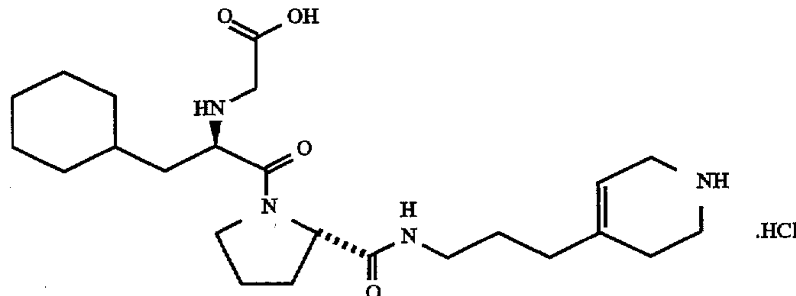
HO 2 CCH 2 -D-Cha-Pro-4-NHCH 2 CH 2 CH 2 -3,4-dehydro-piperidine.HCl
