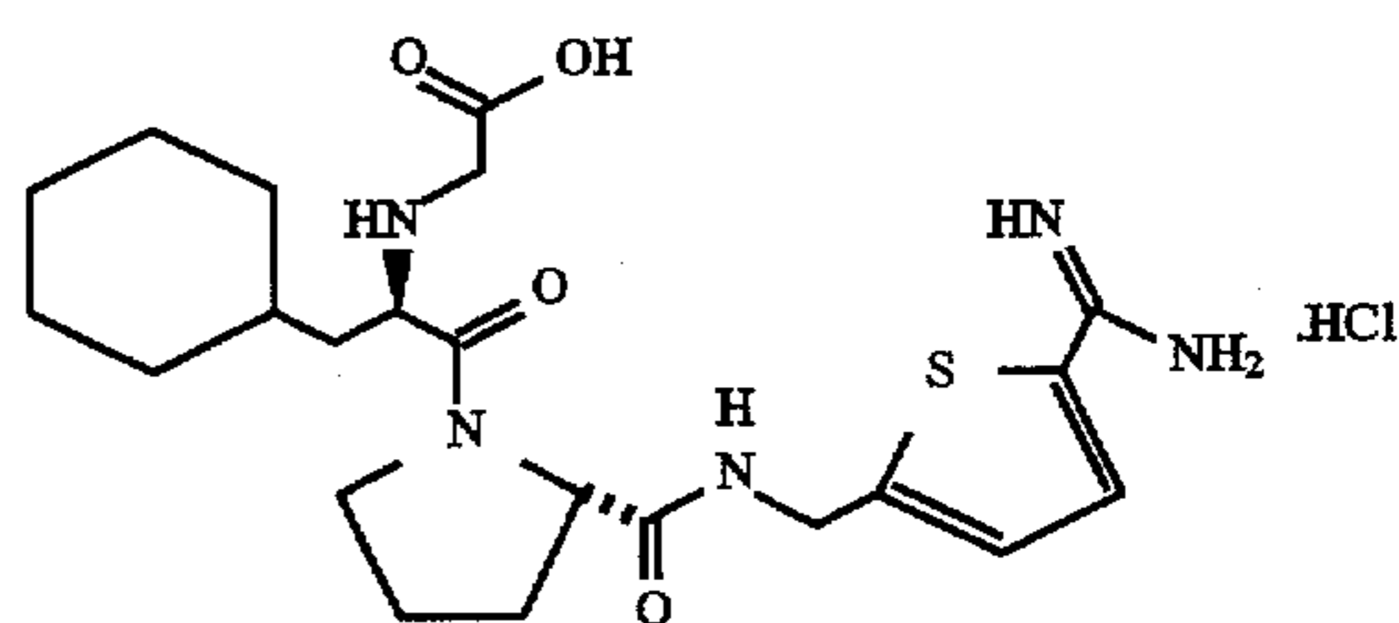
HO 2 CCH 2 -D-Cha-Pro-4-NHCH 2 -2-amidinothiophene·HCl (N-(carboxymethyl)-D-cyclohexylalanyl-N-[[5-(aminoiminomethyl)thiophen-2-yl]methyl]-L-prolinamide hydrochloride)
