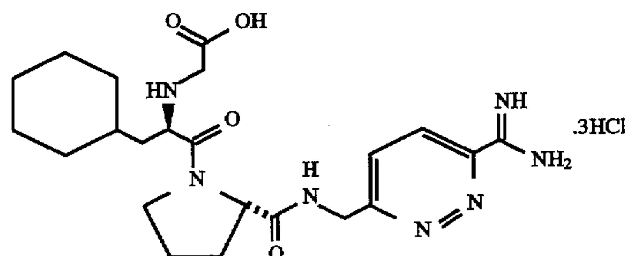
\text{HO}_2\text{CCH}_2\text{-D-Cha-Pro-3-NHCH}_2\text{-6-amidino-pyridazine.3HCl} ( \text{N-(carboxymethyl)-D-cyclohexylalanyl-N-[6-(aminoimino-methyl)pyridazin-3-yl]methyl-L-prolinamide trihydrochloride} )
