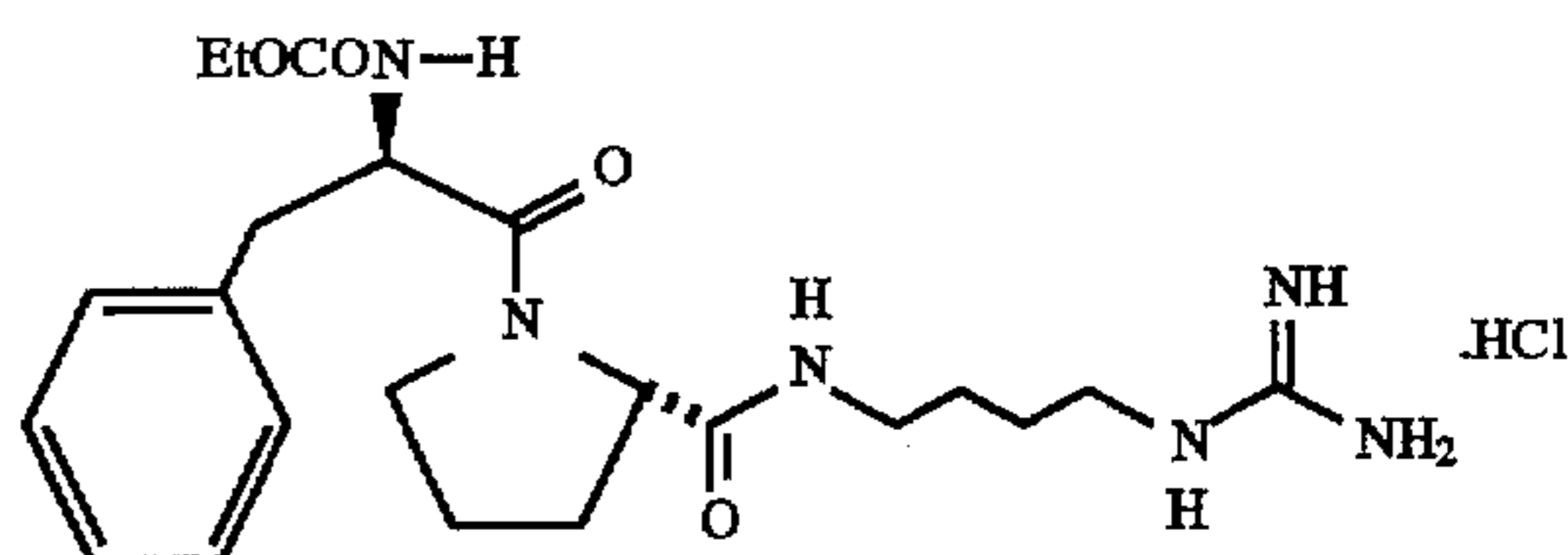
EtOCO-D-Phe-Pro-Agm.HCl
