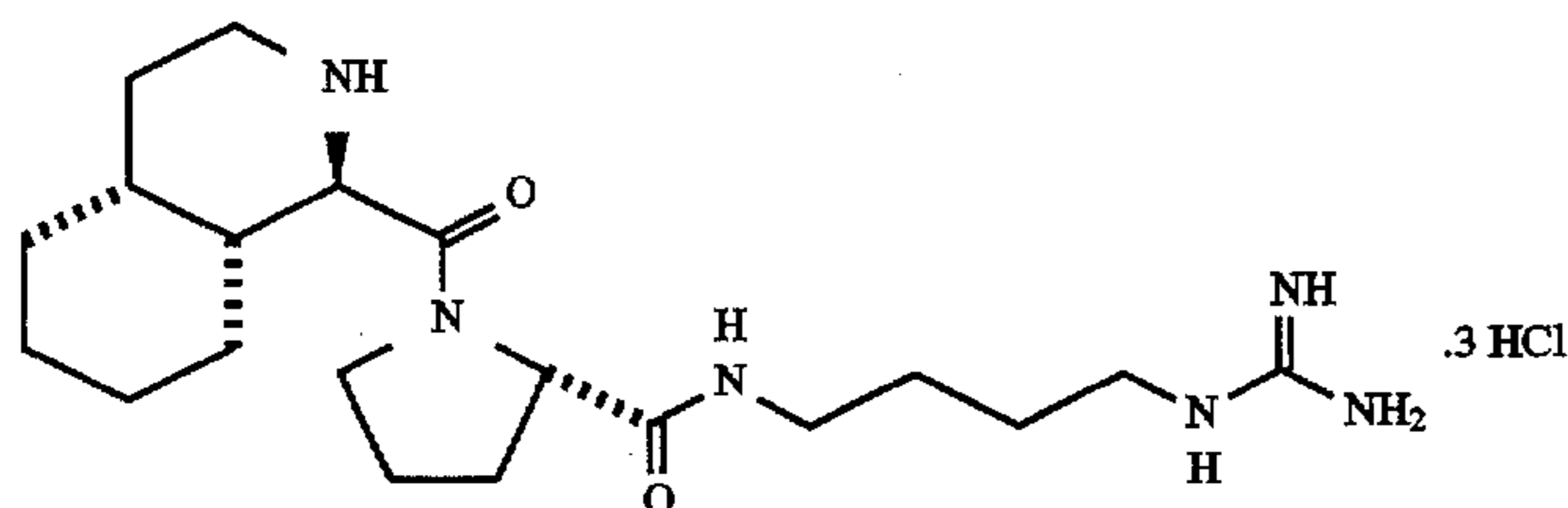
(1R, 4aR, 8aR)-1-Piq-Pro-Agm.3HCl (N-[4-[(aminoiminomethyl)amino]butyl]-1-[[4aR,8aR]-decahydro-1(R)-isoquinolinyl]carbonyl]-1-prolinamide trihydrochloride)
