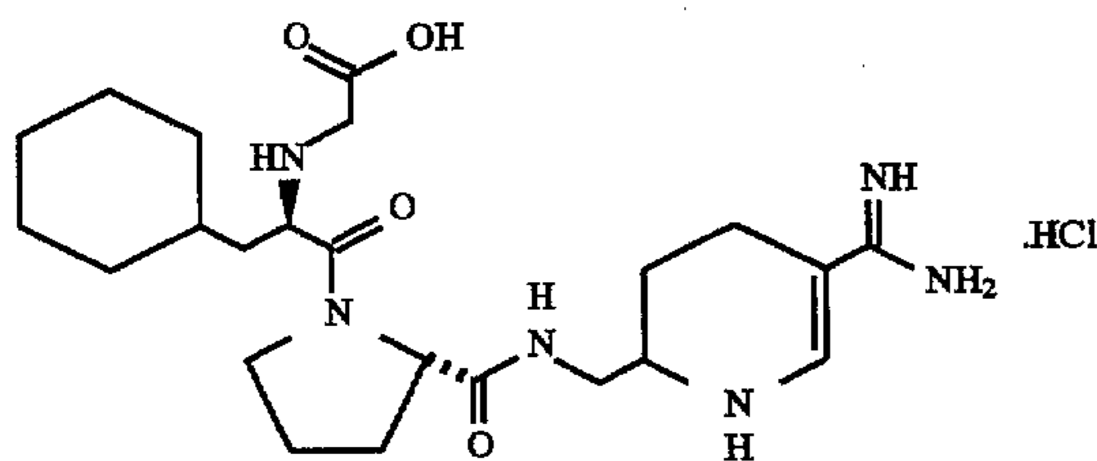
\text{HO}_2\text{CCH}_2\text{-D-Cha-Pro-2-NHCH}_2\text{-5-amidino-5,6-dehydropiperidine.HCl} ( \text{N-(carboxymethyl)-D-cyclohexylalanyl-N-[5-(aminoimino-methyl)-1,2,3,4-tetrahydropyridin-2-yl]methyl-L-prolinamide hydrochloride} )
