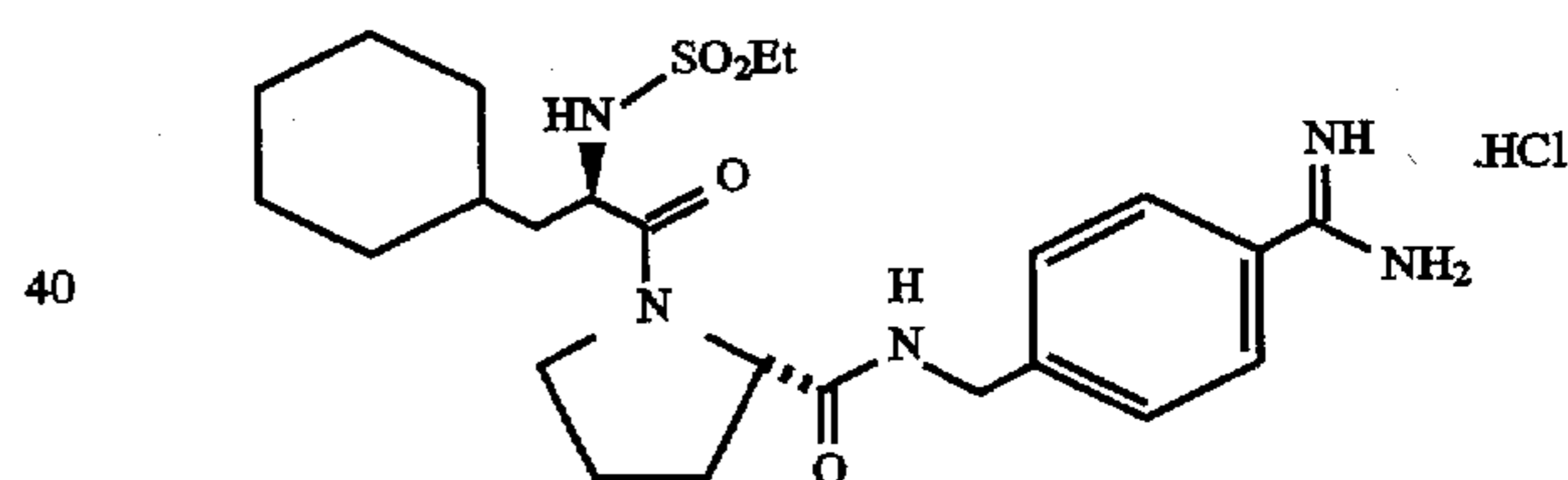
EtSO 2 -D-Cha-Pro-4-NHCH 2 -C 6 H 4 C(NH)NH 2 .HCl (N-(ethylsulfonyl)-D-cyclohexylalanyl-N-[[4-(aminoiminomethyl)phenyl]methyl]-L-prolinamide hydrochloride)
