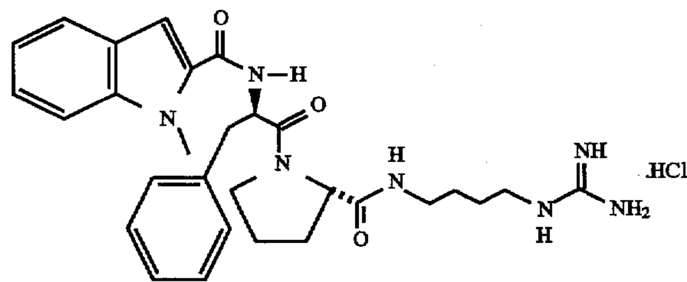
NMI-D-Phe-Pro-Agm.HCl (N-[(1-methyl-1H-indol-2-yl)carbonyl]-D-phenylalanyl-N-[4-[(aminoiminomethyl)amino]butyl]-L-prolinamide monohydrochloride)
