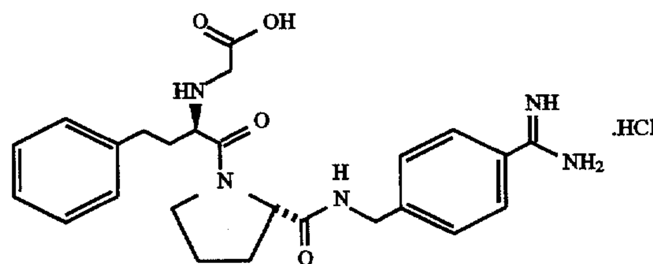
\text{HOOCCH}_2\text{-D-hPhe-Pro-p-NHCH}_2\text{C}_6\text{H}_4\text{C(NH)NH}_2\cdot\text{HCl} (N-(carboxymethyl)-D-homophenylalanyl-N-[[4-(aminoiminomethyl)phenyl]methyl]-L-prolinamide hydrochloride)
