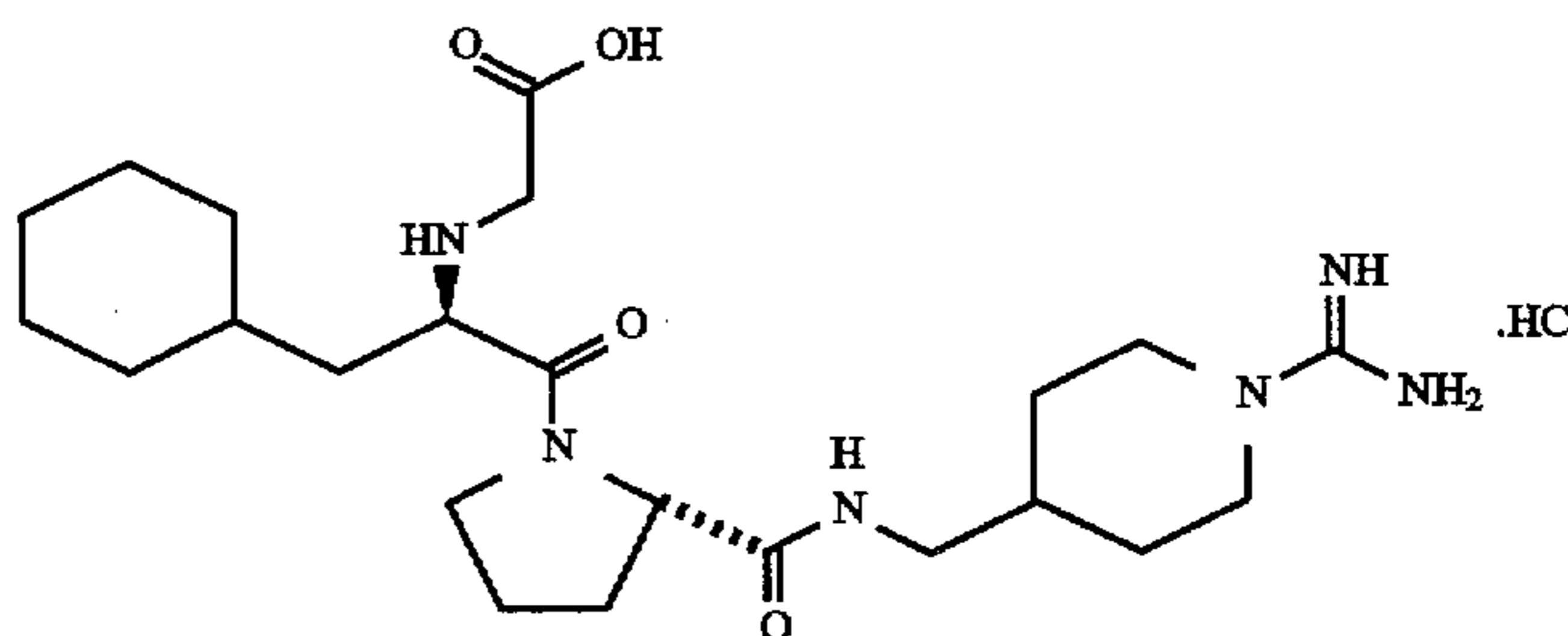
HO 2 CCH 2 -D-Cha-Pro-4-NHCH 2 -1-amidinopiperidine.HCl (N-(carboxymethyl)-d-cyclohexylalanyl-N-[[1-(aminoiminomethyl)-hexahydropyridin-4-yl]-methyl]-L-prodimamide hydrochloride)
