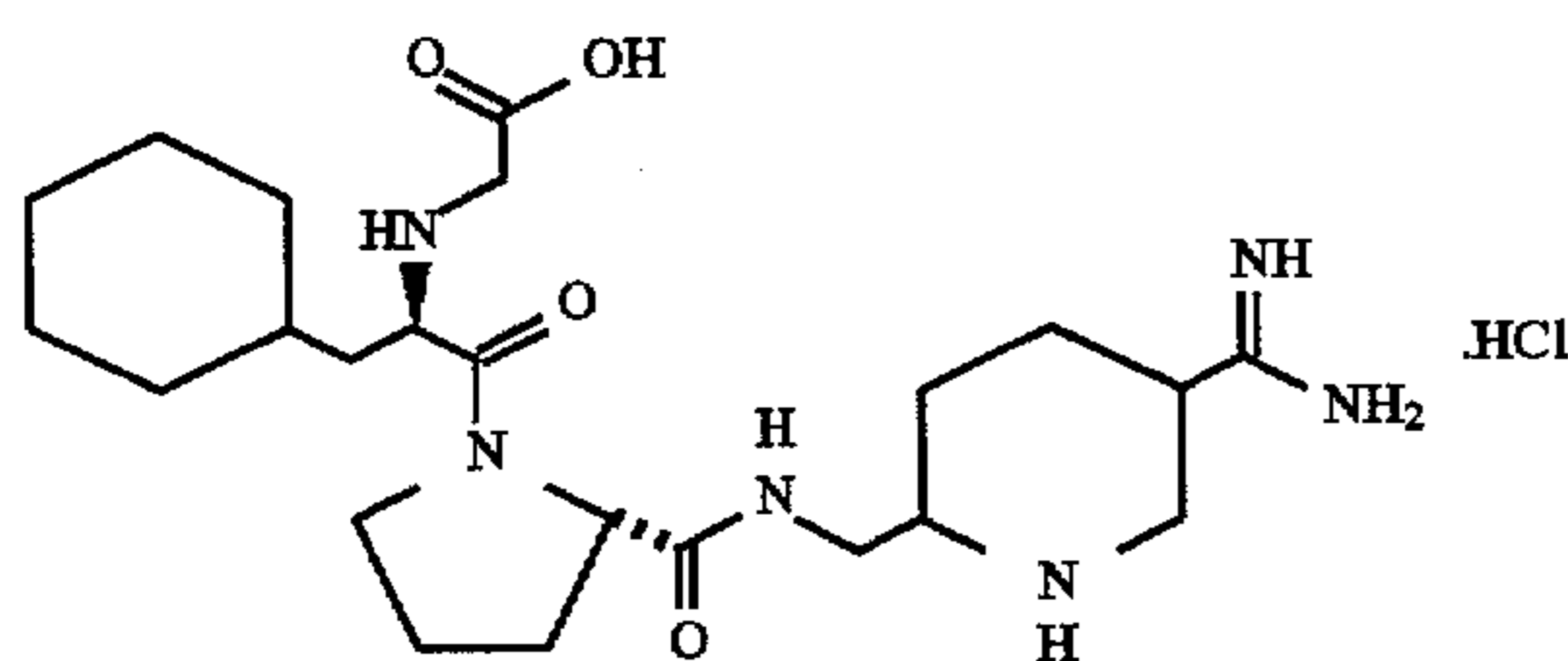
\text{HO}_2\text{CCH}_2\text{-D-Cha-Pro-2-NHCH}_2\text{-5-amidinopiperidine.HCl}
