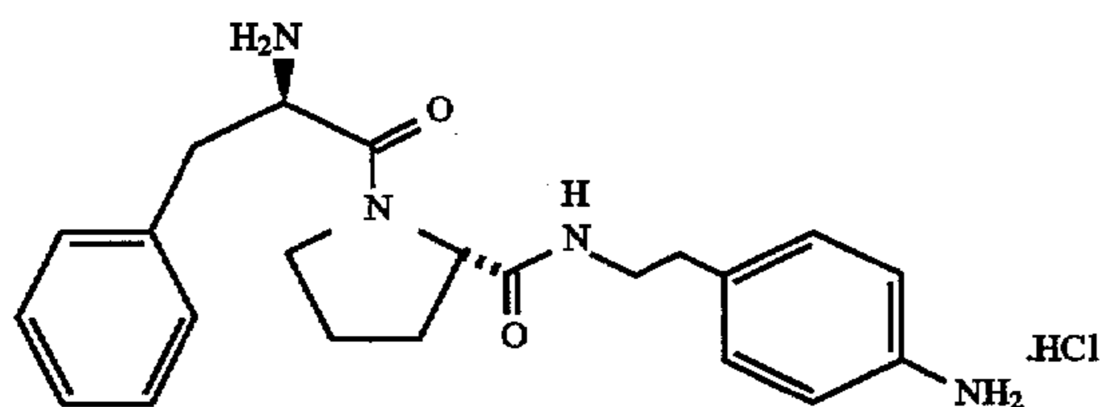
D-Phe-Pro-p-NHCH 2 CH 2 C 6 H 4 NH 2 .HCl
