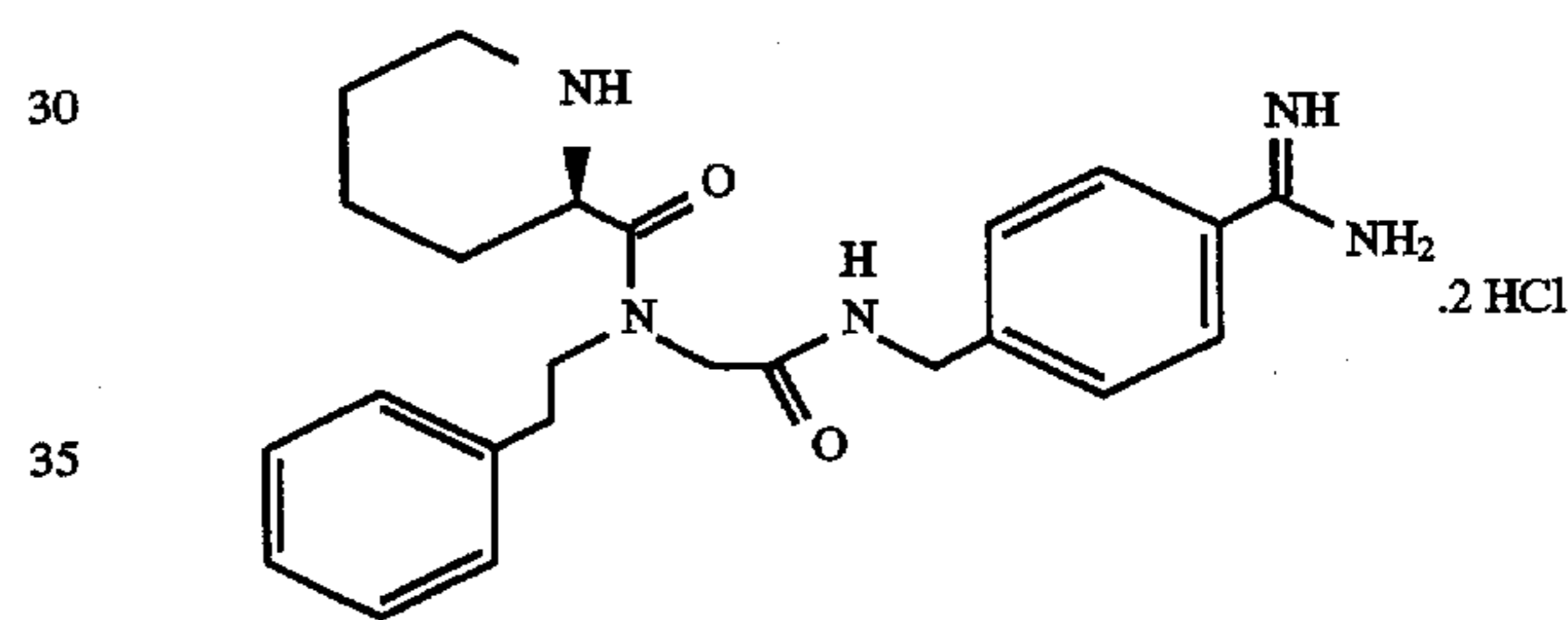
D-hPro-N(PhCH 2 CH 2 )Gly-p-NHCH 2 C 6 H 4 C(NH)NH 2 .2HCl (D-homopropyl-N(α)-(2-phenylethyl)-N-[[4-(aminoiminomethyl)phenyl]methyl]glycinamide dihydrochloride)
