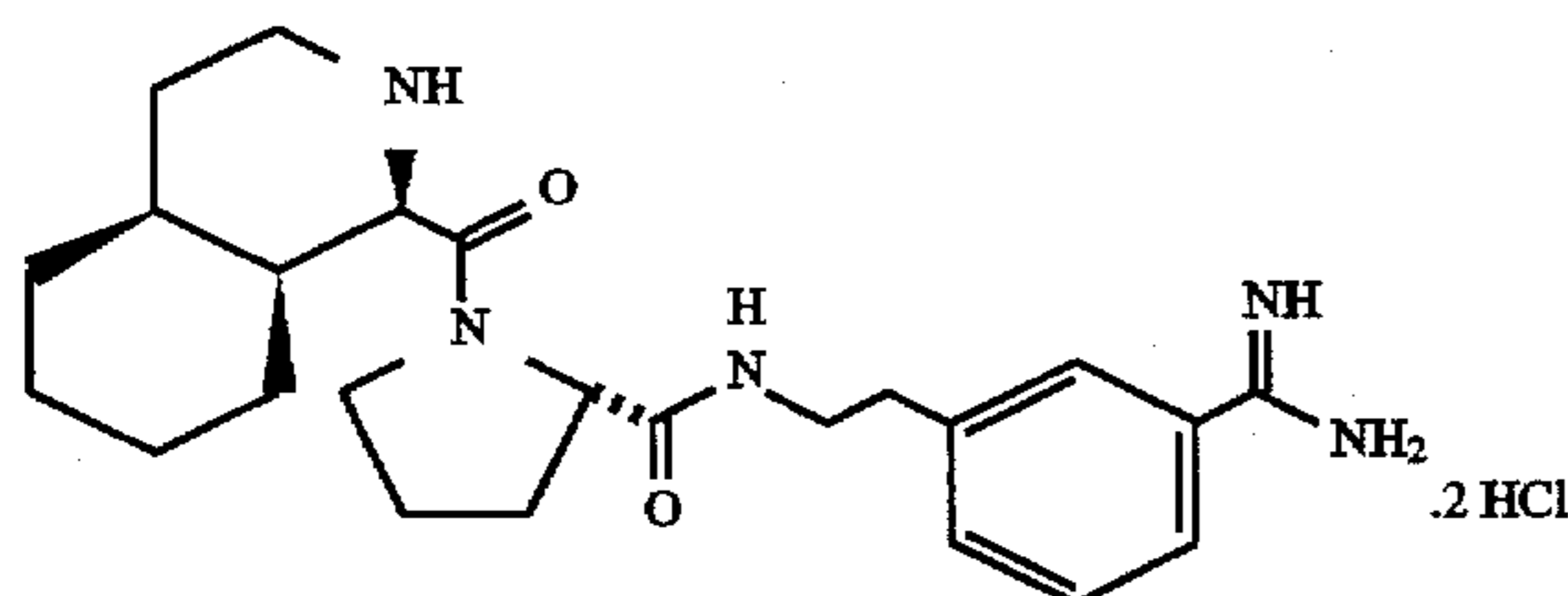
D-1-Piq-Pro-m-NHCH 2 CH 2 —C 6 H 4 C(=NH)NH 2 .2HCl
