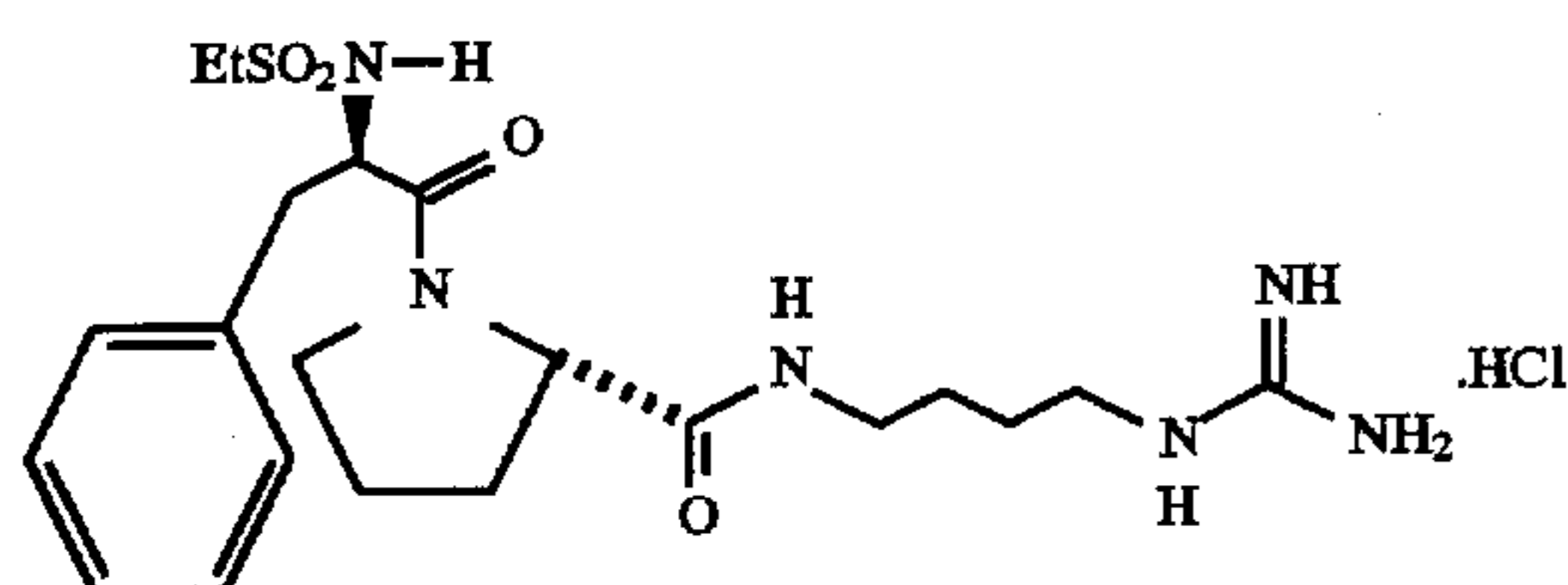
EtSO 2 -D-Phe-Pro-Agm.HCl
