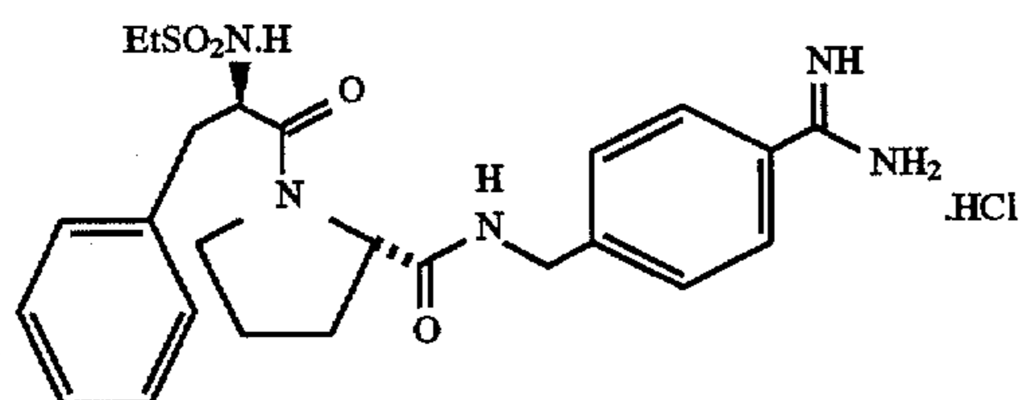
EtSO 2 -D-Phe-Pro-p-NHCH 2 C 6 H 4 C(=NH)NH 2 .HCl (N-(ethylsulfonyl)-D-phenylalanyl-N-[[4-(aminoiminomethyl)phenyl]methyl]-L-prolinamide hydrochloride)
