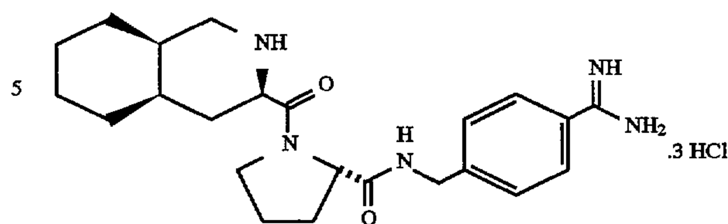
D-3-Piq-Pro-p-NHCH 2 C 6 H 4 C(NH)NH 2 .3HCl
