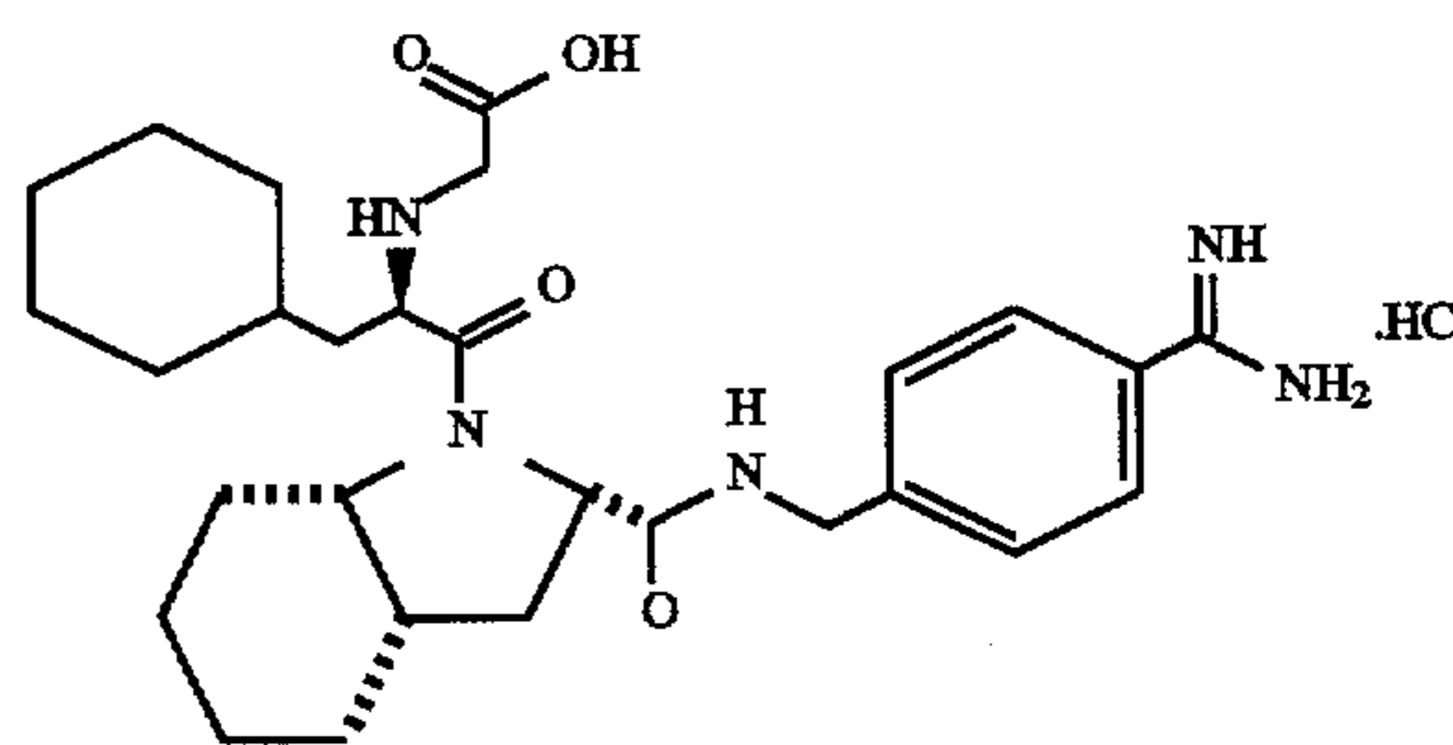
HOOCCH 2 -D-Cha-cis-Ohi-p-NHCH 2 C 6 H 4 C(NH)NH 2 ·HCl ([(S-cis)-N-[[4-aminoiminomethyl]phenyl]methyl]-1-[N-(carboxymethyl)-D-cyclohexylalanyl]-1H-indole-2-carboxamide hydrochloride)
