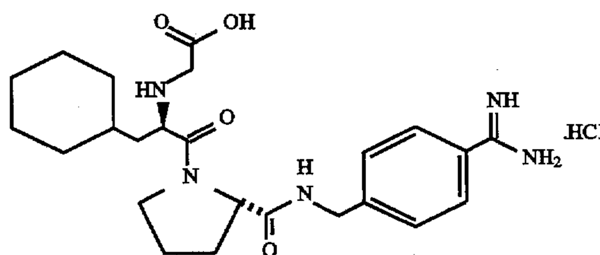
HOOCCH 2 -D-Cha-Pro-p-NHCH 2 C 6 H 4 C(NH)NH 2 ·HCl (N-(carboxymethyl)-D-cyclohexylalanyl-N-[[4-(aminoiminomethyl)phenyl]methyl]-L-prolinamide)
