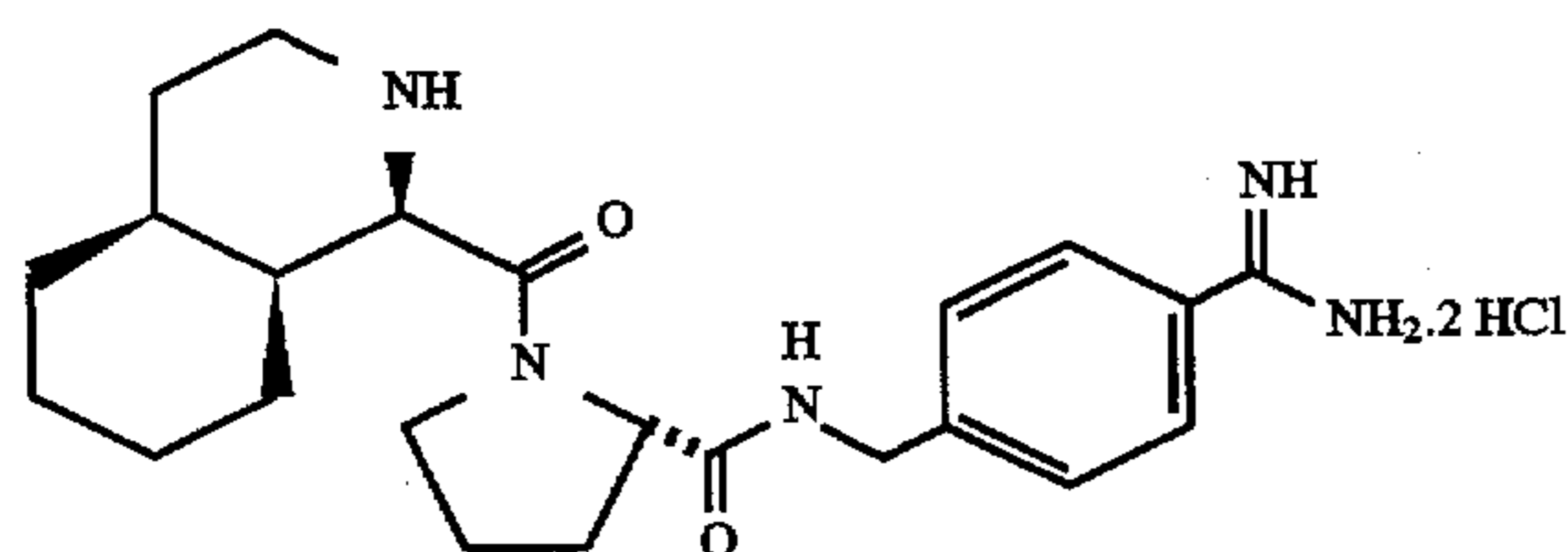
1-Piq-Pro-p-NHCH 2 C 6 H 4 C(NH)NH 2 .2HCl (N-[[4-(aminomethyl)phenyl]methyl]-1-[[4aS,8aS)-decahydro-1(R)-isoquinolinyl]carbonyl]-L-prolinamide dihydrochloride)
