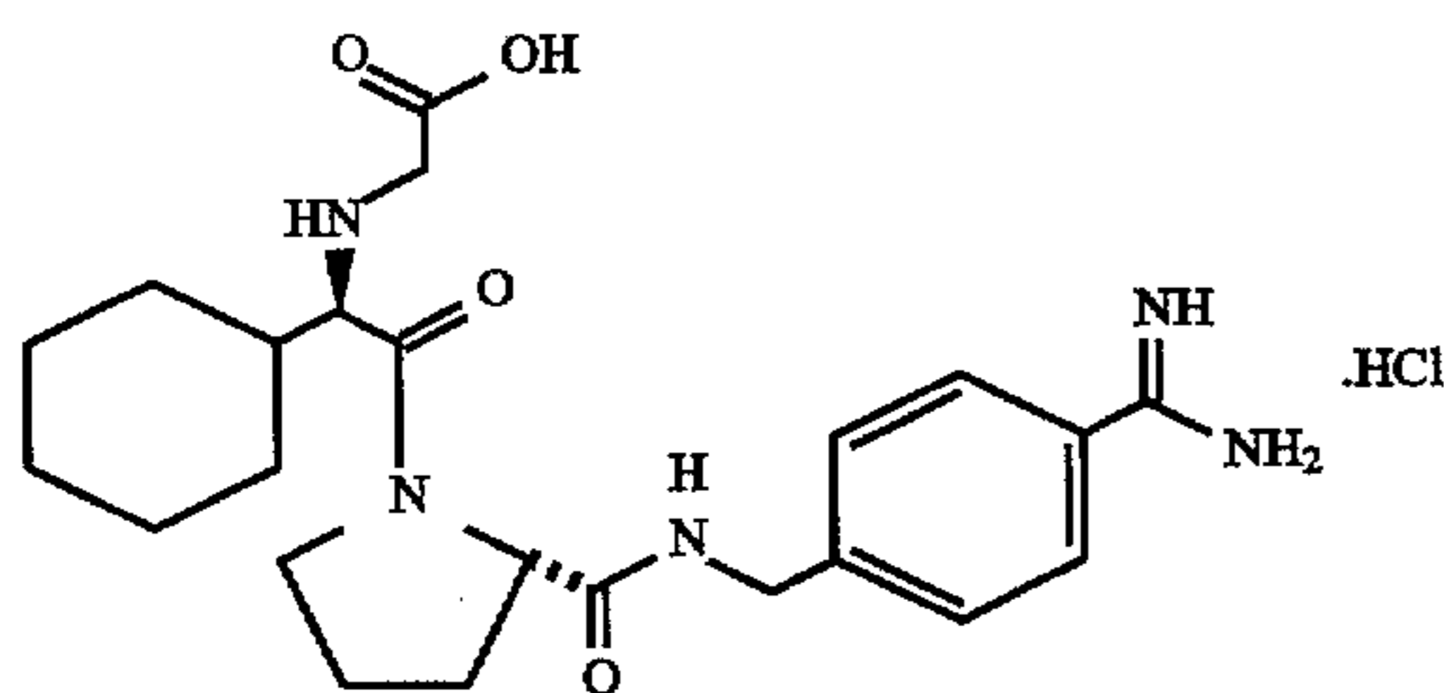
\text{HOOCCH}_2\text{-D-Chg-Pro-p-NHCH}_2\text{C}_6\text{H}_4\text{C(NH)NH}_2\cdot\text{HCl} (N-(carboxymethyl)-D-cyclohexylglycyl-N-[[4-(aminoiminomethyl)phenyl]methyl]-L-prolinamide hydrochloride)
