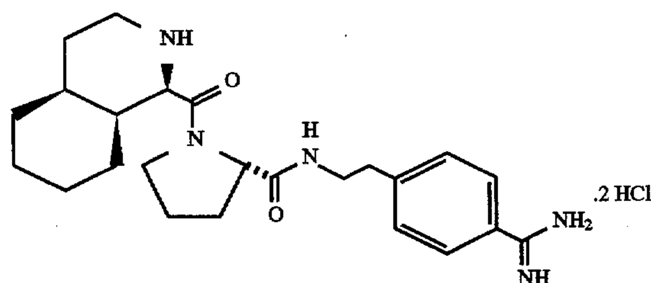
D-1-Piq-Pro-p-NHCH 2 CH 2 —C 6 H 4 C(=NH)NH 2 .2HCl
