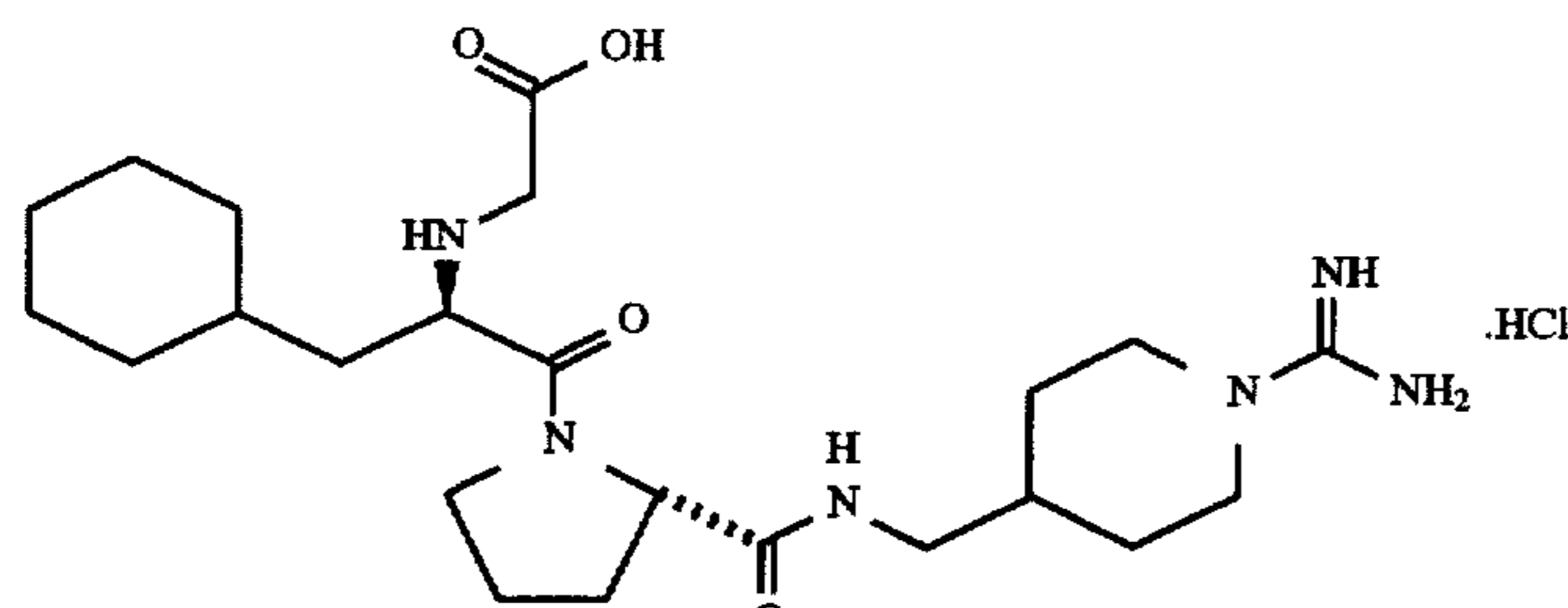
HO 2 CCH 2 -D-Cha-Pro-4-NHCH 2 -1-amidinopiperidine.HCl (N-(carboxymethyl)-d-cyclohexylalanyl-N-[[1-(aminoiminomethyl)-hexahydropyridin-4-yl]-methyl]-L-prodimamide hydrochloride)
