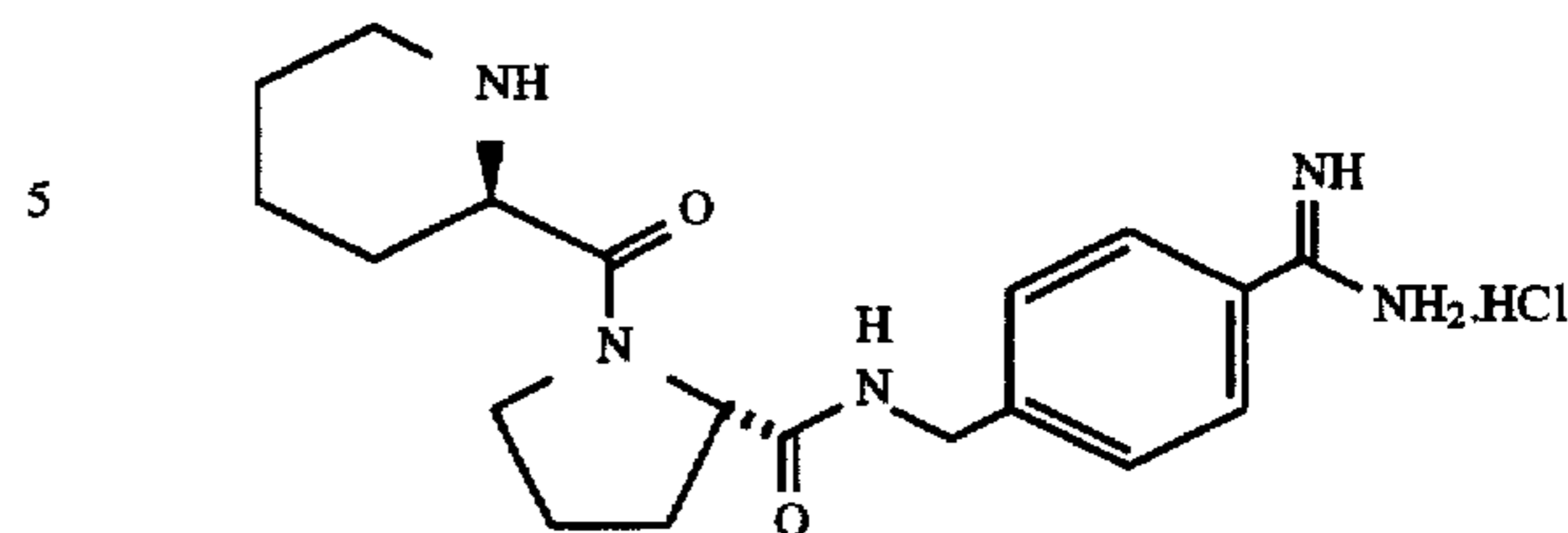
D-hPro-Pro-p-NHCH 2 C 6 H 4 C(NH)NH 2 ·HCl (D-homopropyl-N-[[4-(aminoiminomethyl)phenyl]methyl]-L-prolinamide hydrochloride)
