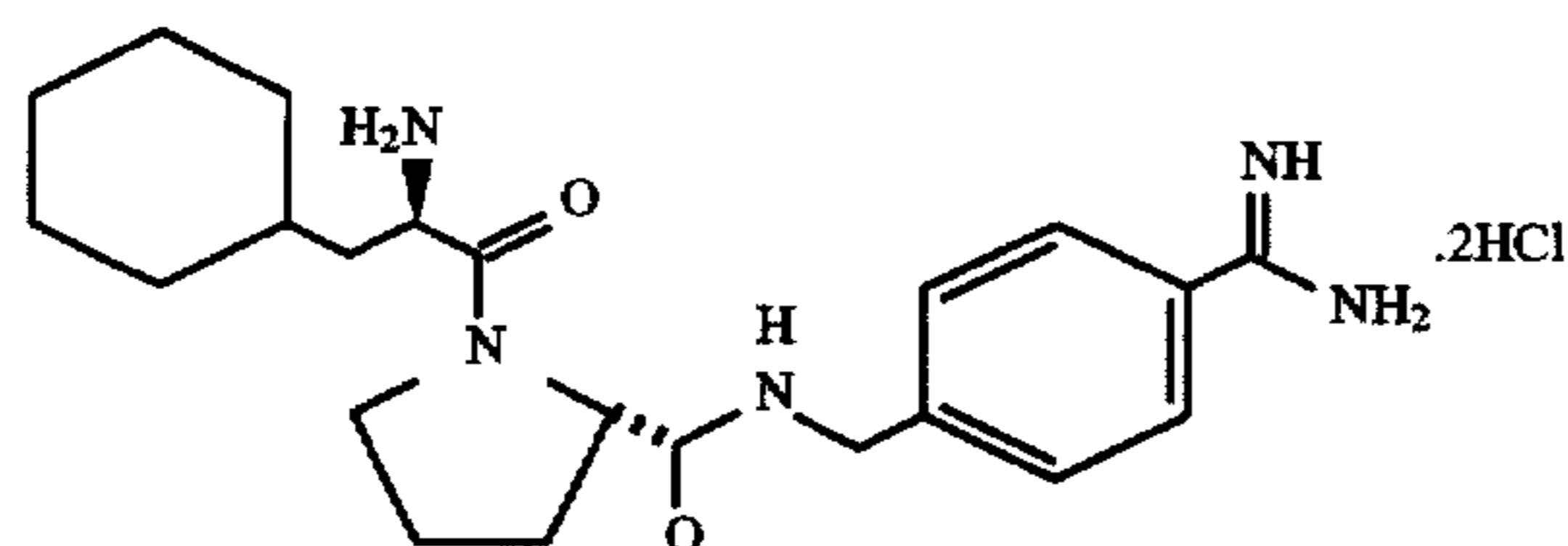
D-Cha-Pro-p-NHCH 2 C 6 H 4 C(NH)NH 2 .2HCl (D-cyclohexylalanyl-N-[[4-(aminoiminomethyl)phenyl]methyl]-L-prolinamide di-hydrochloride)
