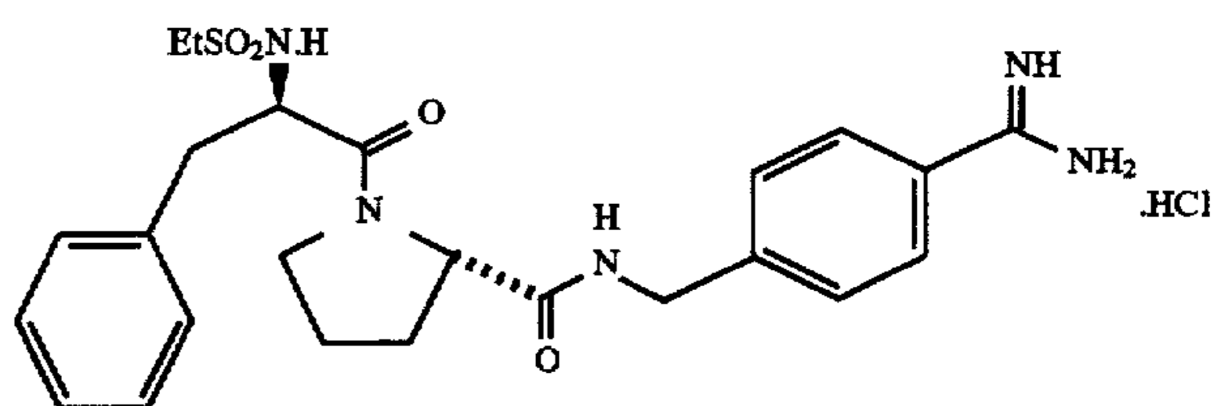
EtSO 2 -D-Phe-Pro-p-NHCH 2 -C 6 H 4 C(NH)NH 2 ·HCl (N-(ethylsulfonyl)-D-phenylalanyl-N-[[4-(aminoiminomethyl)phenyl]methyl]-L-prolinamide hydrochloride)
