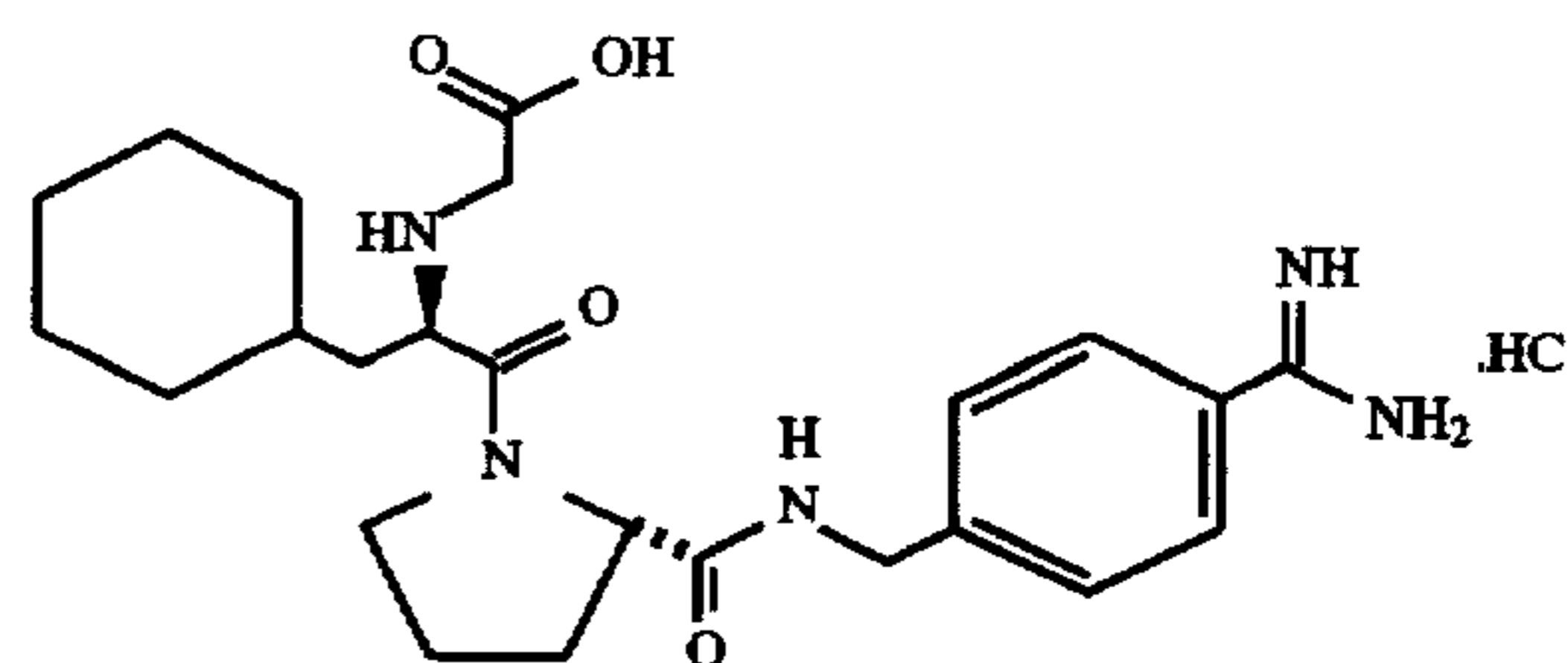
HOOCCH 2 -D-Cha-Pro-p-NHCH 2 C 6 H 4 C(NH)NH 2 ·HCl (N-(carboxymethyl)-D-cyclohexylalanyl-N-[[4-(aminoiminomethyl)phenyl]methyl]-L-prolinamide)
