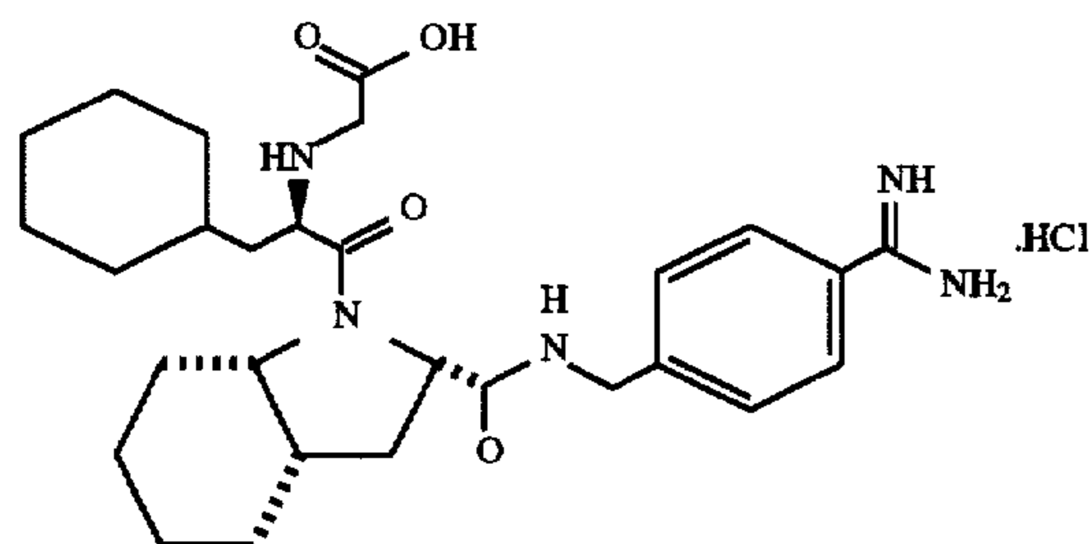
HOOCCH 2 -D-Cha-cis-Ohi-p-NHCH 2 C 6 H 4 C(NH)NH 2 .HCl ((S-cis)-N-[[4-aminoiminomethyl]phenyl]methyl]- 1-[N-(carboxymethyl)-D-cyclohexylalanyl]-octahydro-1H-indole- 2-carboxamide hydrochloride)
