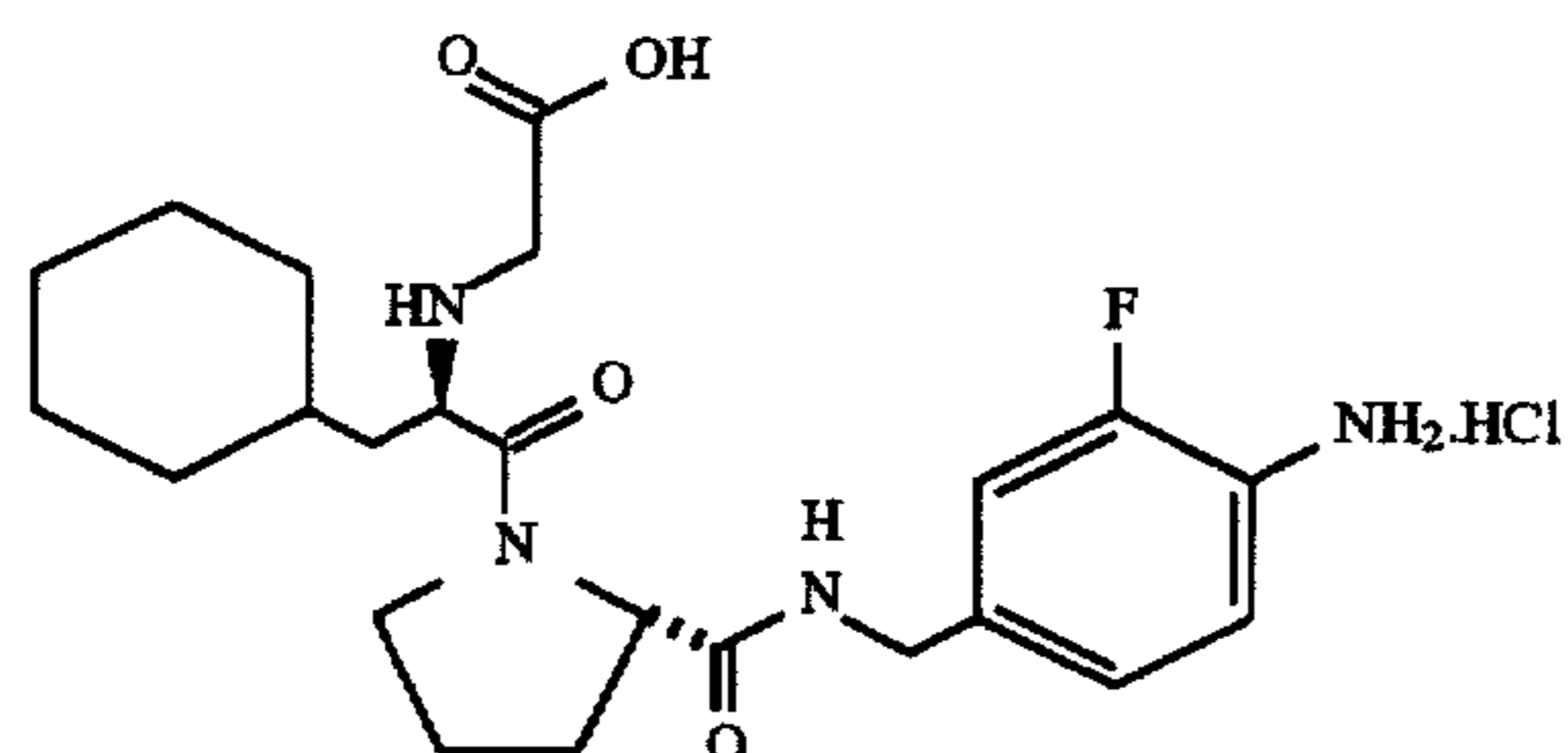
HO 2 CCH 2 -D-Cha-Pro-4-NHCH 2 -2-F-aniline.HCl
