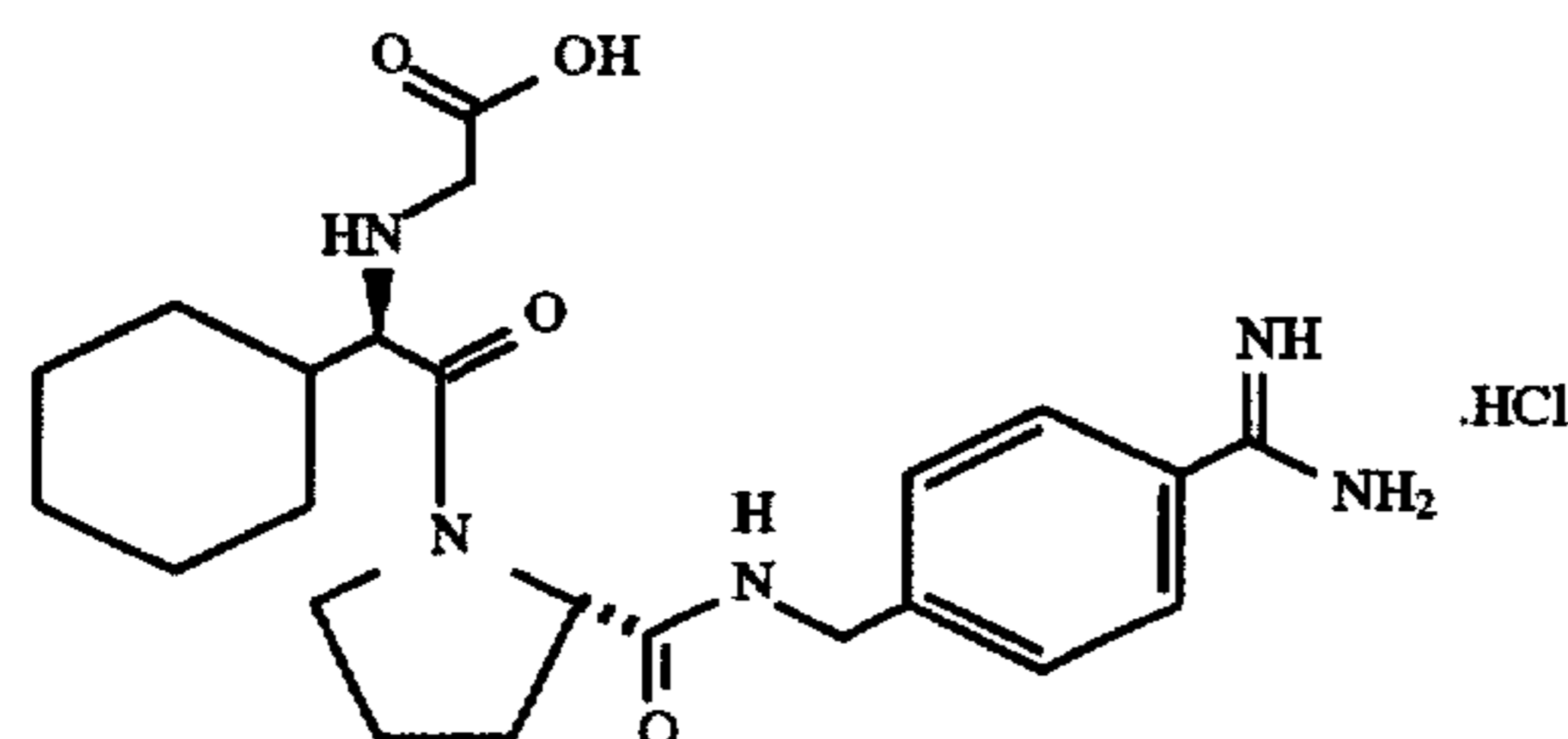
HOOCCH 2 -D-Chg-Pro-p-NHCH 2 C 6 H 4 C(NH)NH 2 .HCl (N-(carboxymethyl)-D-cyclohexylglycyl-N-[[4-(aminoiminomethyl)phenyl]methyl]-L-prolinamide hydrochloride)
