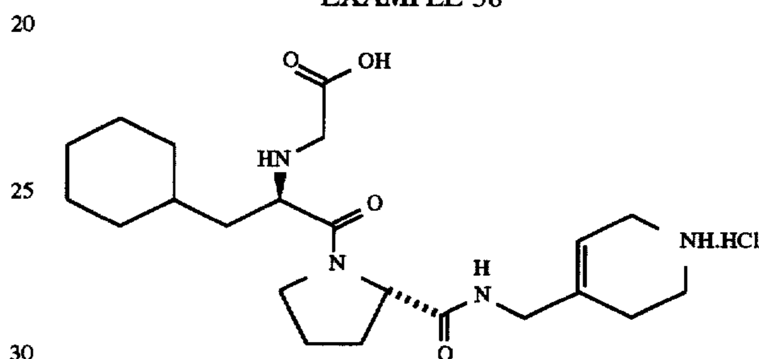
HO 2 CCH 2 -D-Cha-Pro-4-NHCH 2 -3,4-dehydropiperidine.HCl
