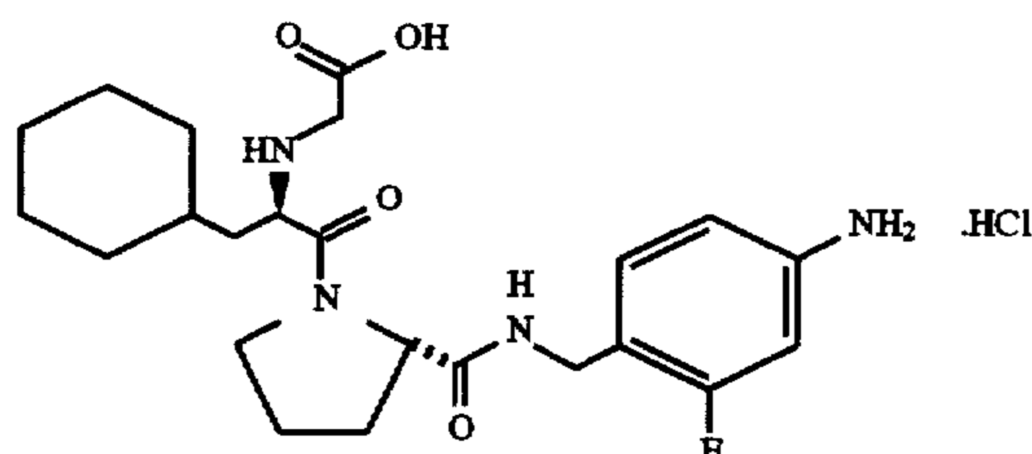
HO 2 CCH 2 -D-Cha-Pro-4-NHCH 2 -3-F-C 6 H 3 NH 2 .HCl
