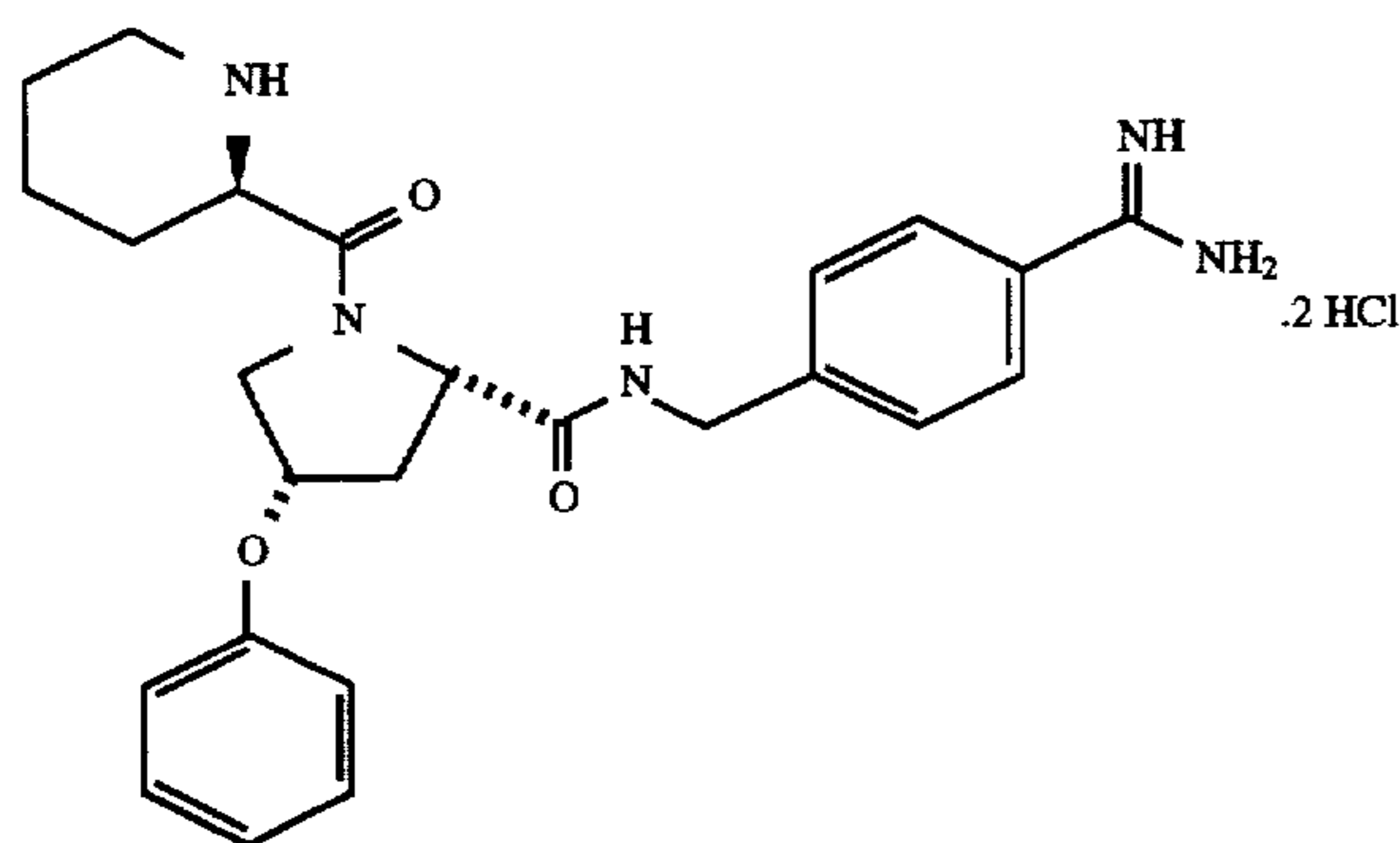
D-hPro-Pro(4-cis-PhO)-p-NHCH 2 -C 6 H 4 C(NH)NH 2 ·2HCl (cis-D-homoprolyl-N-[[4-(aminoiminomethyl)phenyl]methyl]-4-phenoxy-L-prolinamide dihydrochloride)
