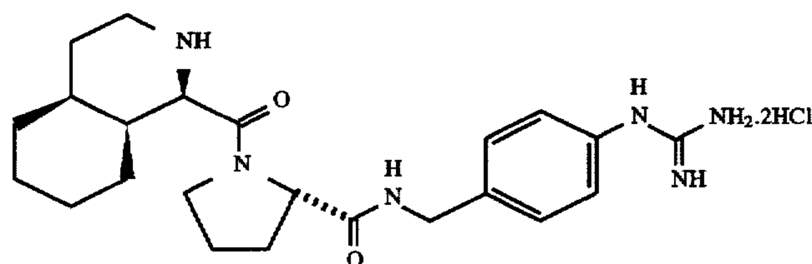
D-1-Piq-Pro-p-NHCH 2 C 6 H 4 NHC(NH)NH 2 .2HCl
