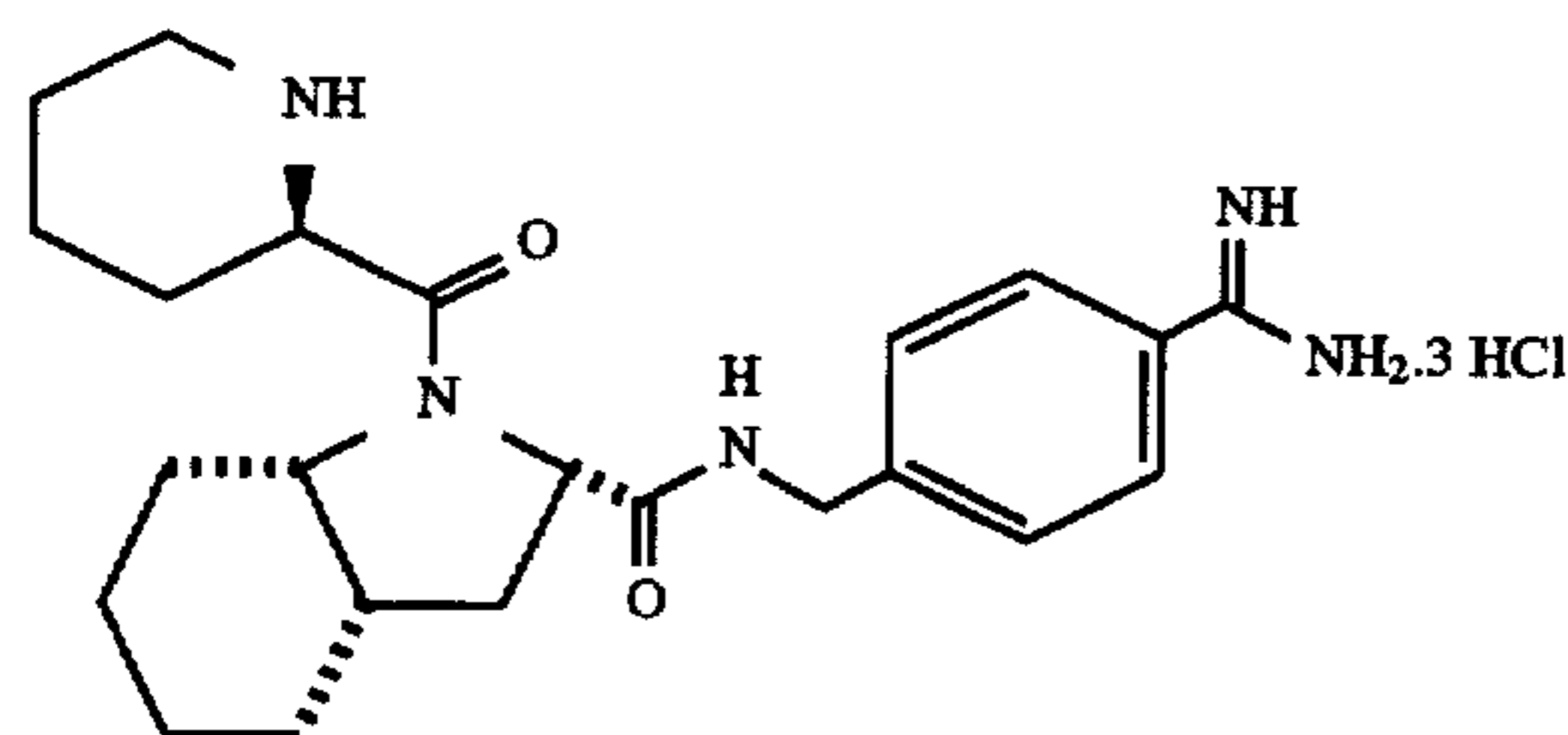
D-hPro—Ohi-p-NHCH 2 C 6 H 4 C(NH)NH 2 ·3HCl ((S-cis)-N-[[4-(aminoiminomethyl)phenyl]methyl]-octahydro-1-D-homopropyl-1H-indole-2-carboxamide trihydrochloride)
