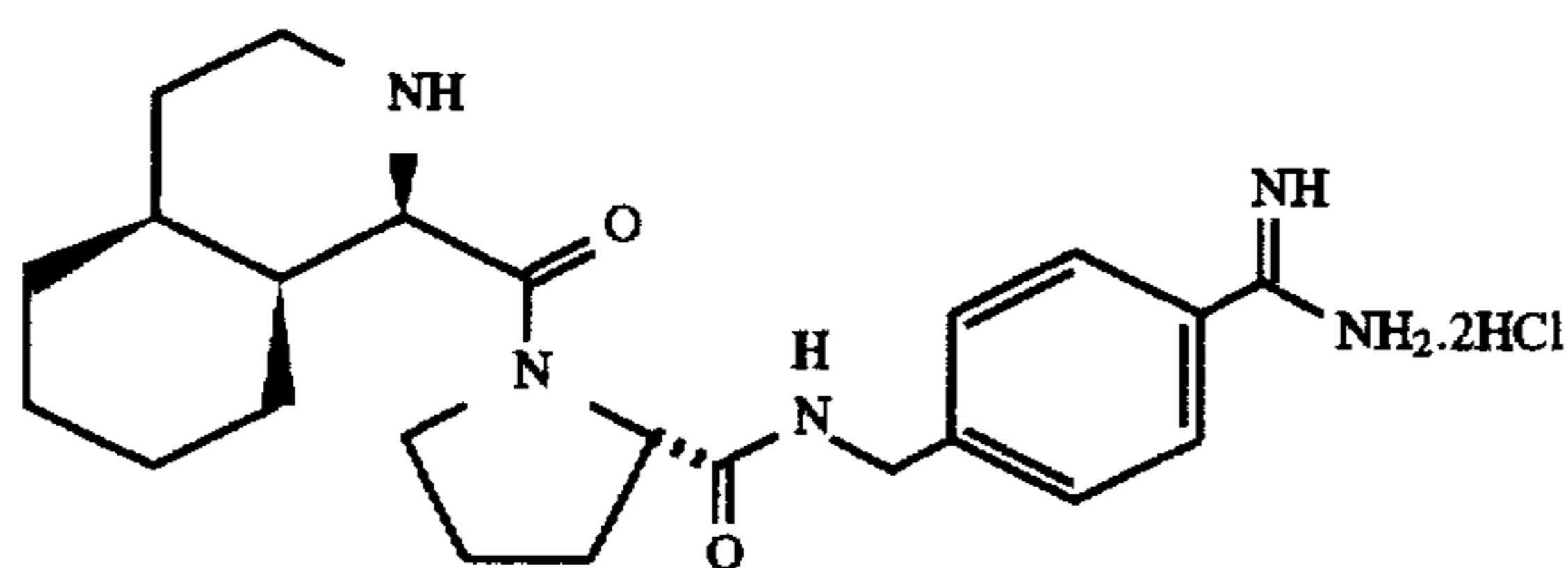
1-Piq-Pro-p-NHCH 2 C 6 H 4 C(NH)NH 2 ·2HCl (N-[[4-(aminomethyl)phenyl]methyl]-1-[[4aS,8aS]-decahydro-1(R)-isoquinolinyl]carbonyl]-L-prolinamide dihydrochloride)
