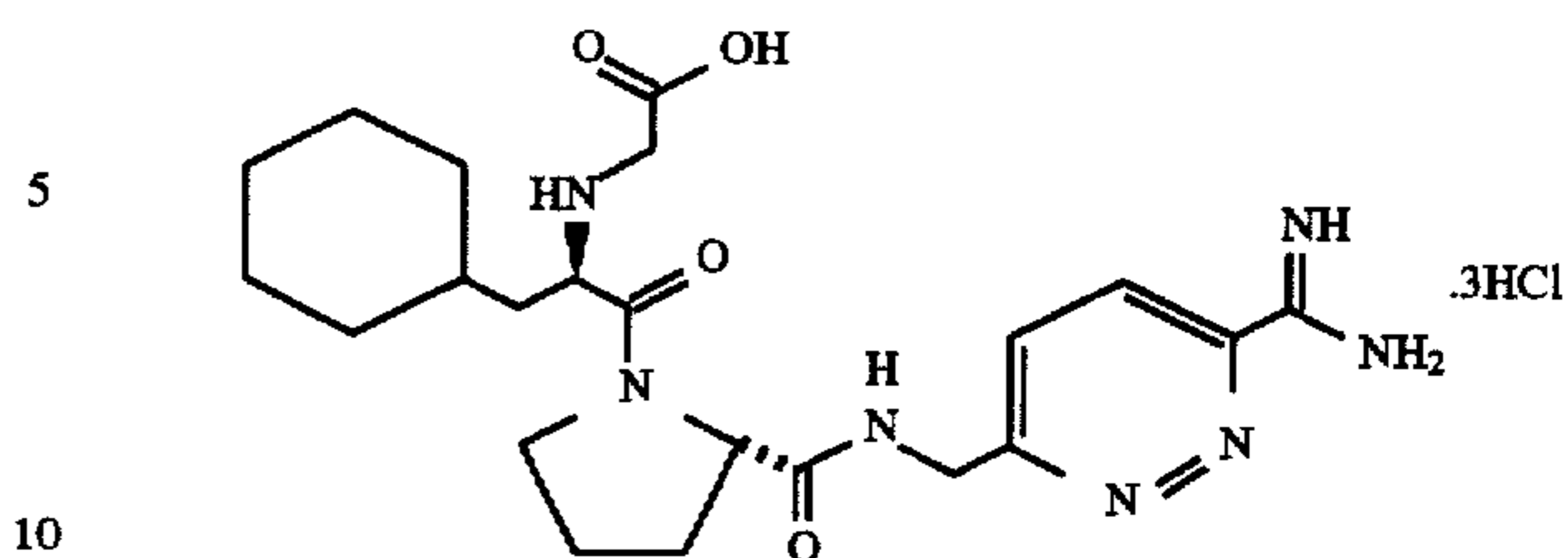
HO_2CCH_2 -D-Cha-Pro-3-NHCH 2 -6-amidino-pyridazine.3HCl (N-(carboxymethyl)-D-cyclohexylalanyl-N-[6-(aminoimino-methyl)pyridazin-3-yl]methyl]L-prolinamide tri-hydrochloride)
