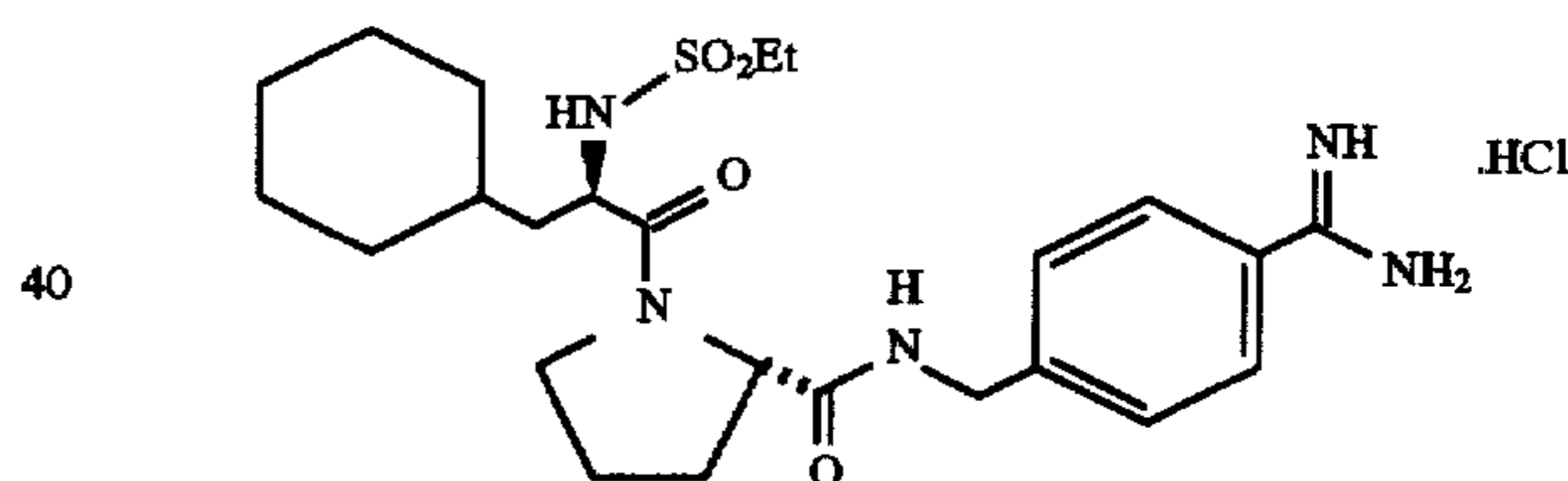
EtSO 2 -D-Cha-Pro-4-NHCH 2 -C 6 H 4 C(NH)NH 2 .HCl (N-(ethylsulfonyl)-D-cyclohexylalanyl-N-[[4-(aminoiminomethyl)phenyl]methyl]-L-prolinamidehydrochloride)
