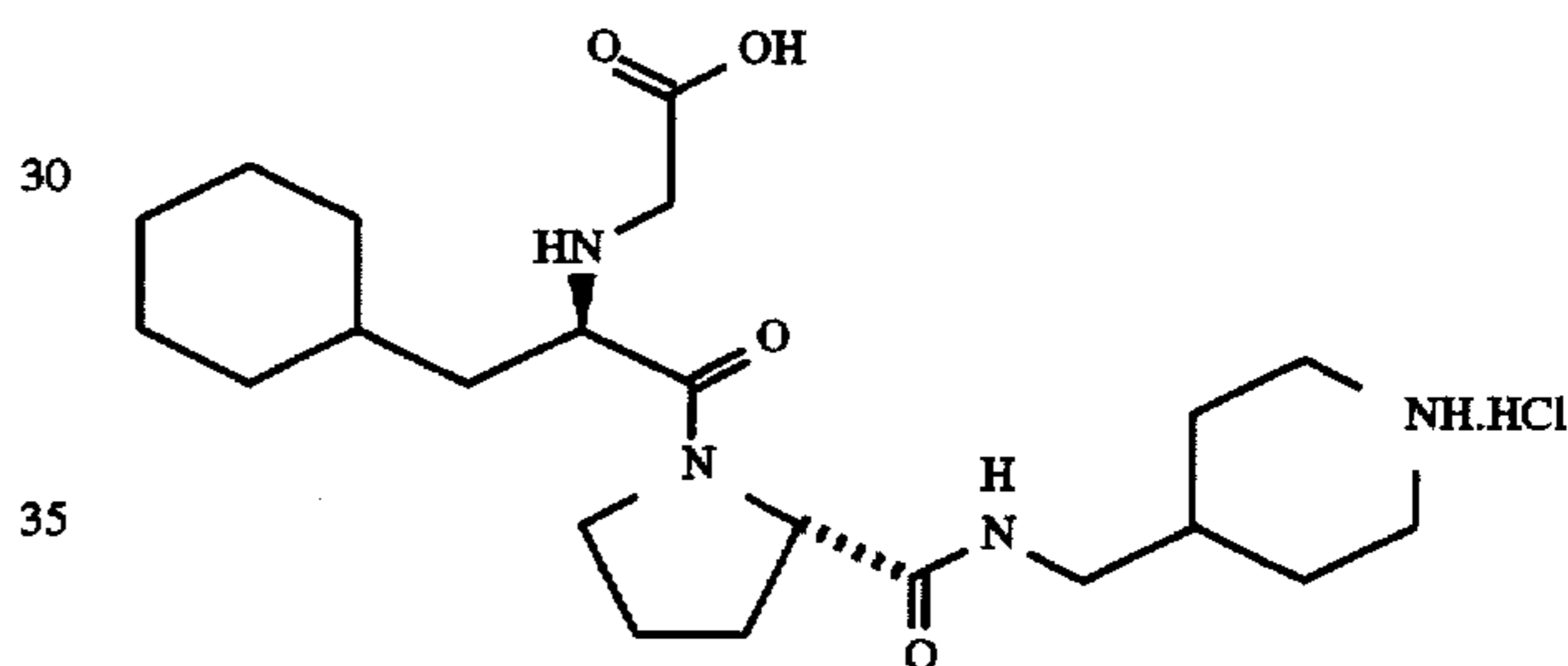
HO 2 CCH 2 -D-Cha-Pro-4-NHCH 2 -piperidine.HCl
