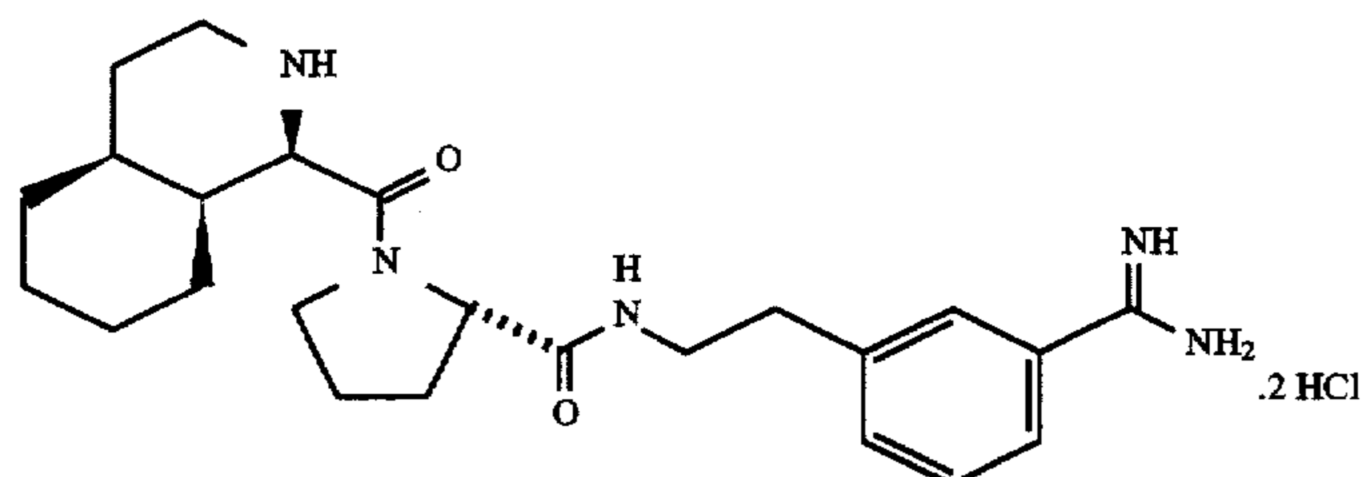
D-1-Piq-Pro-m-NHCH 2 CH 2 -C 6 H 4 C(=NH)NH 2 .2HCl
