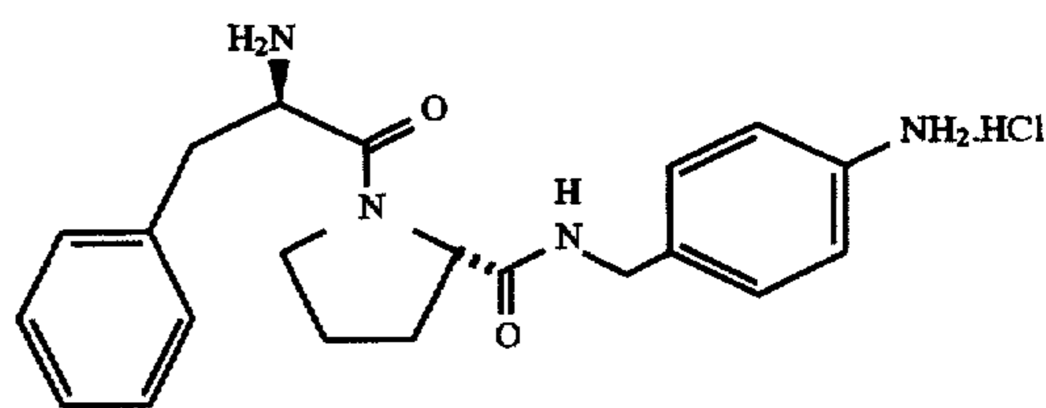
D-Phe-Pro-p-NHCH 2 C 6 H 4 NH 2 .HCl
