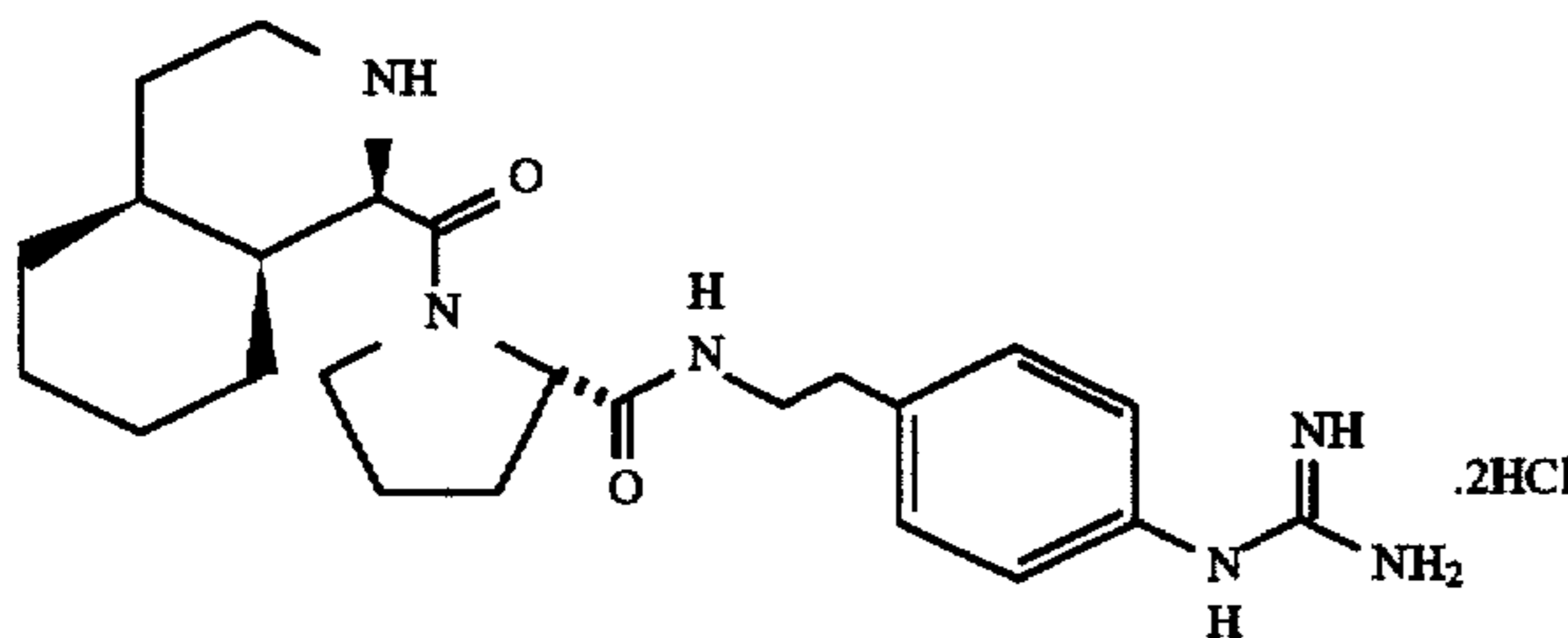
D-1-Piq-Pro-p-NHCH 2 CH 2 C 6 H 4 NHC(NH)NH 2 .2HCl
