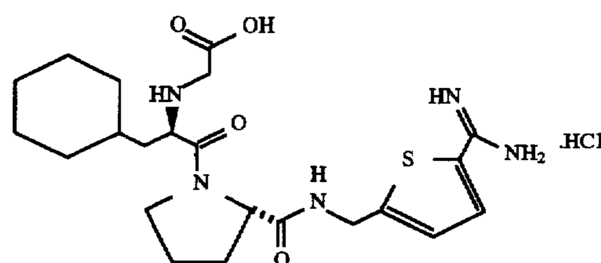
HO 2 CCH 2 -D-Cha-Pro-4-NHCH 2 -2-amidinothiophene.HCl
