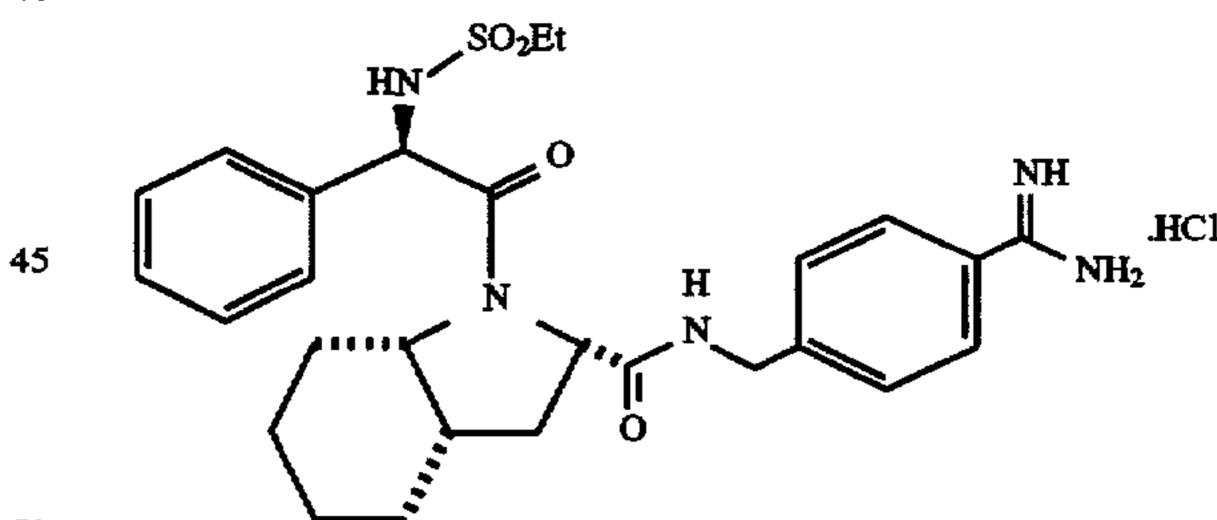
EtSO 2 -Phg-cis-Ohi-p-NHCH 2 C 6 H 4 C(NH)NH 2 .HCl (S-cis)-N-[[4-(amino iminomethyl)phenyl]methyl]-1-[N-(ethylsulfonyl)-D-phenylglycyl]-octahydro-1H-indole-2-carboxamide hydrochloride
