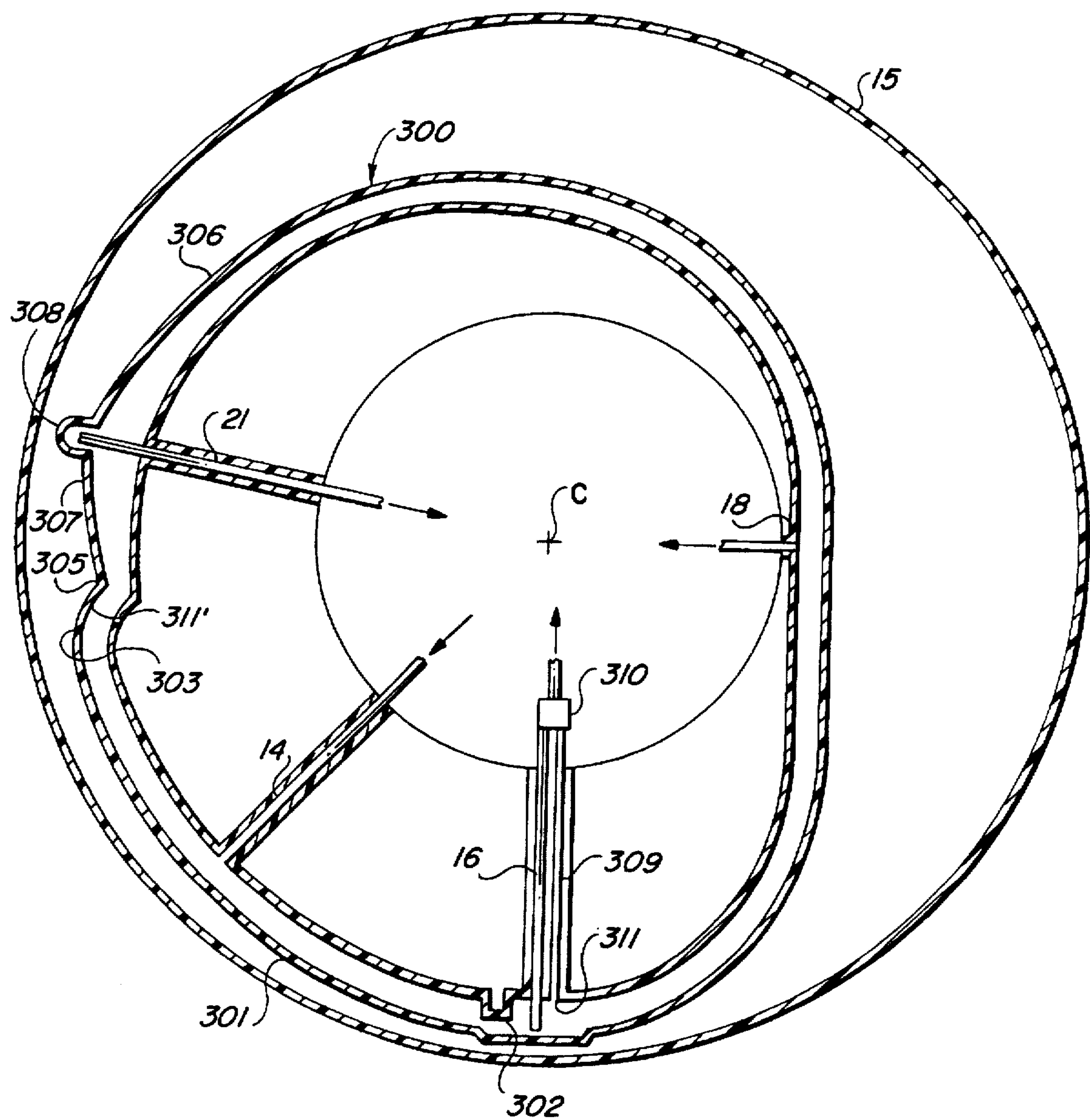
FIG. 3 (PRIOR ART)
