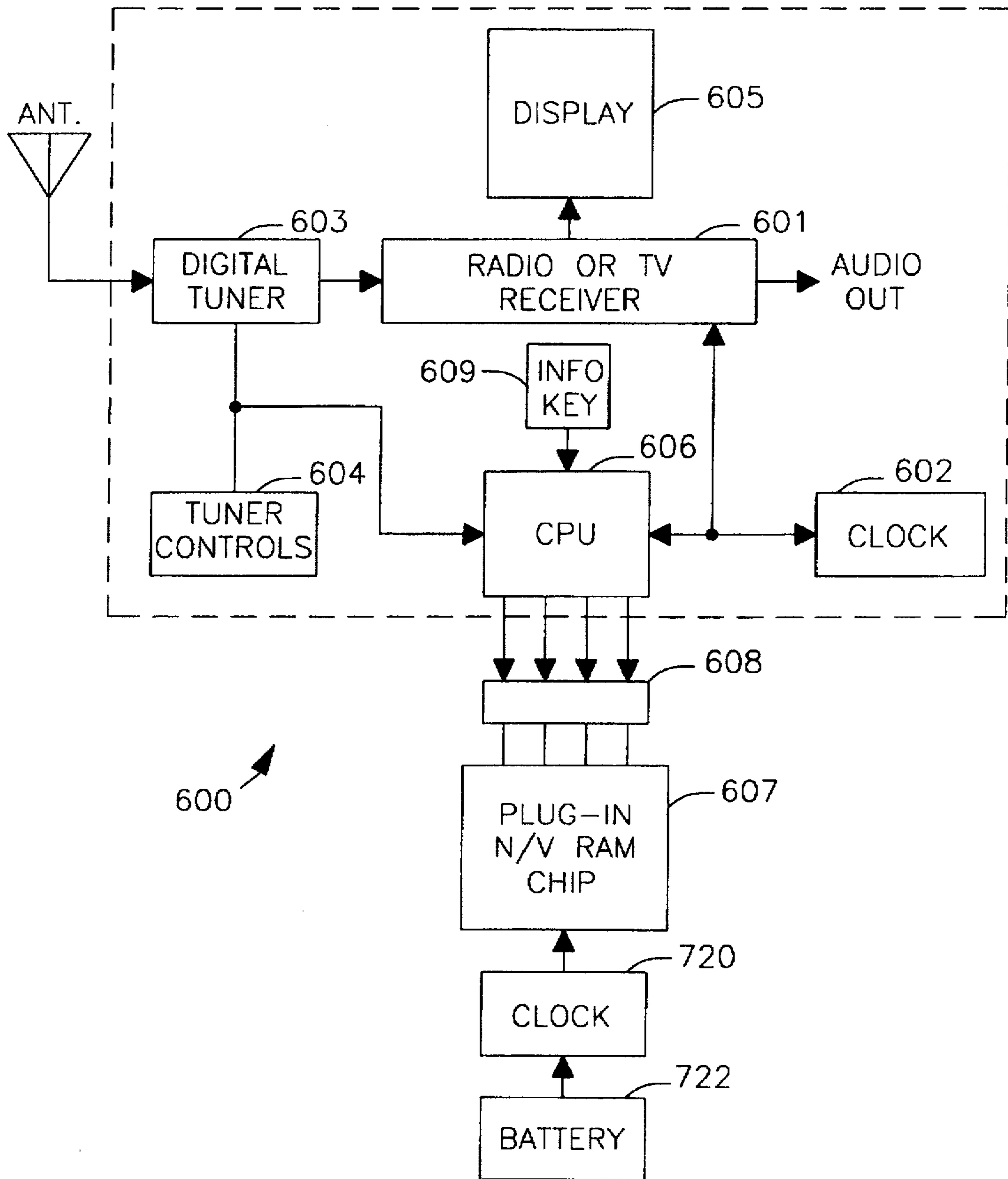
FIG. 8 CAR/HOME RADIO/TV
