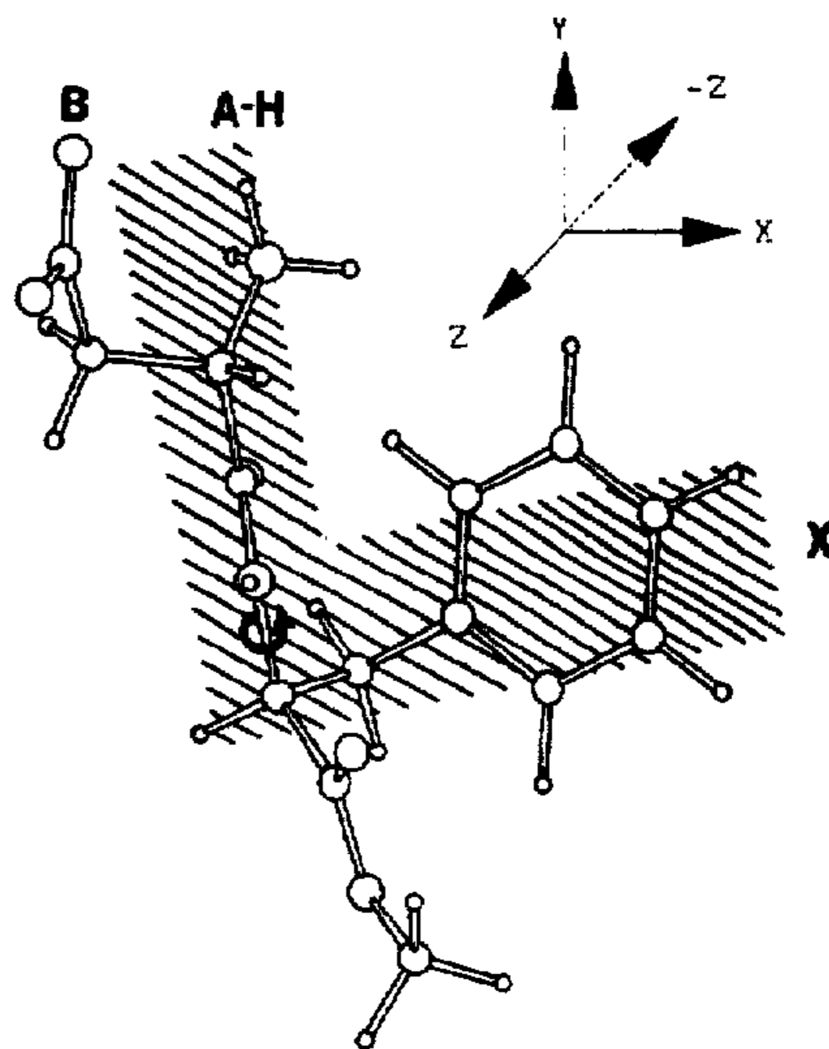
FIG. 2 a-d. Preferred minimum energy conformations of (A) N-(L-aspartyl)-N'-(tetramethylcyclopentanoyl)-(R)-1,1-diaminoethane, (B) N-(L-aspartyl)-N'-(tetramethylcyclopentanoyl) (S)-1,1-diaminoethane, (C) L-aspartyl-D-alanyl-tetramethylcyclopentylamide and (D) L-aspartyl-L-alanyl-tetramethylcyclopentylamide.
