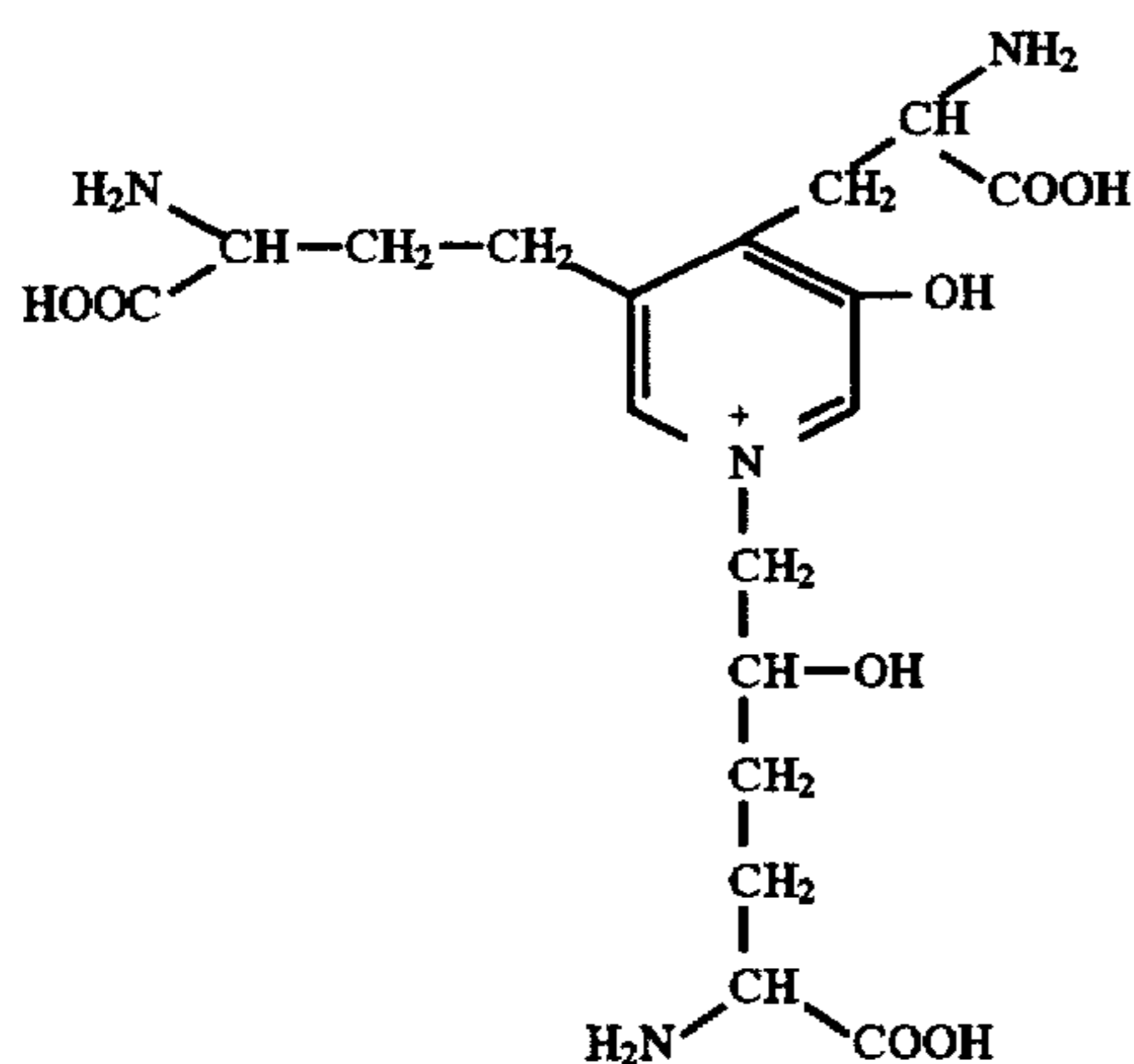
hydroxylysyl pyridinoline (HP)
