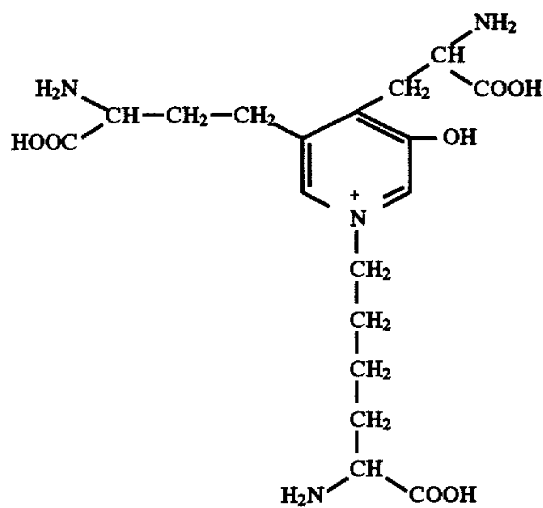
lysyl pyridinoline (LP)
