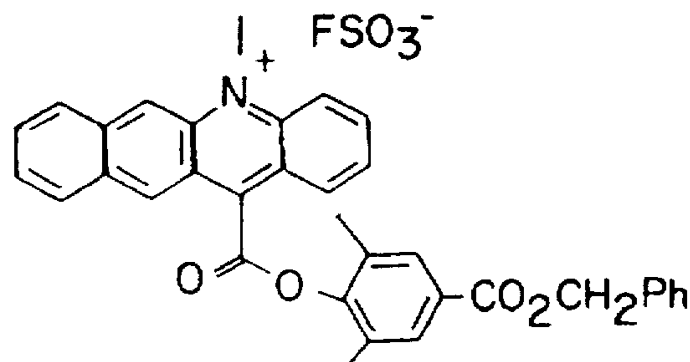
LEAE-Bz
