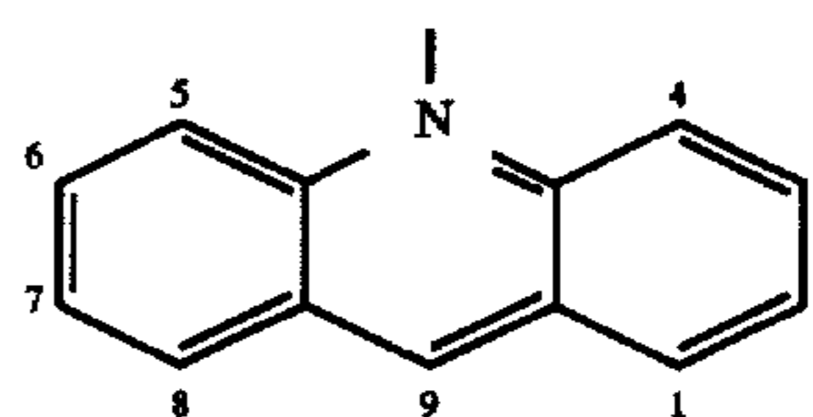
Acridinium nucleus
