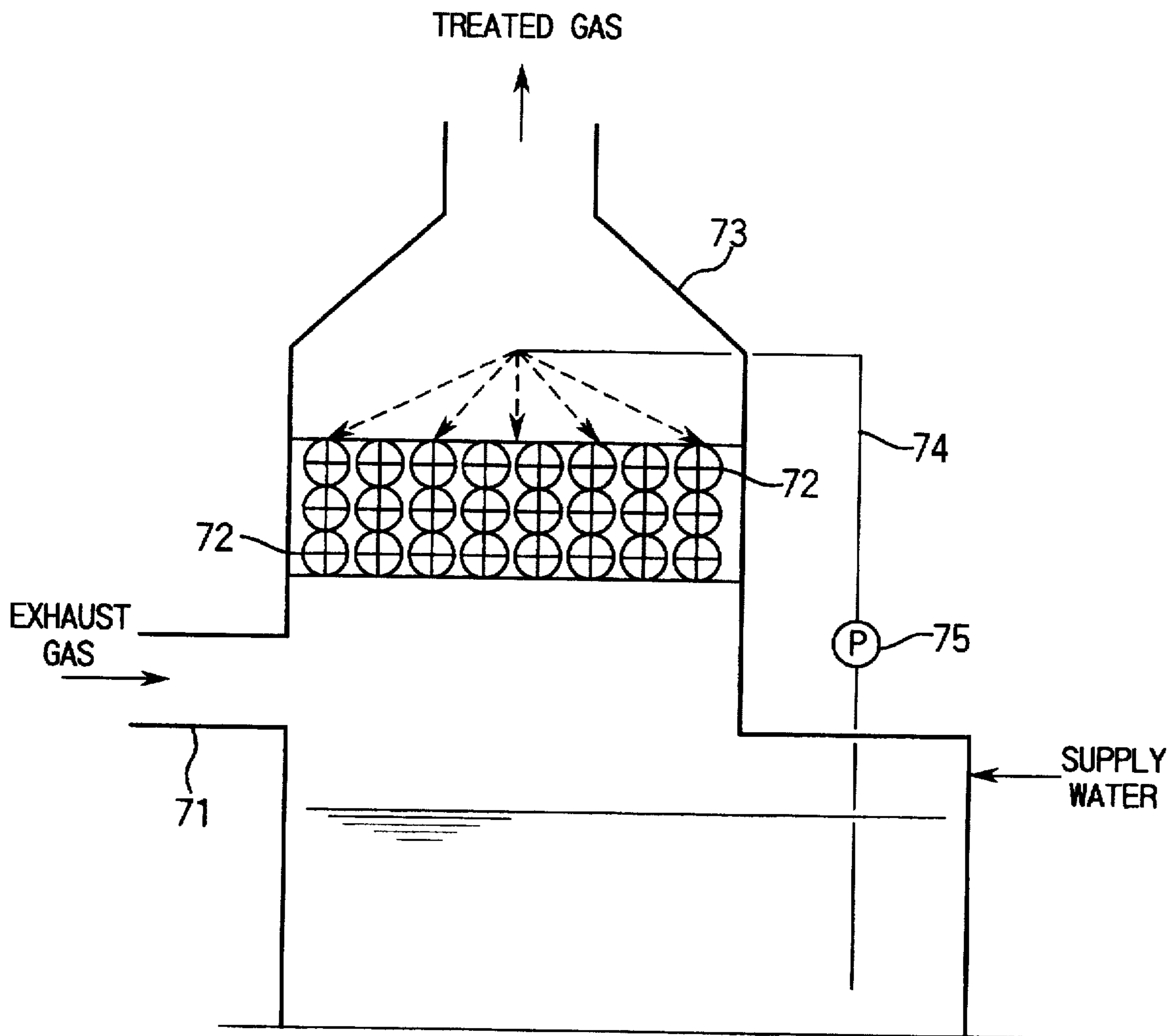
Fig.7 PRIOR ART
