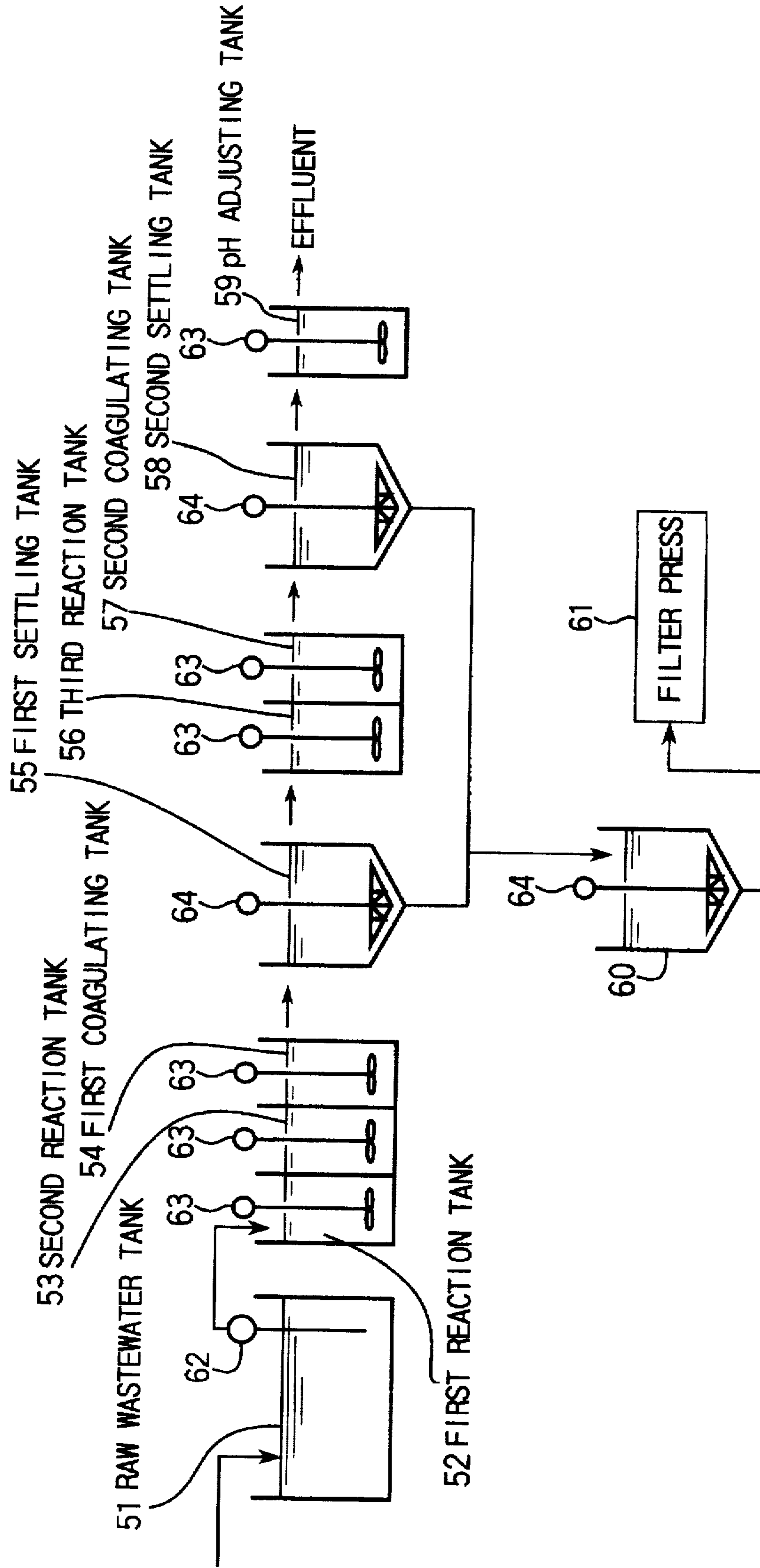
Fig.5 PRIOR ART
