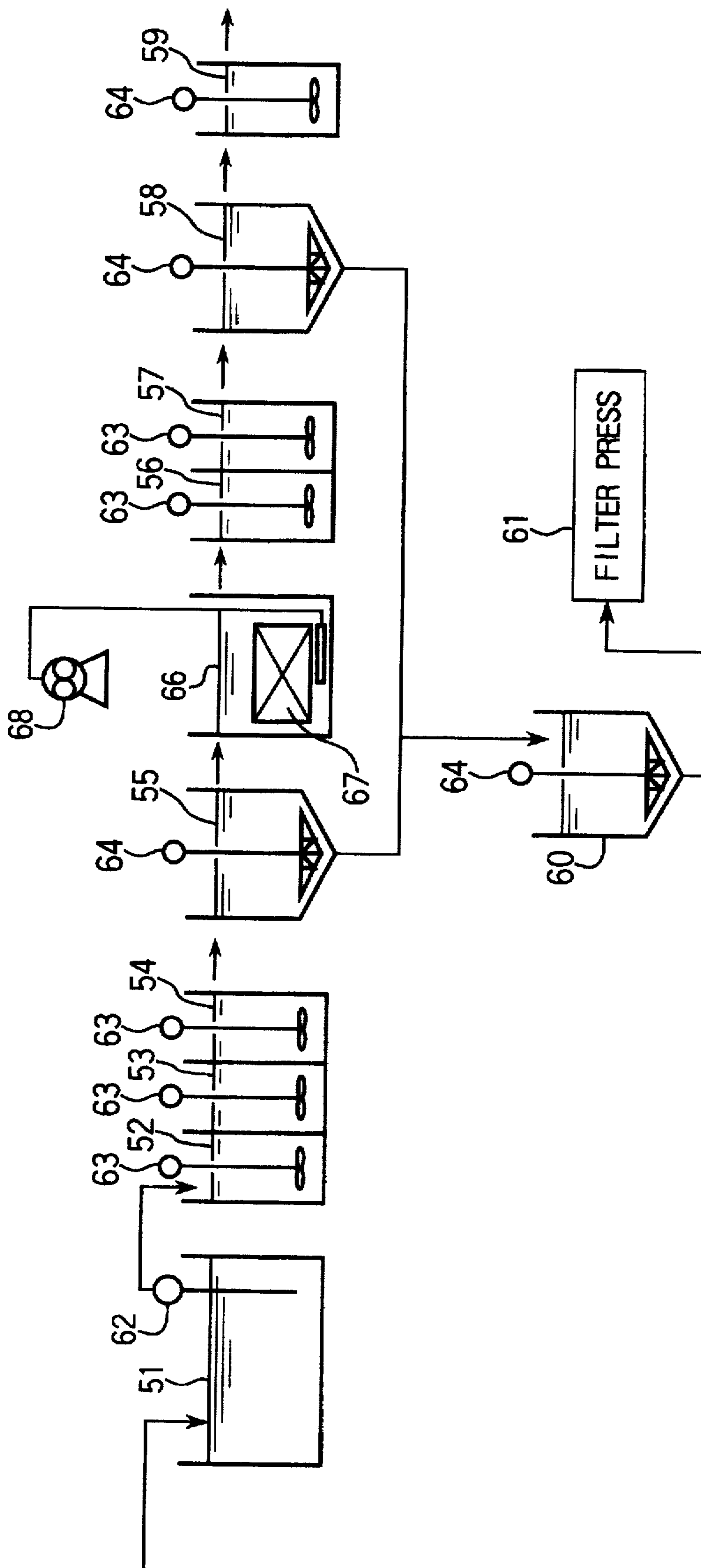
Fig.6 PRIOR ART
