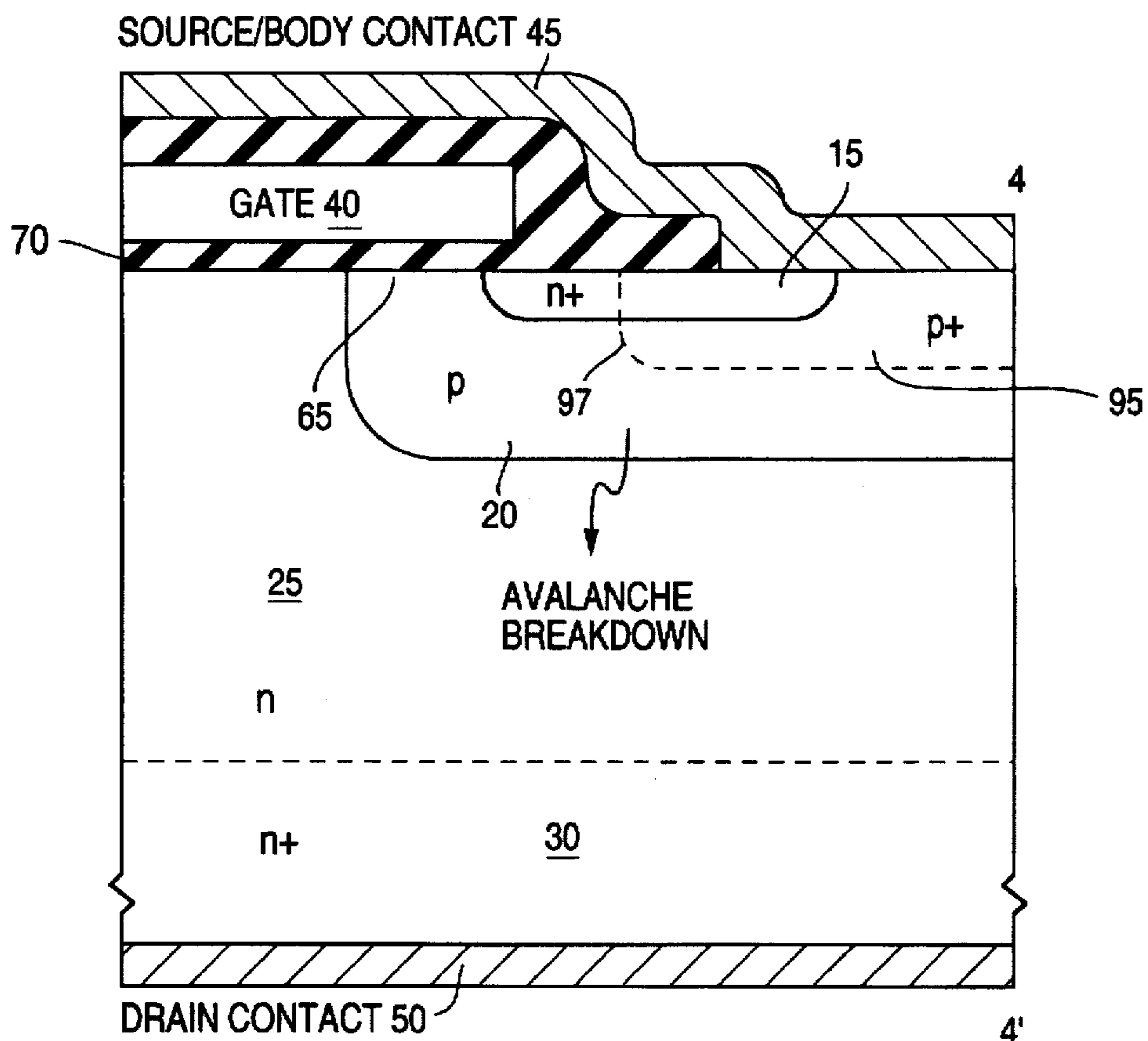
FIG. 4 PRIOR ART
