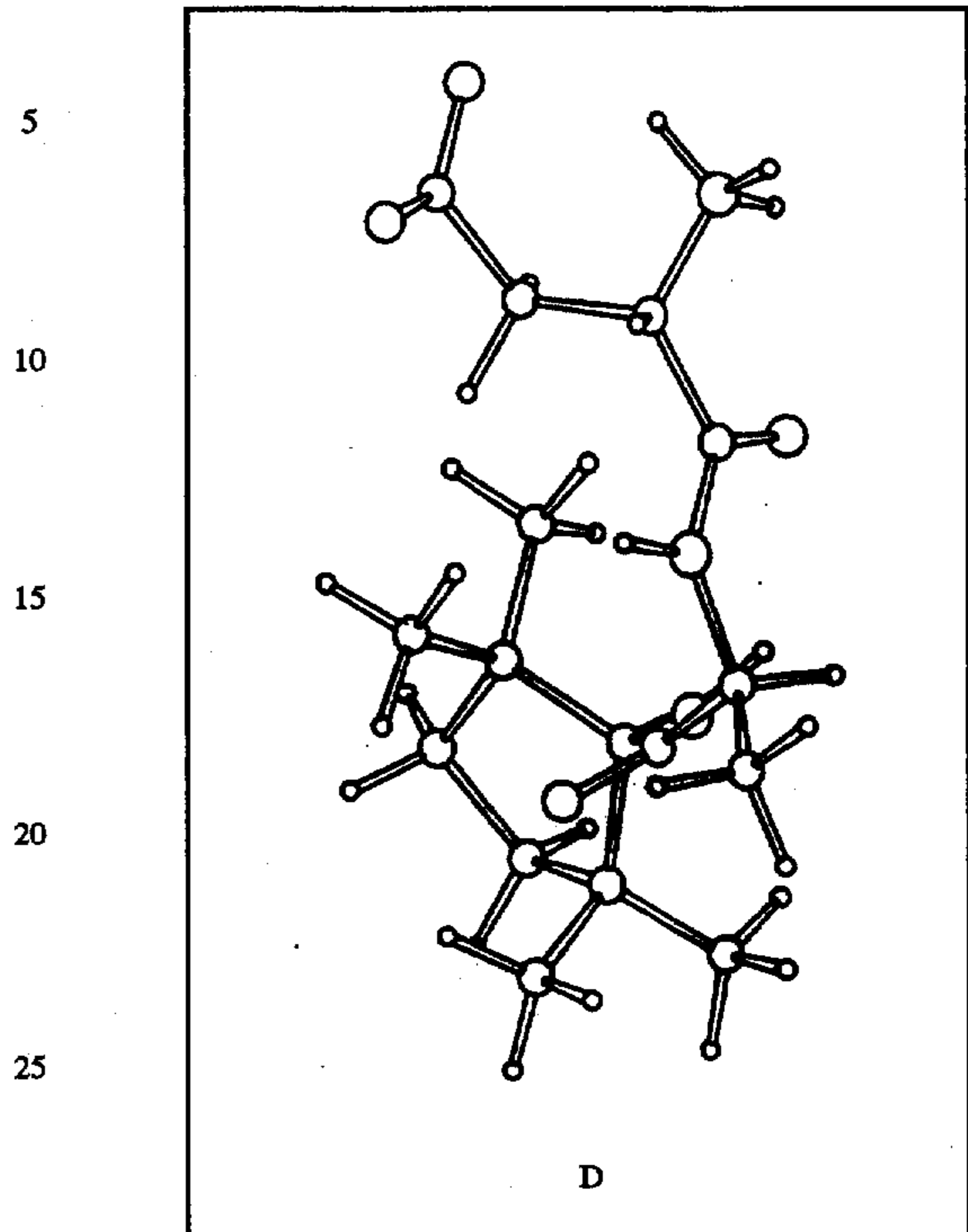
FIG. 2d FIGS. 2a-d. Preferred minimum energy conformations of (A) N-(L-aspartyl)-N'-(tetramethylcyclopentanyl)-(R)-1,1-diaminoethane, (B) N-(L-aspartyl)-N'-(tetramethylcyclopentanyl) (S)-1,1-diaminoethane, (C) L-aspartyl-D-alanyl-tetramethylcyclopentylamide and (D) L-aspartyl-L-alanyl-tetramethylcyclopentylamide.
