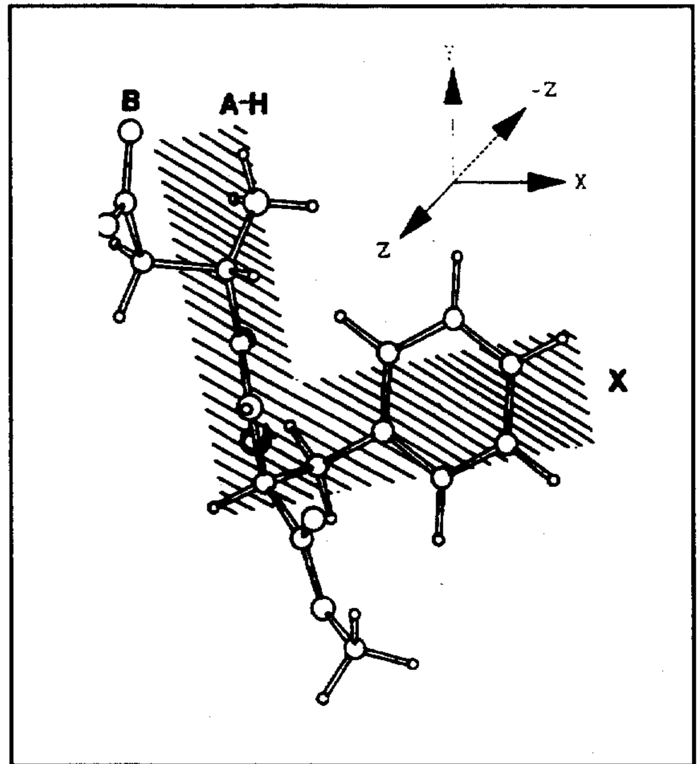
FIG. 2d FIGS. 2a-d. Preferred minimum energy conformations of (A) N-(L-aspartyl)-N'-(tetramethylcyclopentanyl)-(R)-1,1-diaminoethane, (B) N-(L-aspartyl)-N'-(tetramethylcyclopentanyl) (S)-1,1-diaminoethane, (C) L-aspartyl-D-alanyl-tetramethylcyclopentylamide and (D) L-aspartyl-L-alanyl-tetramethylcyclopentylamide.
