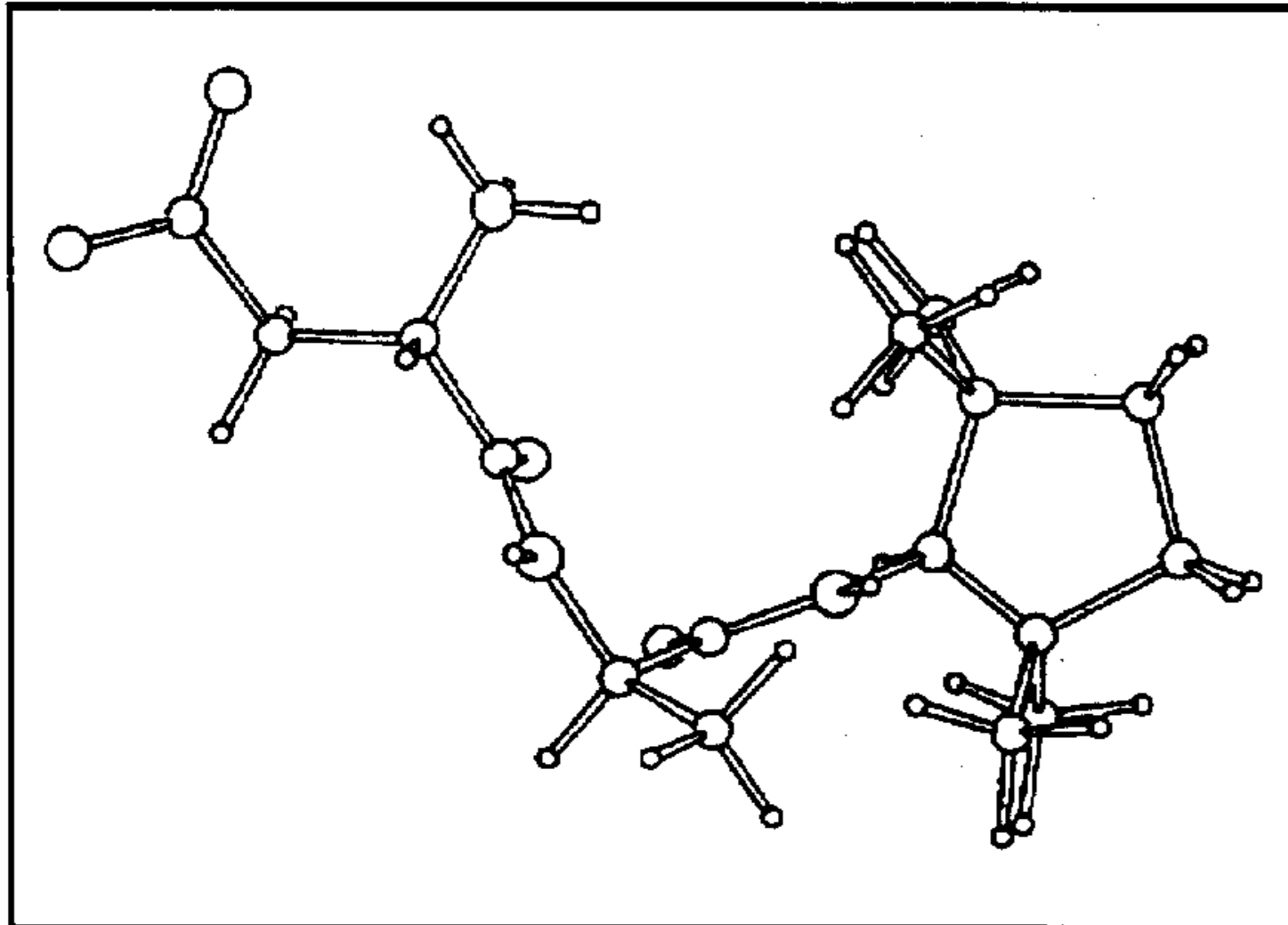
FIG. 2d FIGS. 2a-d. Preferred minimum energy conformations of (A) N-(L-aspartyl)-N'-(tetramethylcyclopentanyl)-(R)-1,1-diaminoethane, (B) N-(L-aspartyl)-N'-(tetramethylcyclopentanyl) (S)-1,1-diaminoethane, (C) L-aspartyl-D-alanyl-tetramethylcyclopentylamide and (D) L-aspartyl-L-alanyl-tetramethylcyclopentylamide.
