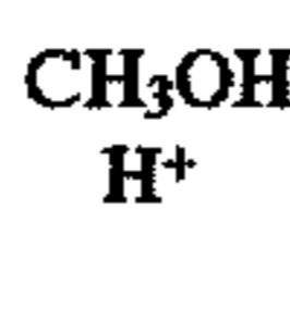
3,6-Dioxaoctanedioic acid
