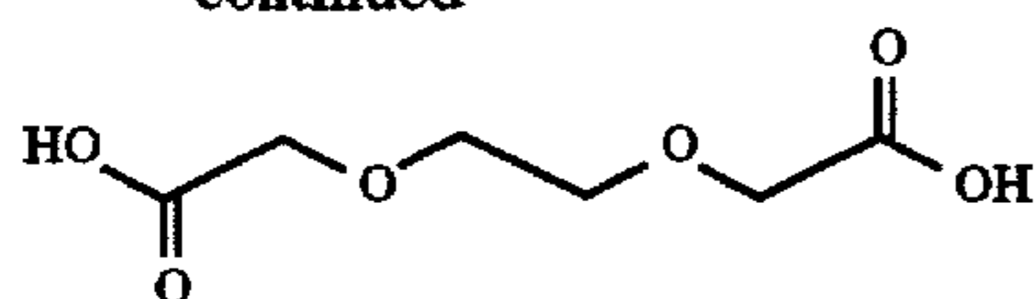
3,6-Dioxaoctanedioic acid
