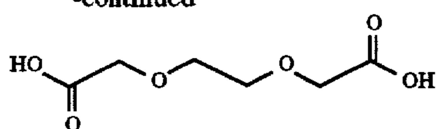
3,6-Dioxaoctanedioic acid
