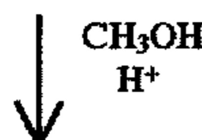
3,6-Dioxaoctanedioic acid
