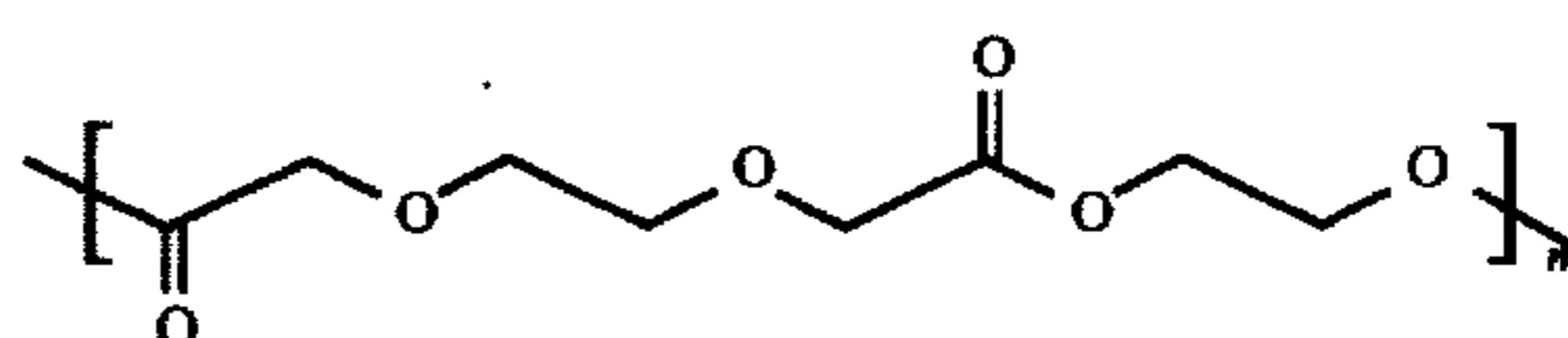
POLY"OXA"ESTERS
