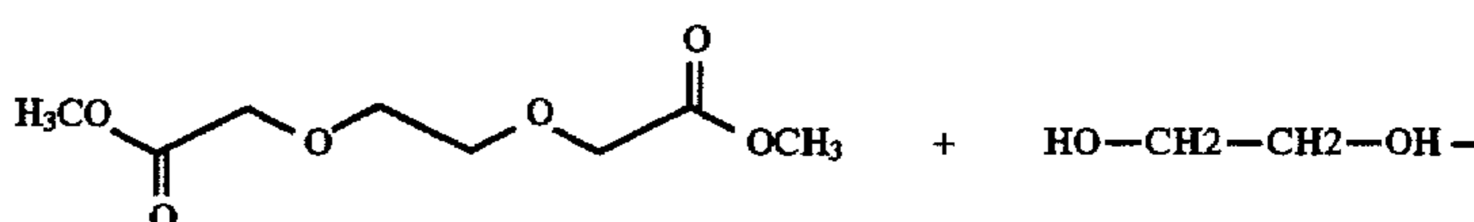
Methyl esters of 3,6-dioxaoctanedioic acid
