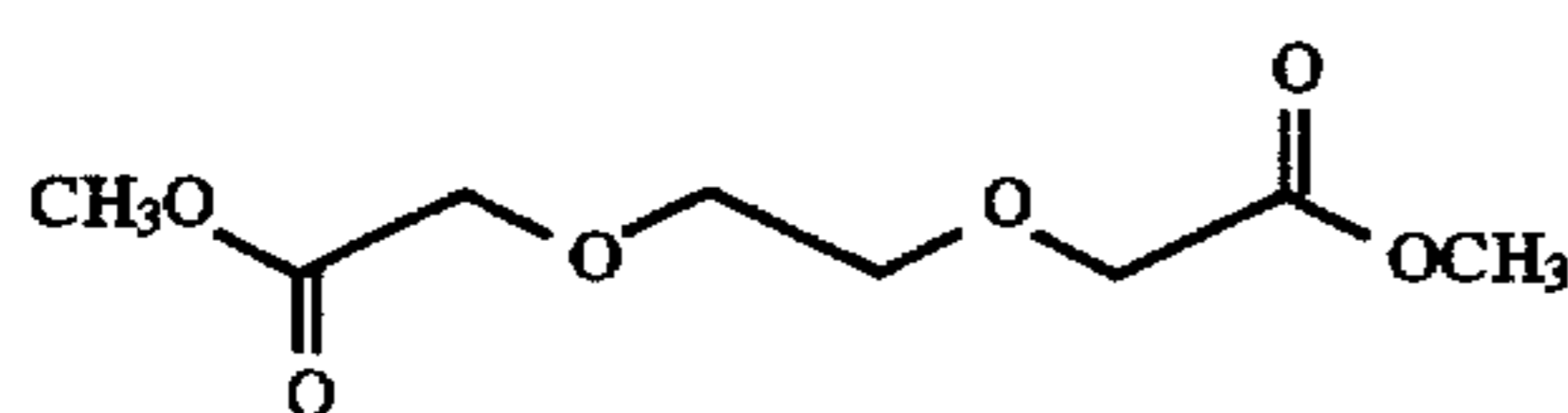
Dimethyl ester of 3,6-dioxaoctanedioic acid
