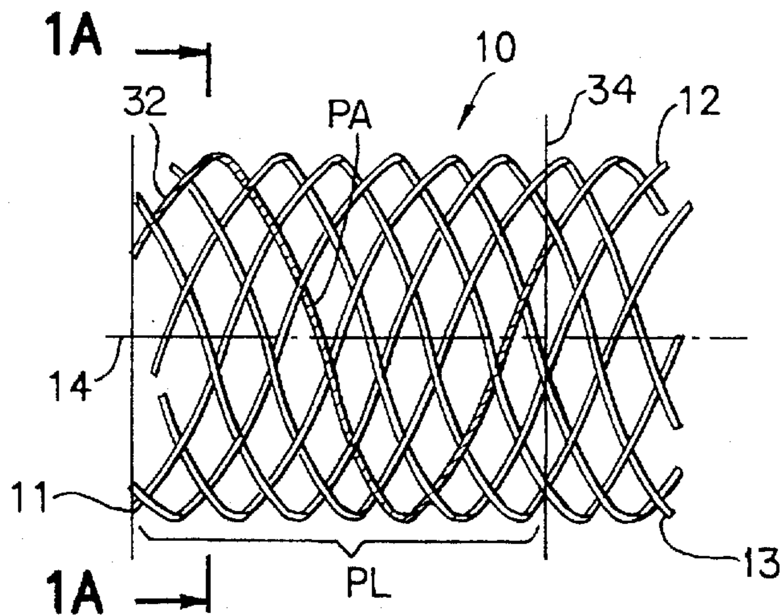
FIG. 1 PRIOR ART
