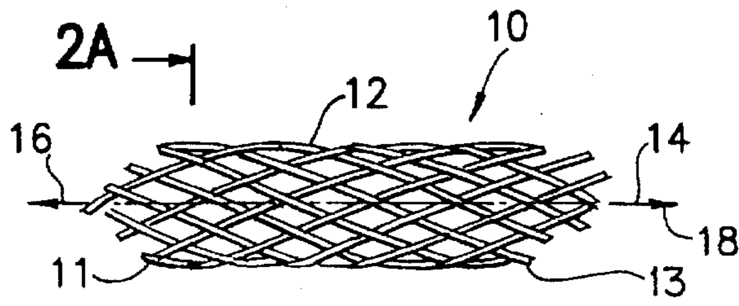
FIG. 2 PRIOR ART
