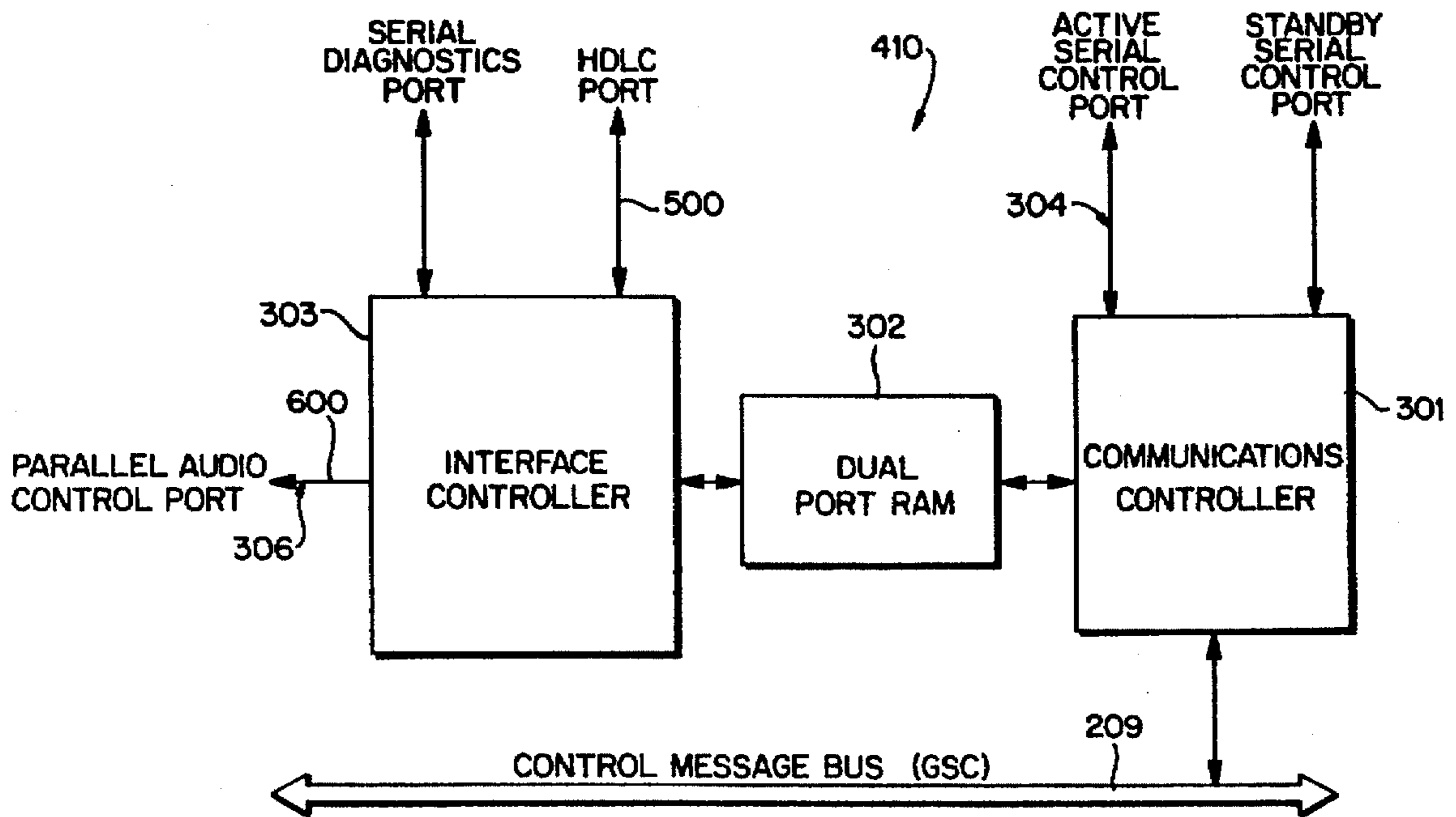
FIG. 4 SWITCH CONTROLLER CARD ARCHITECTURE
