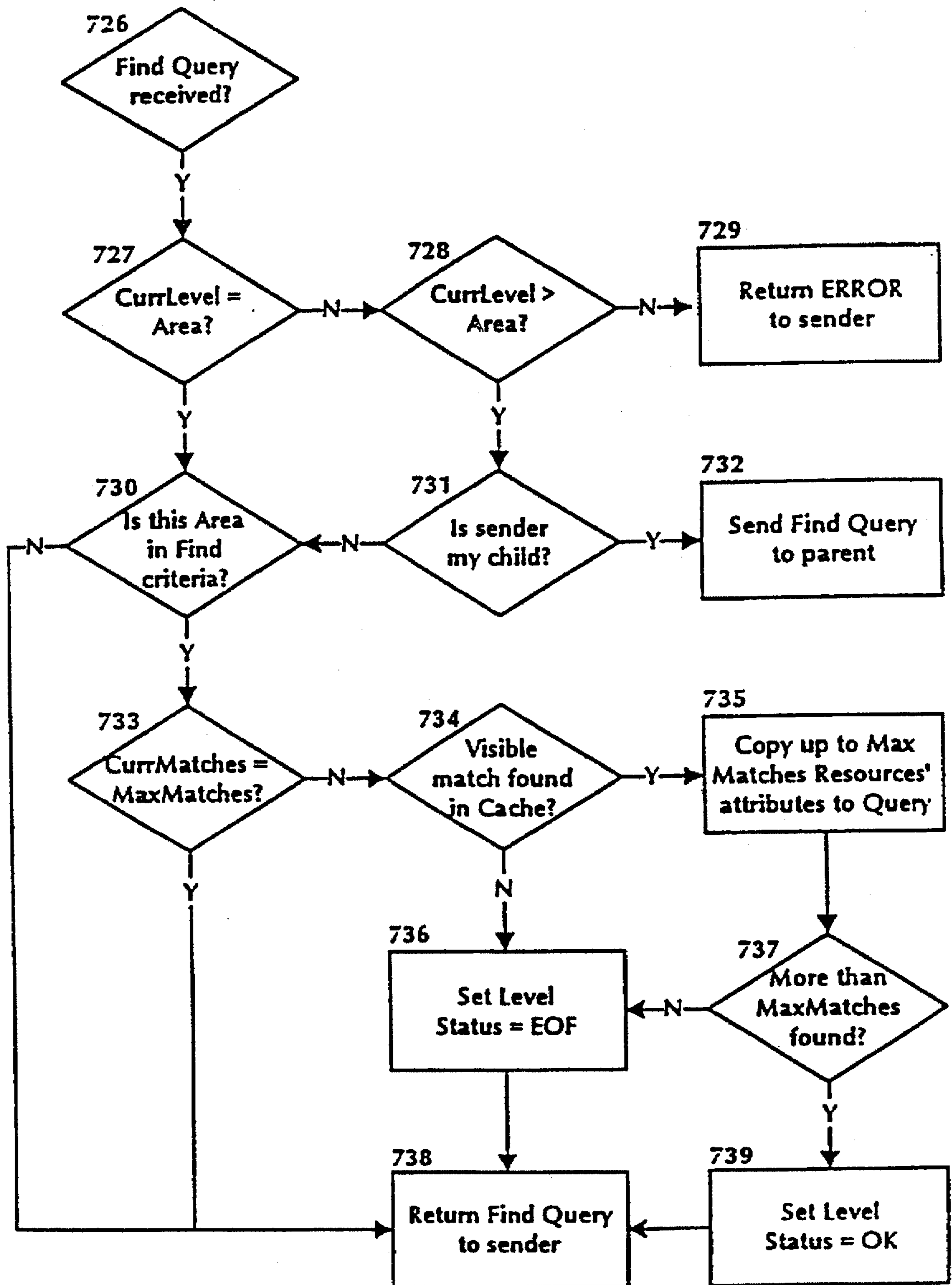
Find Query Process at Area Manager Node
