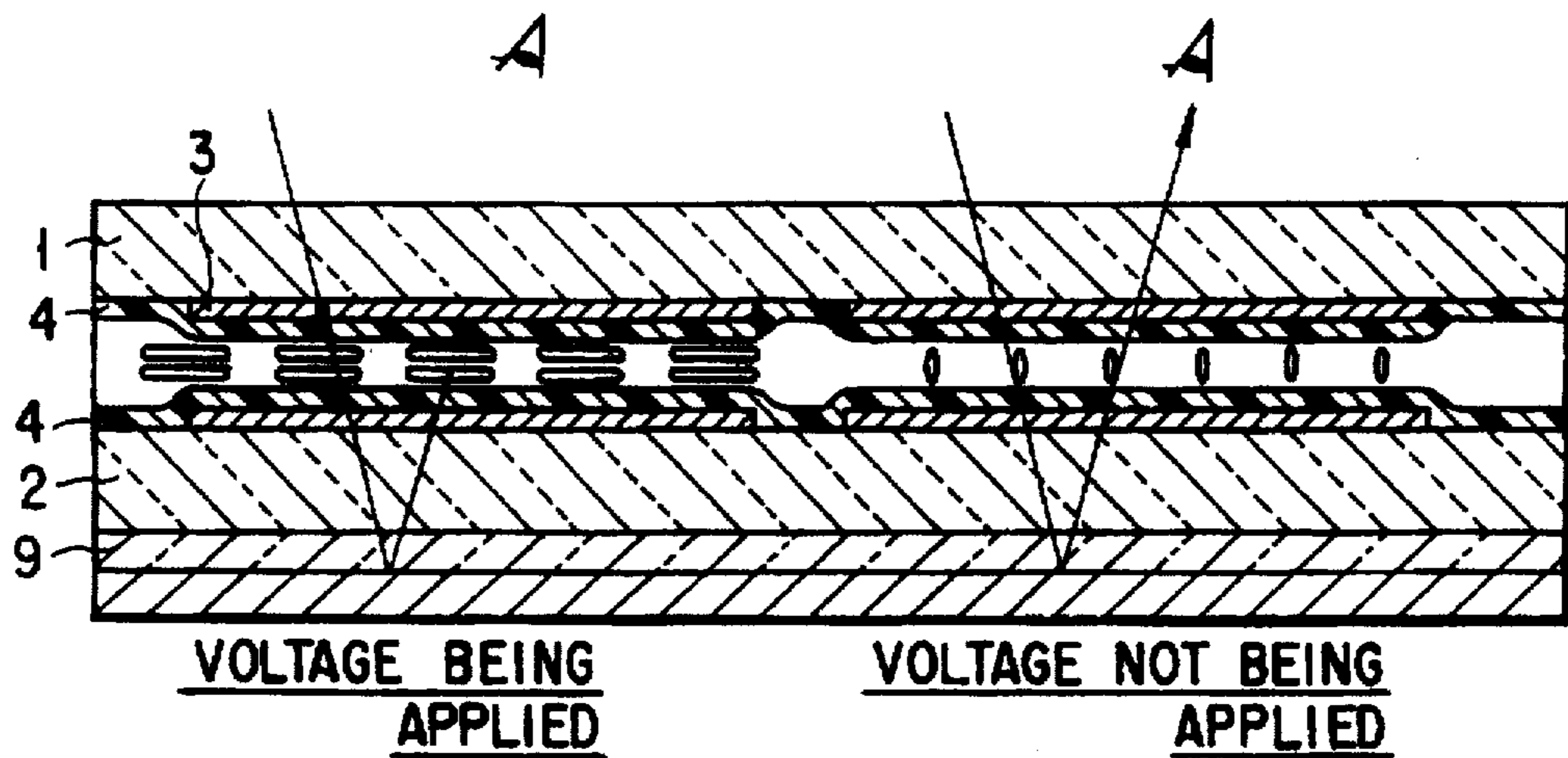
FIG. 6 PRIOR ART
