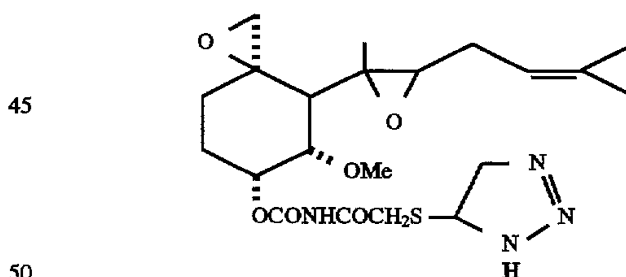
O-[(1,2,3-Triazol-5-yl)thioacetylcarbamoyl]fumagillol
