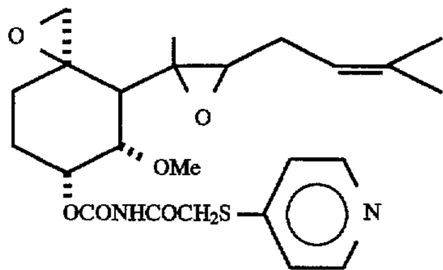
O-[(4-Pyridyl)thioacetylcarbamoyl]fumagillol
