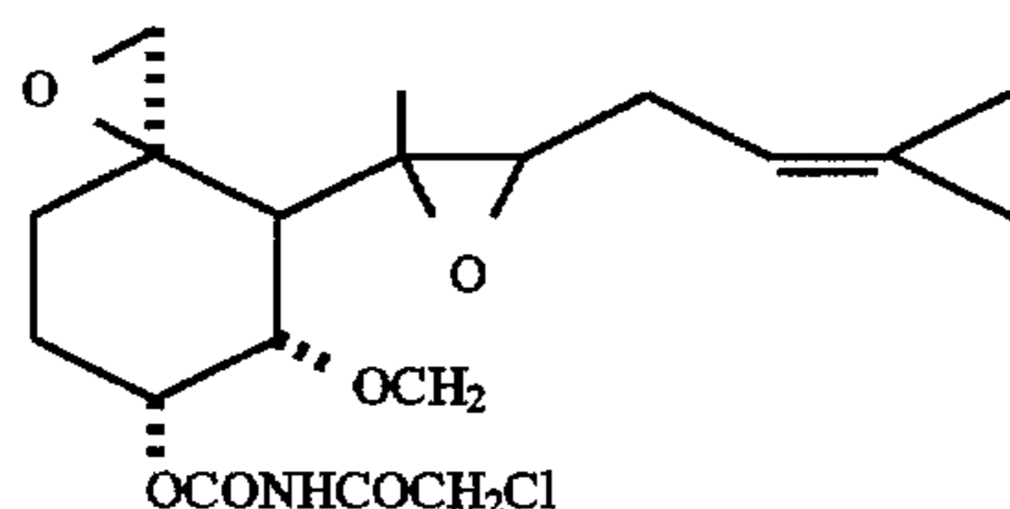
O-Chloroacetylcarbamoylfumagillol
