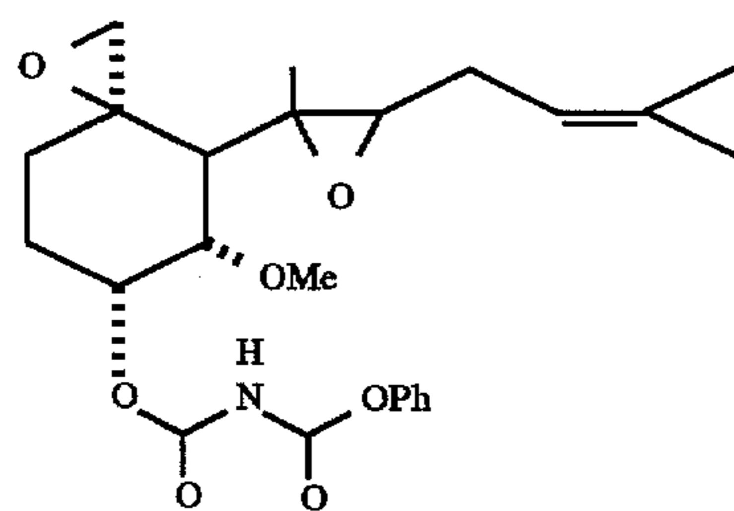
O-[N-(Phenoxycarbonyl)carbamoyl]fumagillol
