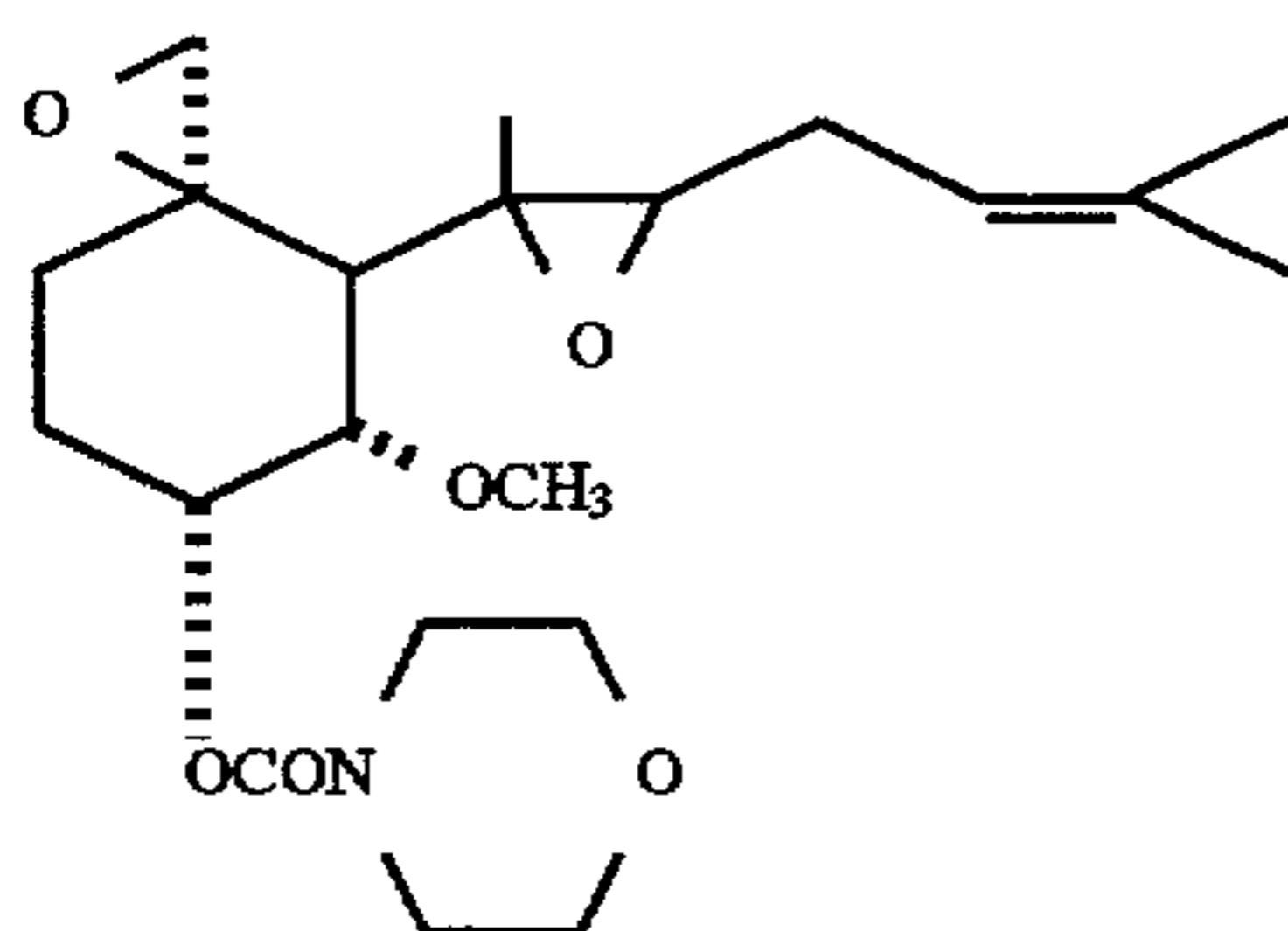
O-Morpholinocarbonylfumagillol
