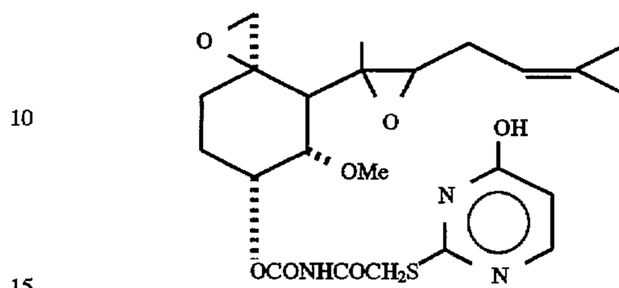
O-[(4-Hydroxypyrimidin-2-yl)thioacetylcarbamoyl]fumagillol
