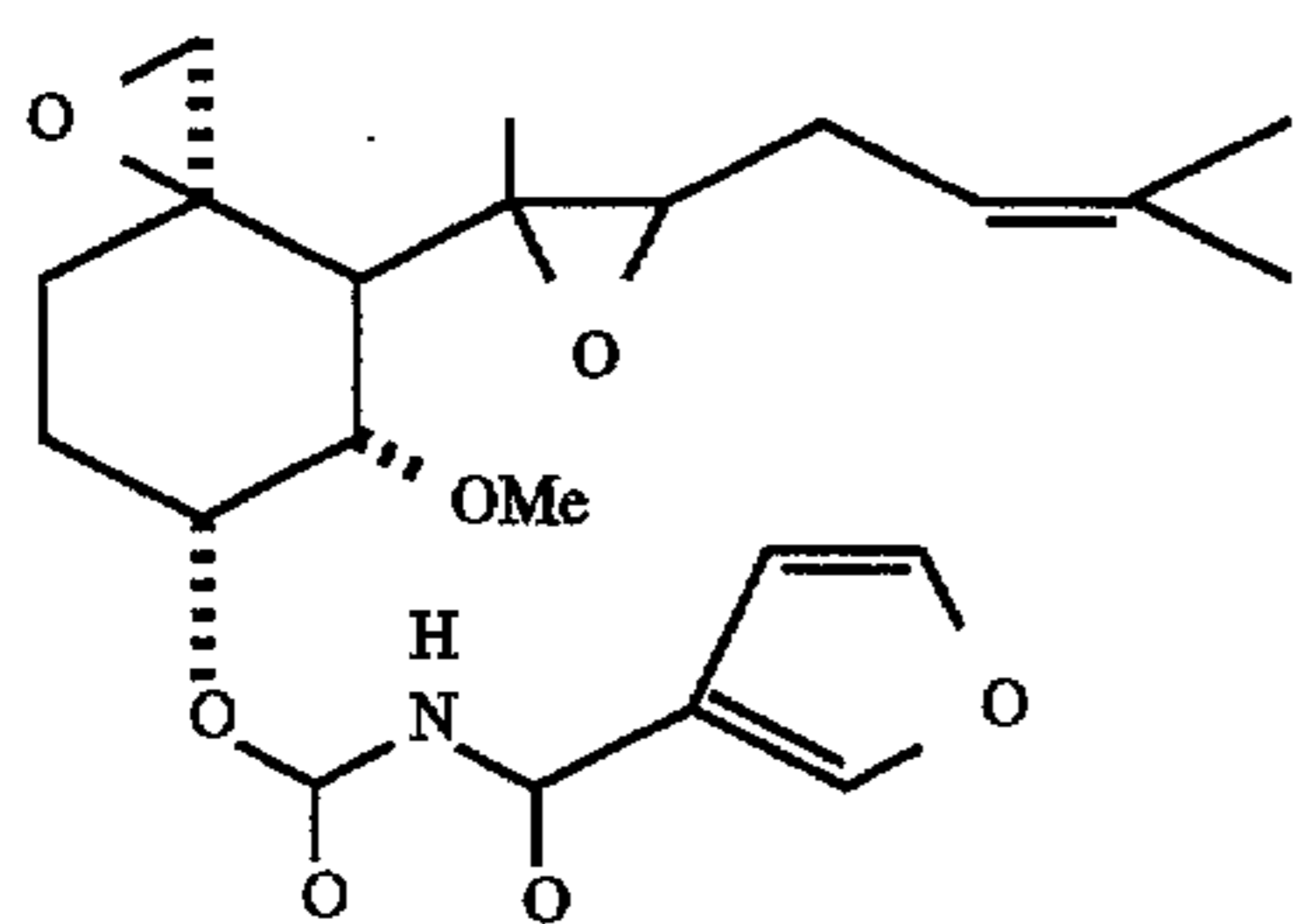
O-[N-(3-Furoyl)carbamoyl]fumagillol
