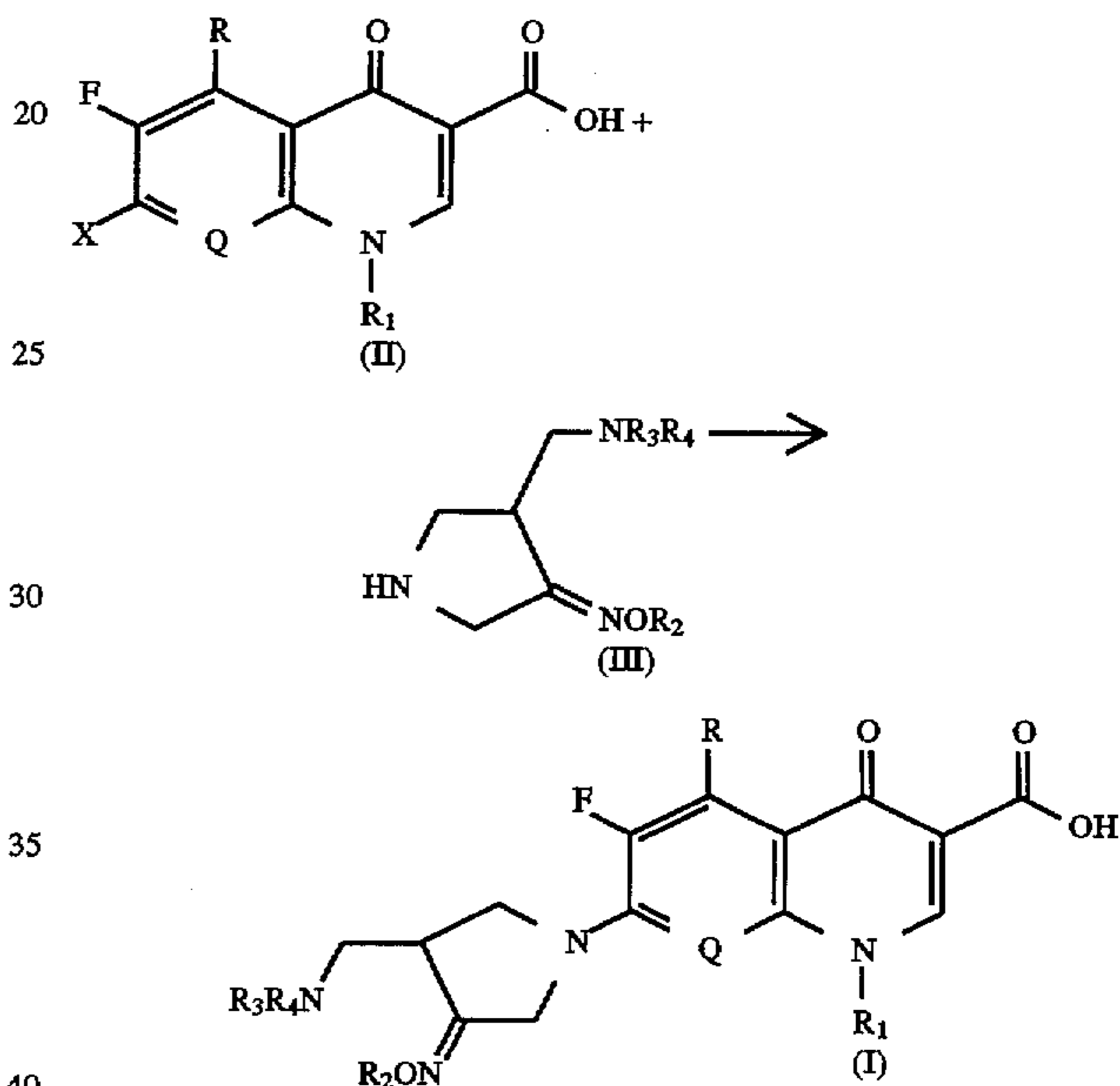
Reaction Scheme 1
