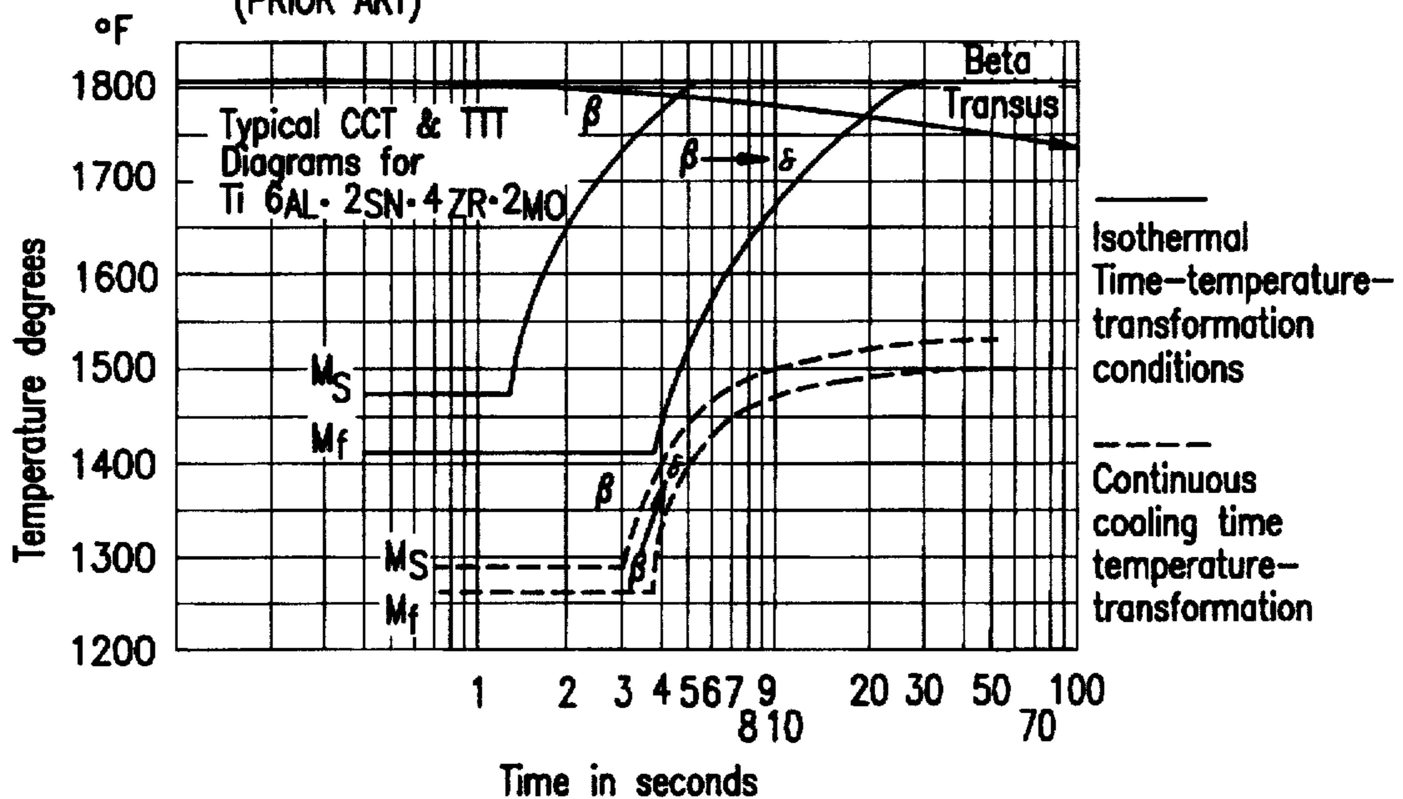
FIG. 3 (PRIOR ART)
