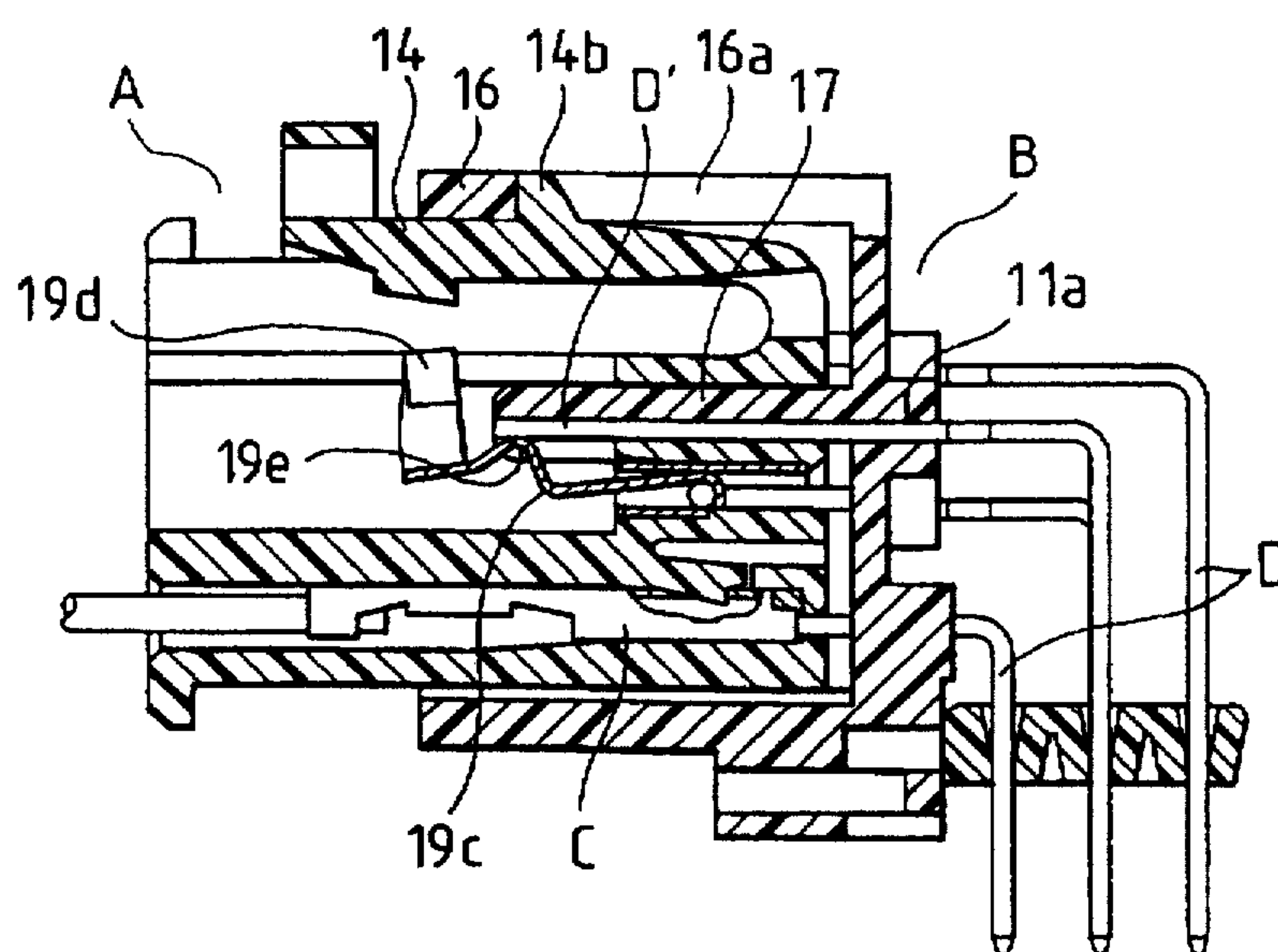
FIG. 6 PRIOR ART
