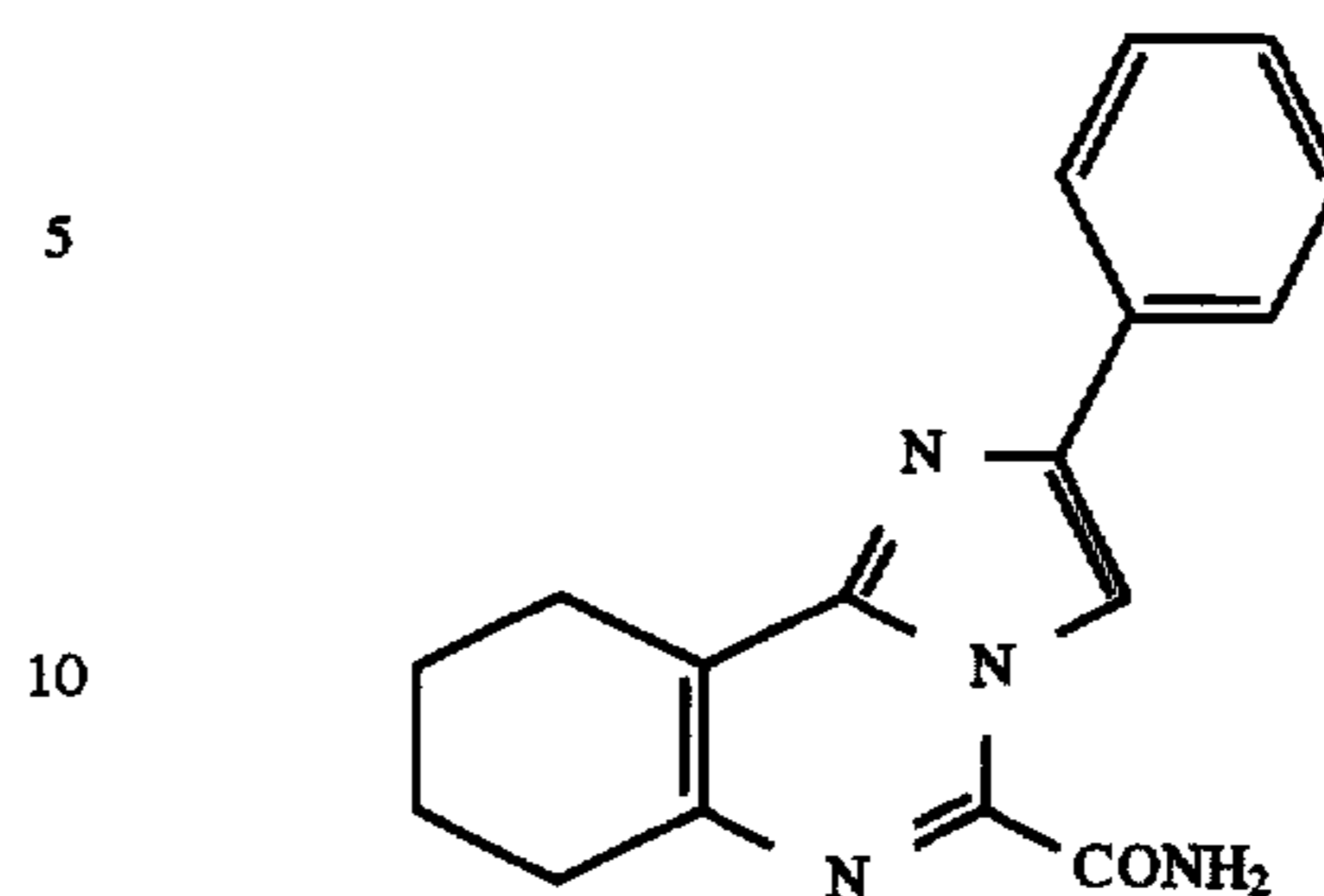
Compound 42
