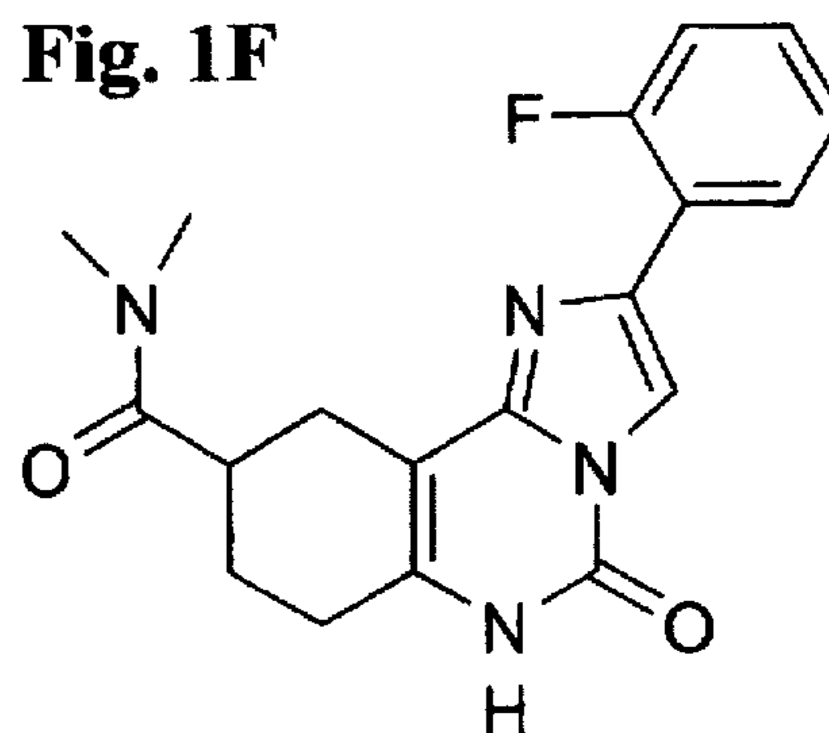
Compound 18
