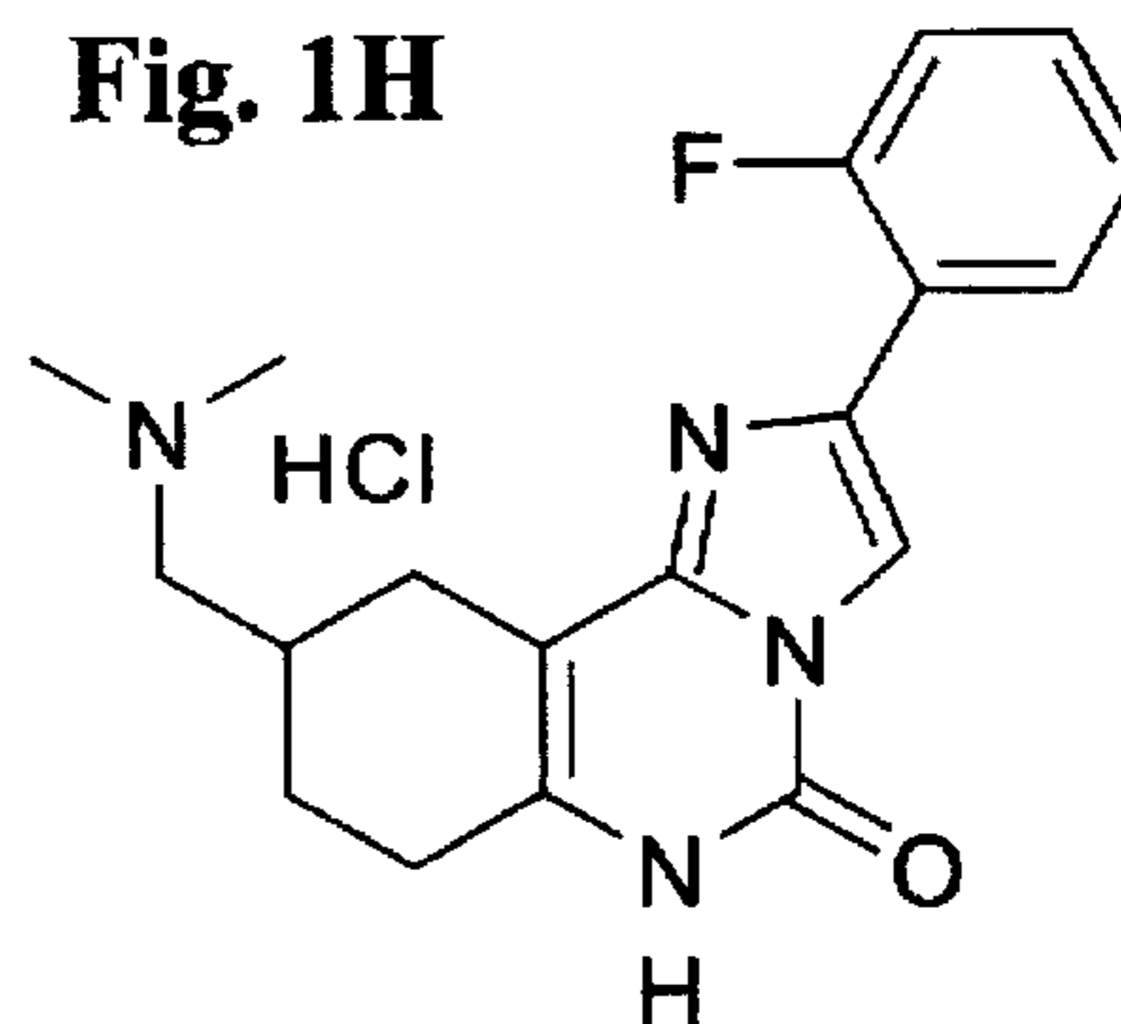
Compound 24
