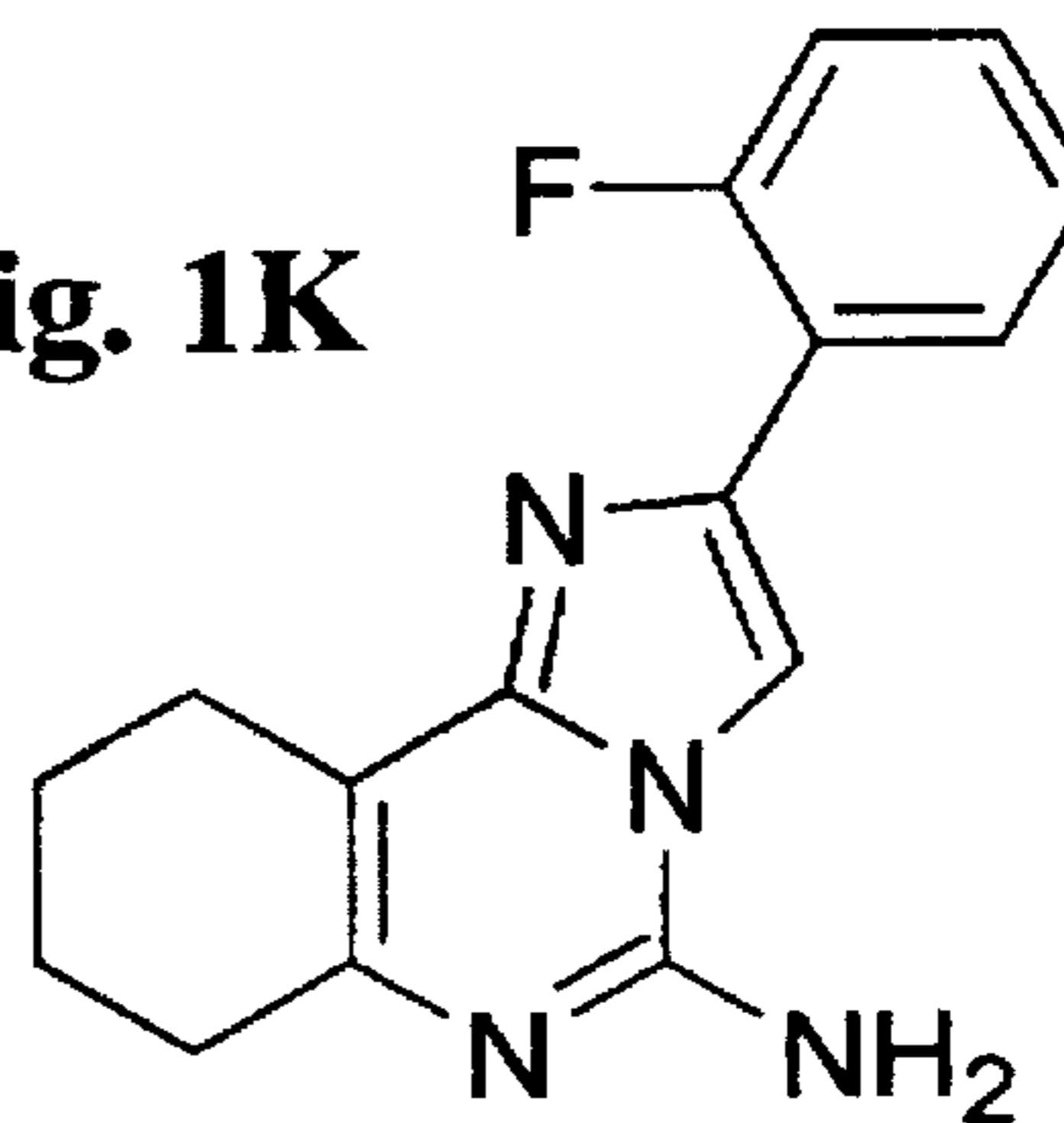
Compound 33
