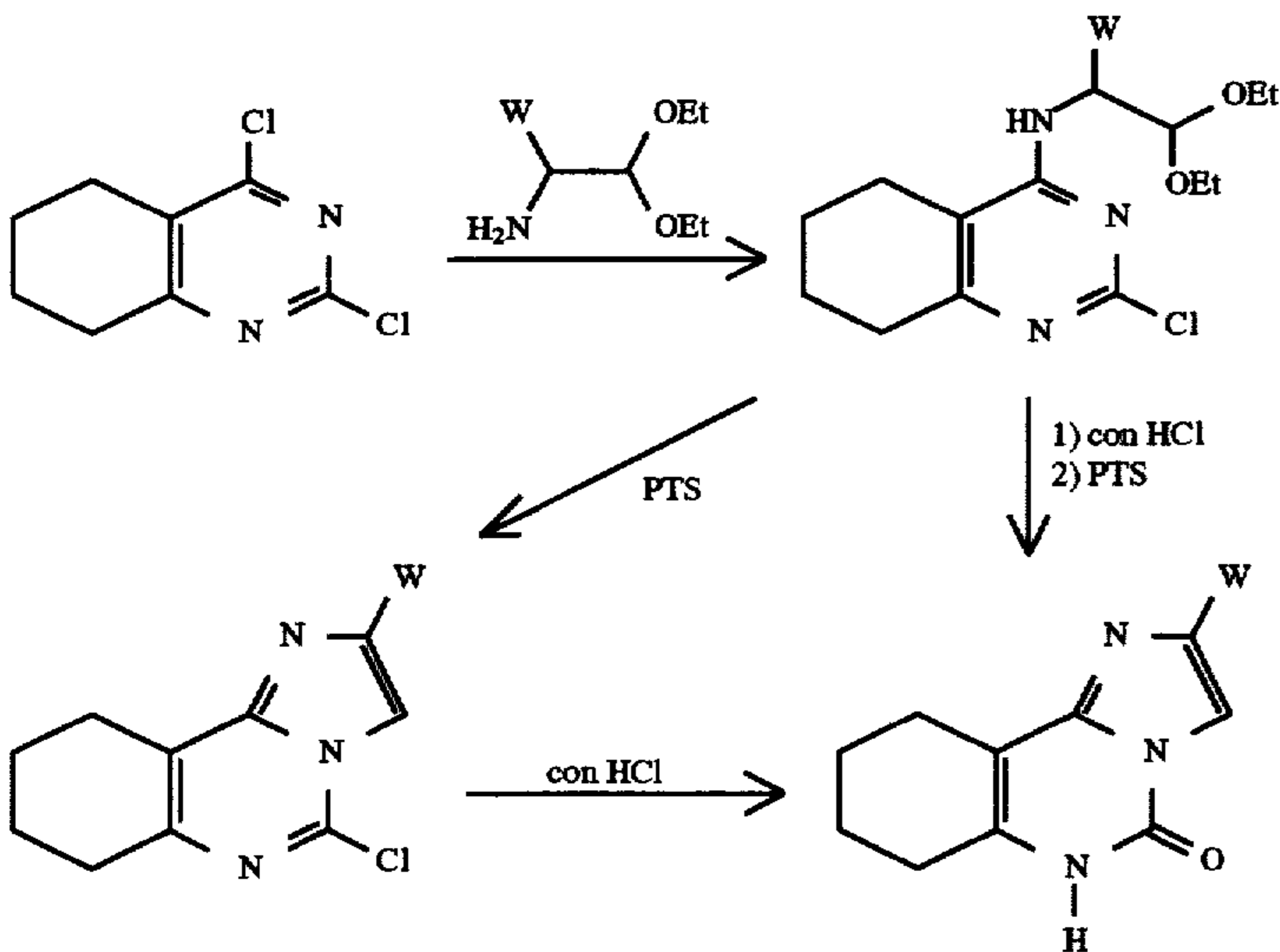
Scheme II
