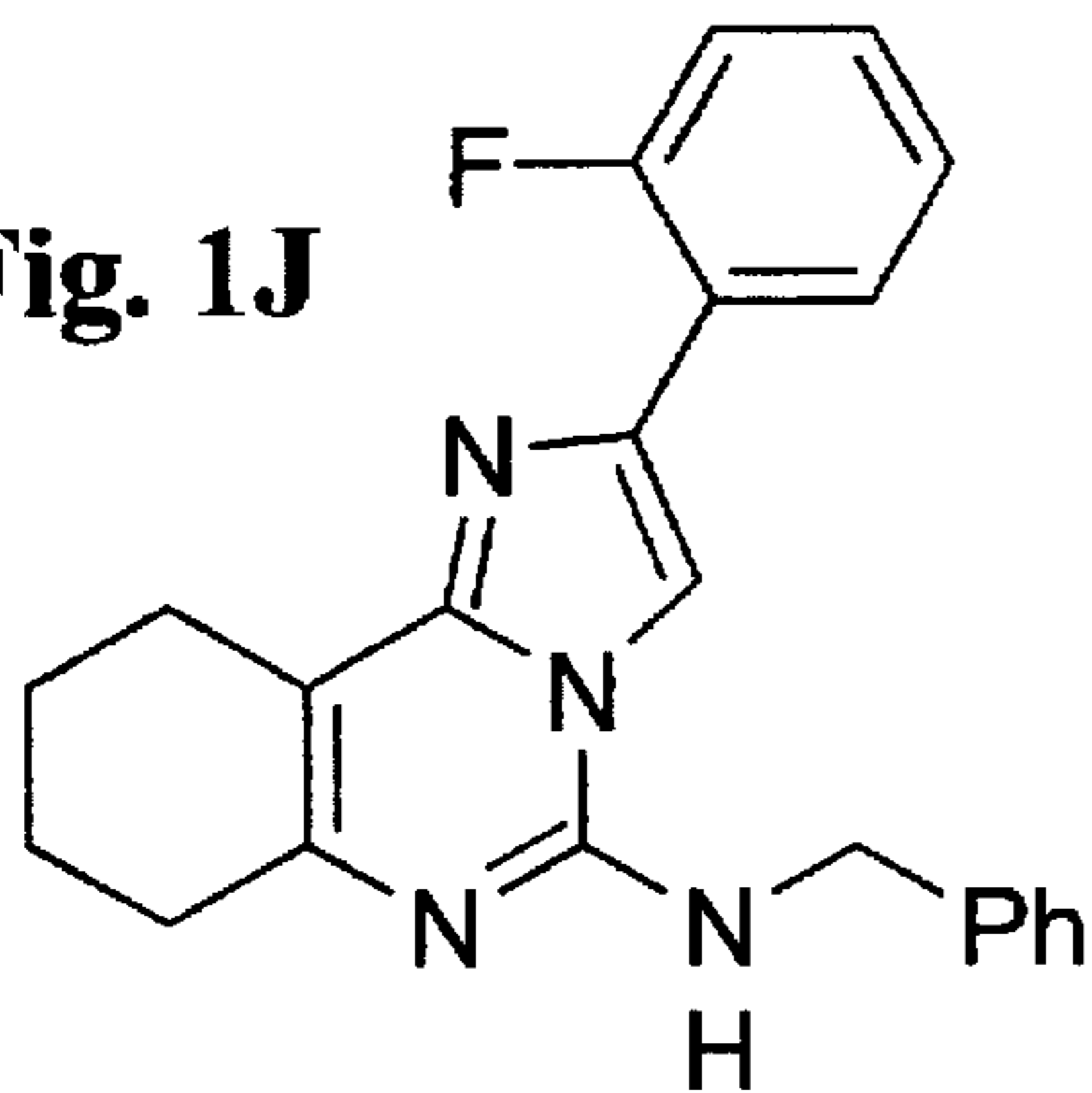
Compound 31
