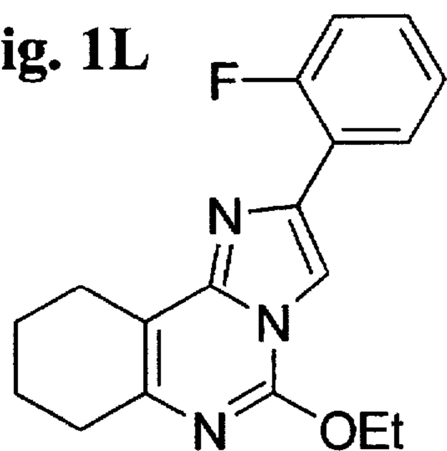
Compound 39
