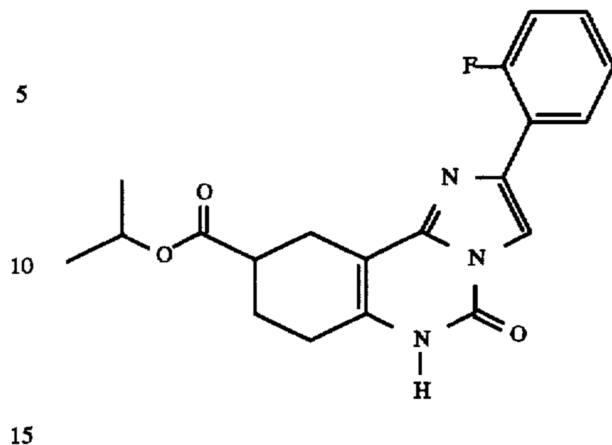
Compound 1
