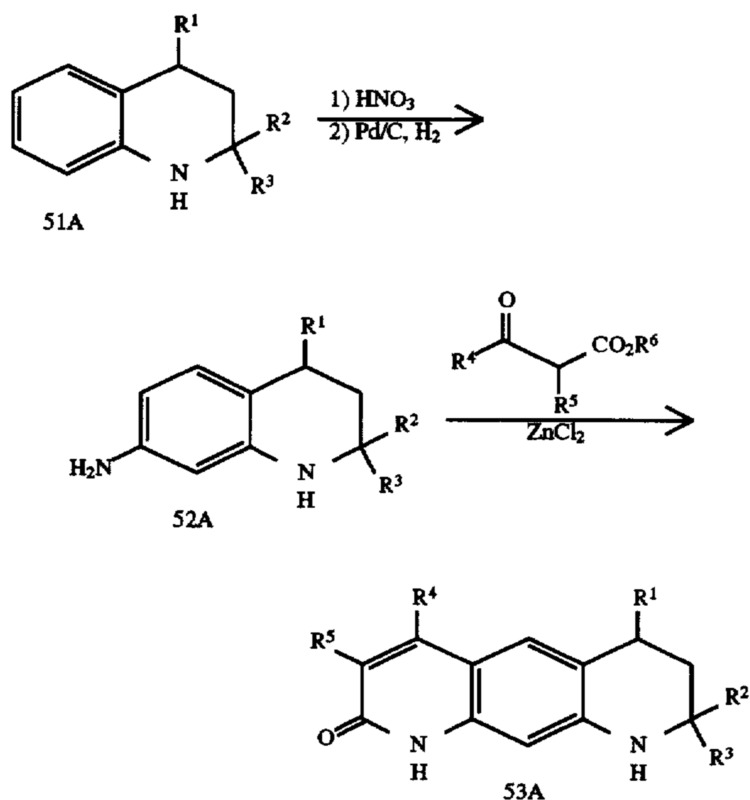
Scheme XLVI
