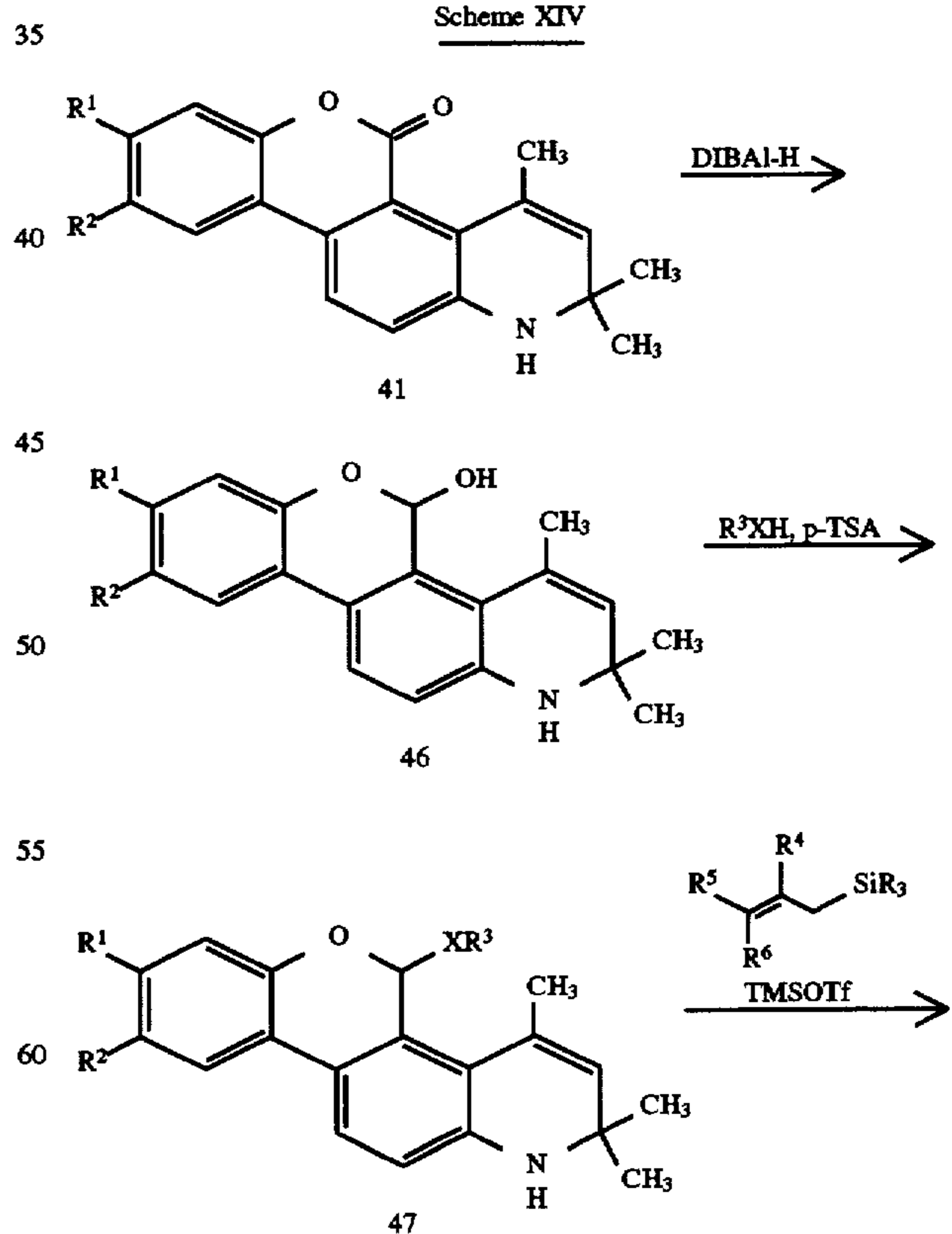
Scheme XIV
