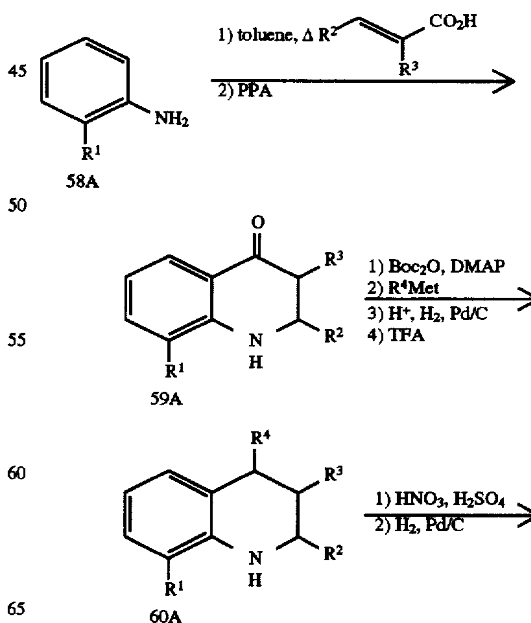
Scheme XLVII
