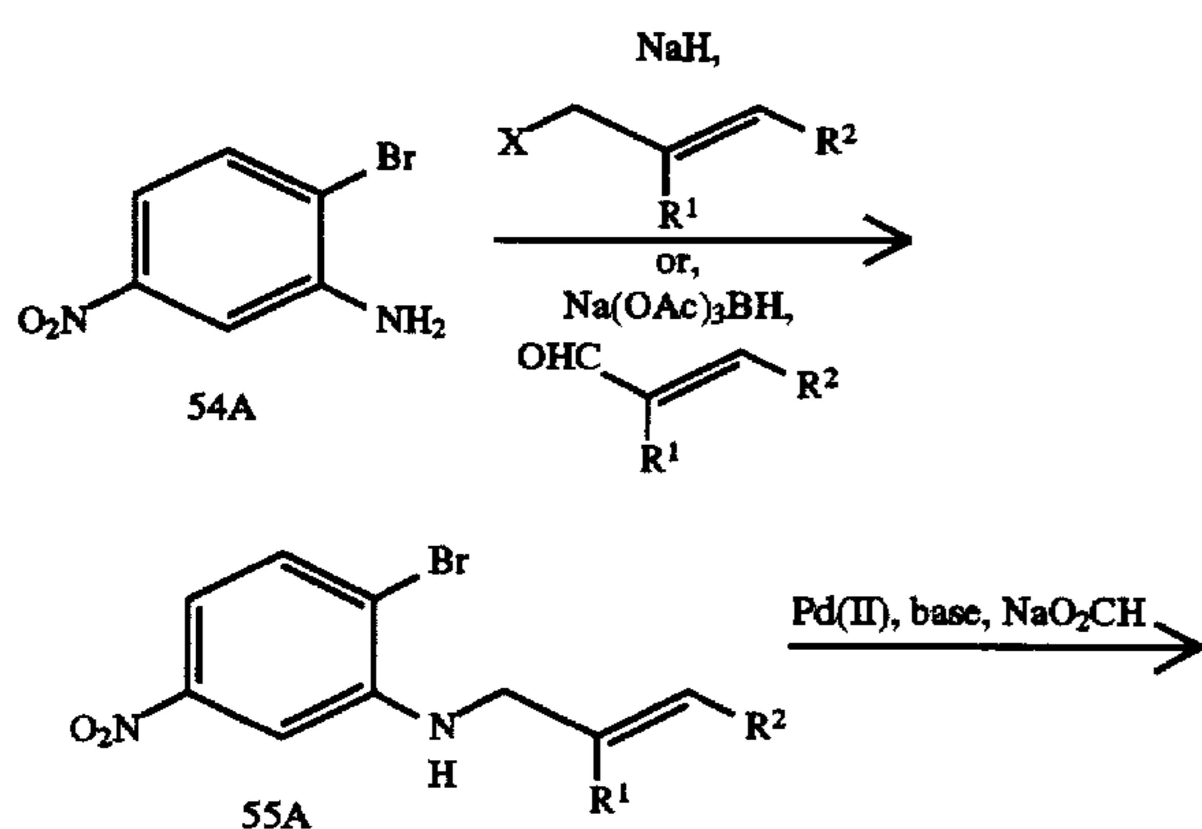
Scheme XLVII
