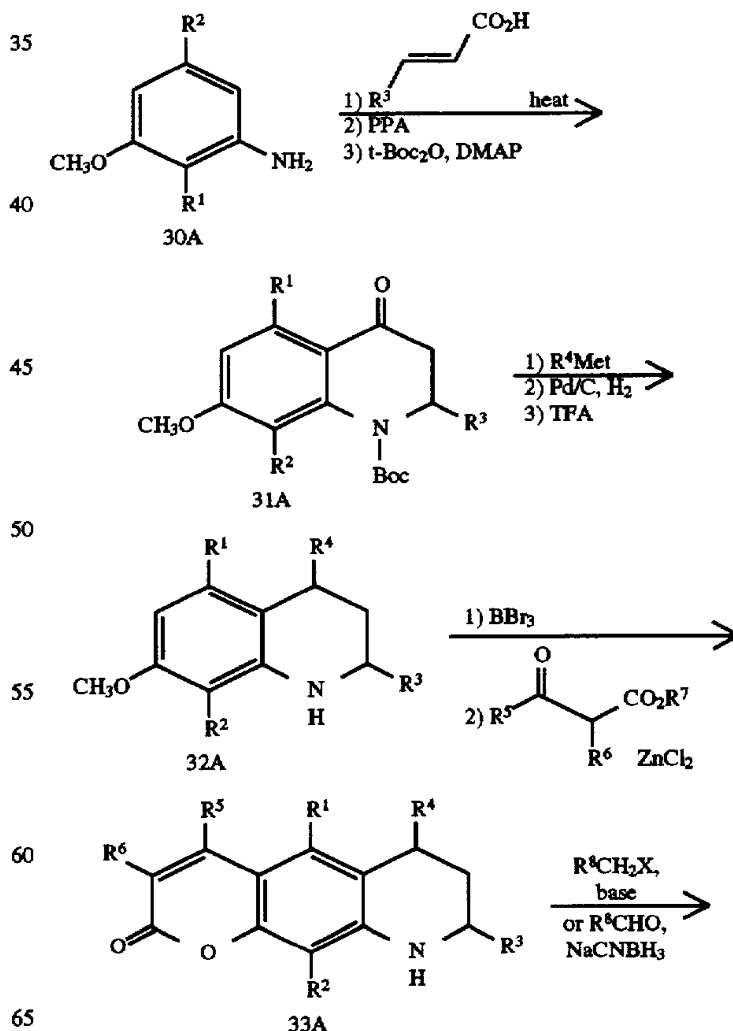
Scheme XL
