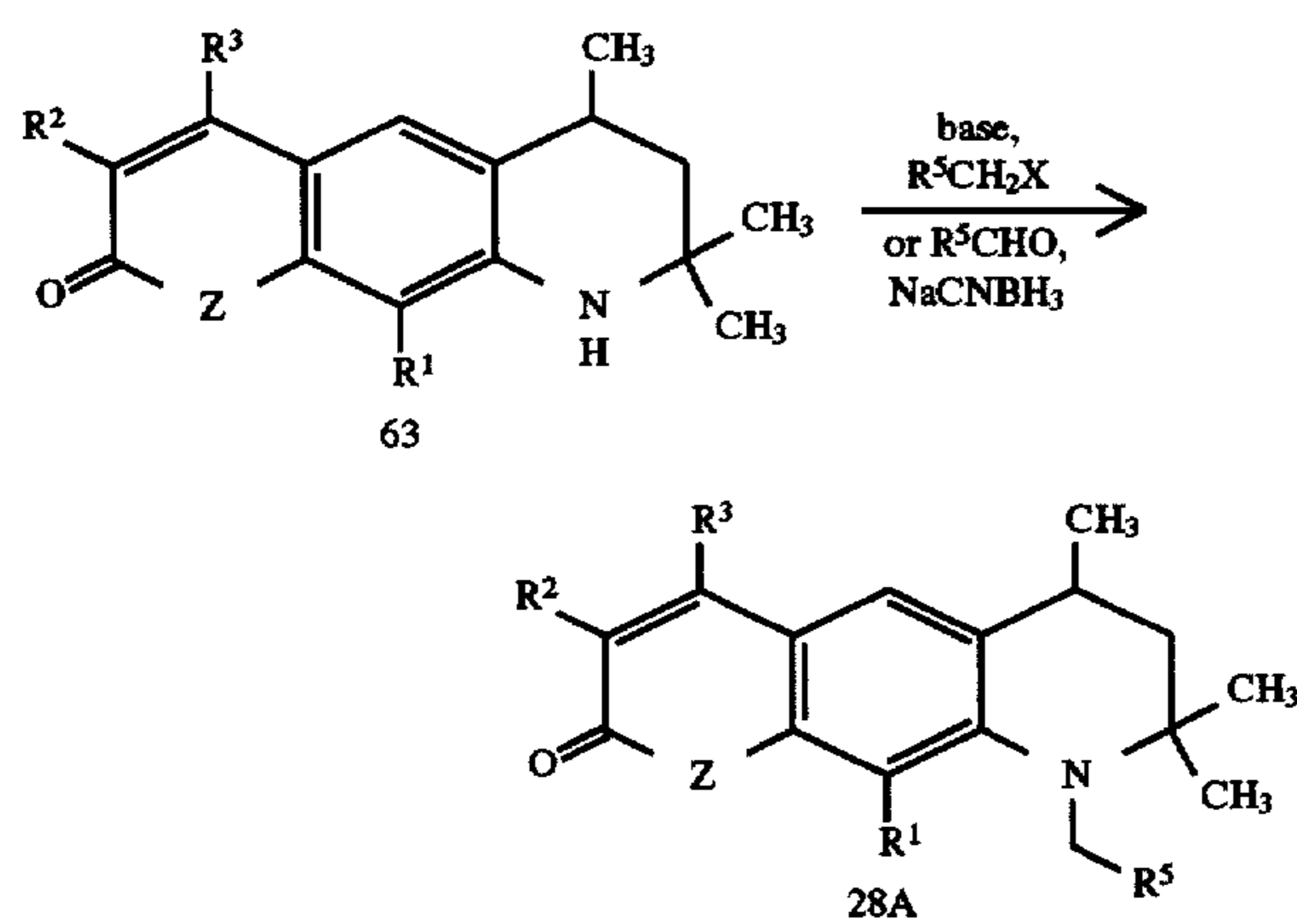
Scheme XXXVIII
