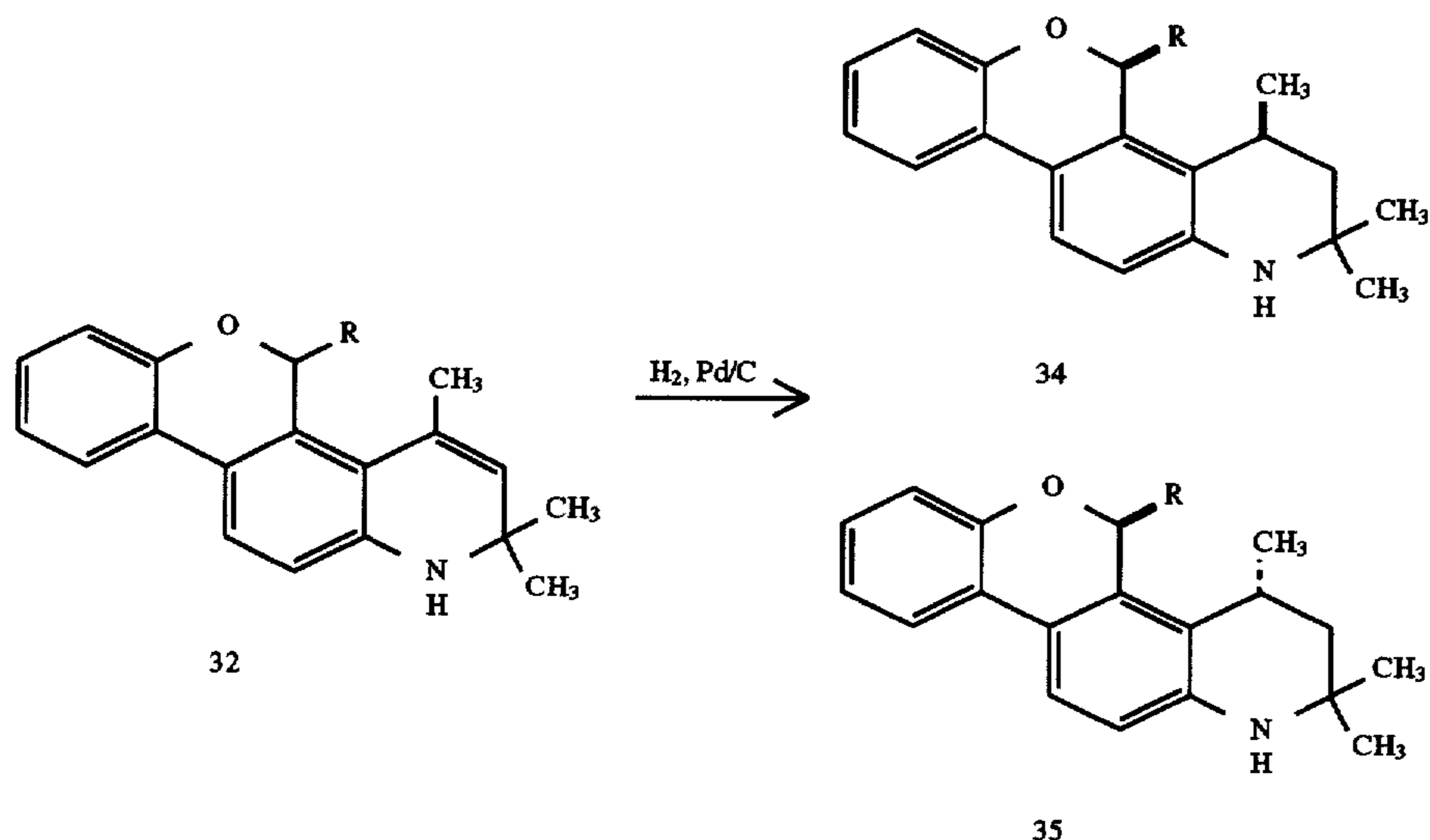
Scheme X
