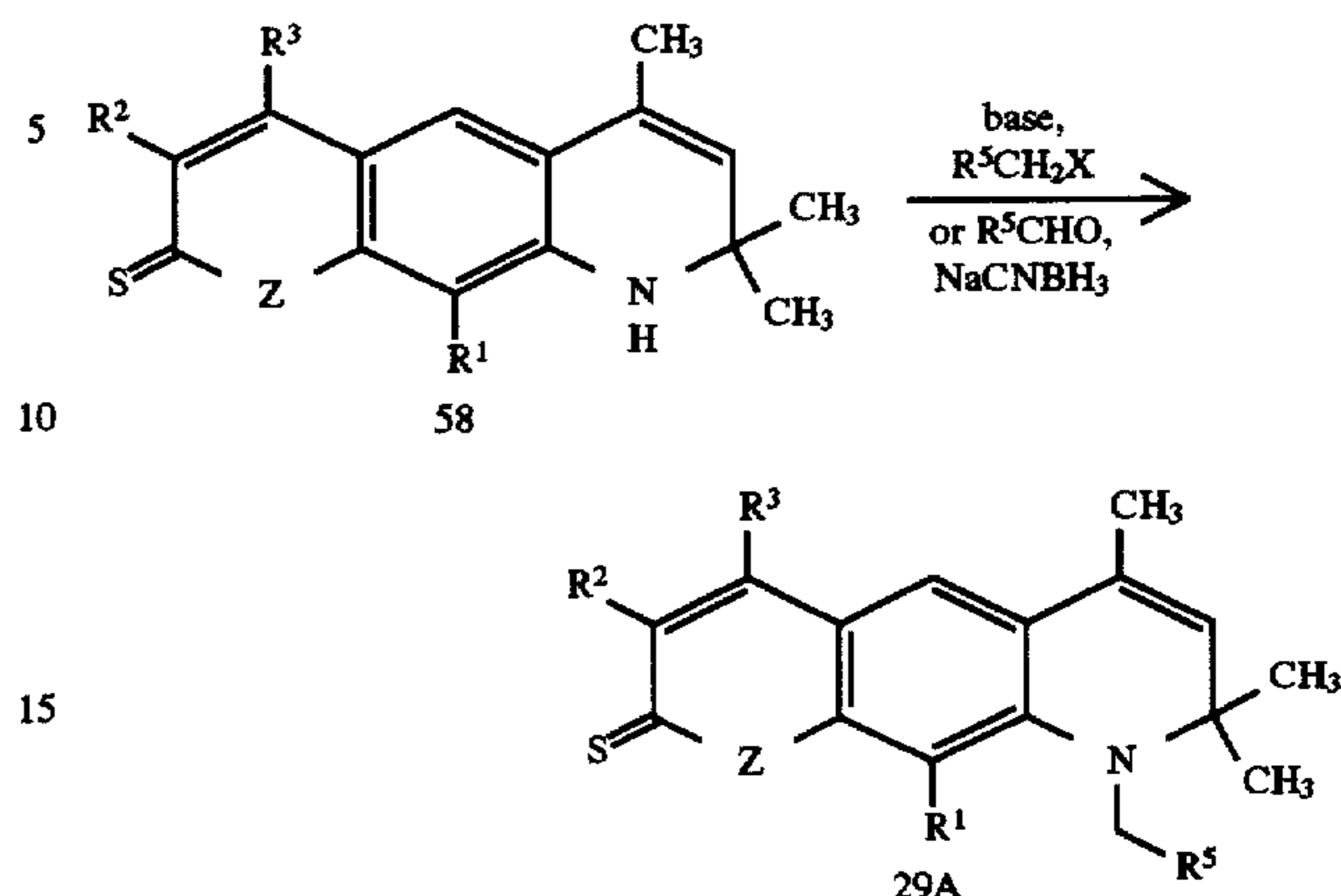
Scheme XXXIX
