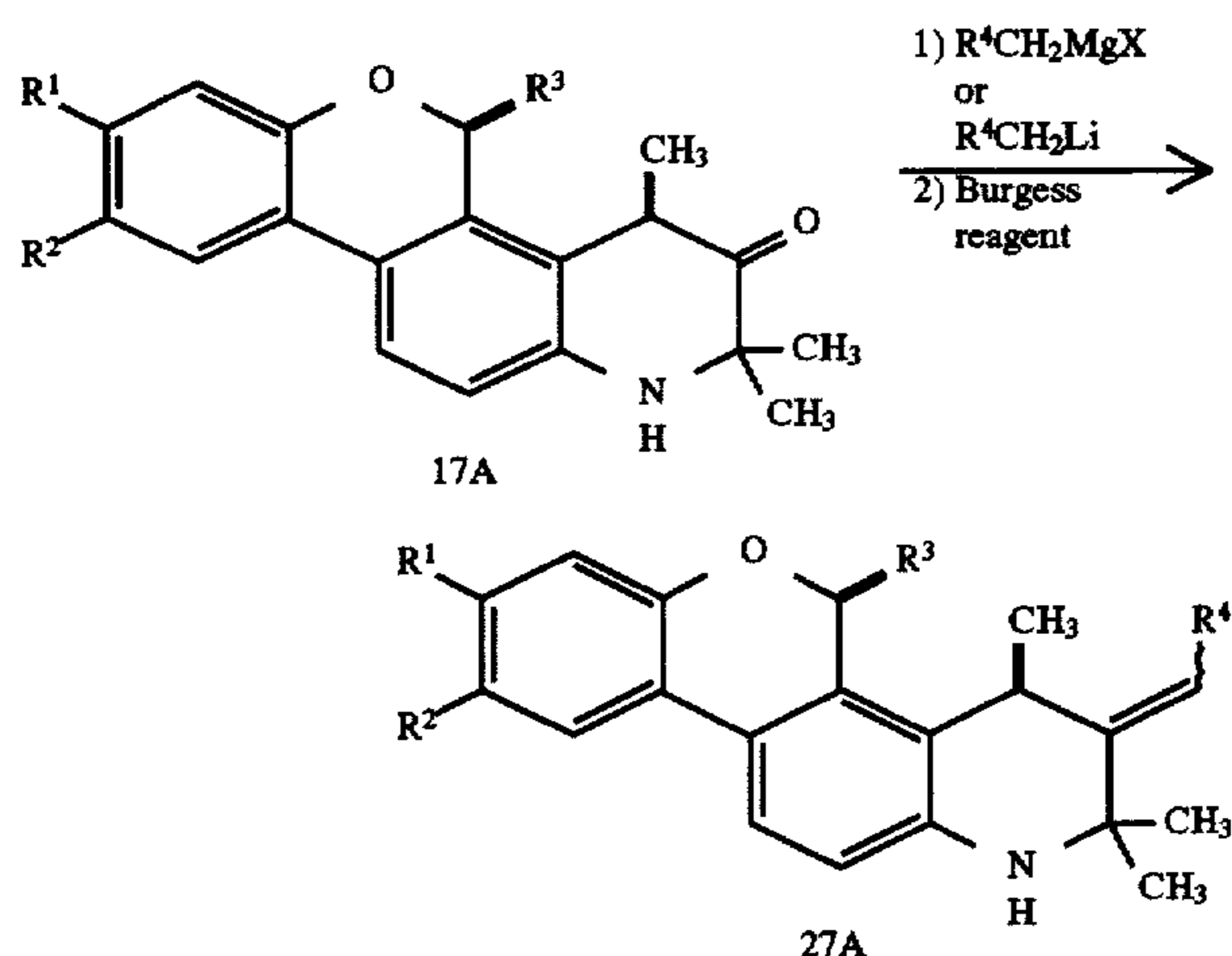
Scheme XXXVII
