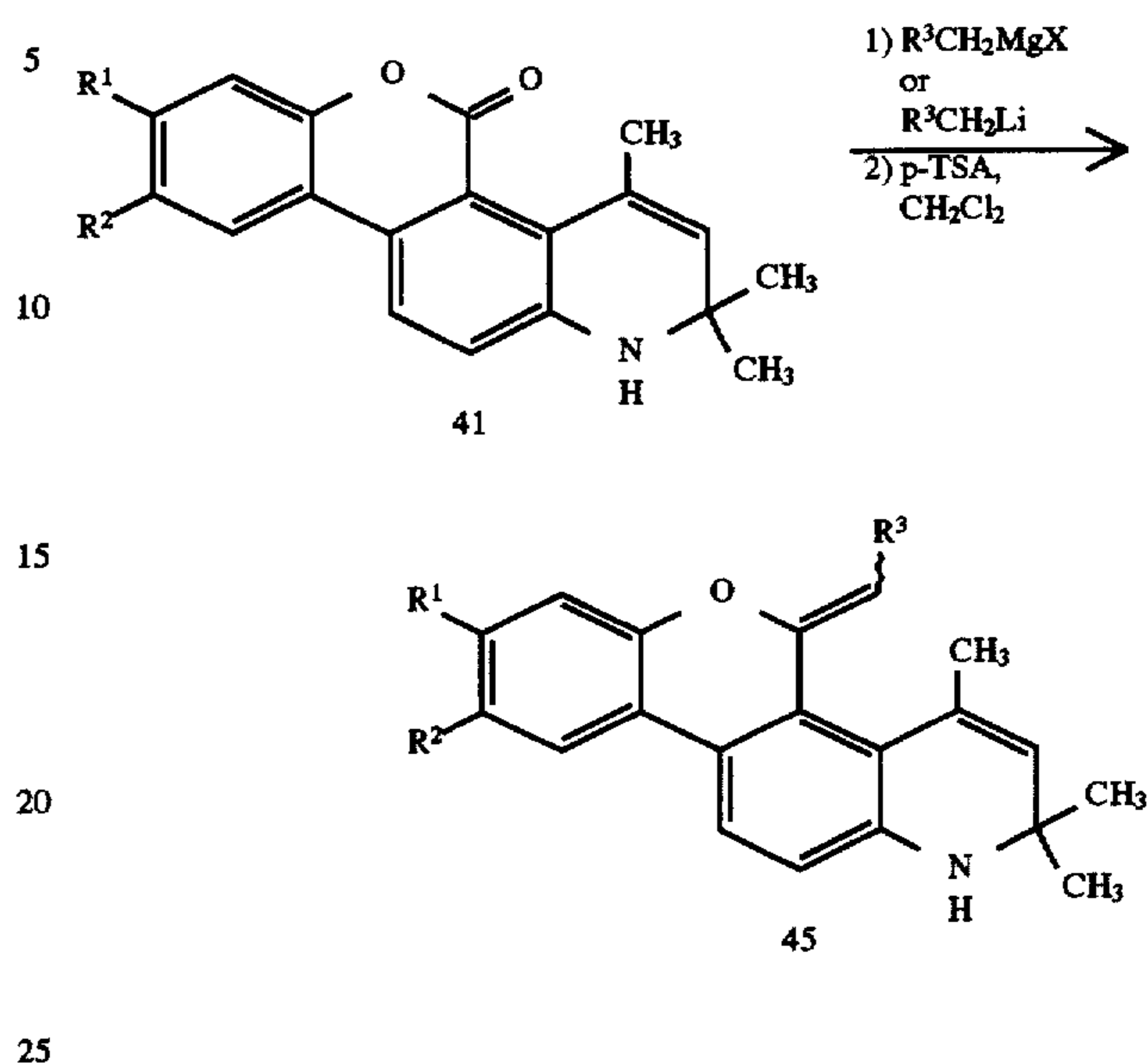
Scheme XIII
