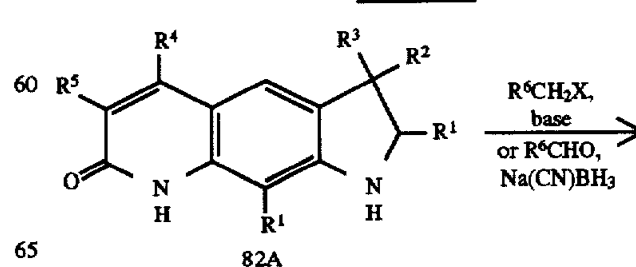
Scheme LV
