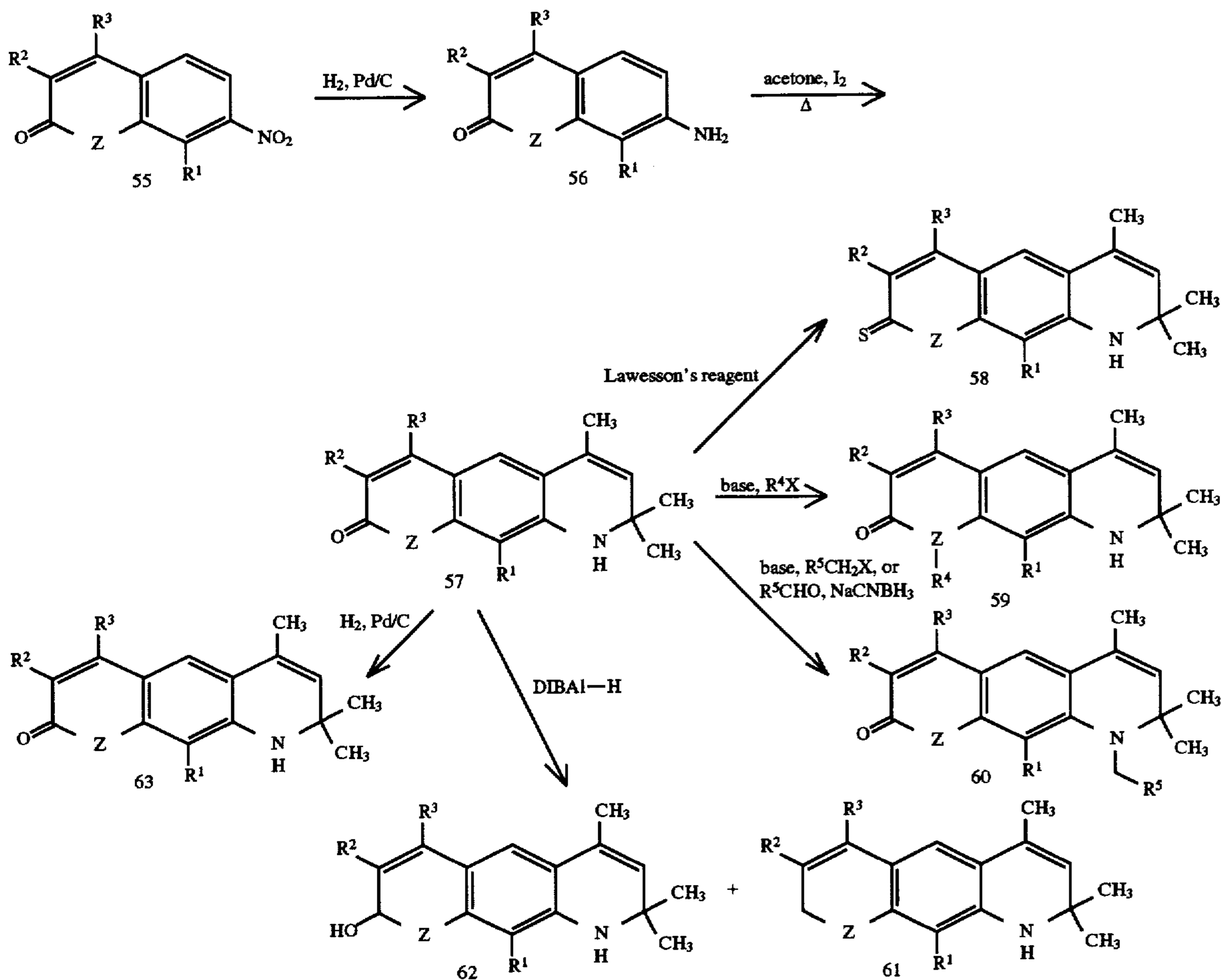
Scheme XVI
