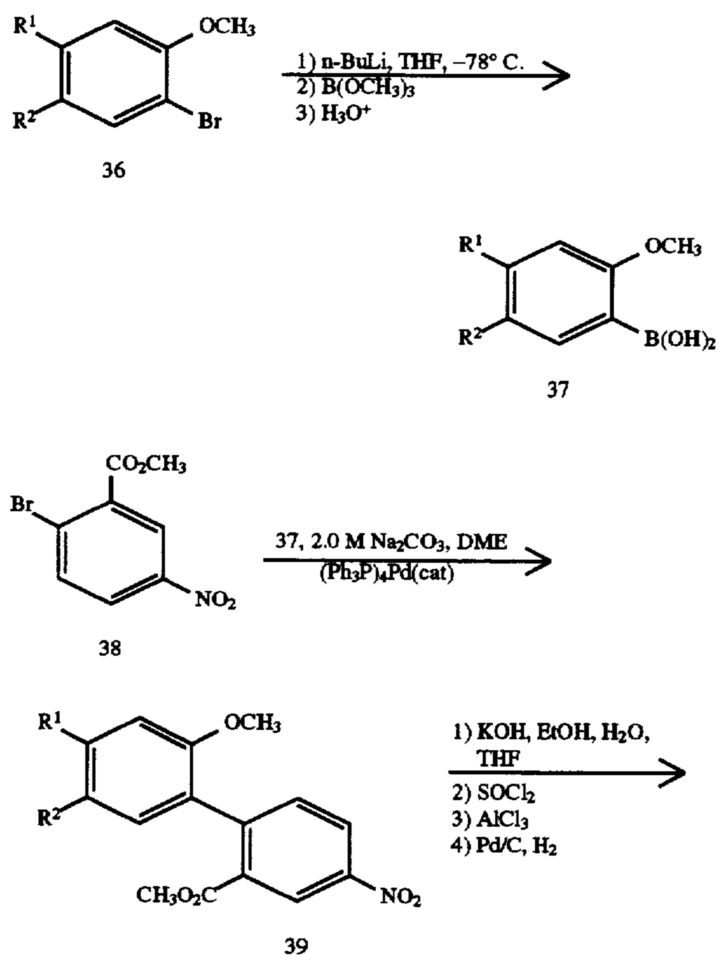
Scheme XI
