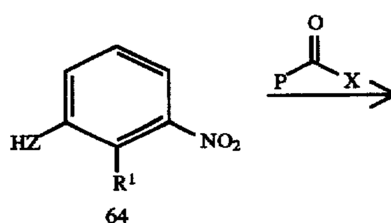
Scheme XVII
