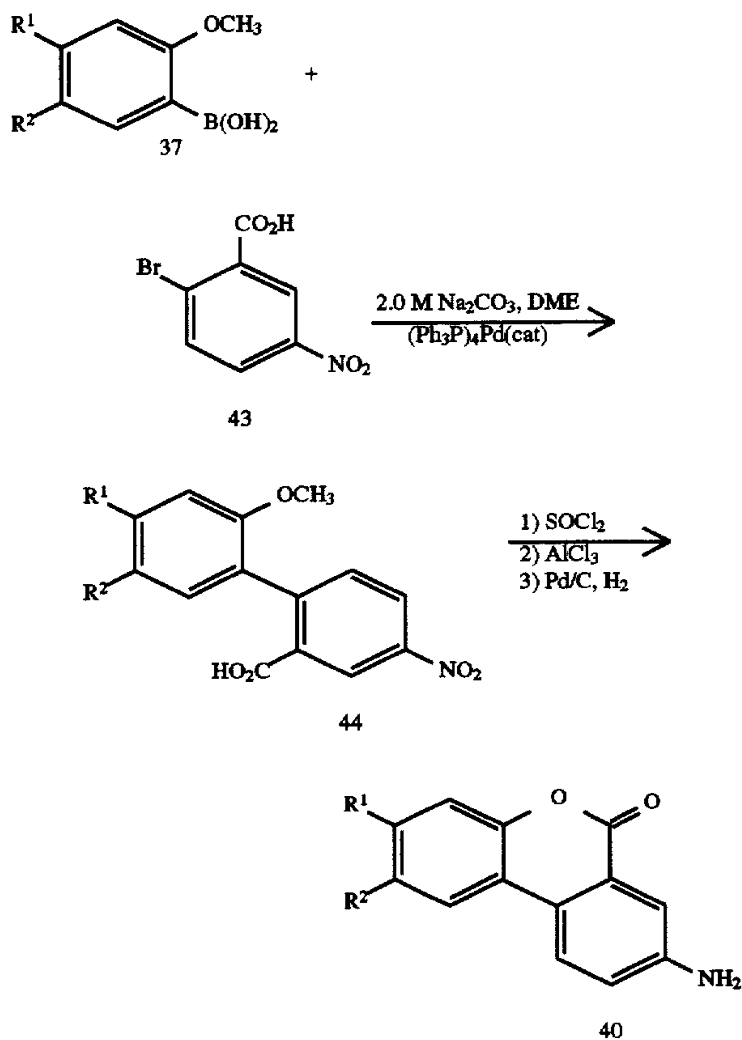
Scheme XII
