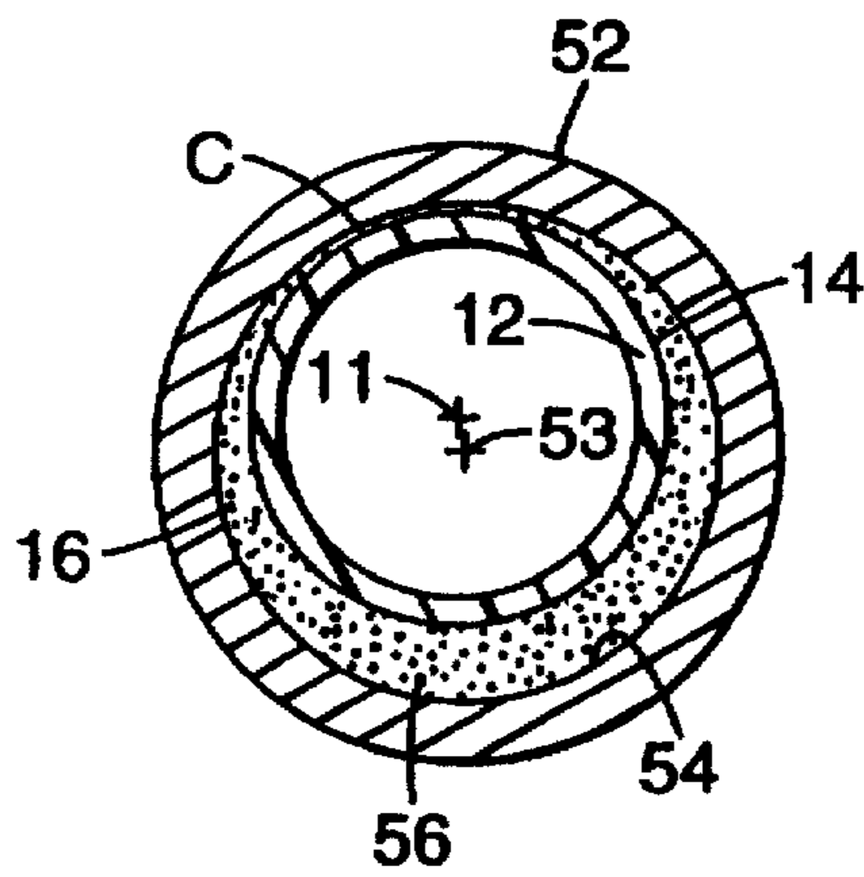
Fig. 3 PRIOR ART
