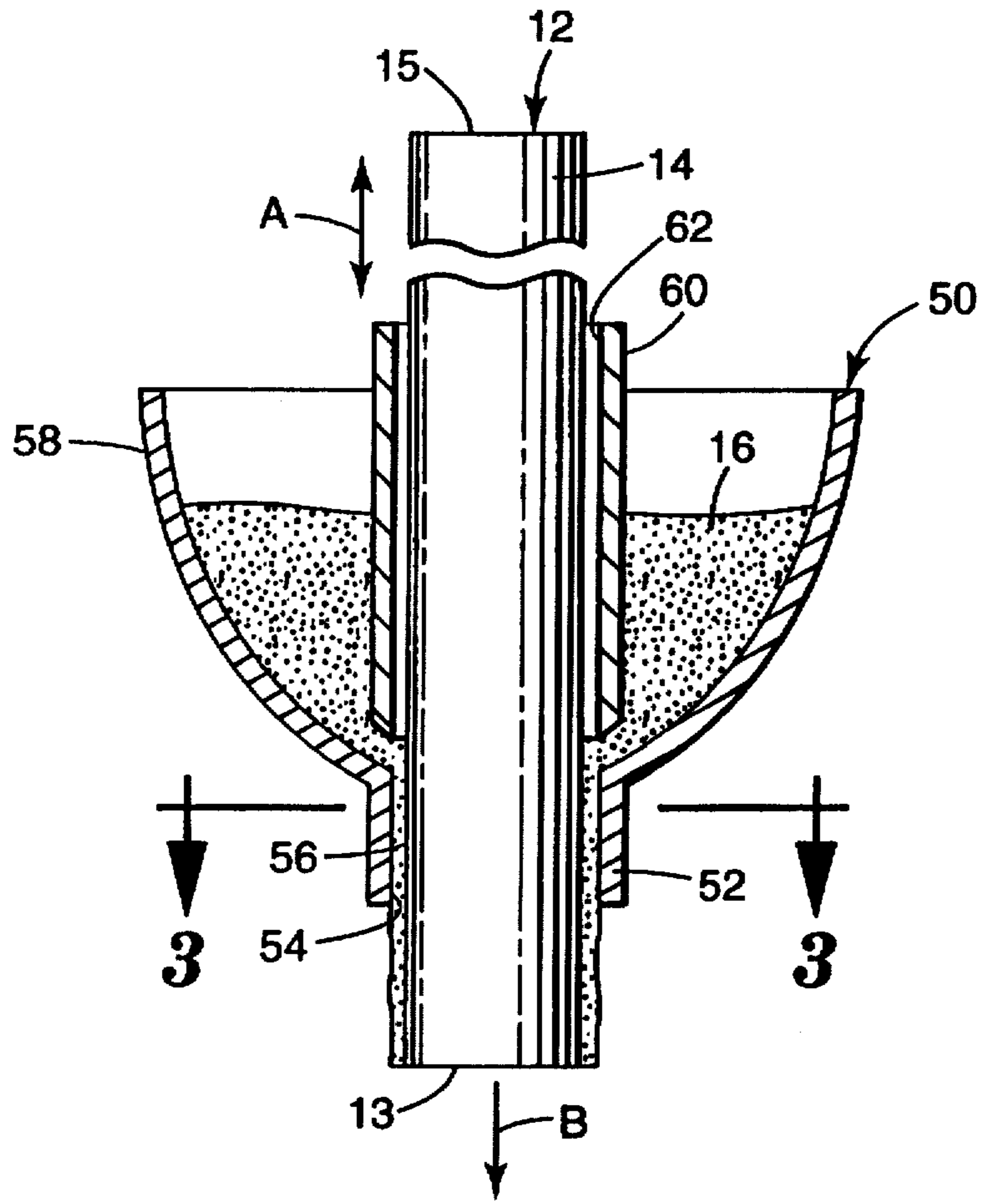
Fig. 2 PRIOR ART
