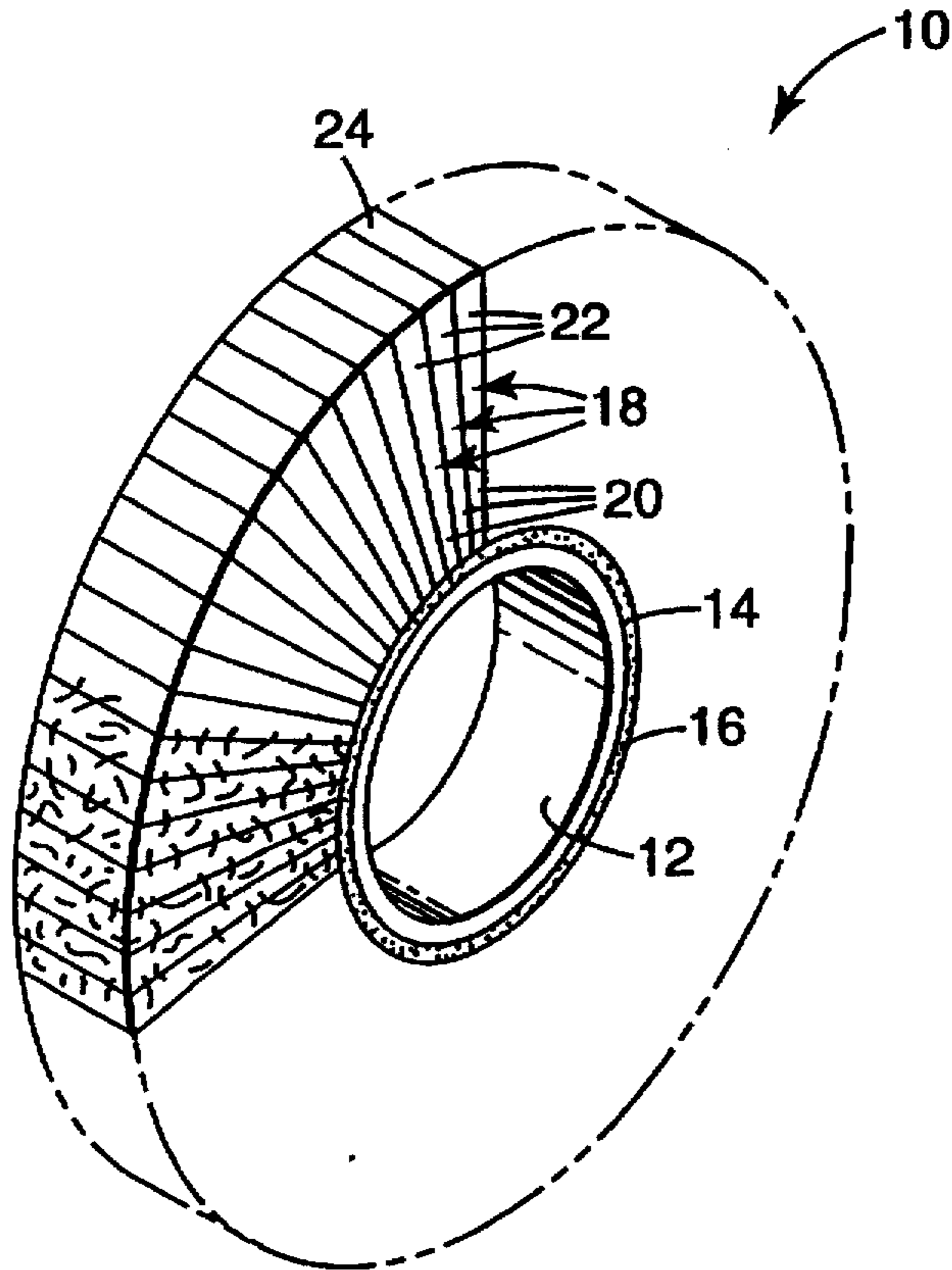
Fig. 1 PRIOR ART
