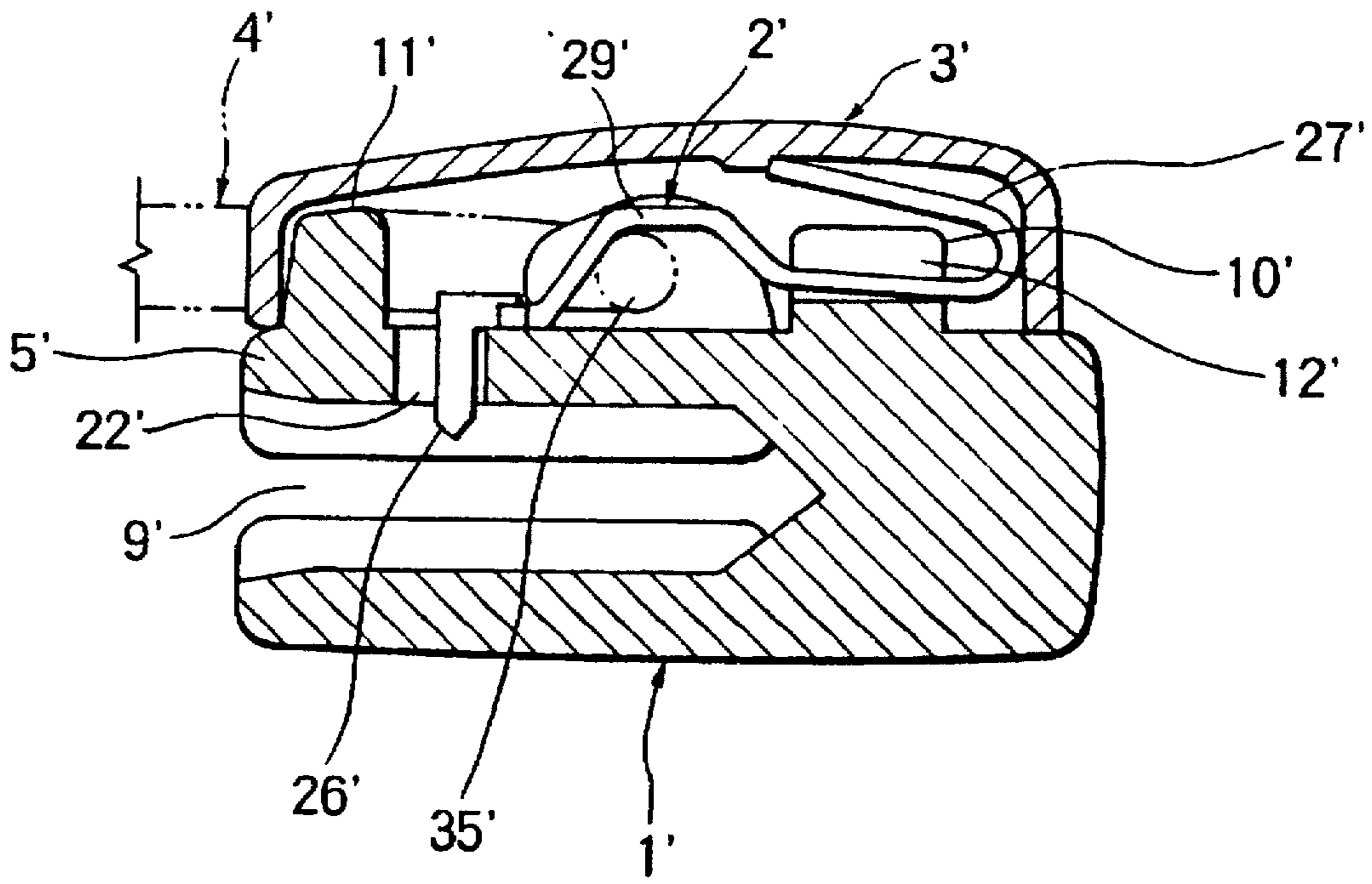
FIG. 7 (PRIOR ART)
