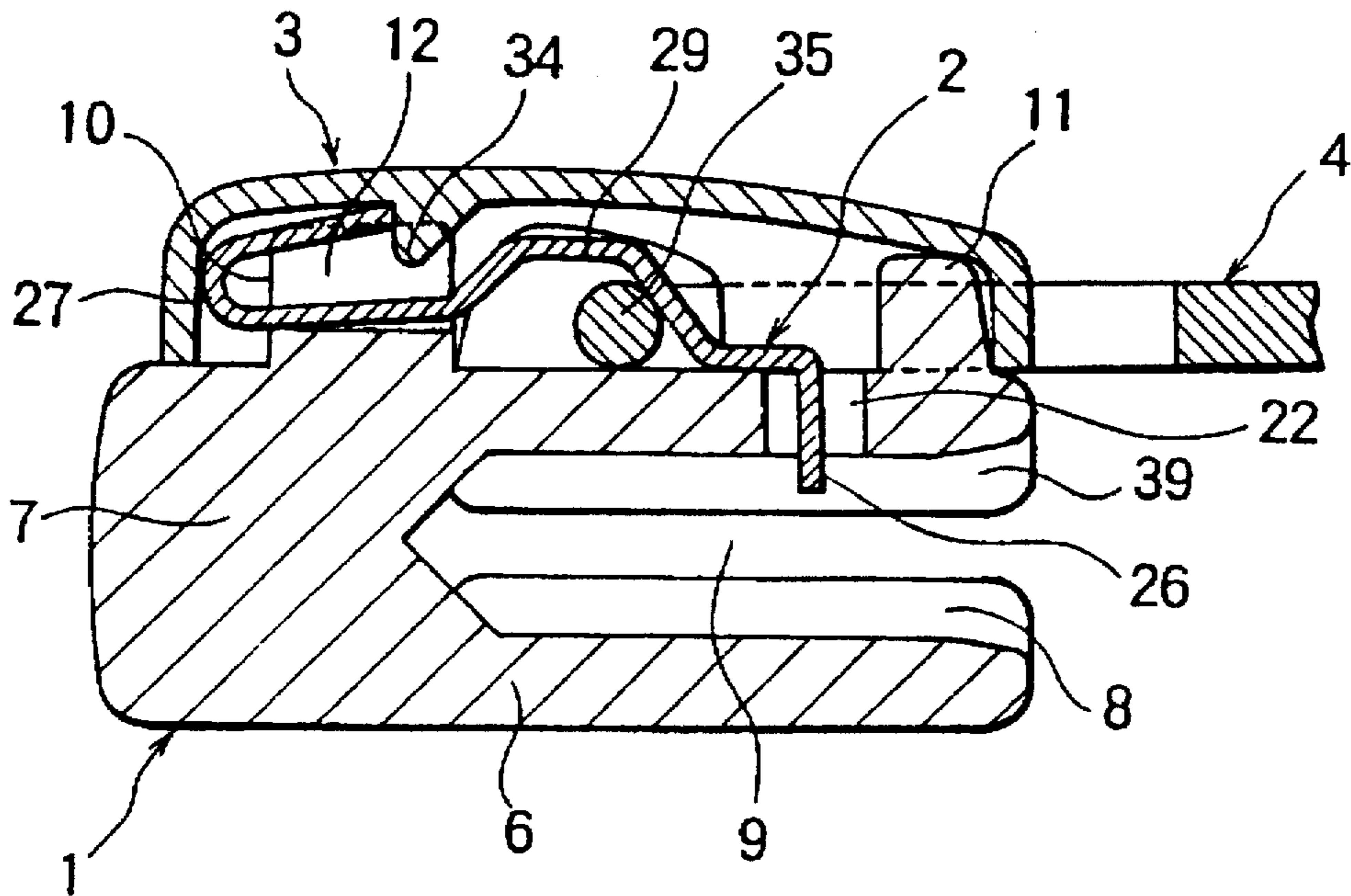
FIG. 7 (PRIOR ART)
