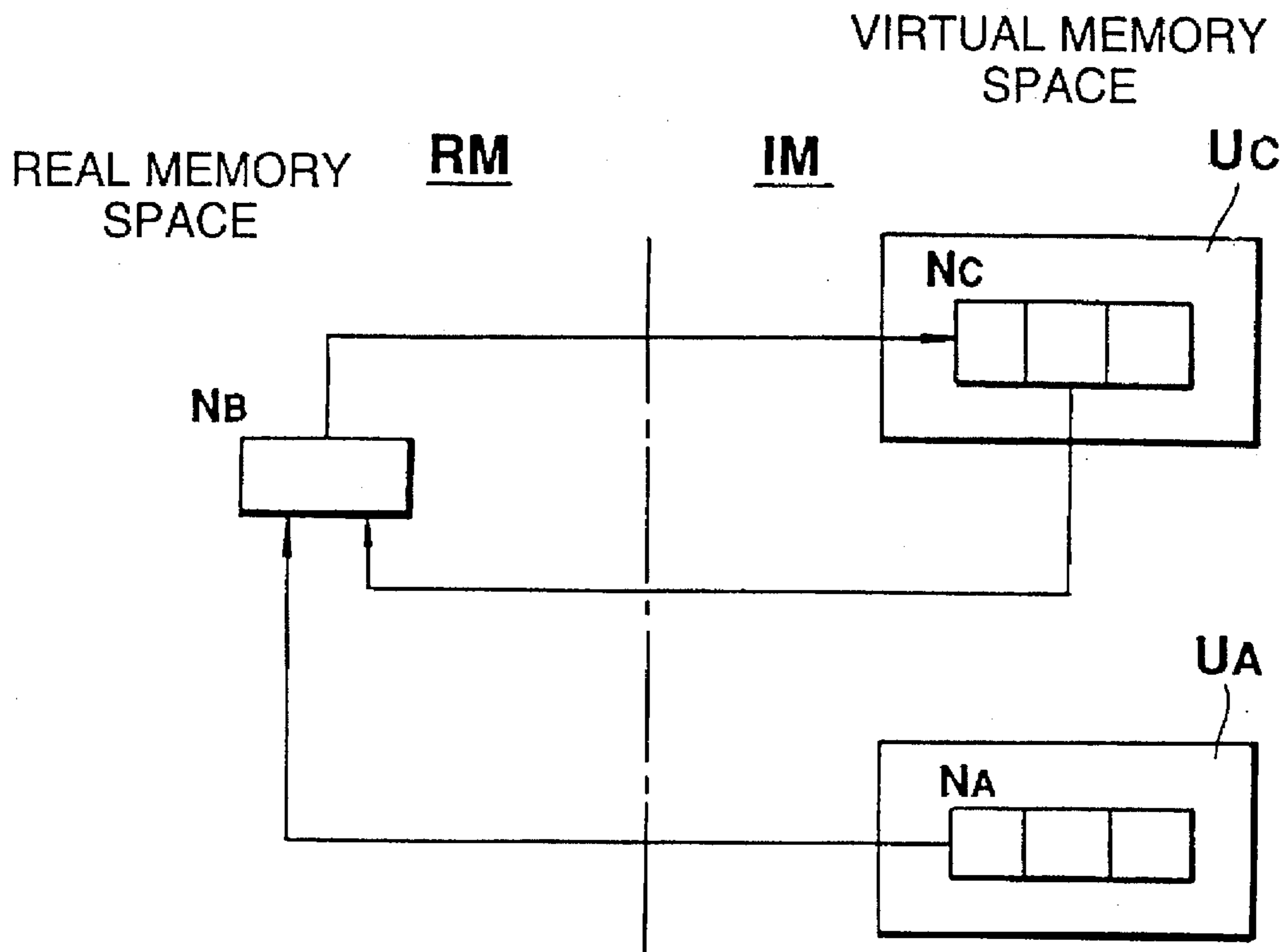
FIG. 14 VIRTUAL MEMORY SPACE
