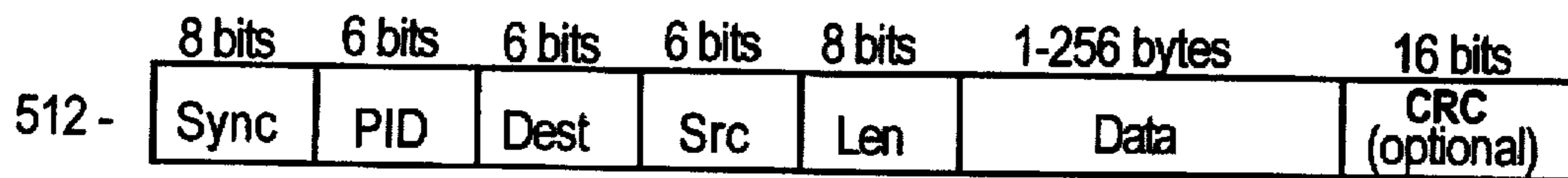
Data Packet
