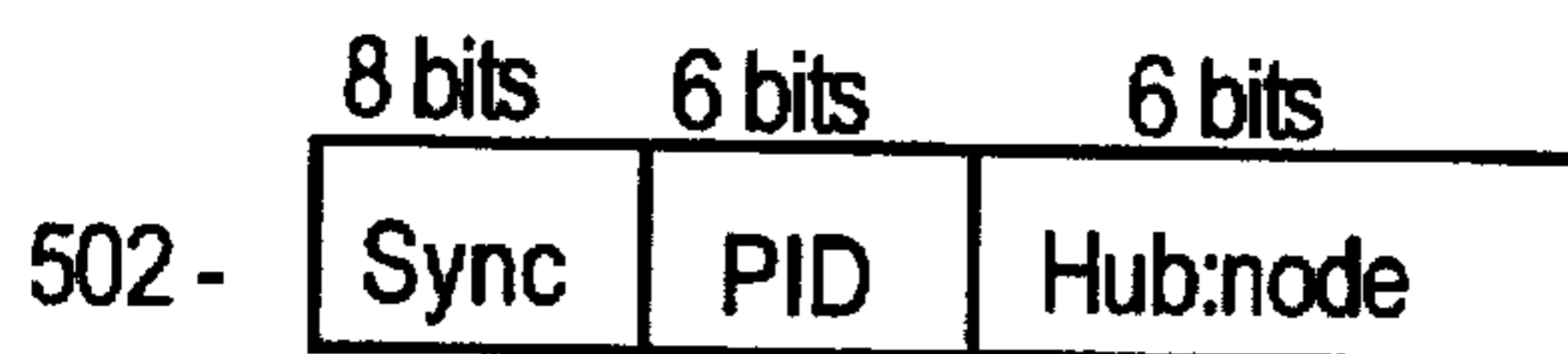
Token Packet
