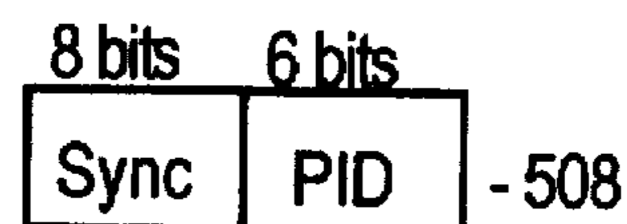
Handshake Packet
