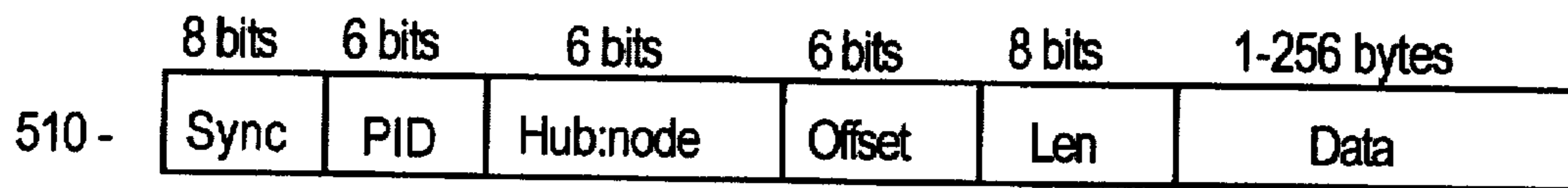
Data Packet
