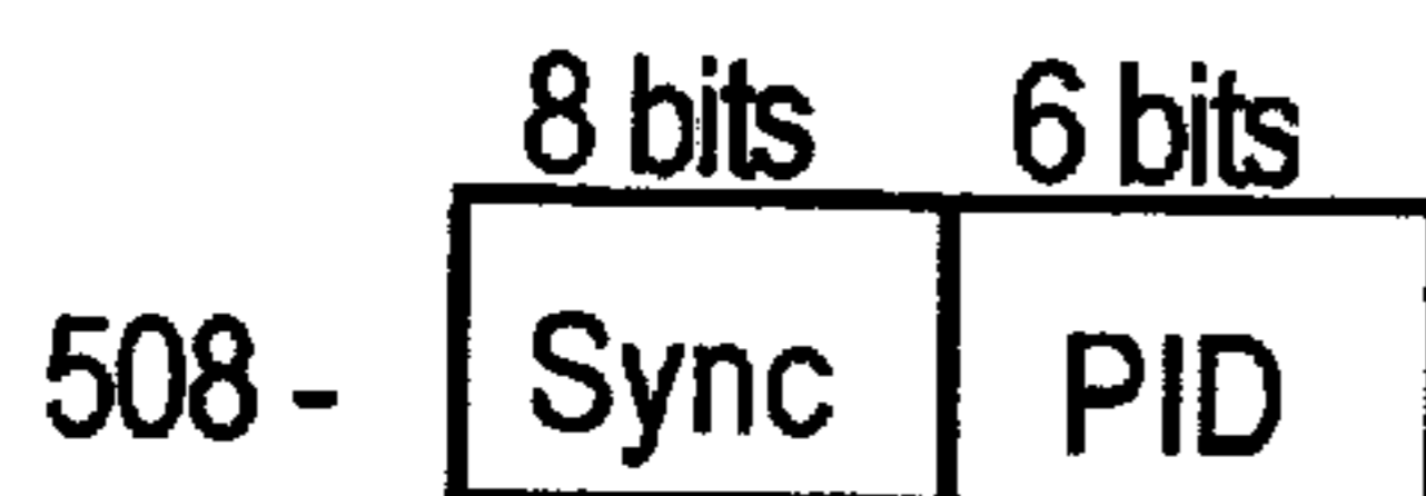
Handshake Packet
