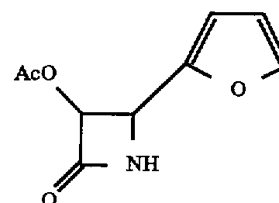
(±)-cis-3-(Acetyloxy)-4-(2-furyl)azetid-2-one (XVb)
