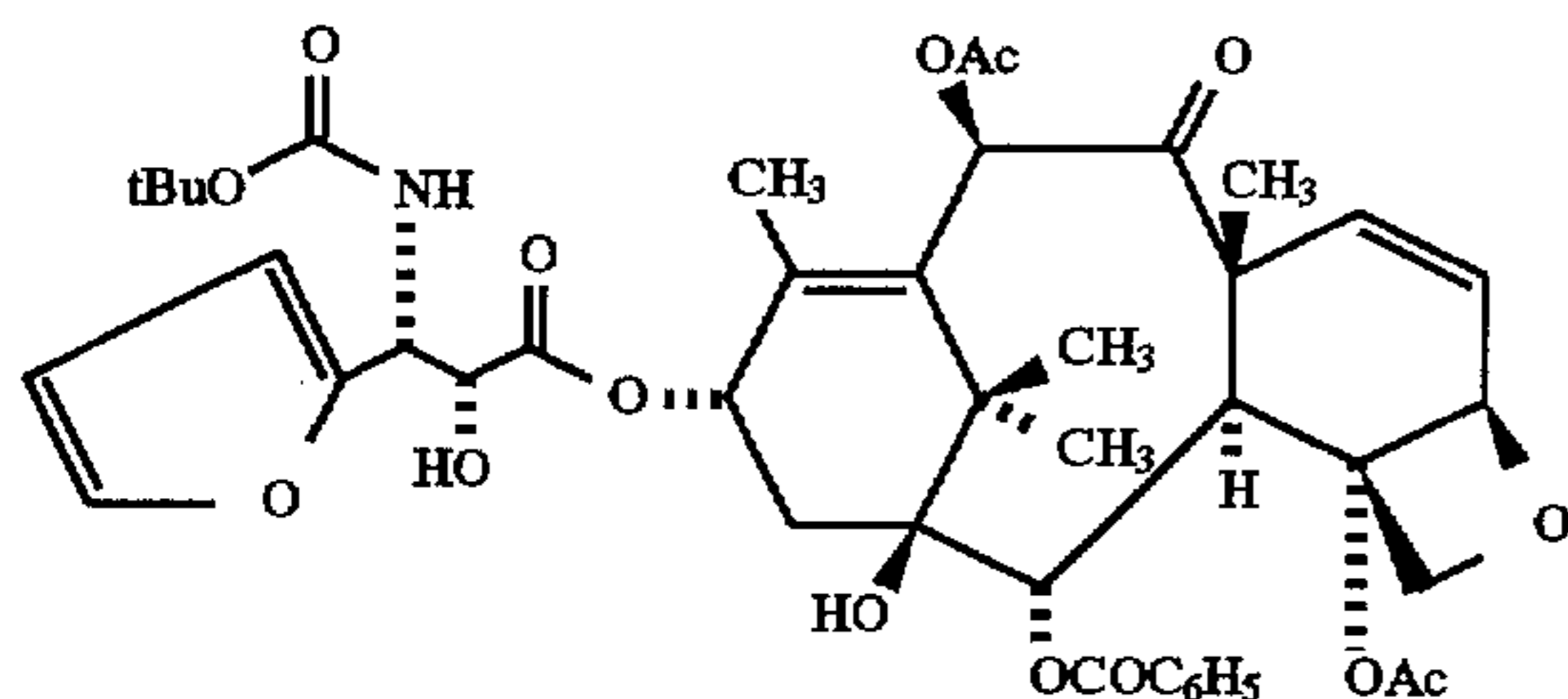
6,7-Dehydro-3'-(2-furyl)-3'-N-debenzoyl-N-t-butoxycarbonylpaclitaxel (Ib)
