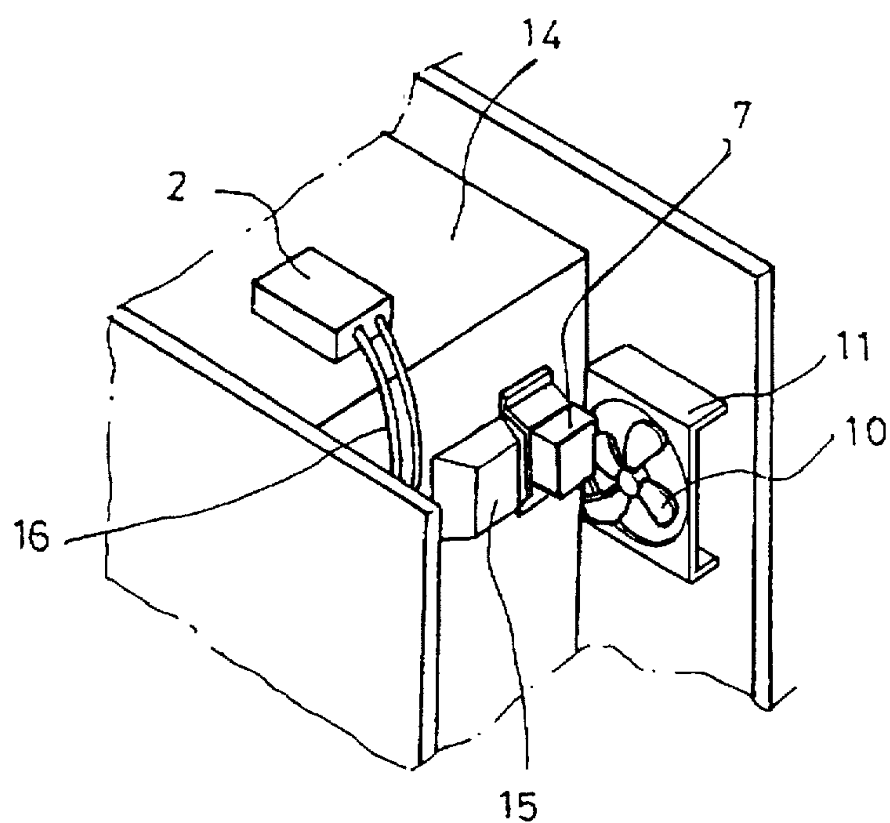
FIG. 2 CONVENTIONAL ART
