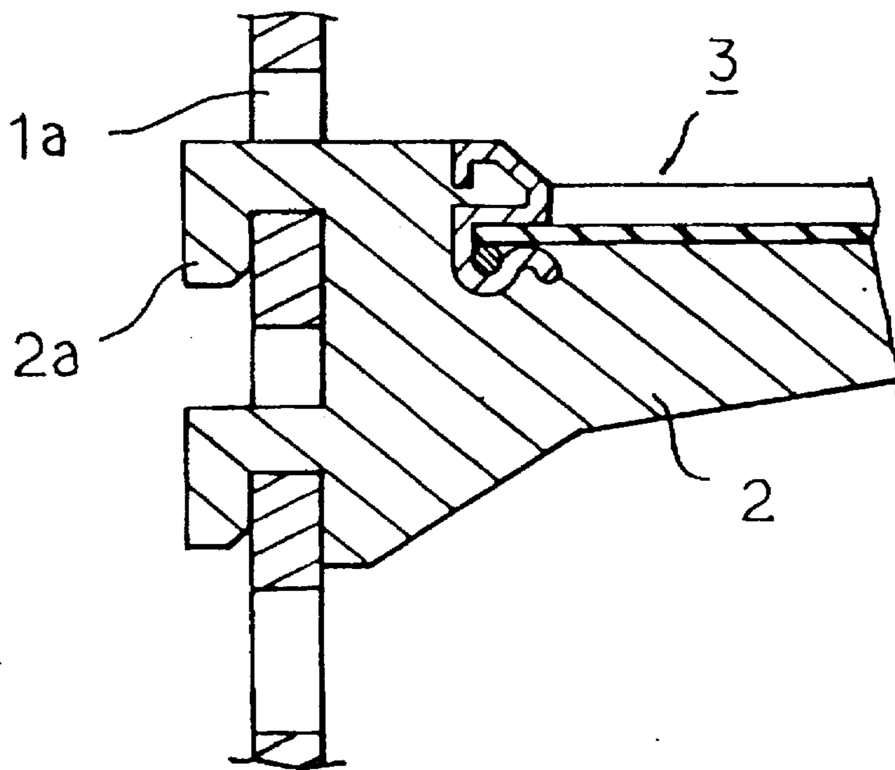
FIG. 2 PRIOR ART
