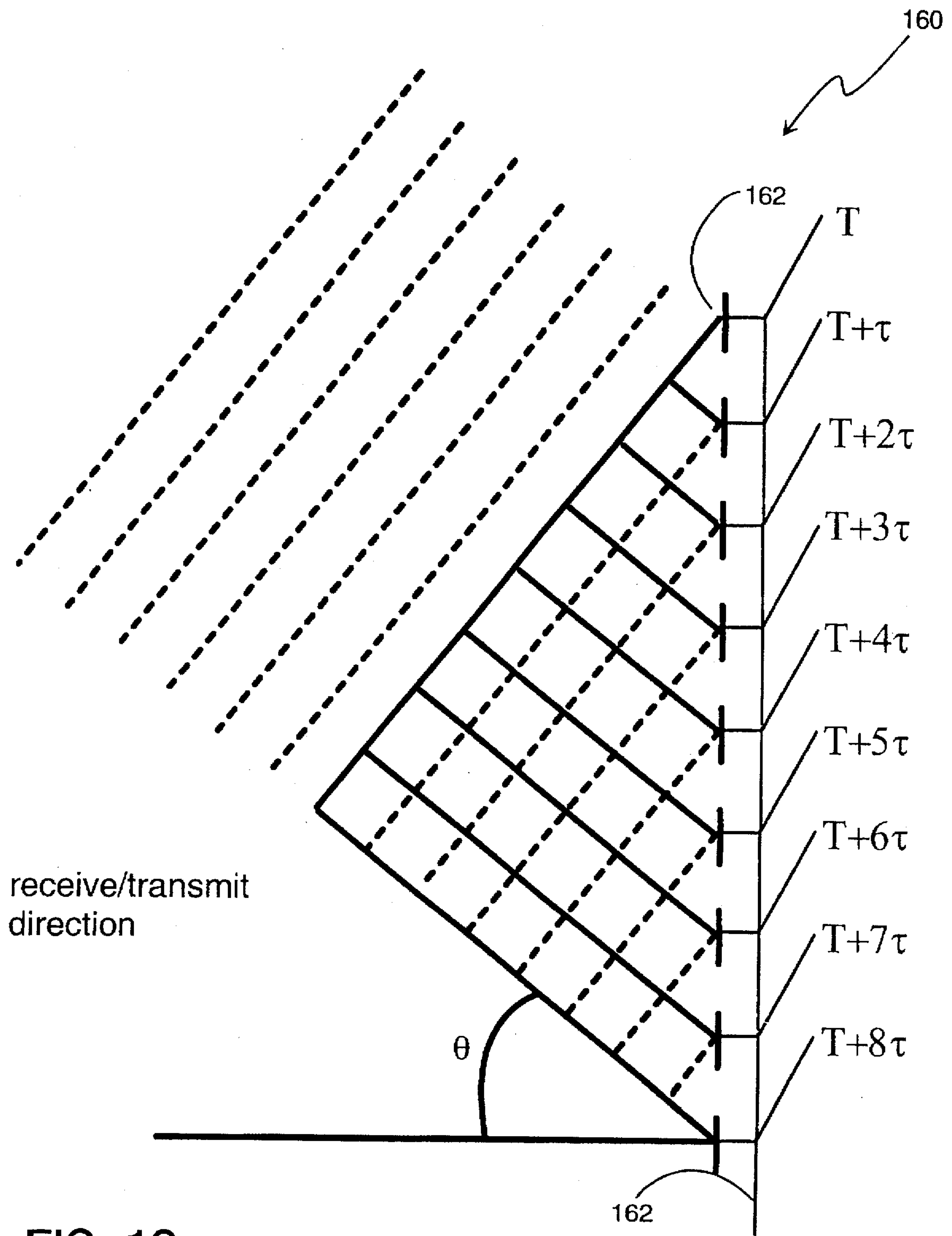
Phased Array Antenna
