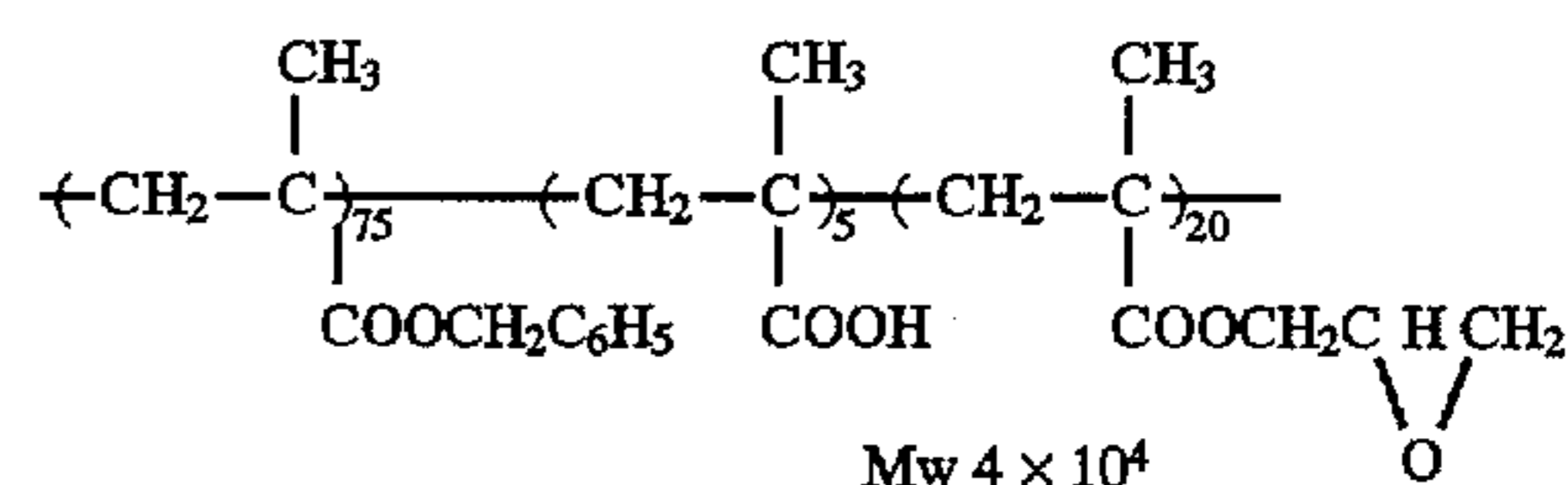
Compound (B)
