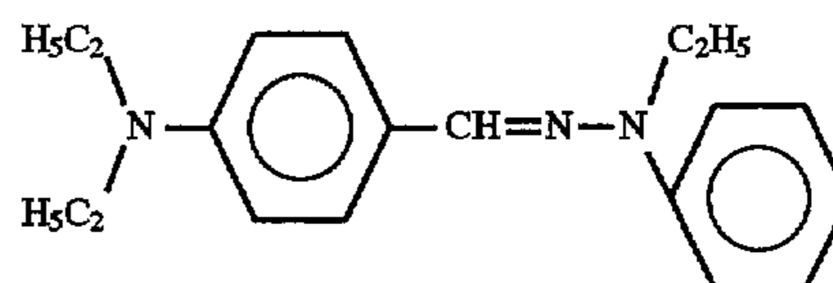
Hydrazone Compound
