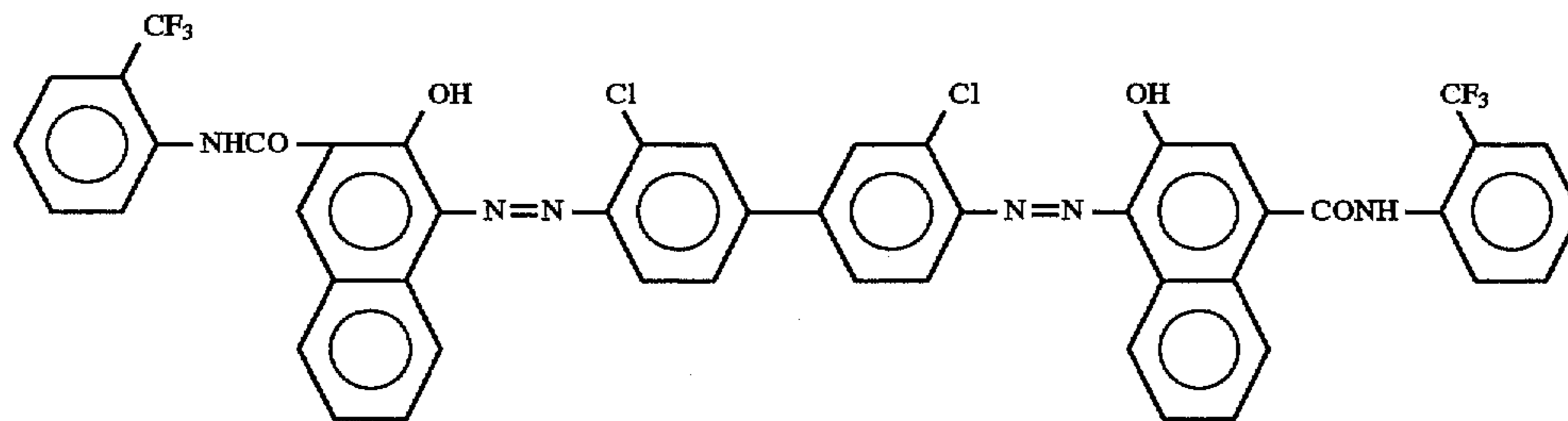
Bisazo Pigment
