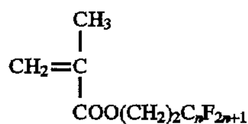
Monomer (m-1)
