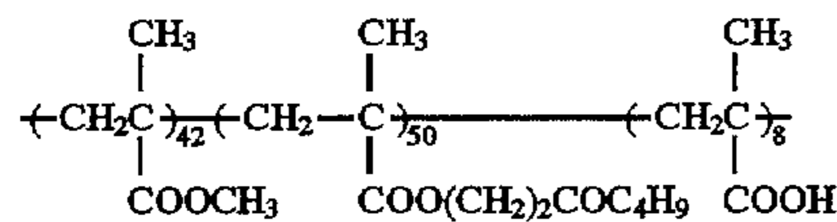
Resin (A-2)
