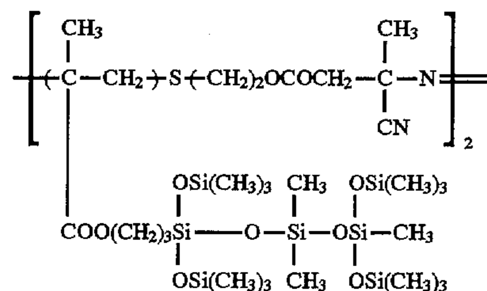
Polymer (P-13)
