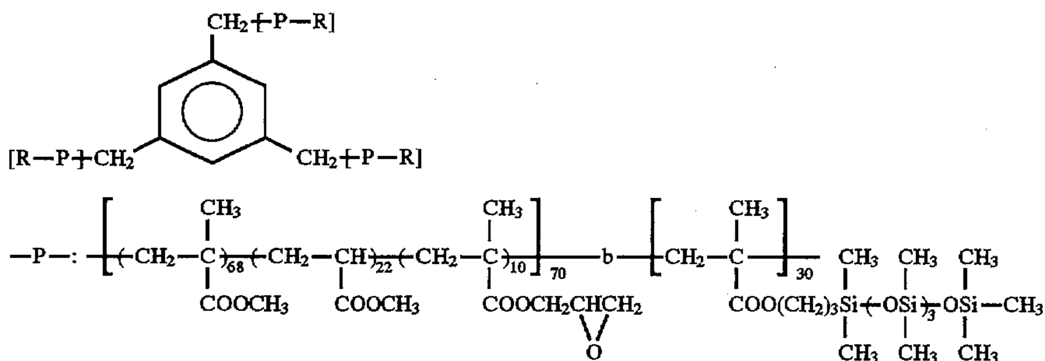
Resin (P-20)
