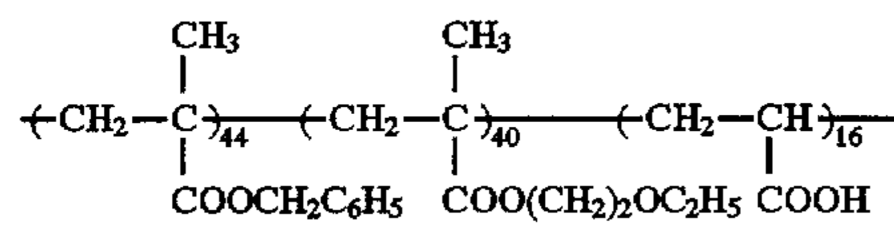
Resin (A-1)
