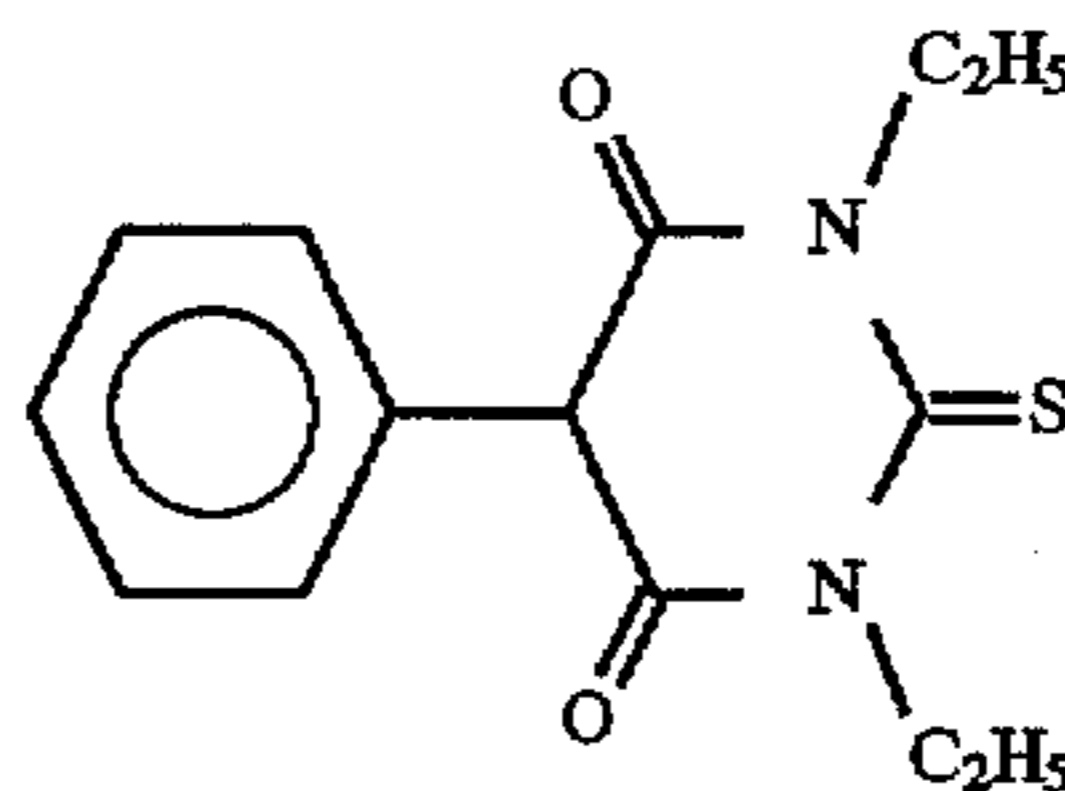
Compound (B)
