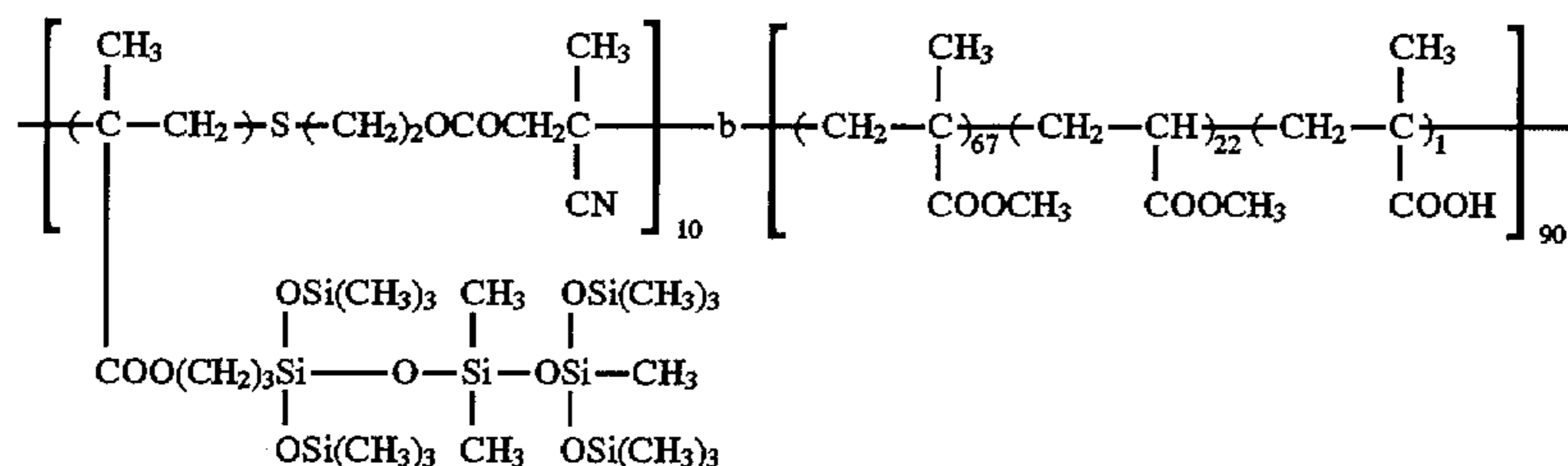
Polymer (P-13)
