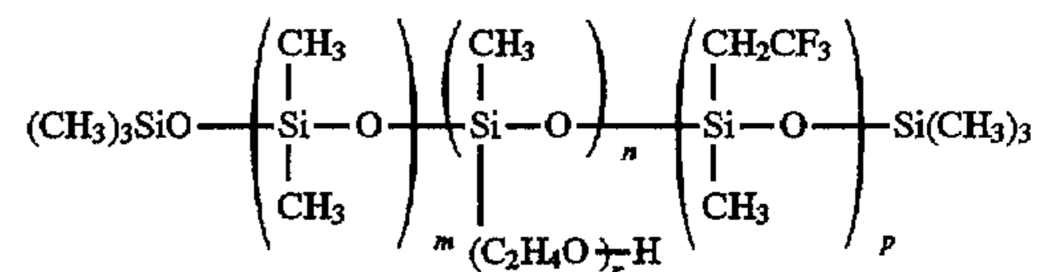
Compound (S-6)
