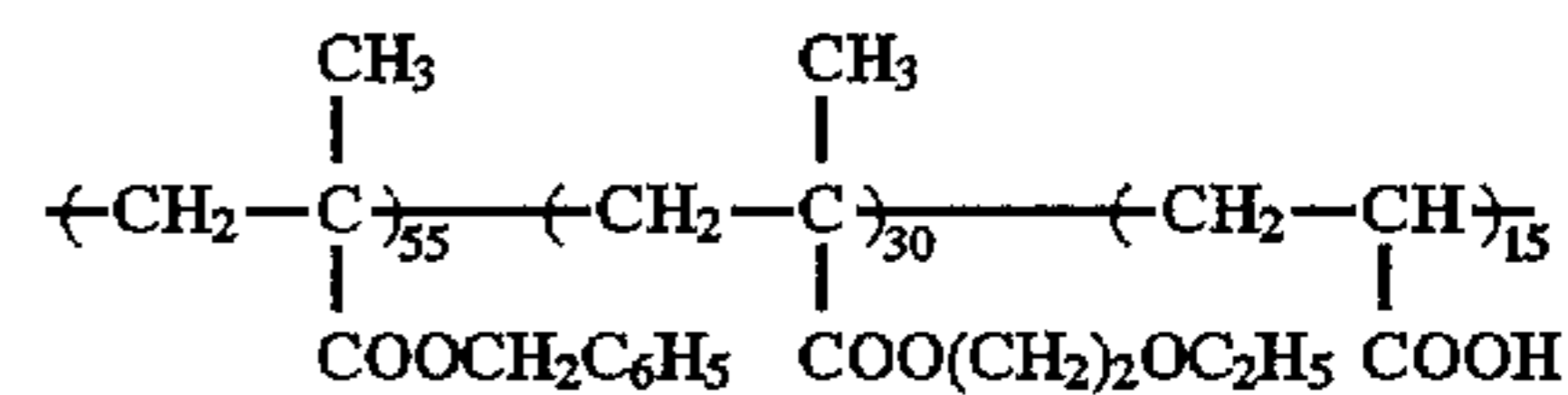
Resin (A-3)
