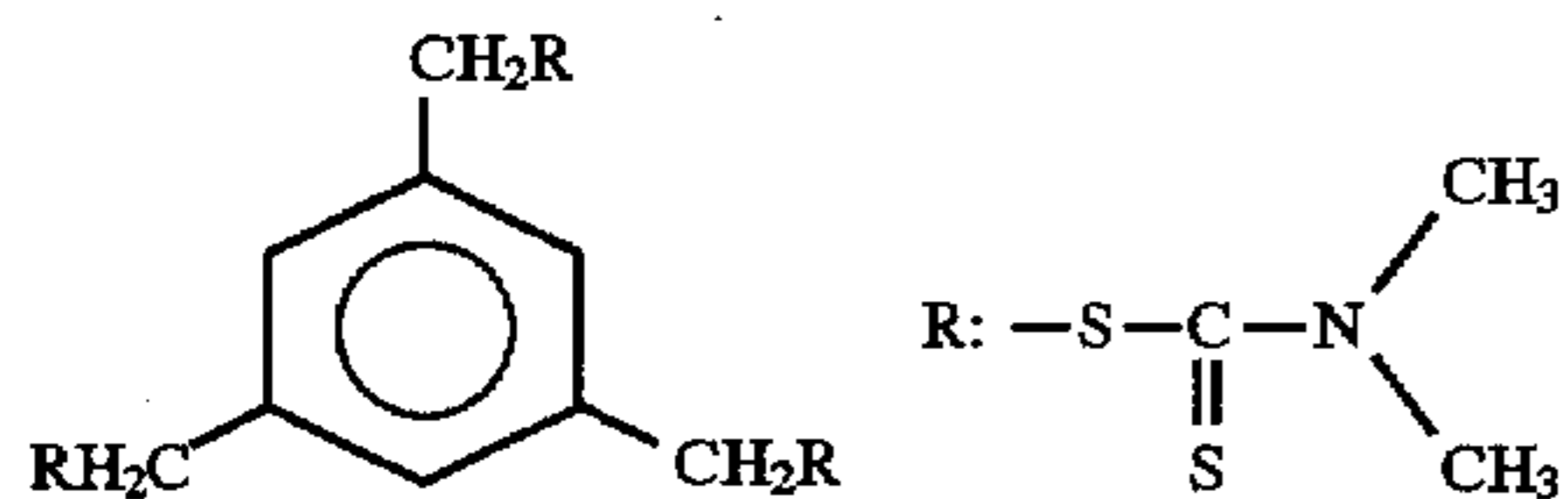
Monomer (m-2)
