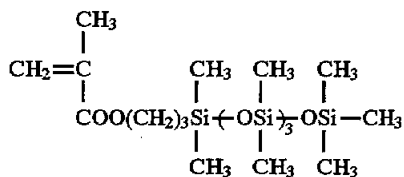
Resin (P-20)
