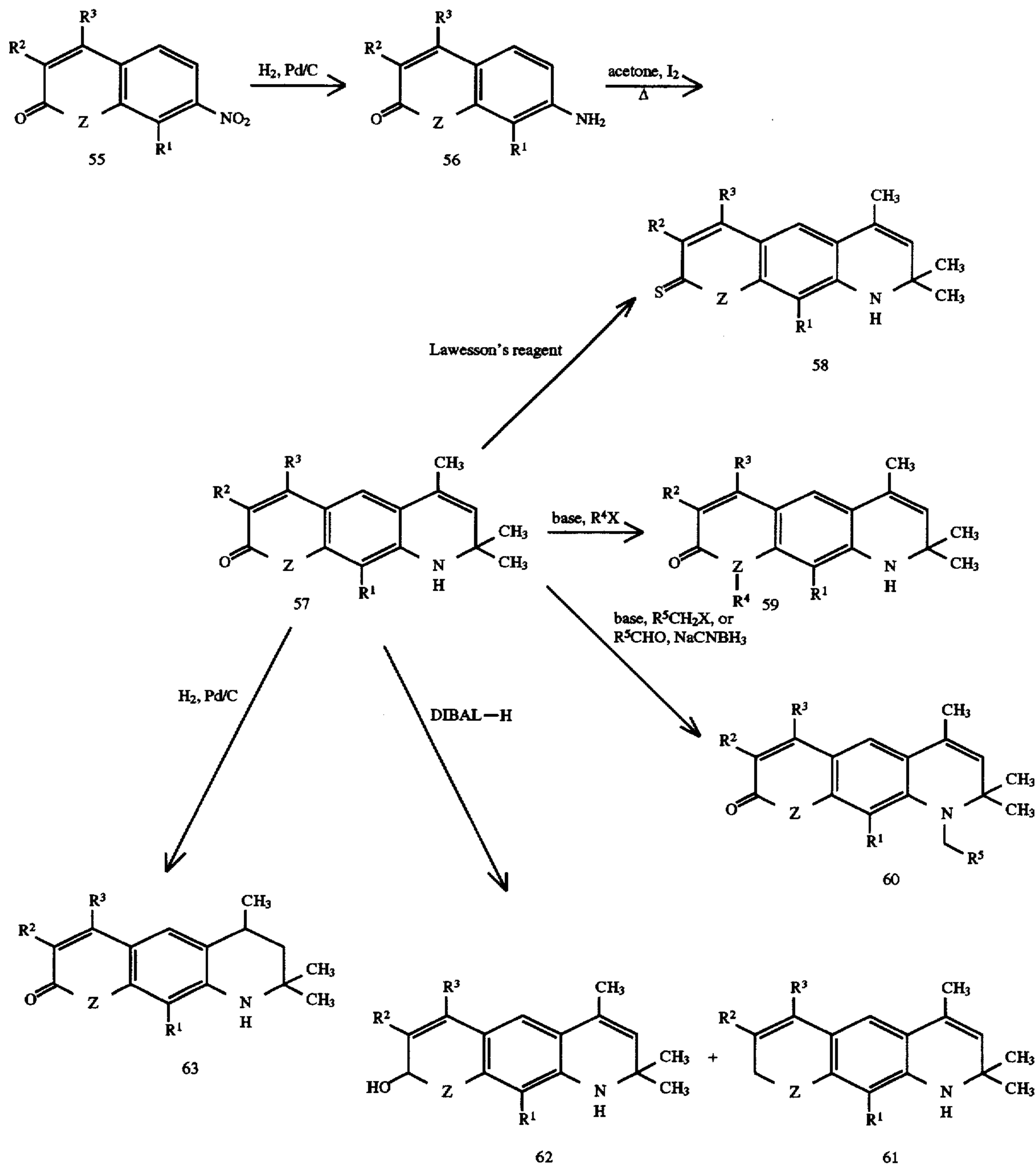
Scheme XVI
