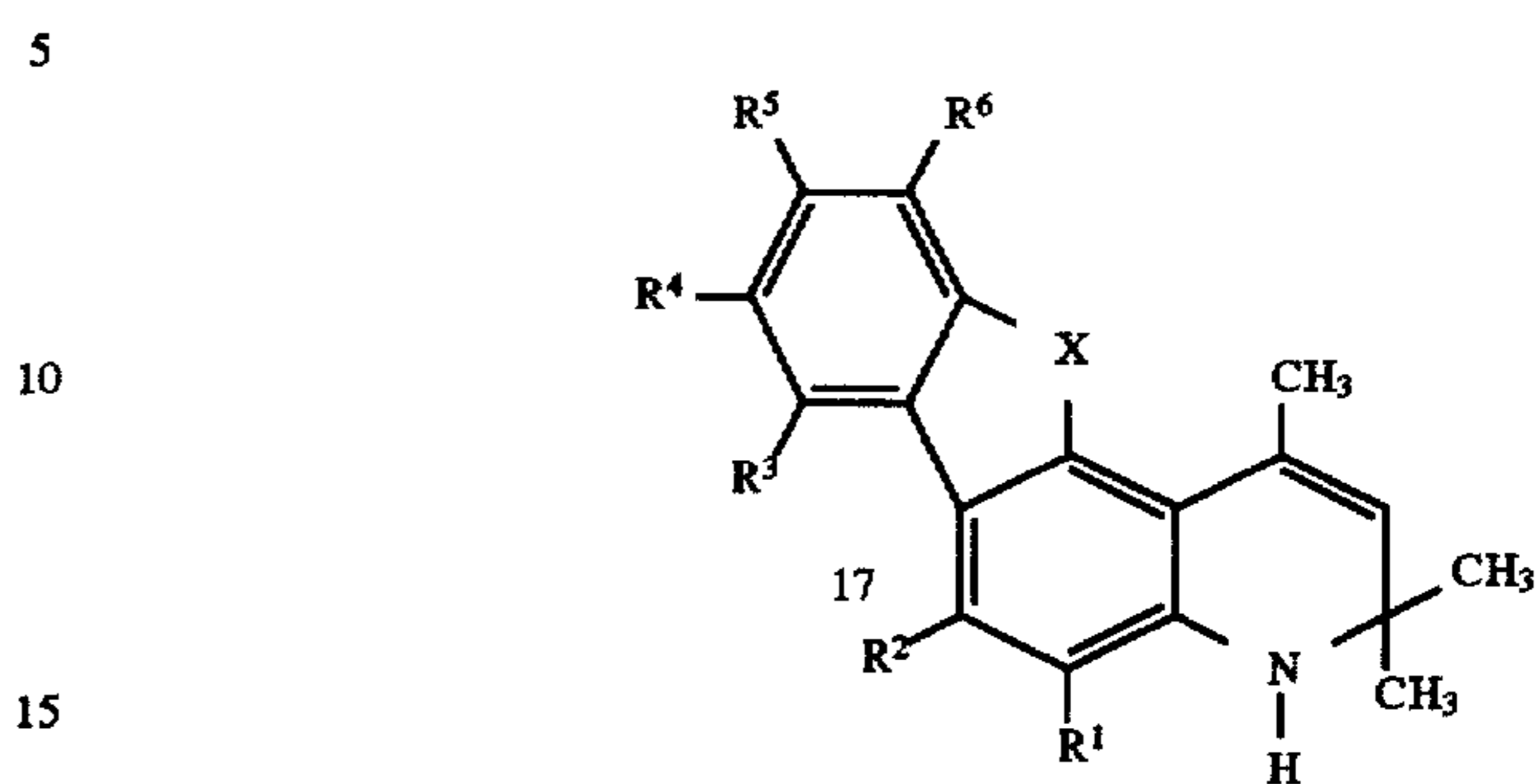
Scheme IV
