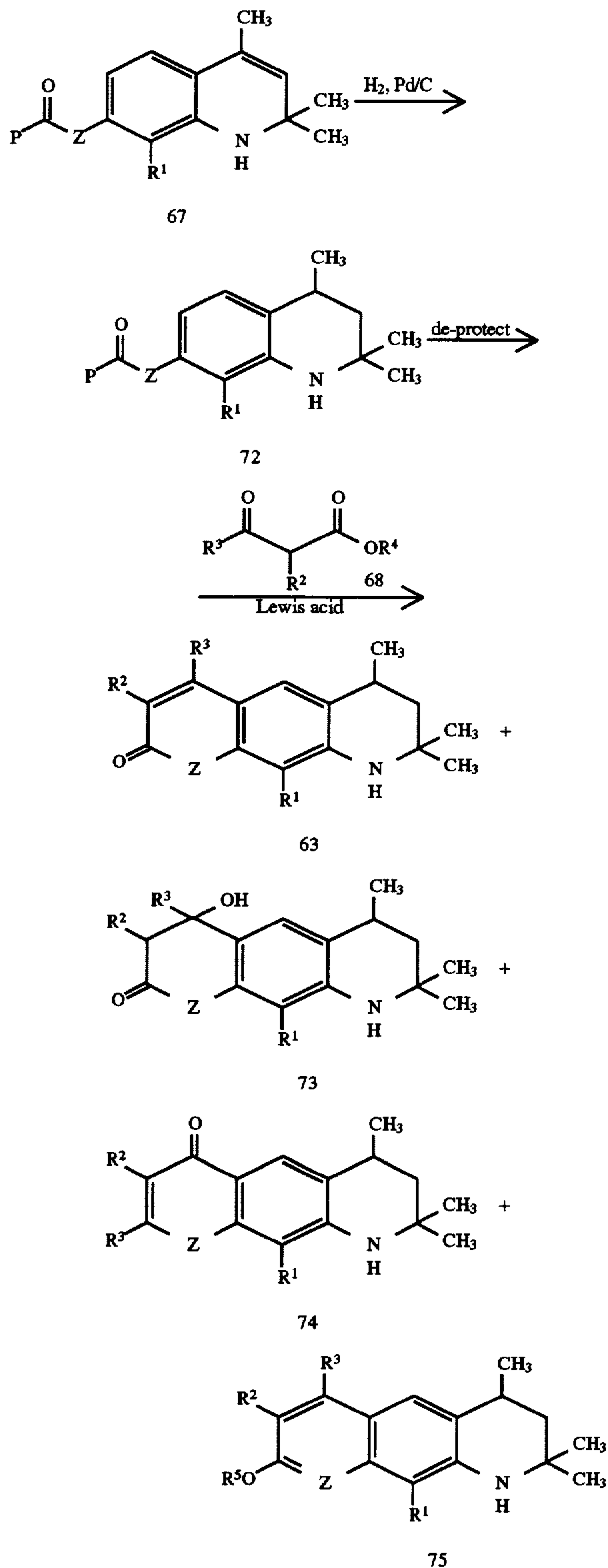
Scheme XVIII
