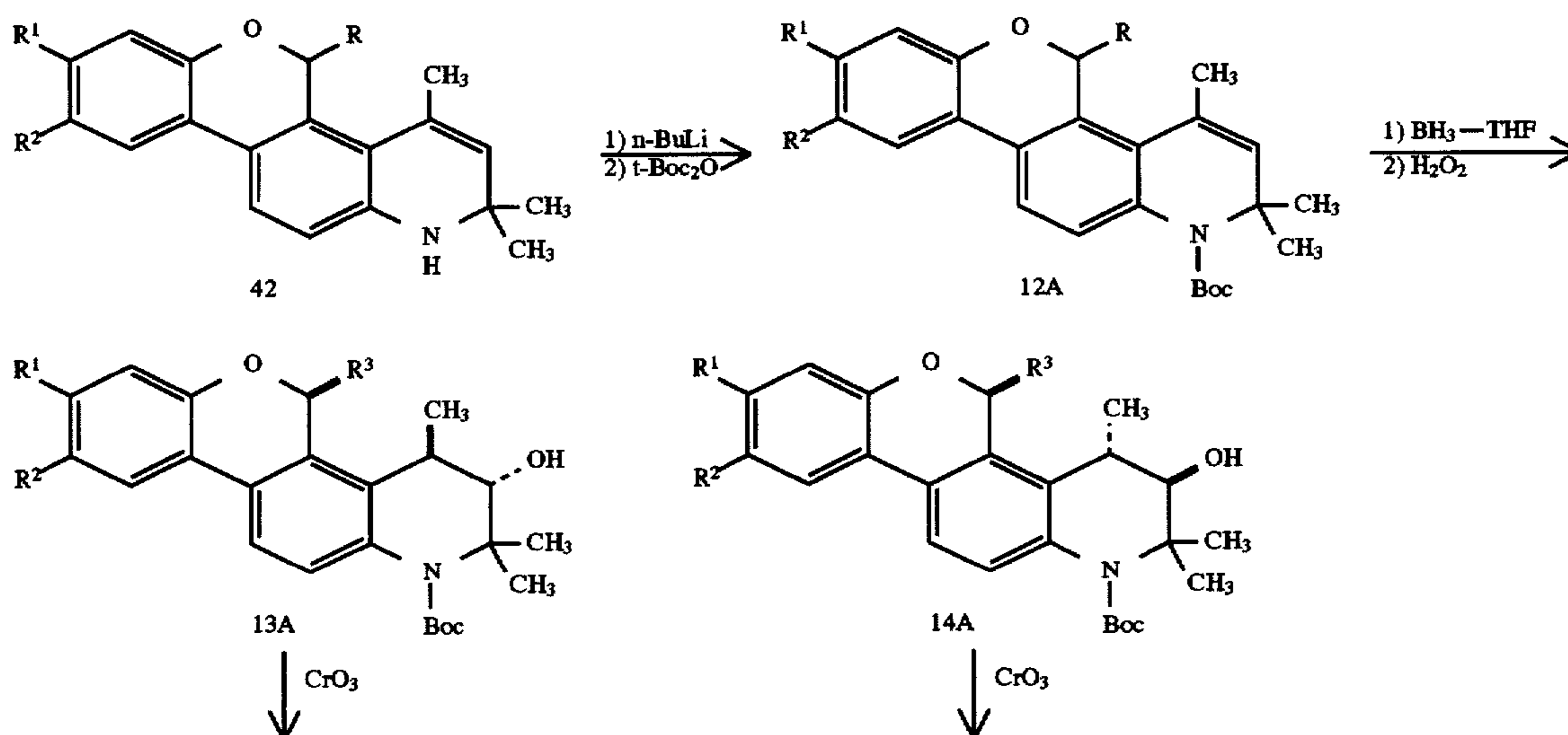
Scheme XXXIII
