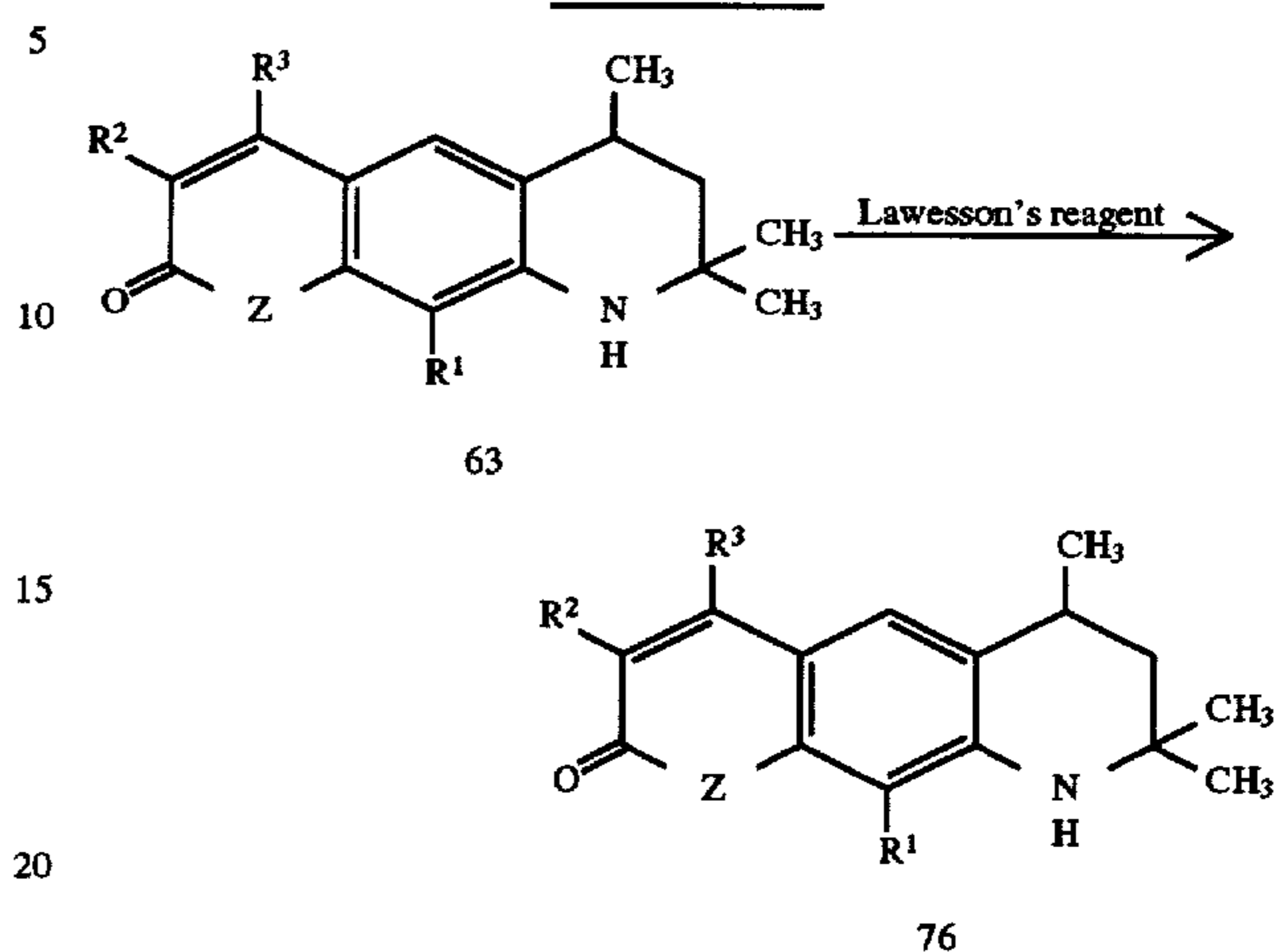
Scheme XIX
