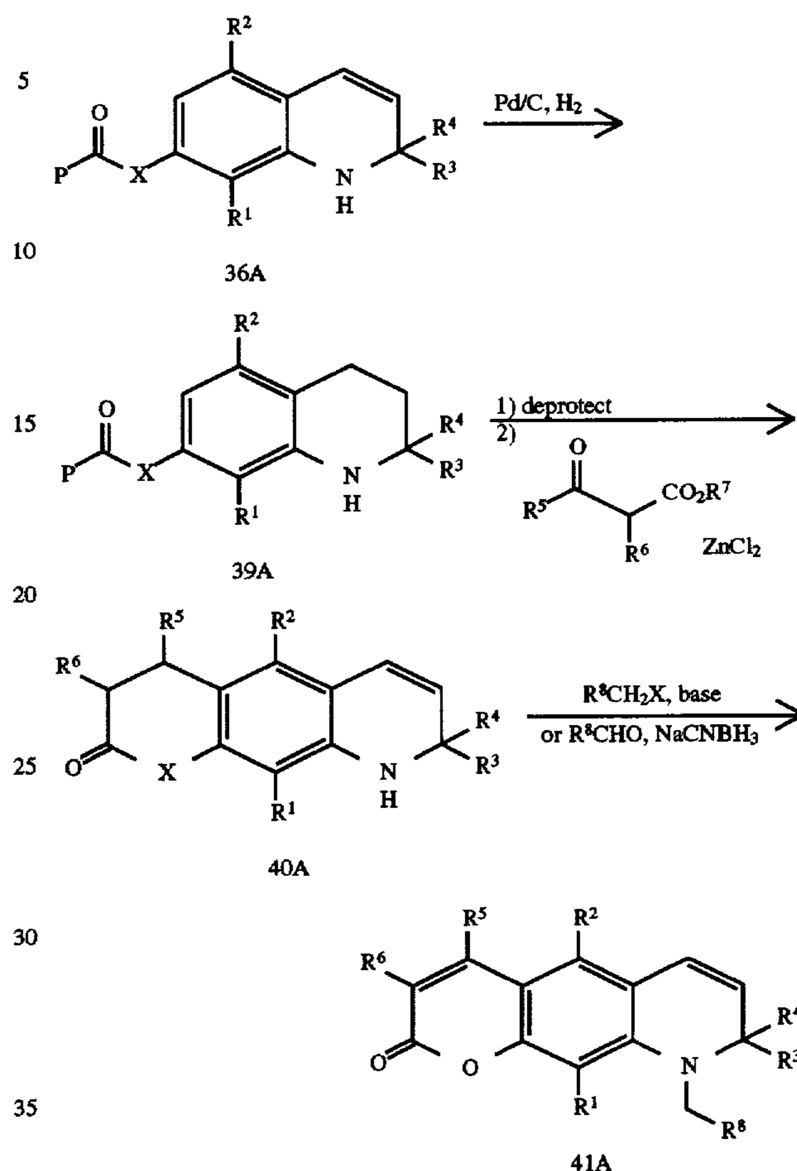
Scheme XLII
