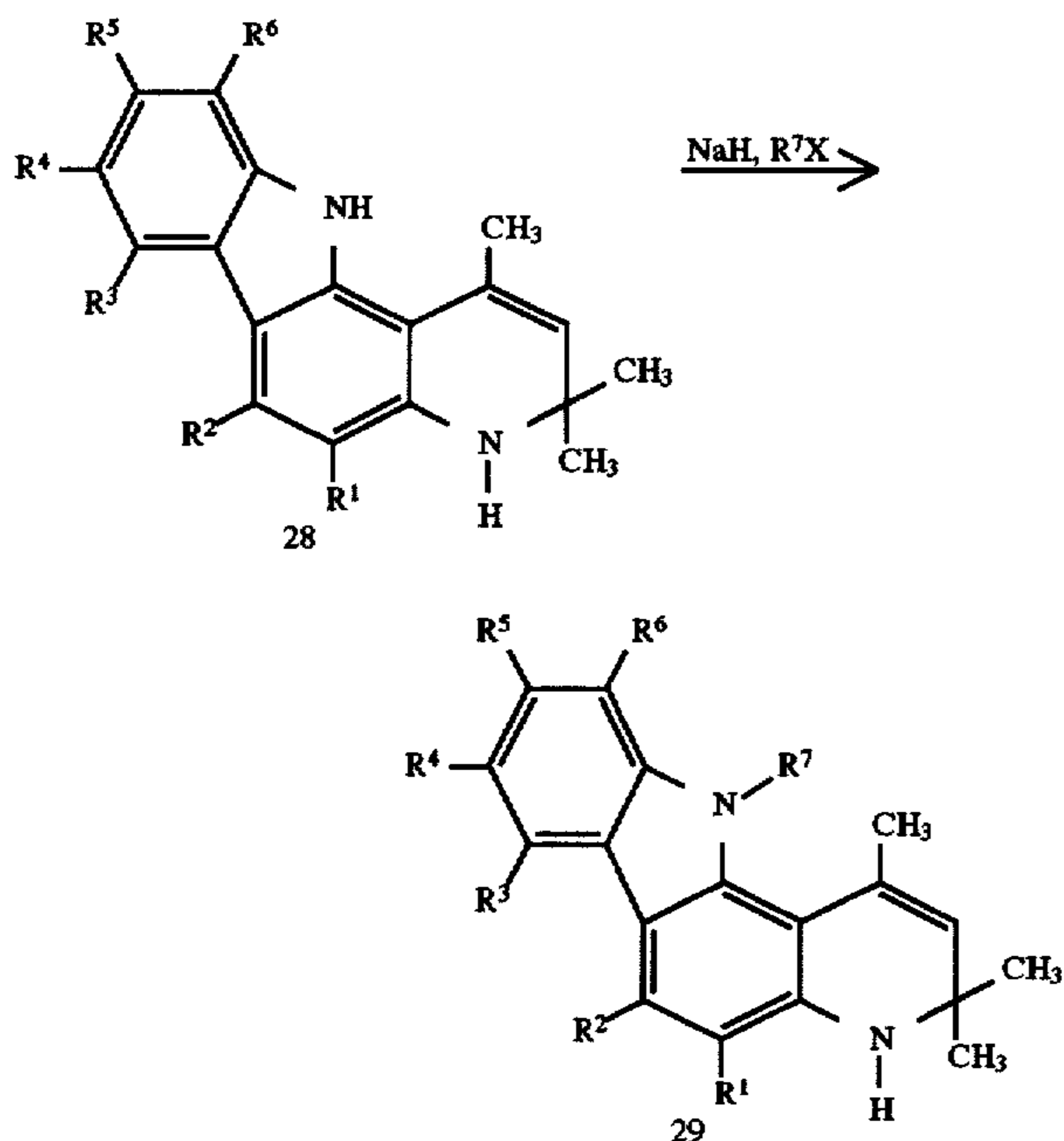
Scheme VIII
