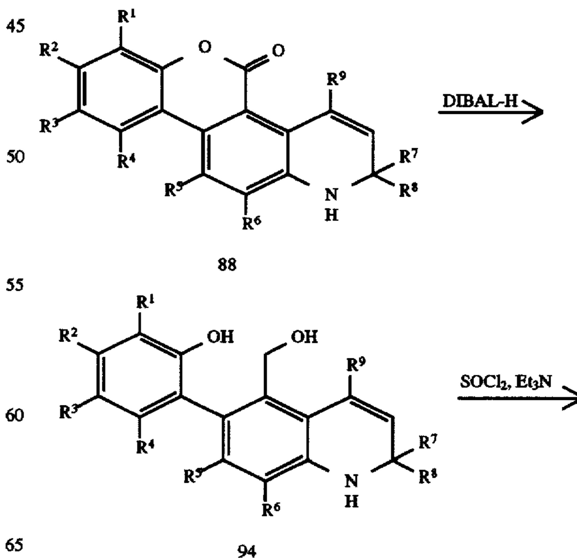
Scheme XXV
