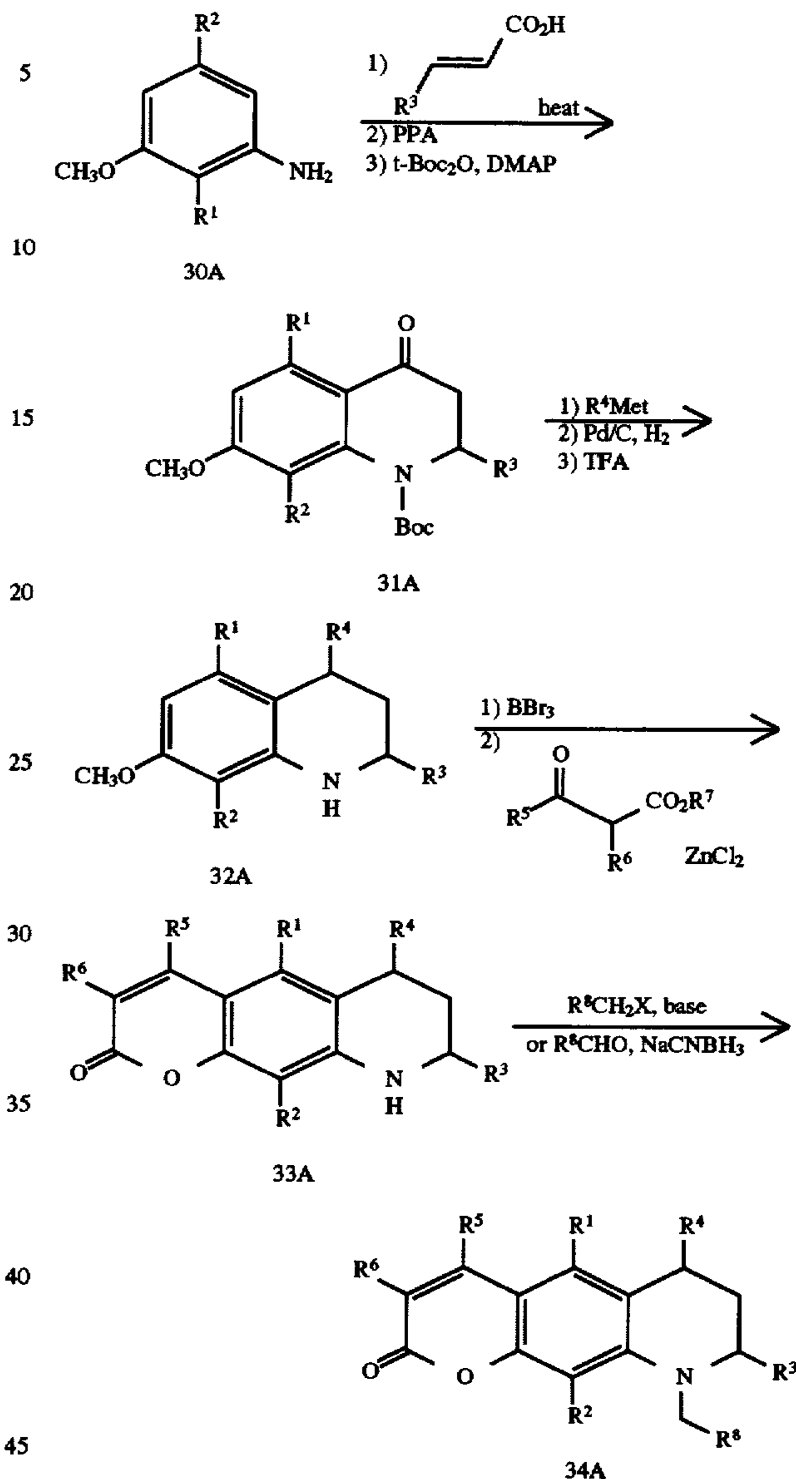
Scheme XL
