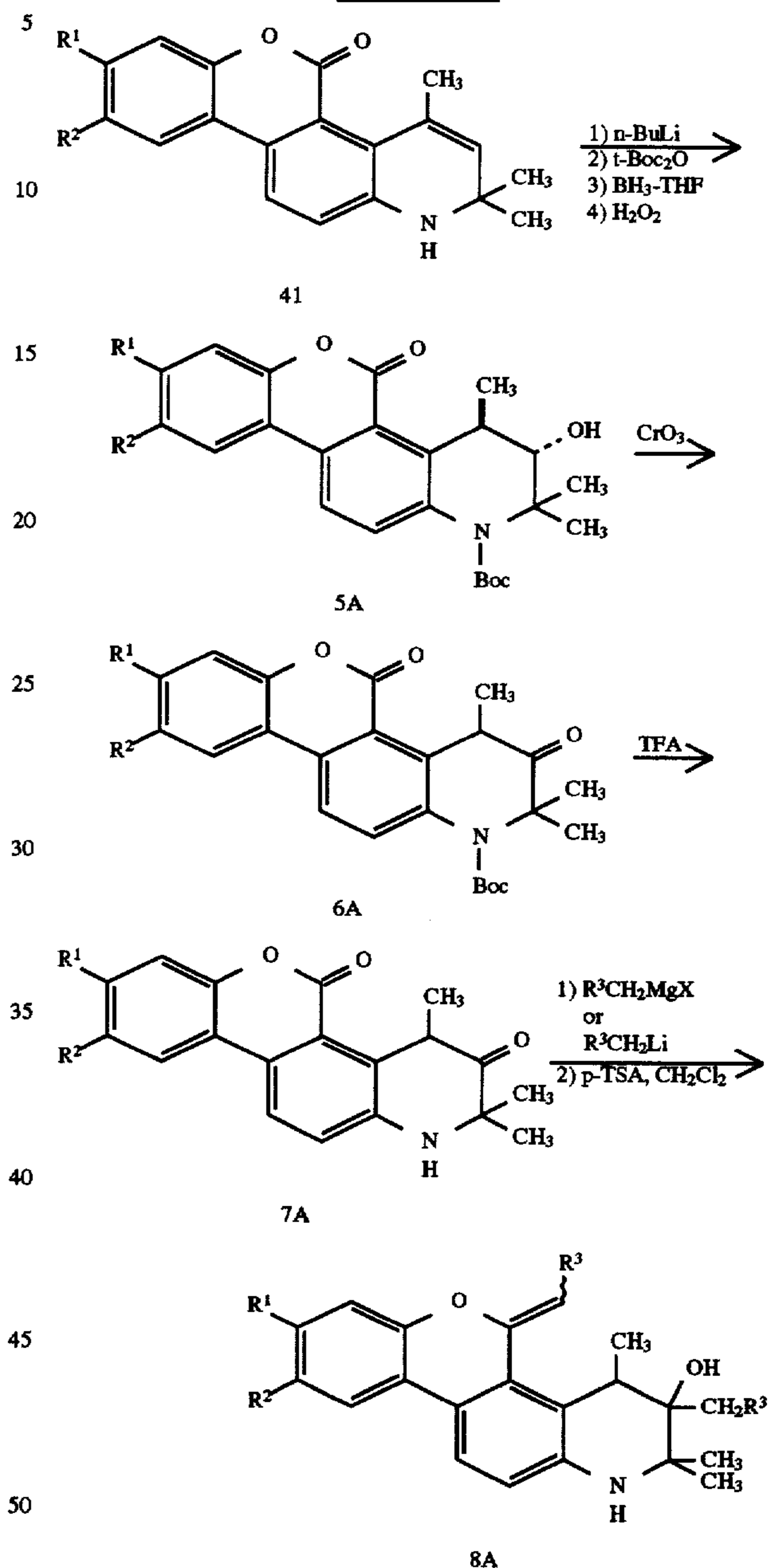
Scheme XXX
