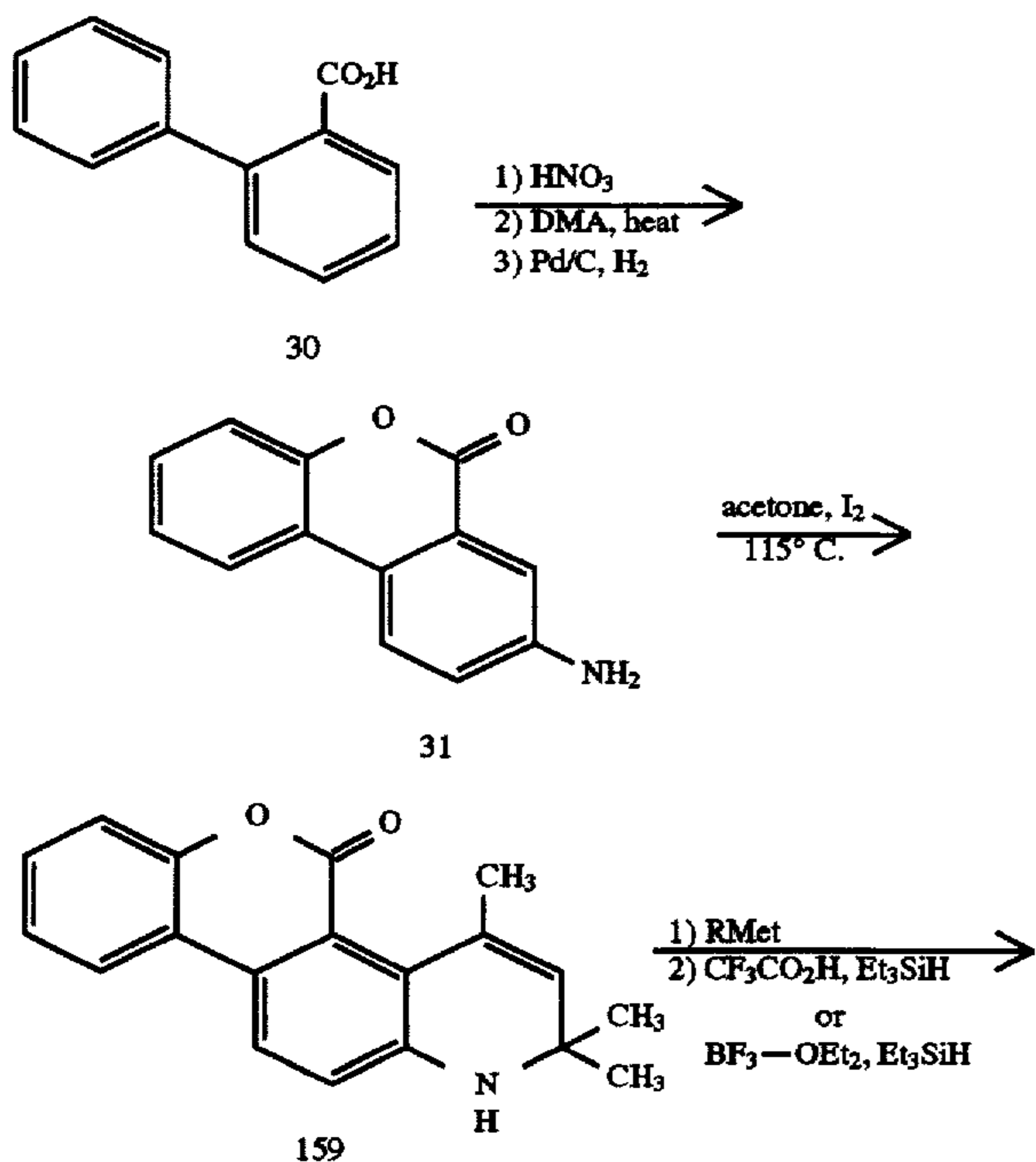
Scheme IX
