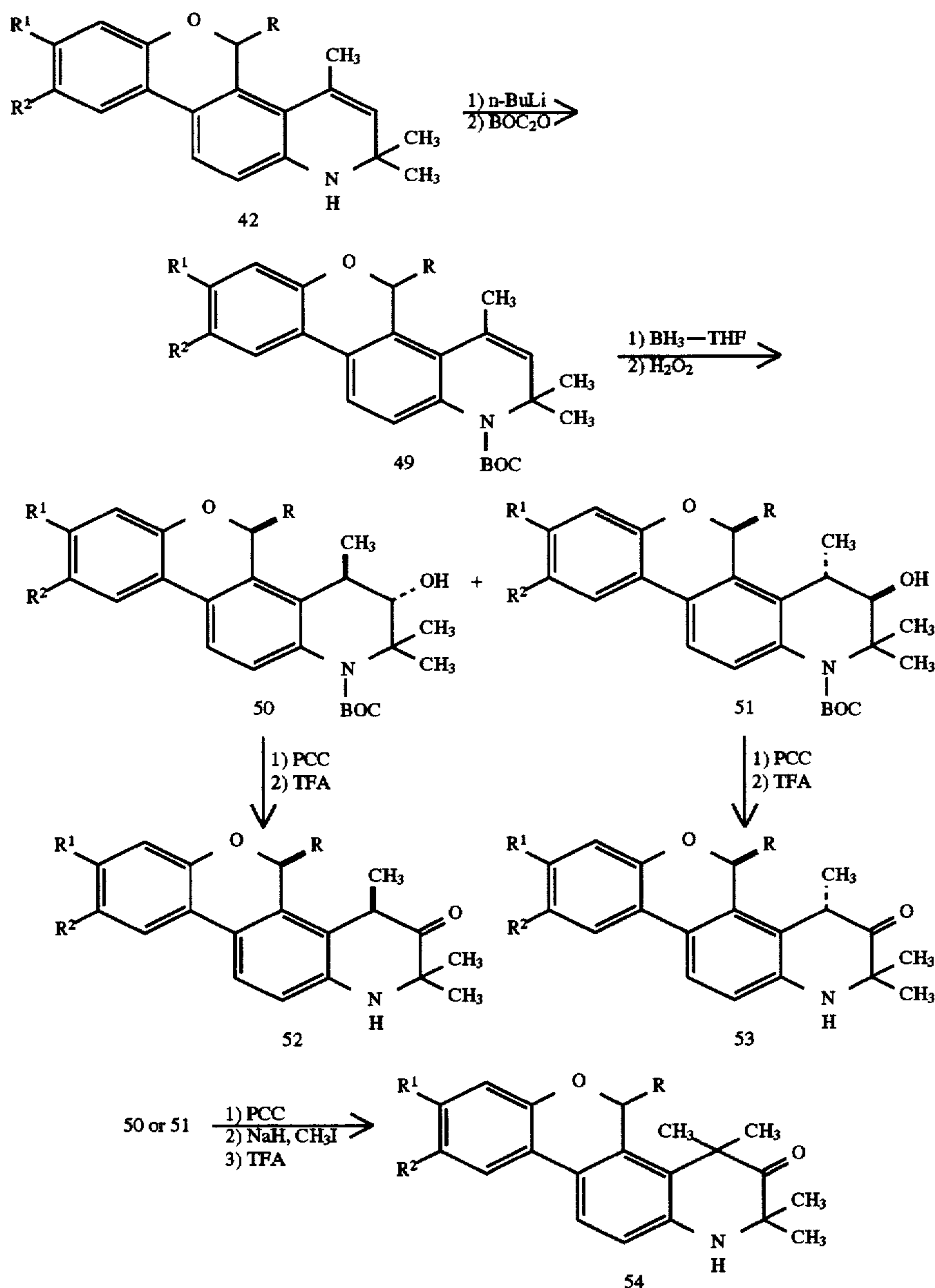
Scheme XV
