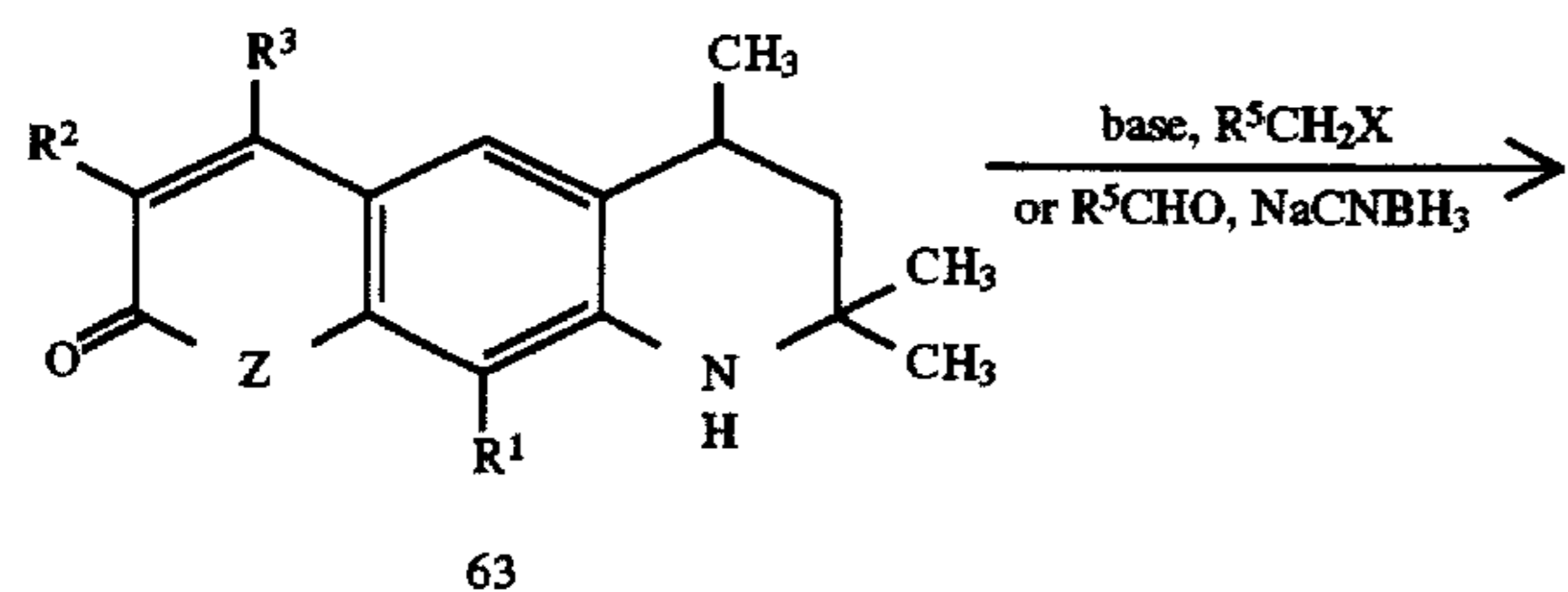
Scheme XXXVIII
