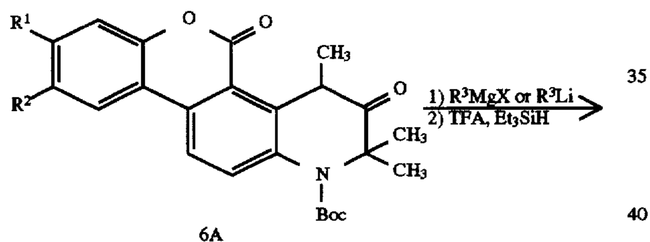
Scheme XXXII
