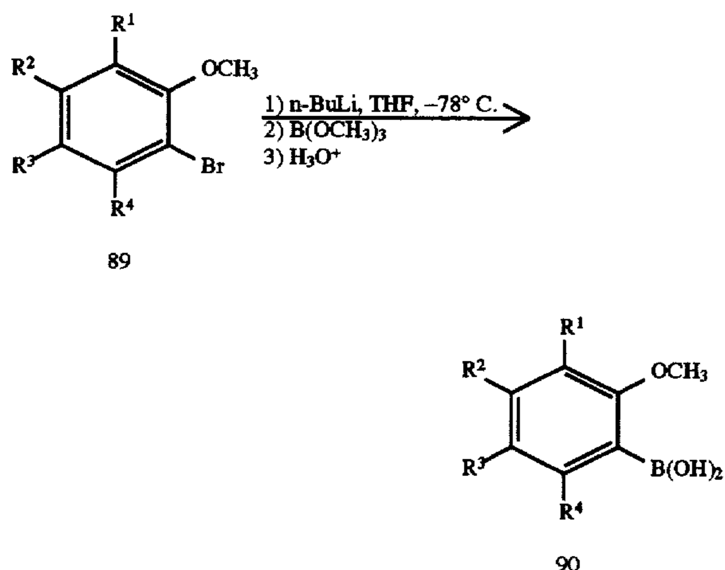
Scheme XXIV
