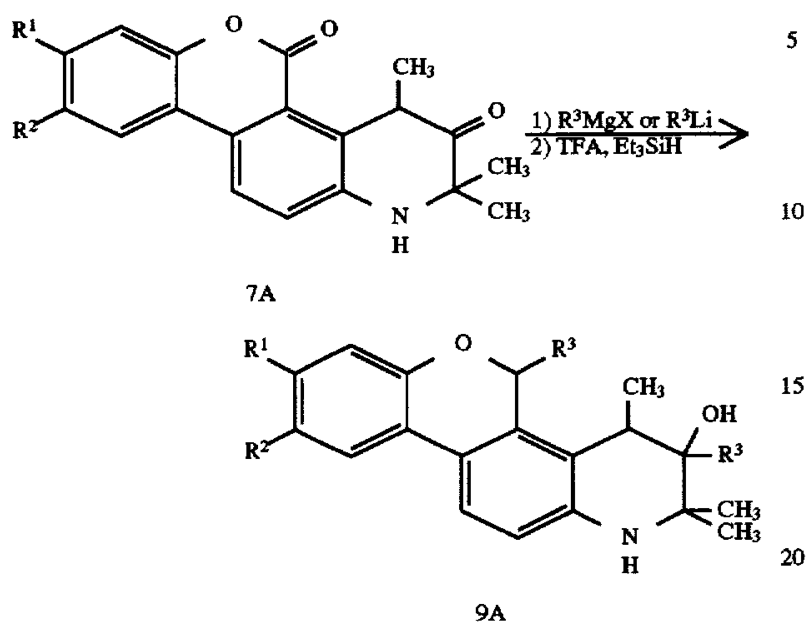
Scheme XXXI
