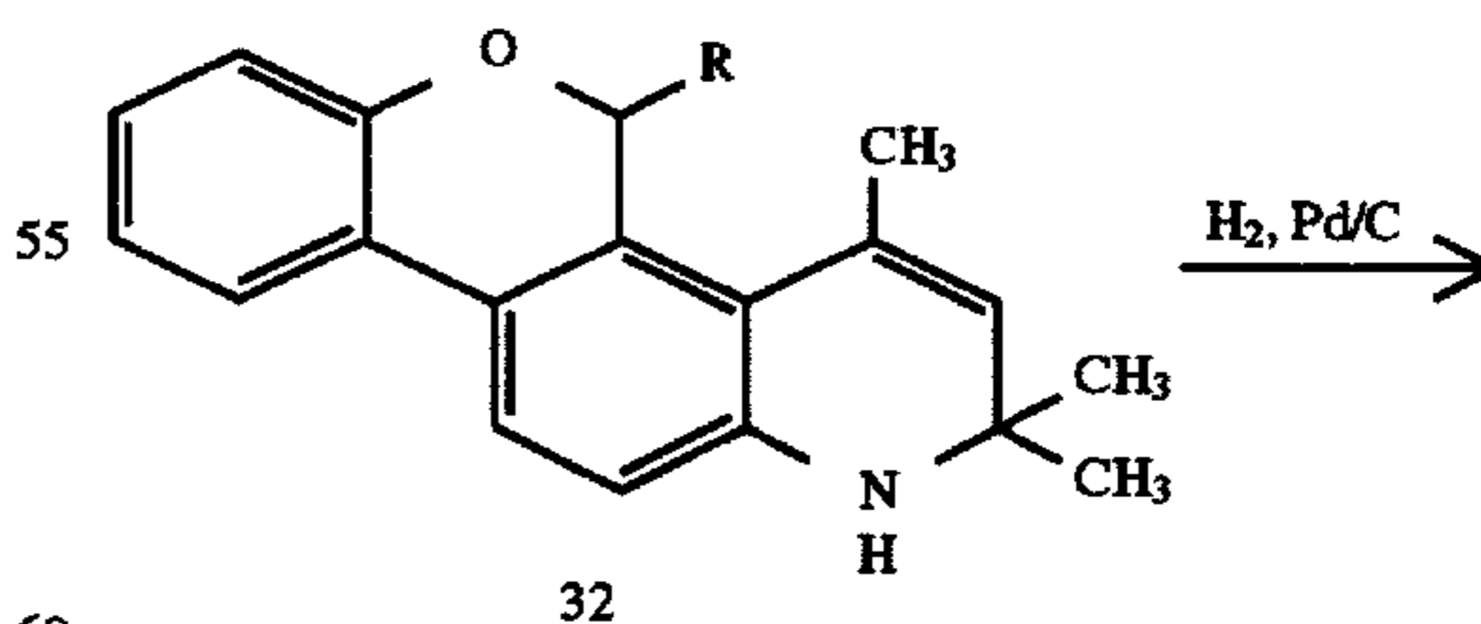
Scheme X
