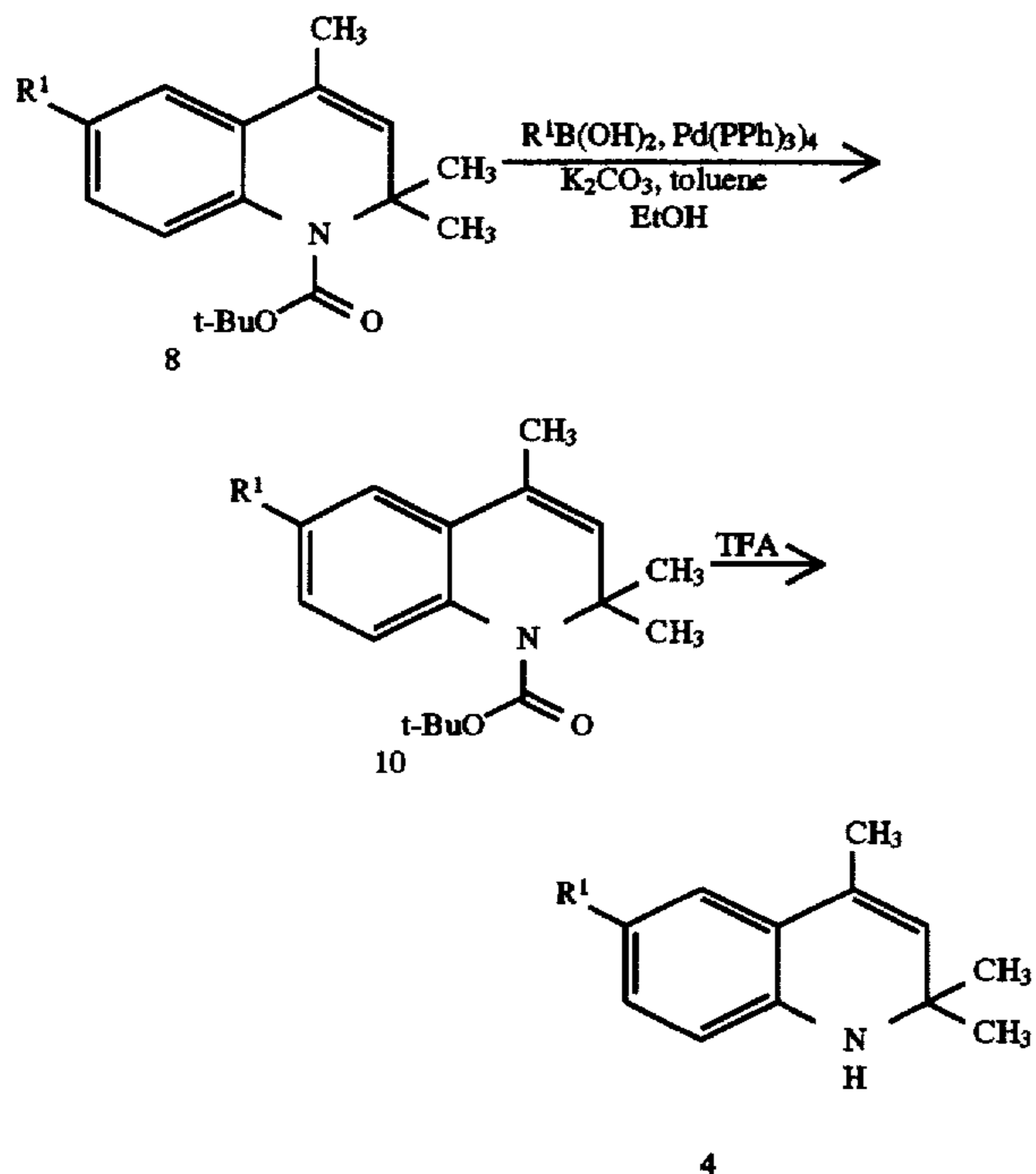
Scheme III
