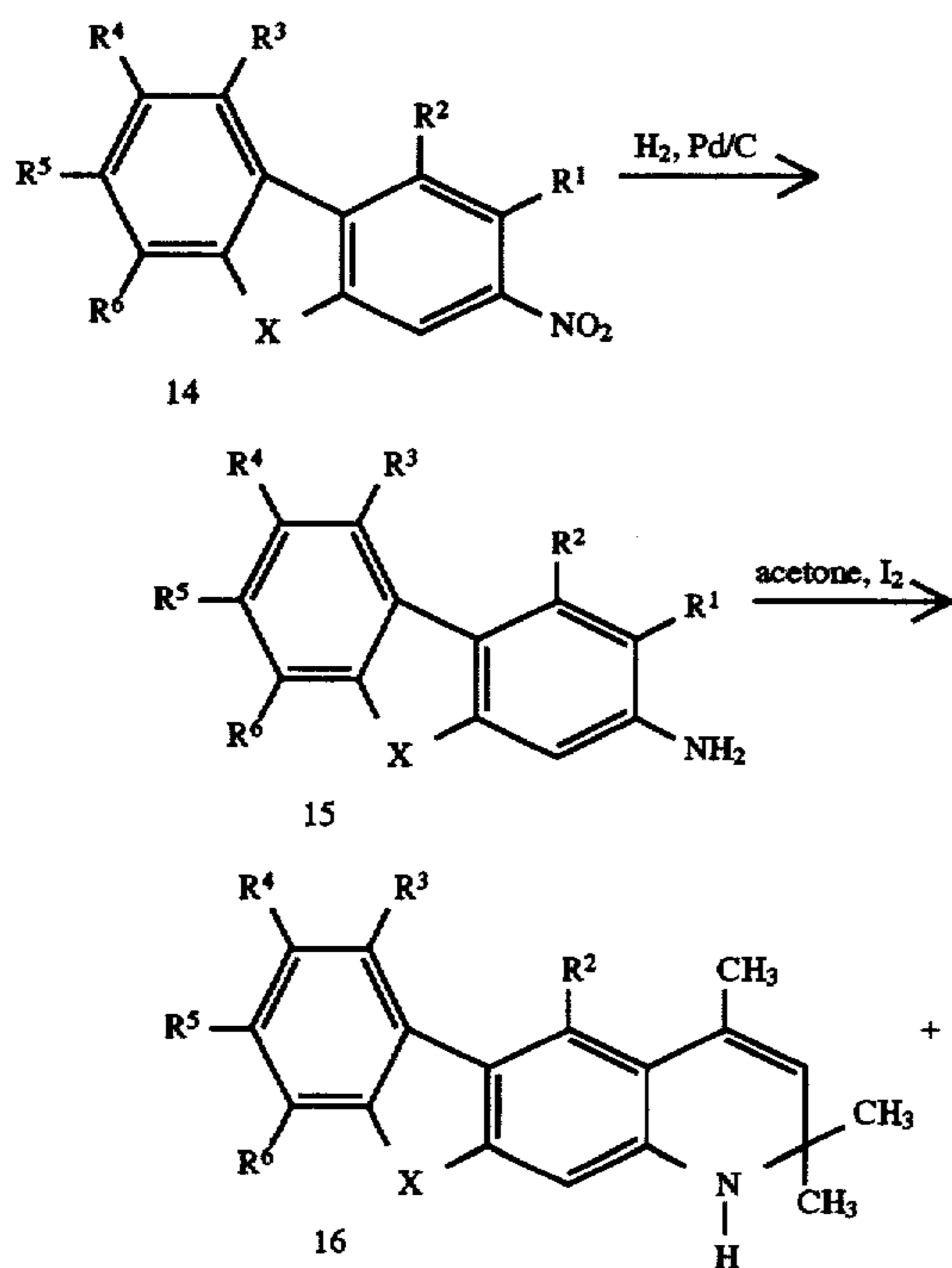
Scheme IV
