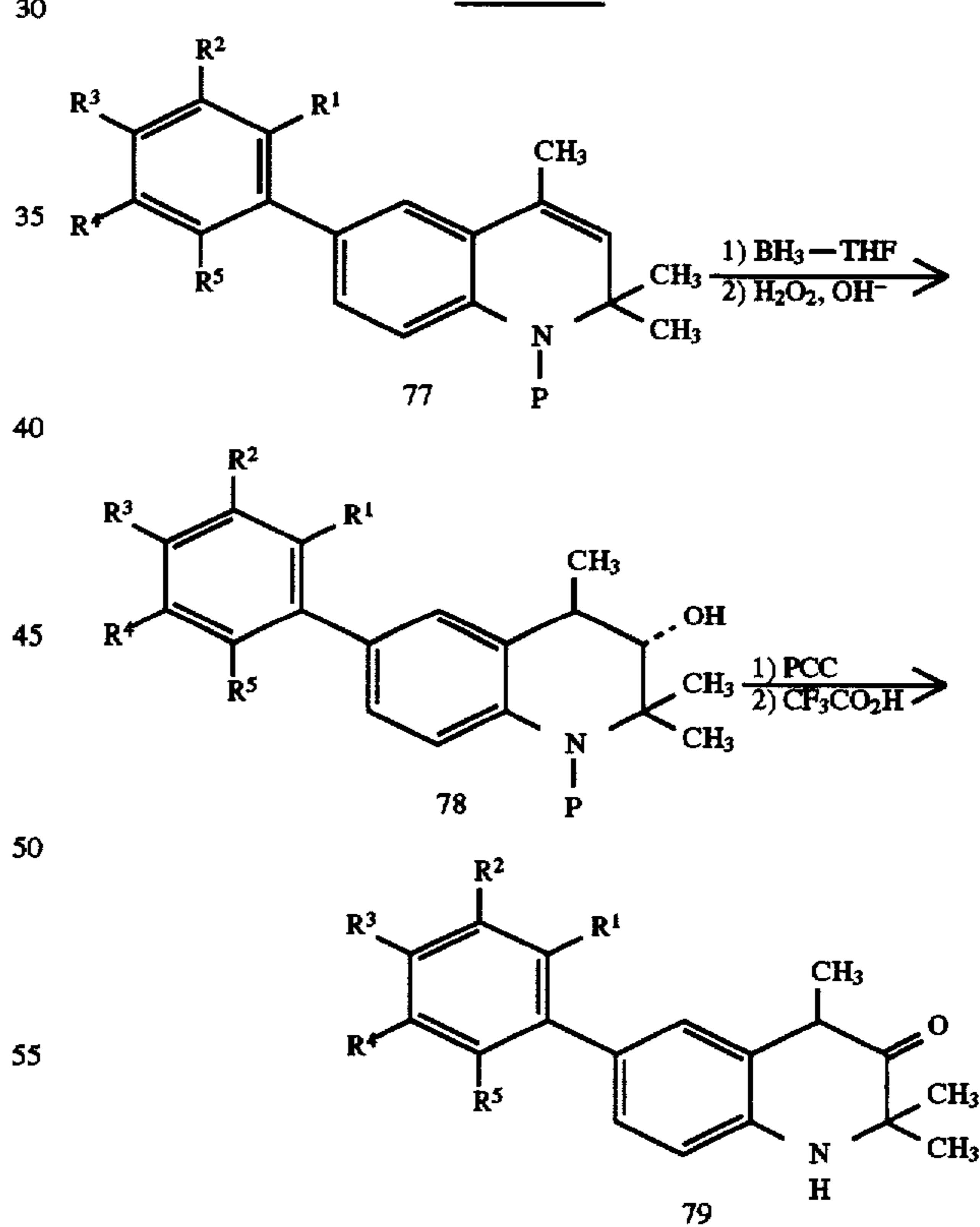
Scheme XX
