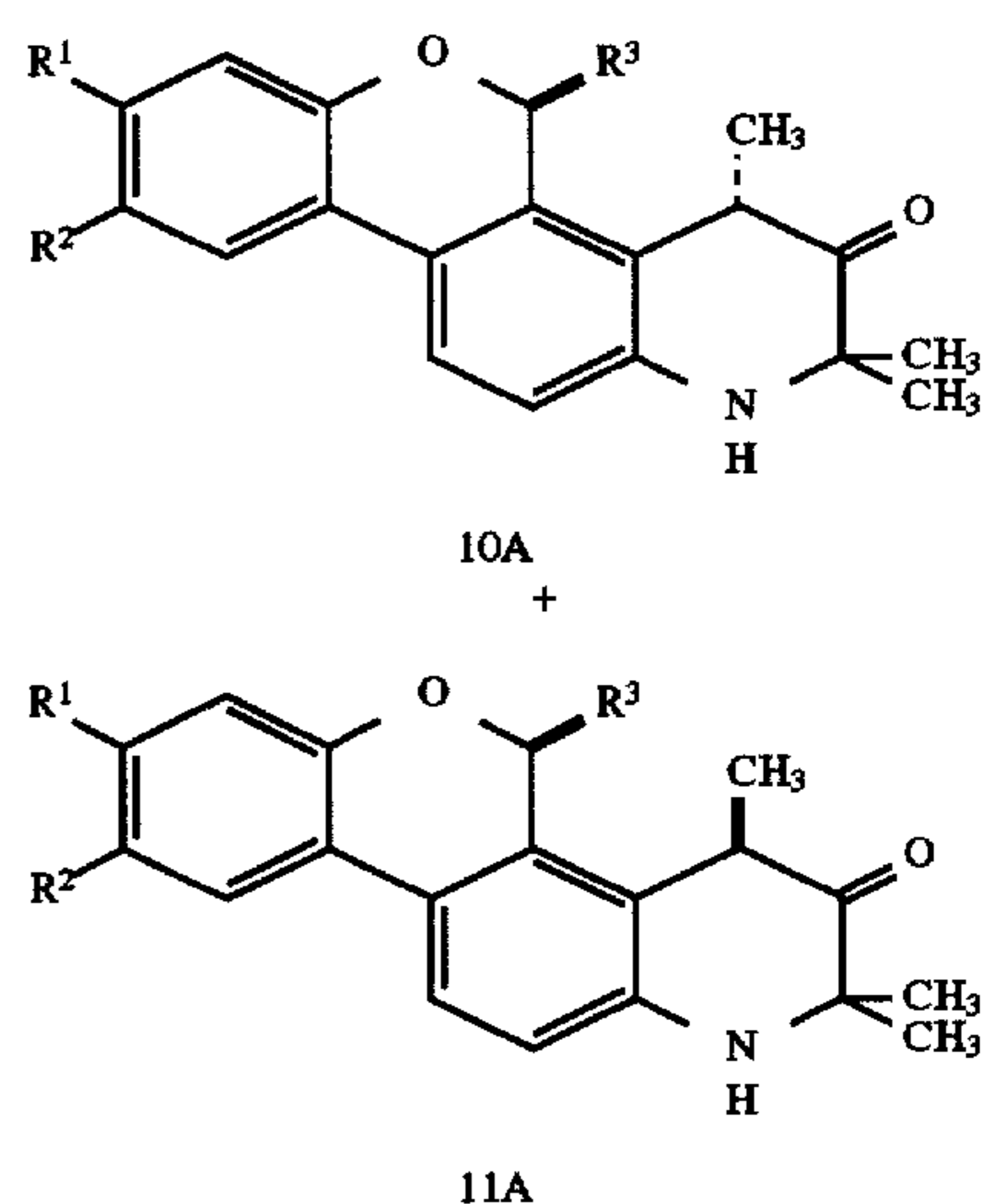
Scheme XXXII
