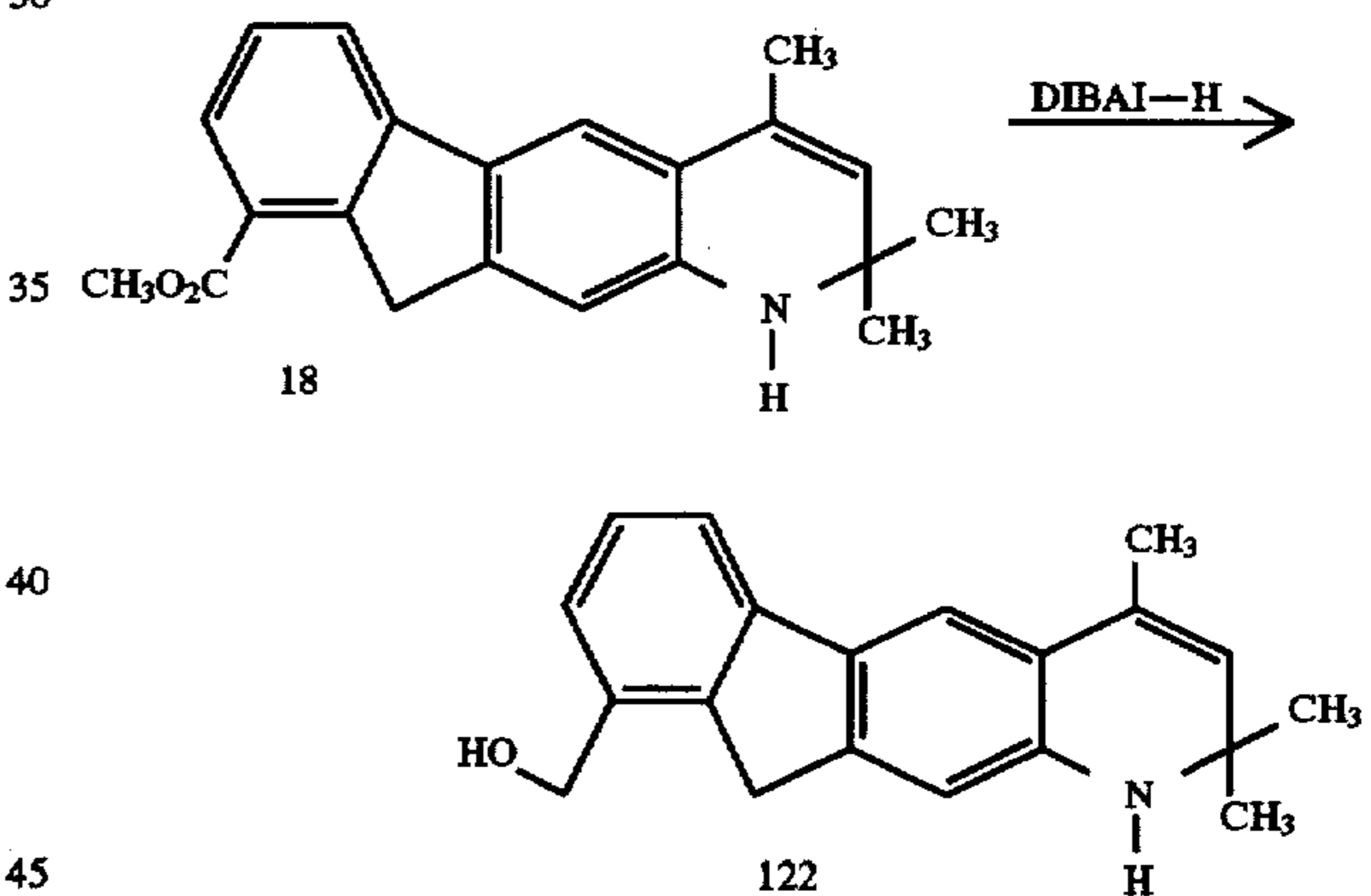
Scheme V
