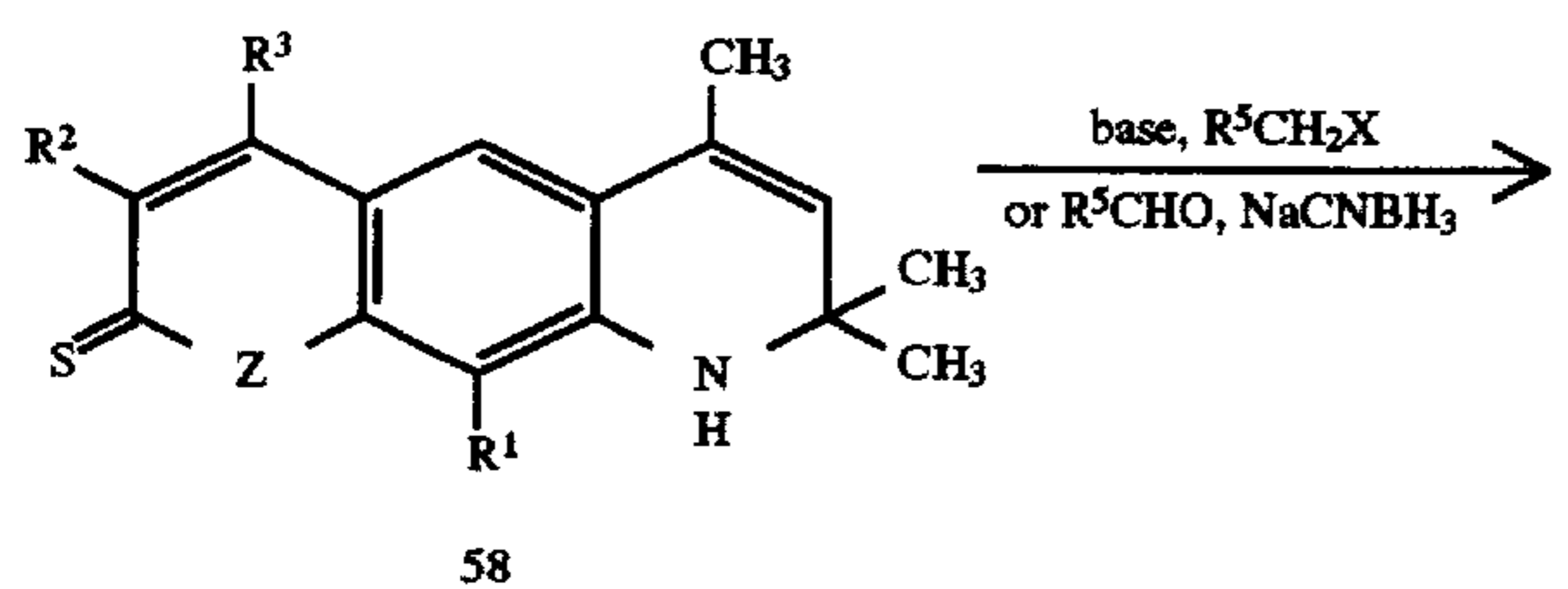
Scheme XXXIX
