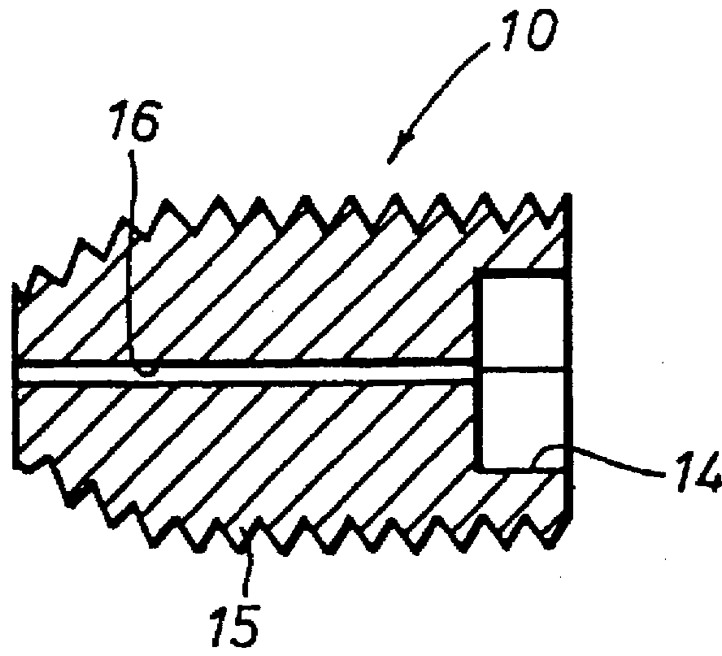
FIG. 2 (PRIOR ART)
