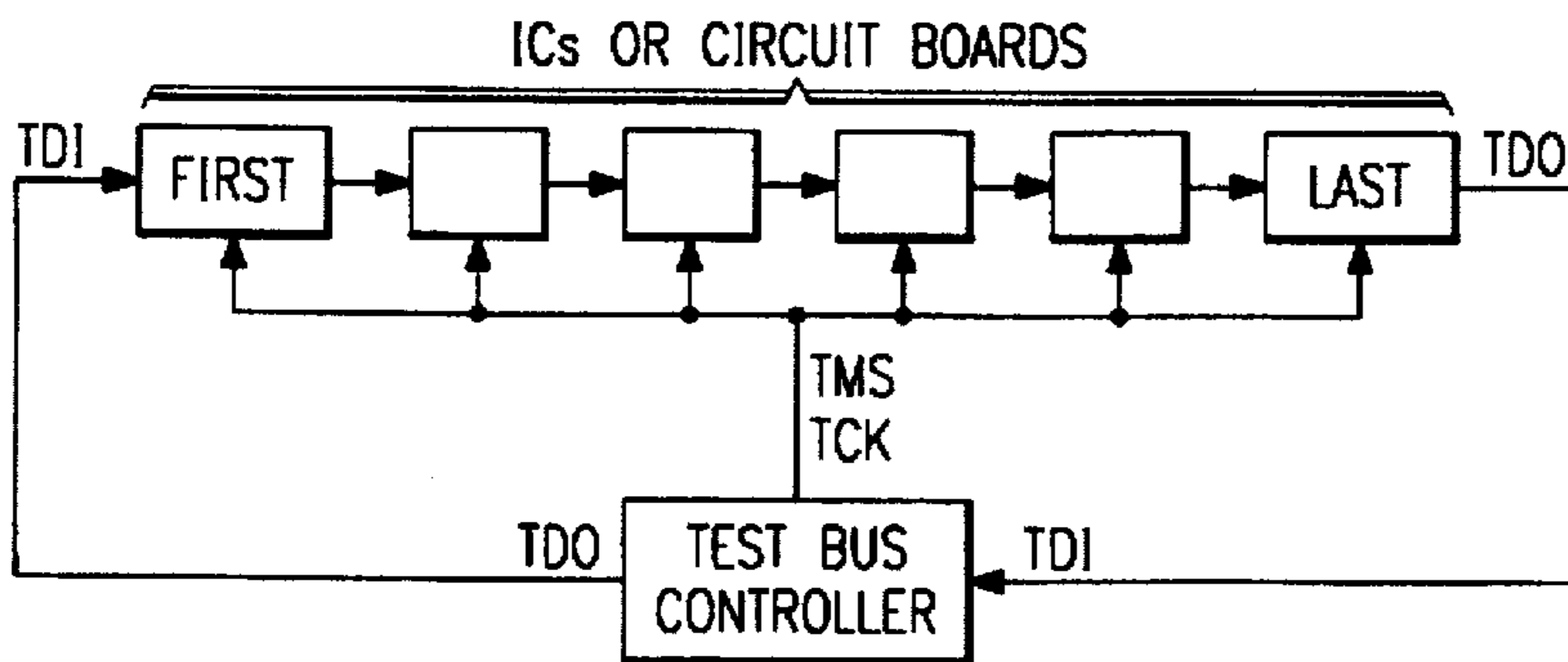
FIG. 3 (PRIOR ART)
