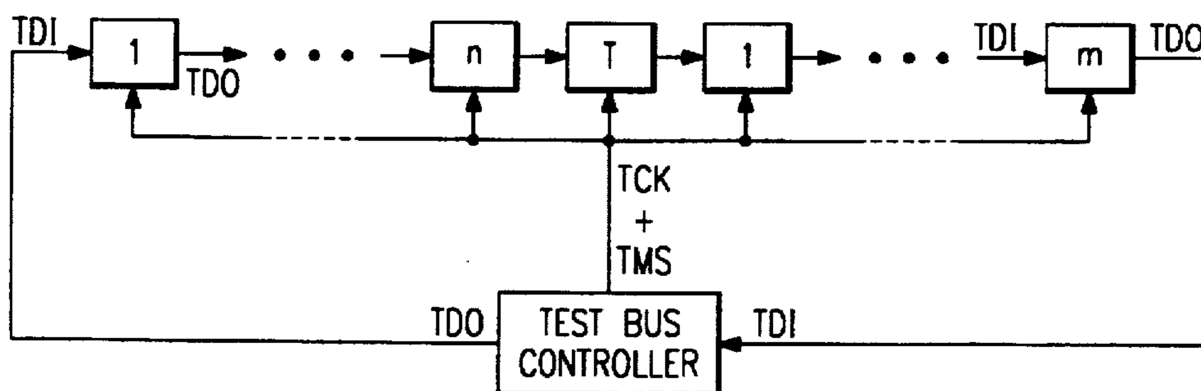
FIG. 7 (PRIOR ART)
