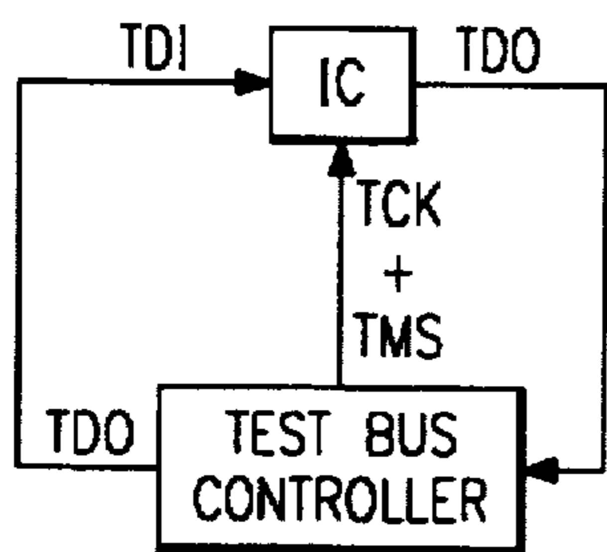
FIG. 4 (PRIOR ART)
