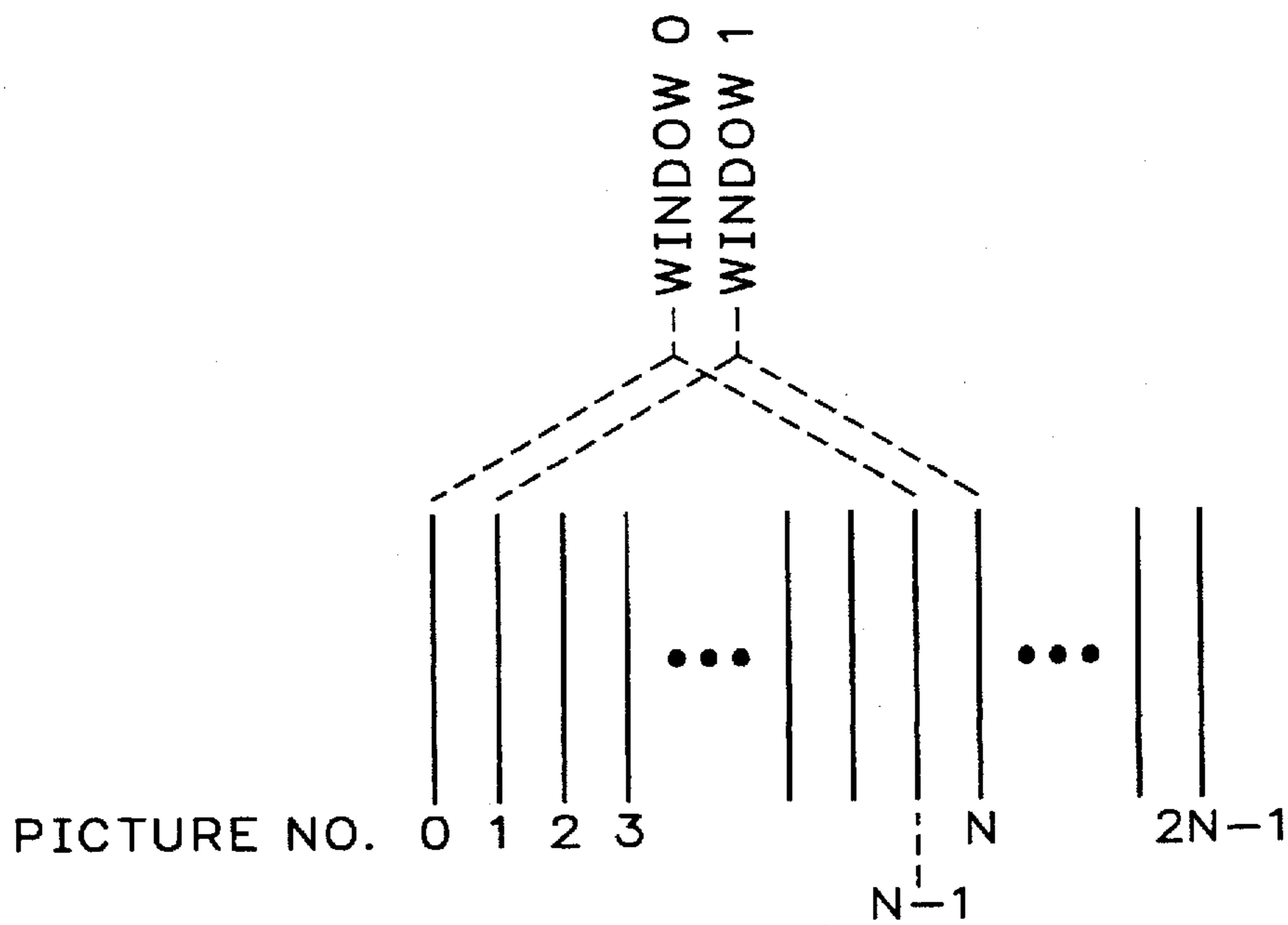
OVERLAPPING WINDOWS
