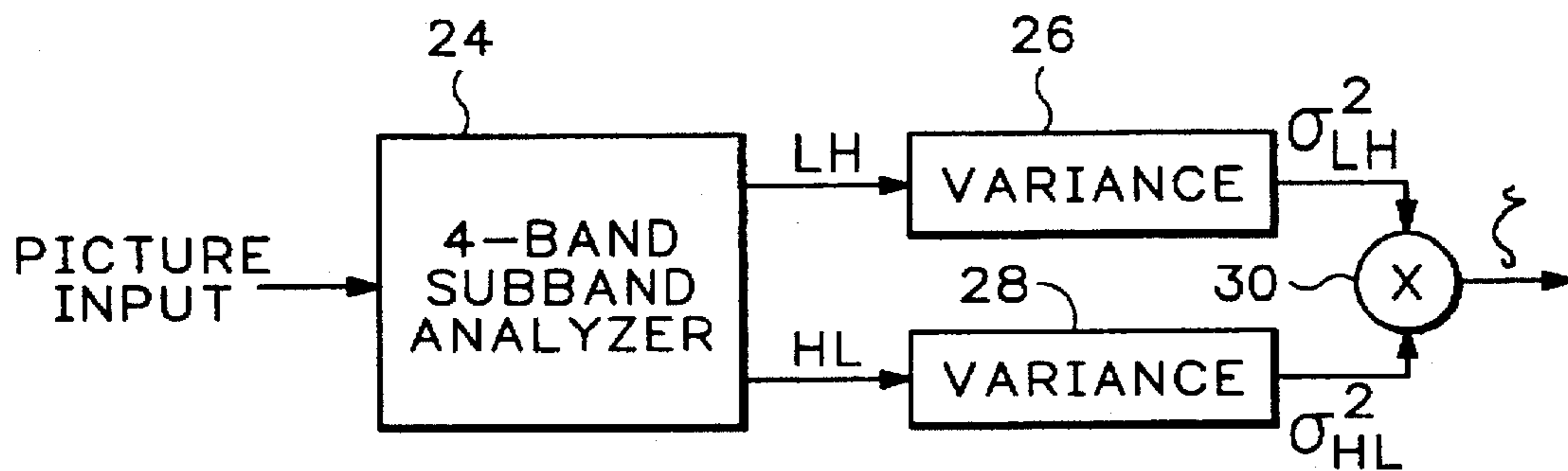
COMPLEXITY PRE-PROCESSOR
