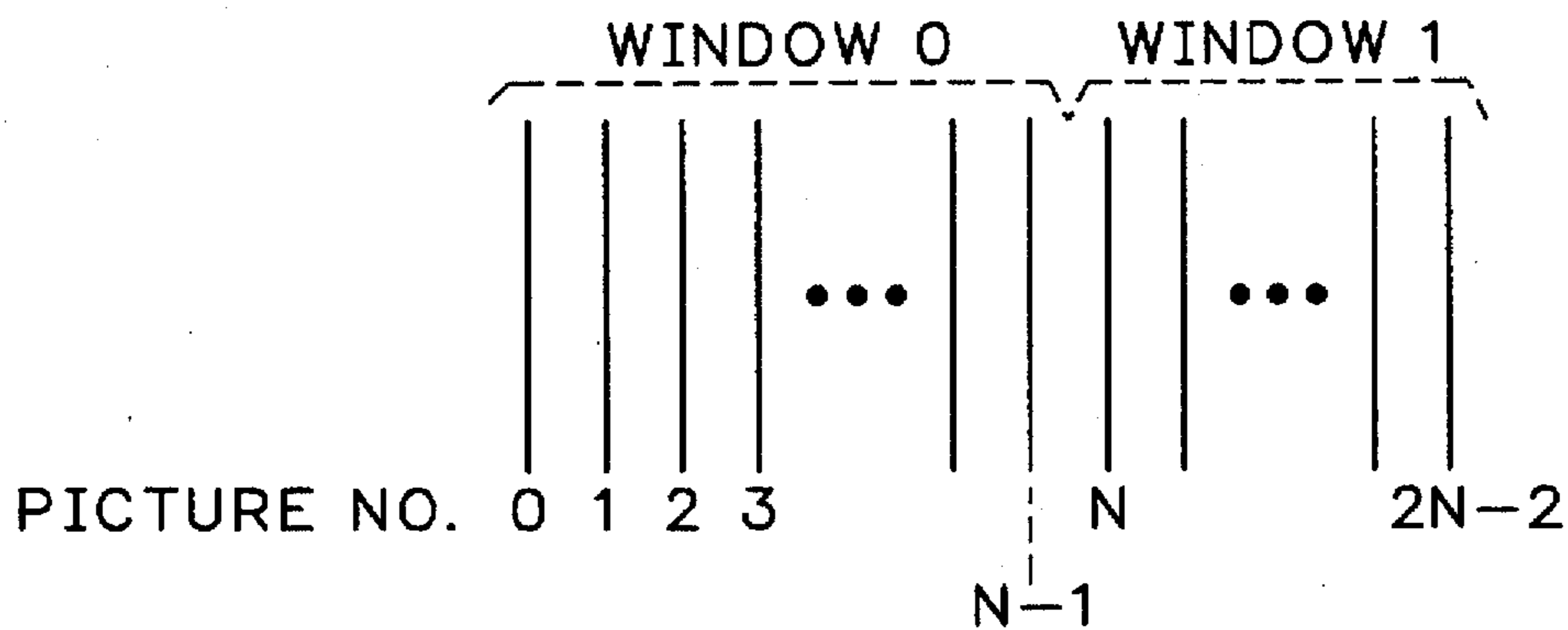
NON-OVERLAPPING WINDOWS
